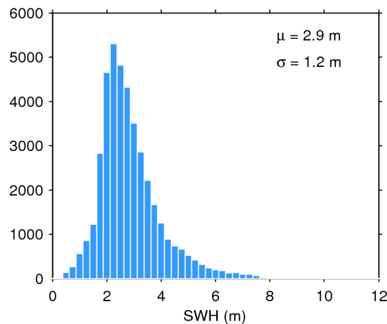
Figure 20. Histogram of science-valid SWH over oceans and lakes for 13/02/2020. The mean ( \mu ) and standard deviation ( \sigma ) are also shown. Note that values larger than 12 m are excluded from the histogram for the sake of readability but not from the computation of \mu and \sigma .
