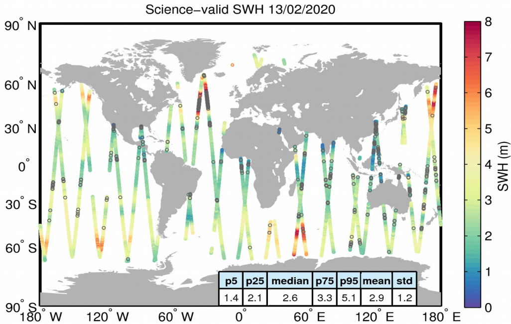
Figure 19. Geographical distribution of science-valid SWH data over oceans and lakes for 13/02/2020. The statistical values shown in the table refer to the SWH in m and are calculated over all measurements shown in the figure. Gray circles denote records that have been rejected based on the editing criteria described in Table 3.
