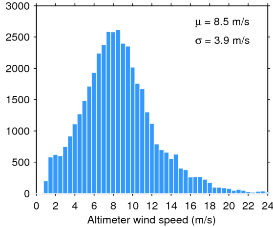
Figure 33. Histogram of flag-valid wind over oceans and lakes for 13/02/2020. The mean ( \mu ) and standard deviation ( \sigma ) are also shown. Note that values larger than 24 m/s are excluded from the histogram for the sake of readability but not from the computation of \mu and \sigma .
