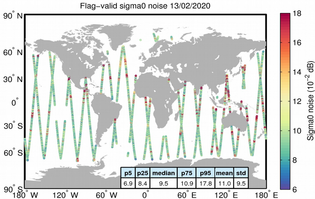
Figure 26. Geographical distribution of flag-valid 20-Hz sigma0 measurement noise over oceans and lakes for 13/02/2020. The statistical values shown in the table refer to the sigma0 noise and are calculated over all measurements shown in the figure.
