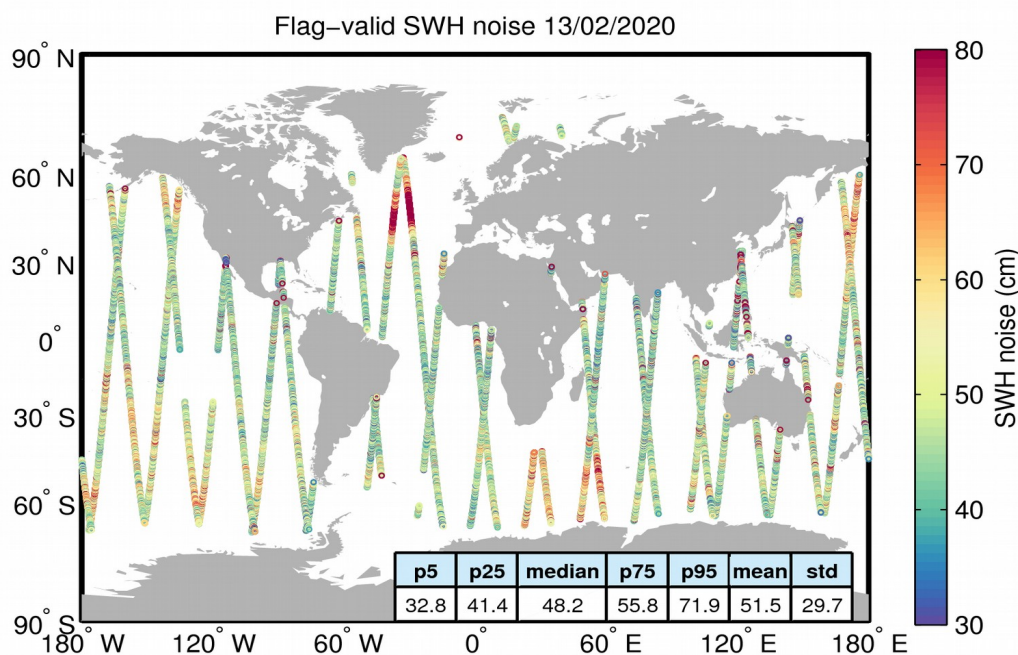
Figure 18. Geographical distribution of flag-valid 20-Hz SWH measurement noise over oceans and lakes for 13/02/2020. The statistical values shown in the figure refer to the SWH noise and are calculated over all measurements shown in the figure.
