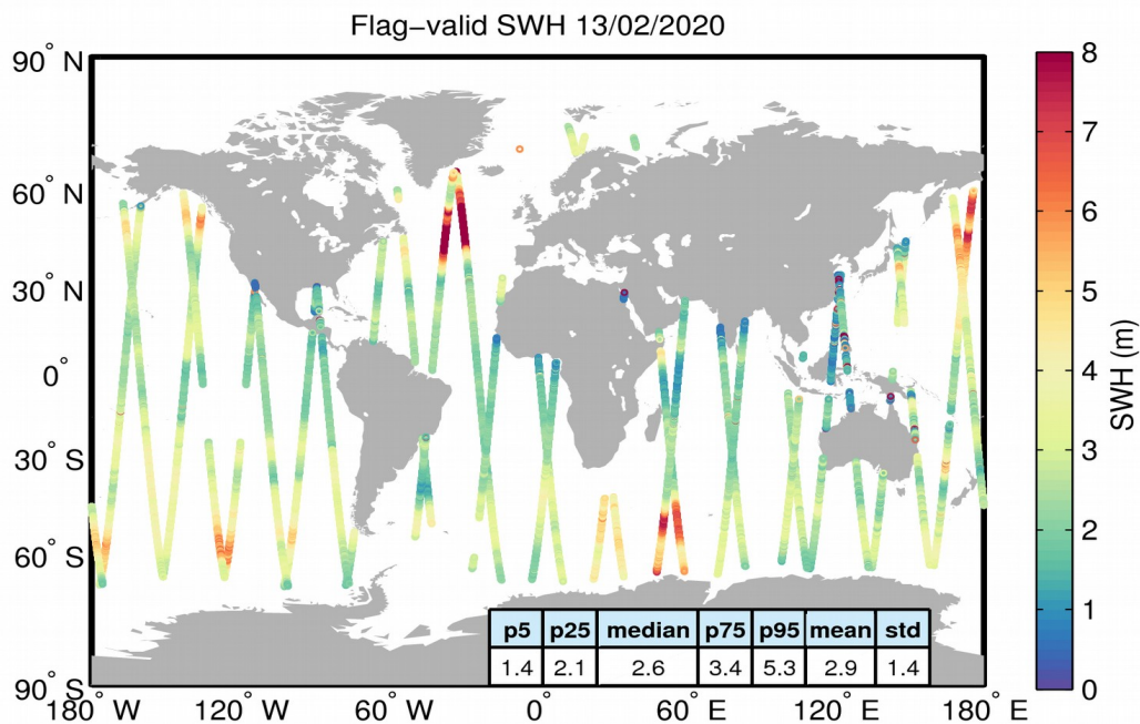
Figure 15. Geographical distribution of flag-valid SWH data over oceans and lakes for 13/02/2020. The statistical values shown in the table refer to the SWH in m and are calculated over all measurements shown in the figure.
