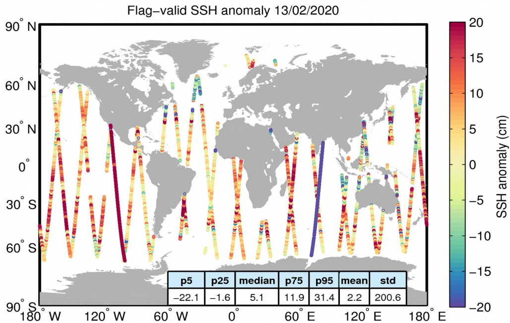
Figure 5. Geographical distribution of flag-valid 1-Hz SSH anomaly data over oceans and lakes for 13/02/2020. The statistical values shown in the table refer to the SSH anomaly in cm and are calculated over all measurements shown in the figure.
