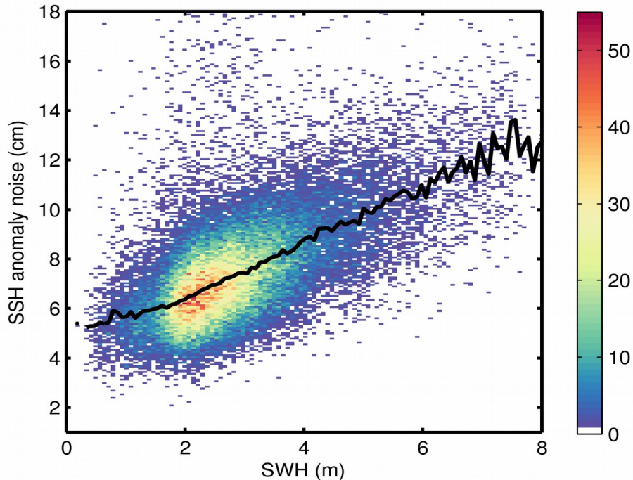
Figure 9. 2D histogram showing flag-valid SSH anomaly noise as a function of SWH for 13/02/2020. The black line denotes the median SSH anomaly noise as a function of SWH.
