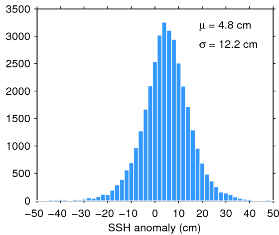
Figure 11. Histogram of science-valid SSH anomaly over oceans and lakes for 13/02/2020. The mean ( \mu ) and standard deviation ( \sigma ) are also shown. Note that values outside [-50 50] cm are excluded from the histogram for the sake of readability but not from the computation of \mu and \sigma .
