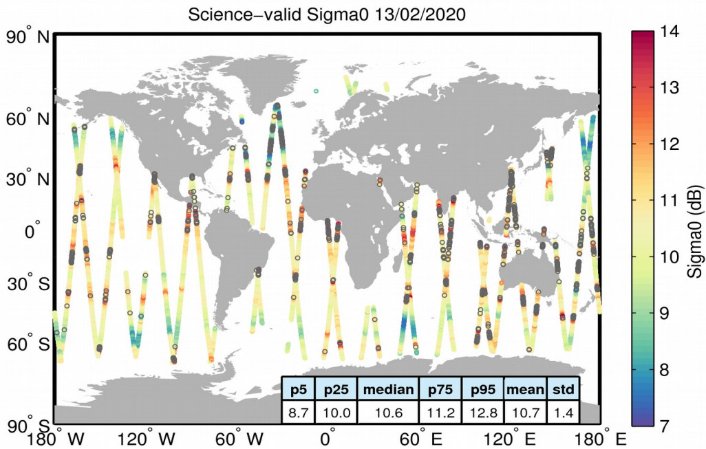
Figure 27. Geographical distribution of science-valid sigma0 data over oceans and lakes for 13/02/2020. The statistical values shown in the table refer to the sigma0 in dB and are calculated over all measurements shown in the figure. Gray circles denote records that have been rejected based on the editing criteria described in Table 4.
