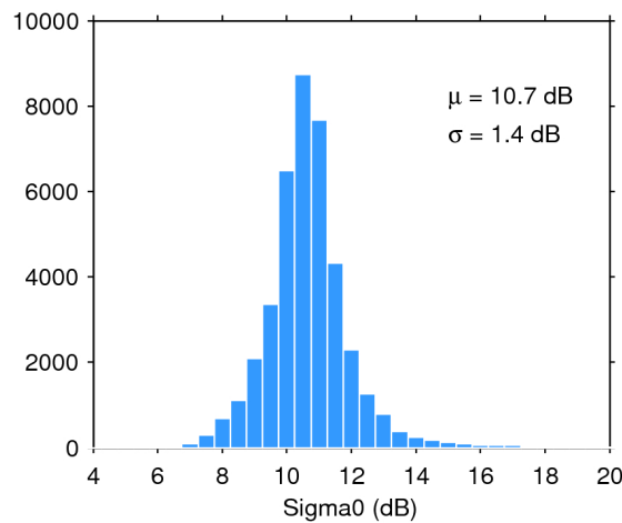
Figure 28. Histogram of science-valid sigma0 over oceans and lakes for 13/02/2020. The mean ( \mu ) and standard deviation ( \sigma ) are also shown. Note that values outside [4 20] dB are excluded from the histogram for the sake of readability but not from the computation of \mu and \sigma .
