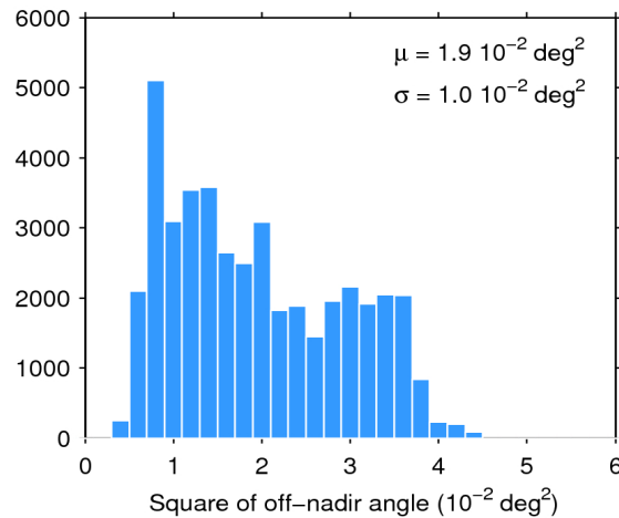
Figure 39. Histogram of flag-valid mispointing over oceans and lakes for 13/02/2020. The mean ( \mu ) and standard deviation ( \sigma ) are also shown. Note that values larger than 6 \cdot 10^{-2} \text{ deg}^2 are excluded from the histogram for the sake of readability but not from the computation of \mu and \sigma .
