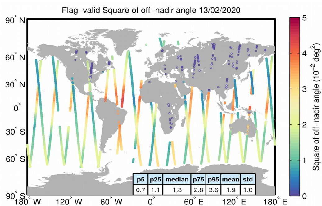
Figure 37. Geographical distribution of flag-valid mispointing data over oceans and lakes for 13/02/2020. The statistical values shown in the table refer to the mispointing in 10^{-2} deg 2 and are calculated over all measurements shown in the figure.
