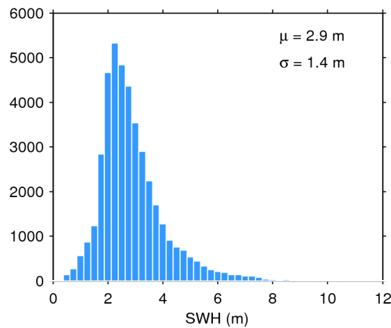
Figure 17. Histogram of flag-valid SWH over oceans and lakes for 13/02/2020. The mean ( \mu ) and standard deviation ( \sigma ) are also shown. Note that values larger than 12 m are excluded from the histogram for the sake of readability but not from the computation of \mu and \sigma .
