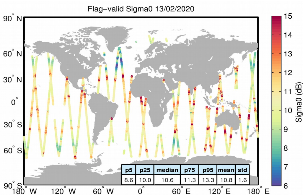
Figure 23. Geographical distribution of flag-valid sigma0 data over oceans and lakes for 13/02/2020. The statistical values shown in the table refer to the sigma0 in dB and are calculated over all measurements shown in the figure.
