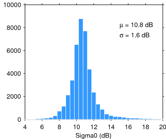
Figure 25. Histogram of flag-valid sigma0 over oceans and lakes for 13/02/2020. The mean ( \mu ) and standard deviation ( \sigma ) are also shown. Note that values outside [4 20] dB are excluded from the histogram for the sake of readability but not from the computation of \mu and \sigma .
