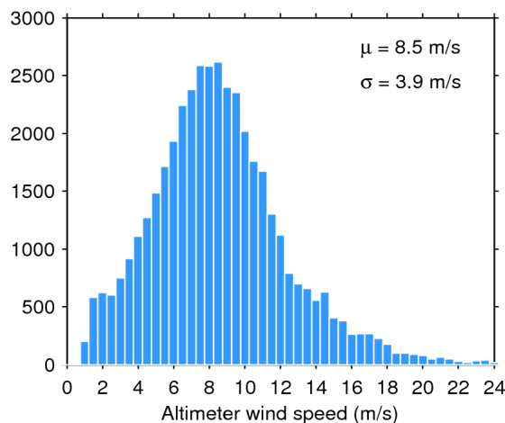
Figure 35. Histogram of science-valid wind over oceans and lakes for 13/02/2020. The mean ( \mu ) and standard deviation ( \sigma ) are also shown. Note that values larger than 24 m/s are excluded from the histogram for the sake of readability but not from the computation of \mu and \sigma .
