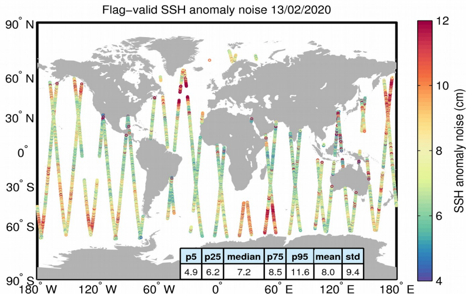
Figure 8. Geographical distribution of flag-valid 20-Hz SSH anomaly measurement noise over oceans and lakes for 13/02/2020. The statistical values shown in the table refer to the SSH anomaly noise and are calculated over all measurements shown in the figure.
