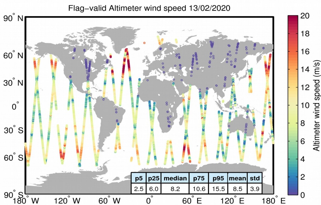
Figure 31. Geographical distribution of flag-valid wind data over oceans and lakes for 13/02/2020. The statistical values shown in the table refer to the wind in m/s and are calculated over all measurements shown in the figure.
