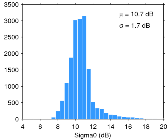
Figure 25. Histogram of flag-valid sigma0 over oceans and lakes for 12/02/2020. The mean ( \mu ) and standard deviation ( \sigma ) are also shown. Note that values outside [4 20] dB are excluded from the histogram for the sake of readability but not from the computation of \mu and \sigma .
