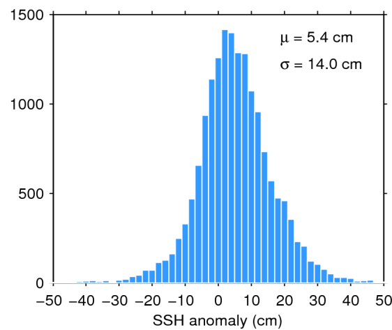
Figure 7. Histogram of flag-valid SSH anomaly over oceans and lakes for 12/02/2020. The mean ( \mu ) and standard deviation ( \sigma ) are also shown. Note that values outside [-50 50] cm are excluded from the histogram for the sake of readability but not from the computation of \mu and \sigma .
