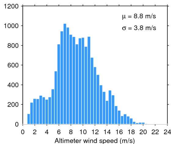
Figure 35. Histogram of science-valid wind over oceans and lakes for 12/02/2020. The mean ( \mu ) and standard deviation ( \sigma ) are also shown. Note that values larger than 24 m/s are excluded from the histogram for the sake of readability but not from the computation of \mu and \sigma .
