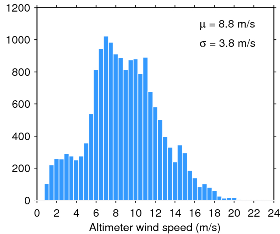
Figure 33. Histogram of flag-valid wind over oceans and lakes for 12/02/2020. The mean ( \mu ) and standard deviation ( \sigma ) are also shown. Note that values larger than 24 m/s are excluded from the histogram for the sake of readability but not from the computation of \mu and \sigma .
