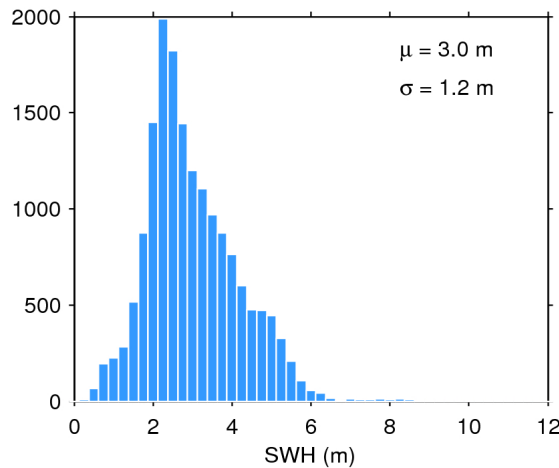
Figure 20. Histogram of science-valid SWH over oceans and lakes for 12/02/2020. The mean ( \mu ) and standard deviation ( \sigma ) are also shown. Note that values larger than 12 m are excluded from the histogram for the sake of readability but not from the computation of \mu and \sigma .
