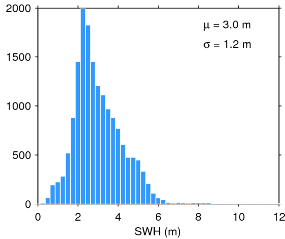
Figure 17. Histogram of flag-valid SWH over oceans and lakes for 12/02/2020. The mean ( \mu ) and standard deviation ( \sigma ) are also shown. Note that values larger than 12 m are excluded from the histogram for the sake of readability but not from the computation of \mu and \sigma .
