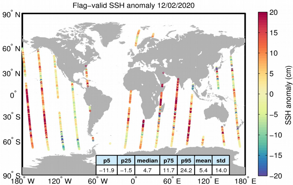
Figure 5. Geographical distribution of flag-valid 1-Hz SSH anomaly data over oceans and lakes for 12/02/2020. The statistical values shown in the table refer to the SSH anomaly in cm and are calculated over all measurements shown in the figure.
