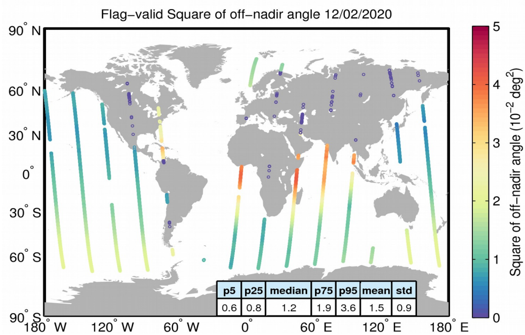
Figure 37. Geographical distribution of flag-valid mispointing data over oceans and lakes for 12/02/2020. The statistical values shown in the table refer to the mispointing in 10^{-2} \text{ deg}^2 and are calculated over all measurements shown in the figure.
