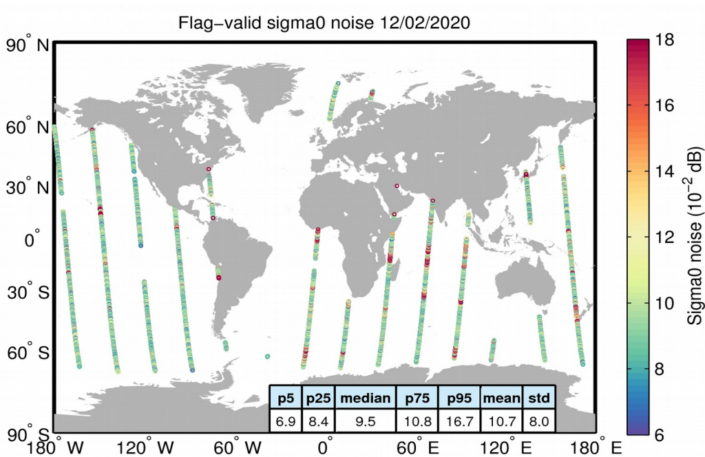
Figure 26. Geographical distribution of flag-valid 20-Hz sigma0 measurement noise over oceans and lakes for 12/02/2020. The statistical values shown in the table refer to the sigma0 noise and are calculated over all measurements shown in the figure.
