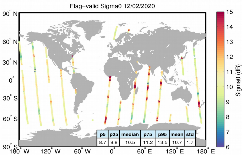
Figure 23. Geographical distribution of flag-valid sigma0 data over oceans and lakes for 12/02/2020. The statistical values shown in the table refer to the sigma0 in dB and are calculated over all measurements shown in the figure.
