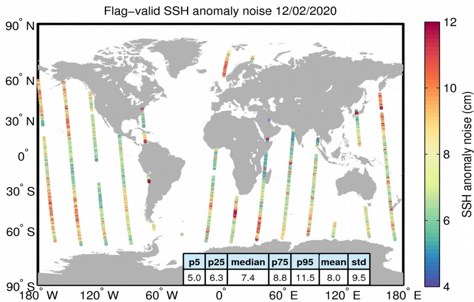
Figure 8. Geographical distribution of flag-valid 20-Hz SSH anomaly measurement noise over oceans and lakes for 12/02/2020. The statistical values shown in the table refer to the SSH anomaly noise and are calculated over all measurements shown in the figure.
