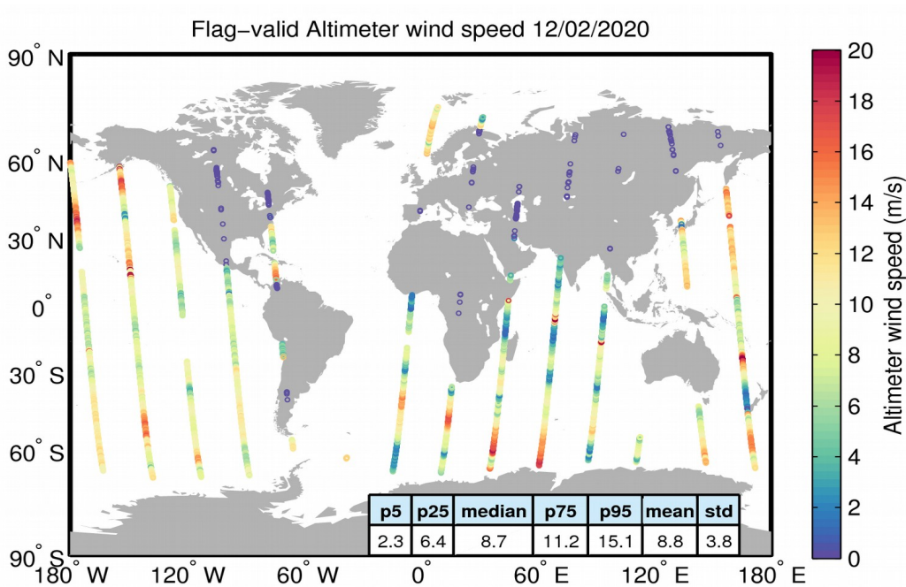
Figure 31. Geographical distribution of flag-valid wind data over oceans and lakes for 12/02/2020. The statistical values shown in the table refer to the wind in m/s and are calculated over all measurements shown in the figure.
