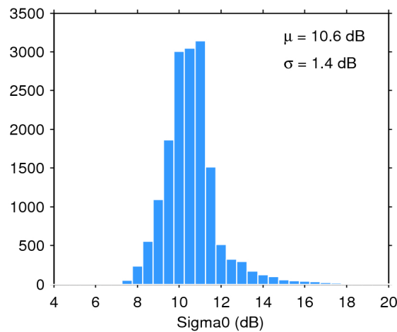
Figure 28. Histogram of science-valid sigma0 over oceans and lakes for 12/02/2020. The mean ( \mu ) and standard deviation ( \sigma ) are also shown. Note that values outside [4 20] dB are excluded from the histogram for the sake of readability but not from the computation of \mu and \sigma .
