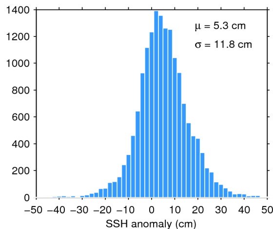
Figure 11. Histogram of science-valid SSH anomaly over oceans and lakes for 12/02/2020. The mean ( \mu ) and standard deviation ( \sigma ) are also shown. Note that values outside [-50, 50] cm are excluded from the histogram for the sake of readability but not from the computation of \mu and \sigma .
