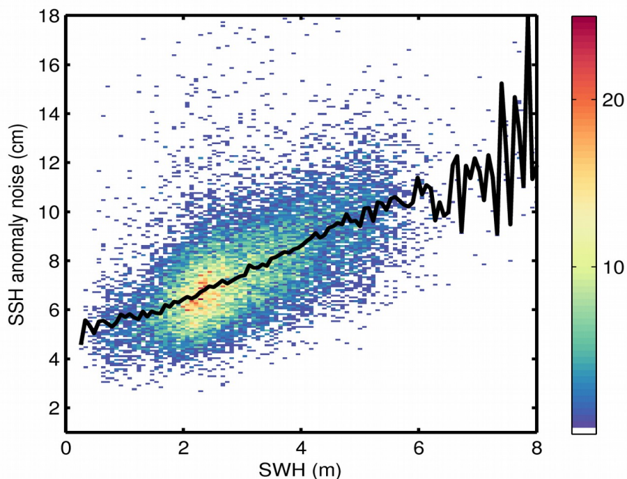
Figure 9. 2D histogram showing flag-valid SSH anomaly noise as a function of SWH for 12/02/2020. The black line denotes the median SSH anomaly noise as a function of SWH.
