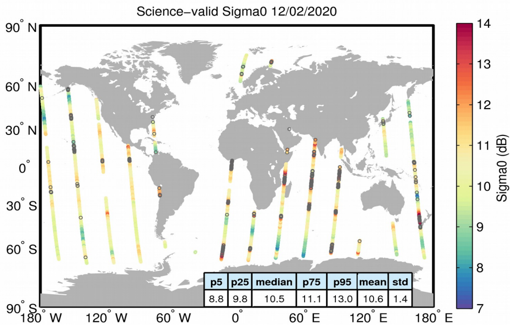
Figure 27. Geographical distribution of science-valid sigma0 data over oceans and lakes for 12/02/2020. The statistical values shown in the table refer to the sigma0 in dB and are calculated over all measurements shown in the figure. Gray circles denote records that have been rejected based on the editing criteria described in Table 4.
