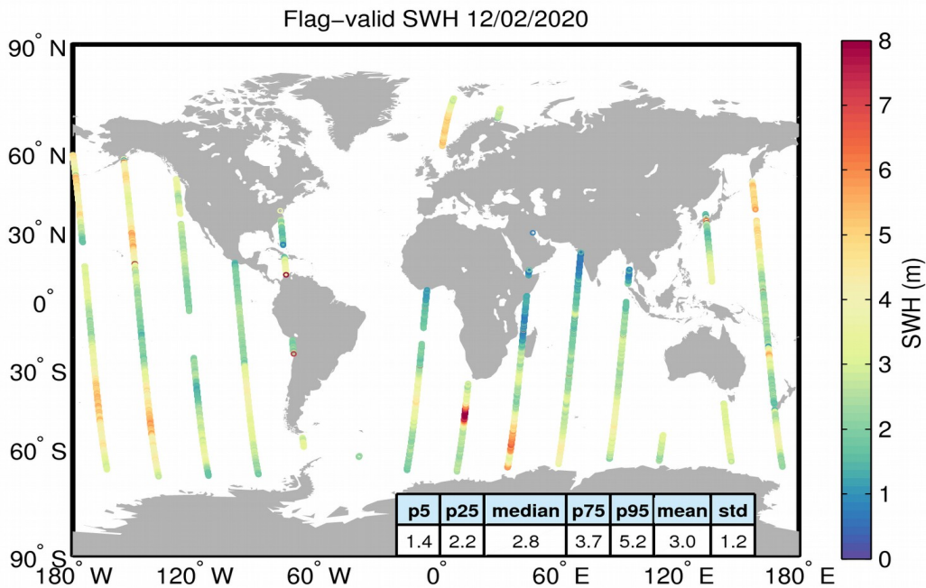
Figure 15. Geographical distribution of flag-valid SWH data over oceans and lakes for 12/02/2020. The statistical values shown in the table refer to the SWH in m and are calculated over all measurements shown in the figure.
