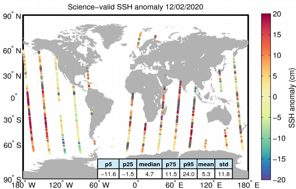
Figure 10. Geographical distribution of science-valid SSH anomaly data over oceans and lakes for 12/02/2020. The statistical values shown in the table refer to the SSH anomaly in cm and are calculated over all measurements shown in the figure. Gray circles denote records that have been rejected based on the editing criteria described in Table 2.
