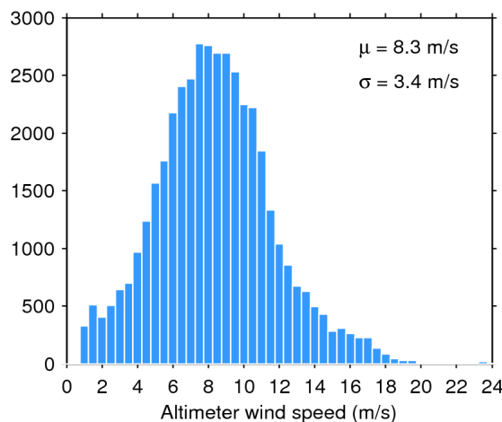
Figure 35. Histogram of science-valid wind over oceans and lakes for 11/02/2020. The mean ( \mu ) and standard deviation ( \sigma ) are also shown. Note that values larger than 24 m/s are excluded from the histogram for the sake of readability but not from the computation of \mu and \sigma .
