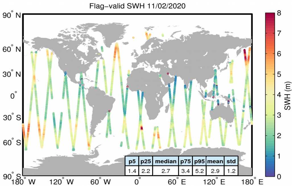
Figure 15. Geographical distribution of flag-valid SWH data over oceans and lakes for 11/02/2020. The statistical values shown in the table refer to the SWH in m and are calculated over all measurements shown in the figure.
