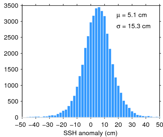
Figure 7. Histogram of flag-valid SSH anomaly over oceans and lakes for 11/02/2020. The mean ( \mu ) and standard deviation ( \sigma ) are also shown. Note that values outside [-50 50] cm are excluded from the histogram for the sake of readability but not from the computation of \mu and \sigma .
