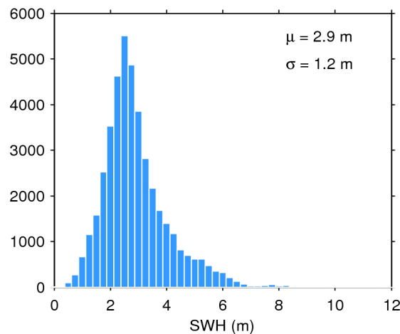
Figure 17. Histogram of flag-valid SWH over oceans and lakes for 11/02/2020. The mean ( \mu ) and standard deviation ( \sigma ) are also shown. Note that values larger than 12 m are excluded from the histogram for the sake of readability but not from the computation of \mu and \sigma .
