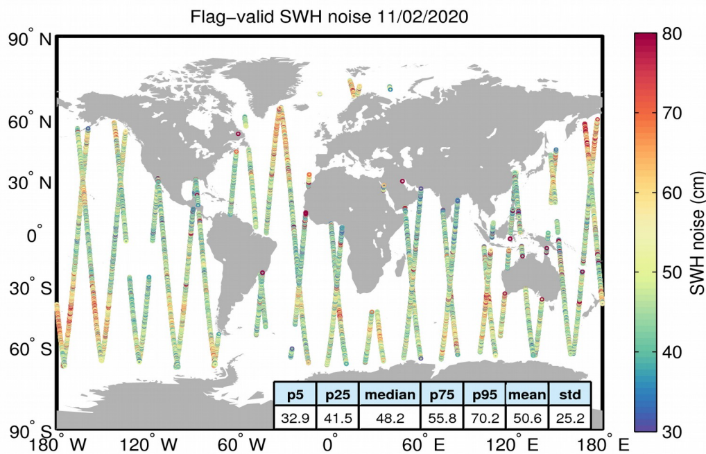
Figure 18. Geographical distribution of flag-valid 20-Hz SWH measurement noise over oceans and lakes for 11/02/2020. The statistical values shown in the figure refer to the SWH noise and are calculated over all measurements shown in the figure.
