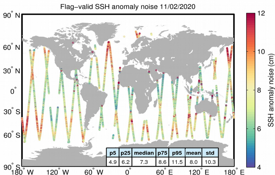
Figure 8. Geographical distribution of flag-valid 20-Hz SSH anomaly measurement noise over oceans and lakes for 11/02/2020. The statistical values shown in the table refer to the SSH anomaly noise and are calculated over all measurements shown in the figure.
