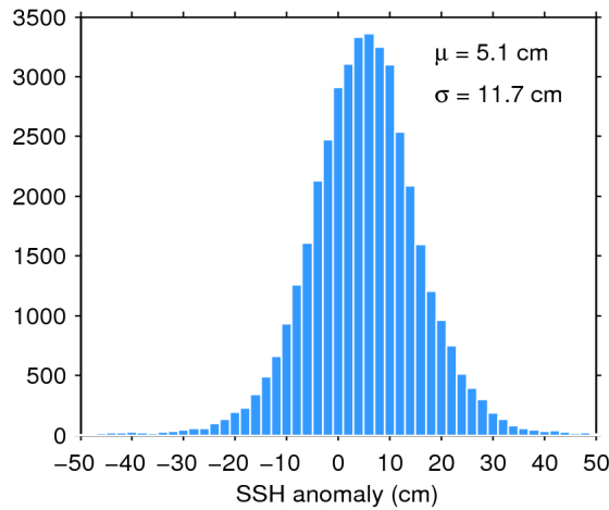
Figure 11. Histogram of science-valid SSH anomaly over oceans and lakes for 11/02/2020. The mean ( \mu ) and standard deviation ( \sigma ) are also shown. Note that values outside [-50 50] cm are excluded from the histogram for the sake of readability but not from the computation of \mu and \sigma .
