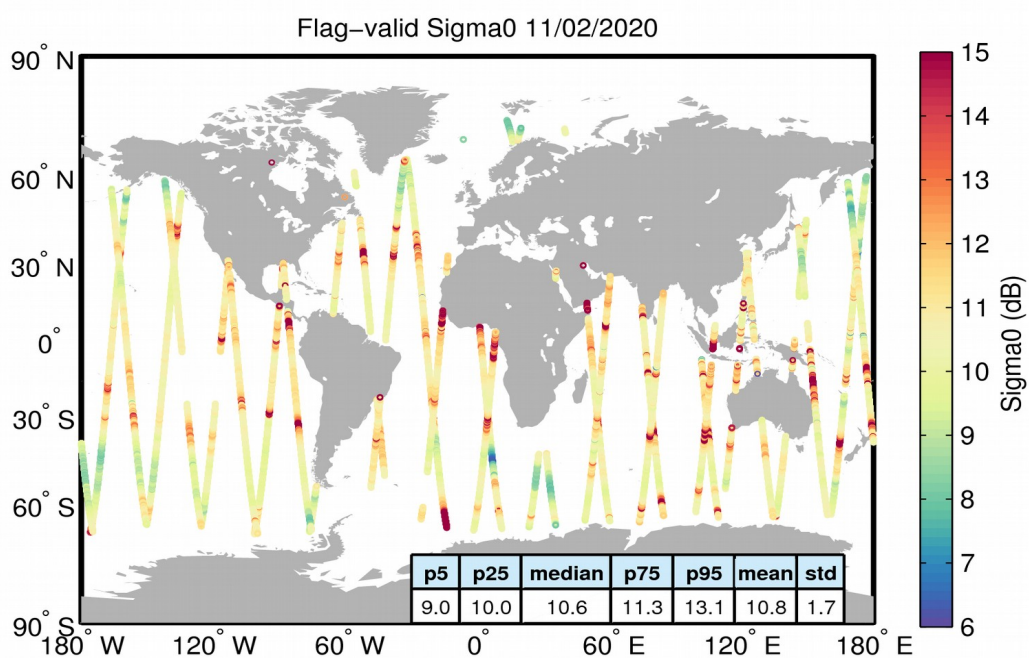
Figure 23. Geographical distribution of flag-valid sigma0 data over oceans and lakes for 11/02/2020. The statistical values shown in the table refer to the sigma0 in dB and are calculated over all measurements shown in the figure.
