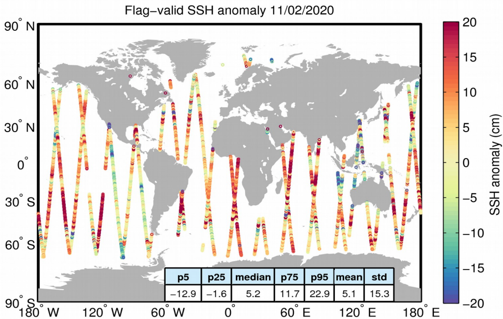
Figure 5. Geographical distribution of flag-valid 1-Hz SSH anomaly data over oceans and lakes for 11/02/2020. The statistical values shown in the table refer to the SSH anomaly in cm and are calculated over all measurements shown in the figure.
