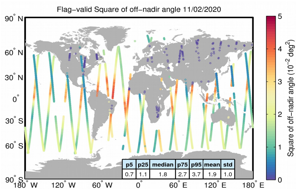
Figure 37. Geographical distribution of flag-valid mispointing data over oceans and lakes for 11/02/2020. The statistical values shown in the table refer to the mispointing in 10^{-2} \text{deg}^2 and are calculated over all measurements shown in the figure.
