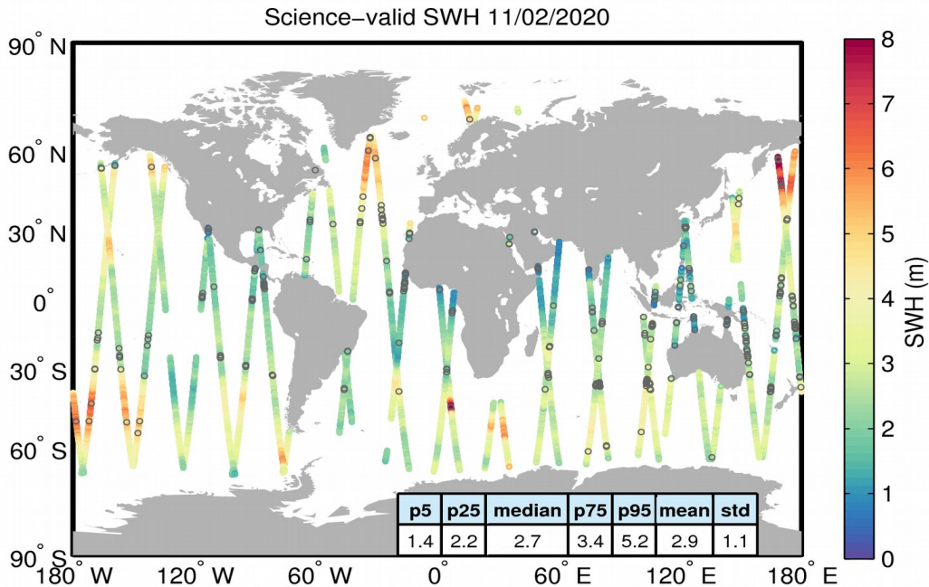
Figure 19. Geographical distribution of science-valid SWH data over oceans and lakes for 11/02/2020. The statistical values shown in the table refer to the SWH in m and are calculated over all measurements shown in the figure. Gray circles denote records that have been rejected based on the editing criteria described in Table 3.
