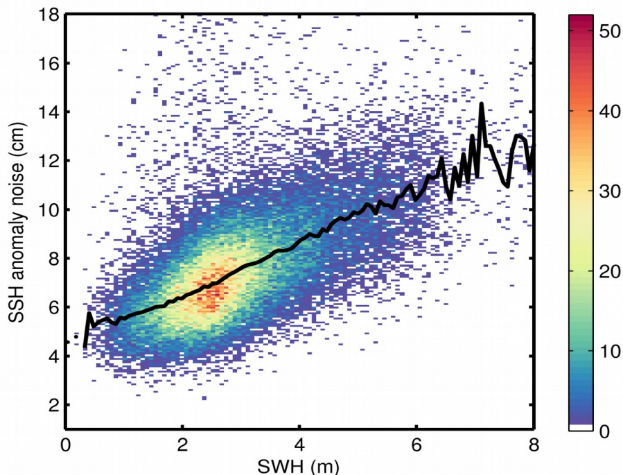
Figure 9. 2D histogram showing flag-valid SSH anomaly noise as a function of SWH for 11/02/2020. The black line denotes the median SSH anomaly noise as a function of SWH.
