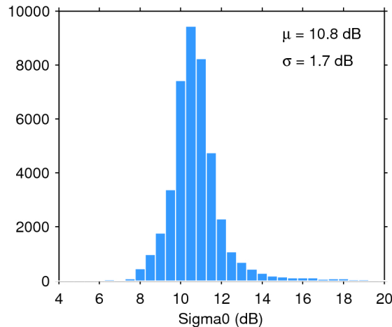
Figure 25. Histogram of flag-valid sigma0 over oceans and lakes for 11/02/2020. The mean ( \mu ) and standard deviation ( \sigma ) are also shown. Note that values outside [4 20] dB are excluded from the histogram for the sake of readability but not from the computation of \mu and \sigma .
