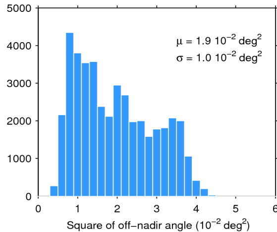
Figure 39. Histogram of flag-valid mispointing over oceans and lakes for 11/02/2020. The mean ( \mu ) and standard deviation ( \sigma ) are also shown. Note that values larger than 6 \cdot 10^{-2} \text{ deg}^2 are excluded from the histogram for the sake of readability but not from the computation of \mu and \sigma .
