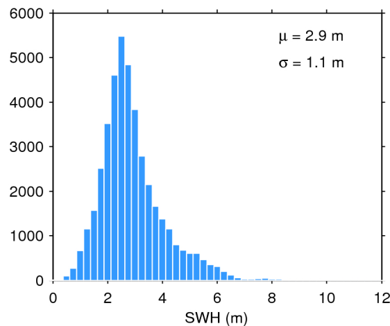
Figure 20. Histogram of science-valid SWH over oceans and lakes for 11/02/2020. The mean ( \mu ) and standard deviation ( \sigma ) are also shown. Note that values larger than 12 m are excluded from the histogram for the sake of readability but not from the computation of \mu and \sigma .
