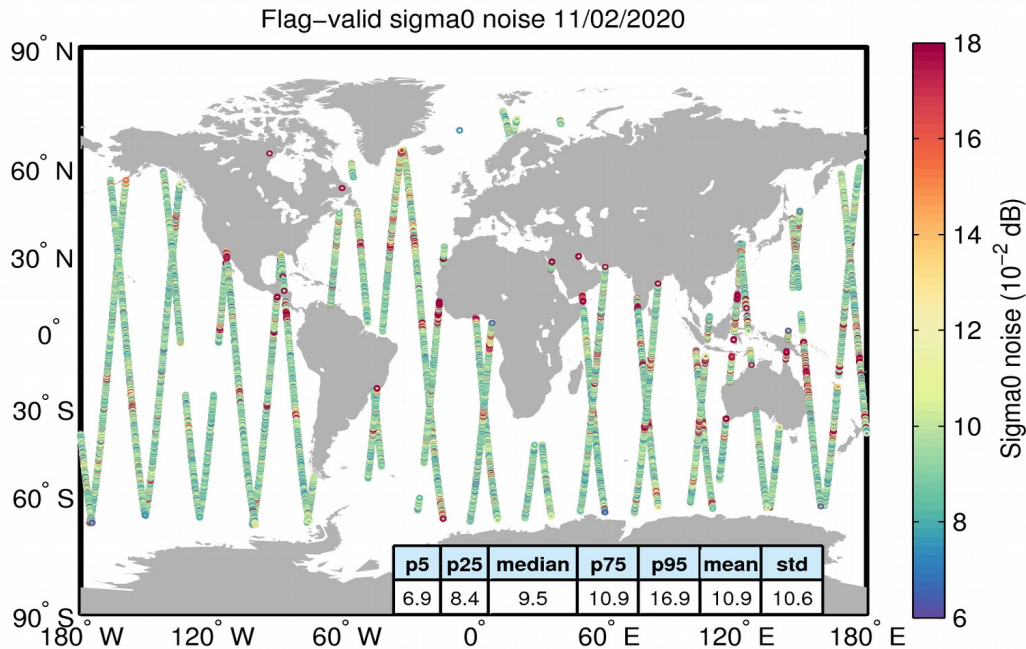
Figure 26. Geographical distribution of flag-valid 20-Hz sigma0 measurement noise over oceans and lakes for 11/02/2020. The statistical values shown in the table refer to the sigma0 noise and are calculated over all measurements shown in the figure.
