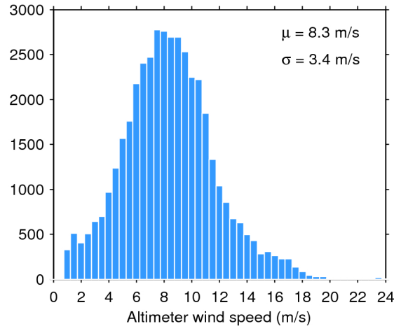
Figure 33. Histogram of flag-valid wind over oceans and lakes for 11/02/2020. The mean ( \mu ) and standard deviation ( \sigma ) are also shown. Note that values larger than 24 m/s are excluded from the histogram for the sake of readability but not from the computation of \mu and \sigma .
