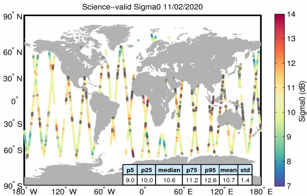
Figure 27. Geographical distribution of science-valid sigma0 data over oceans and lakes for 11/02/2020. The statistical values shown in the table refer to the sigma0 in dB and are calculated over all measurements shown in the figure. Gray circles denote records that have been rejected based on the editing criteria described in Table 4.
