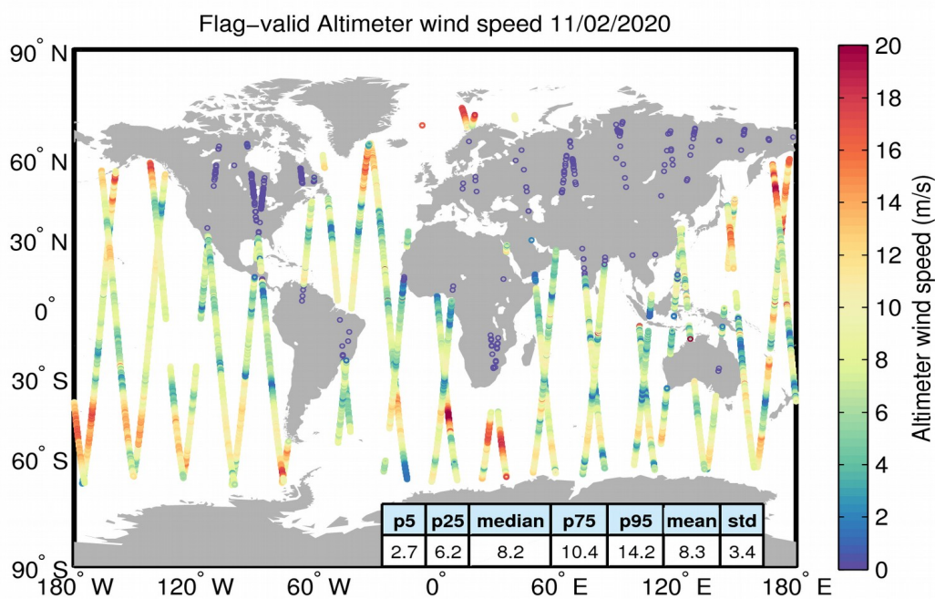
Figure 31. Geographical distribution of flag-valid wind data over oceans and lakes for 11/02/2020. The statistical values shown in the table refer to the wind in m/s and are calculated over all measurements shown in the figure.
