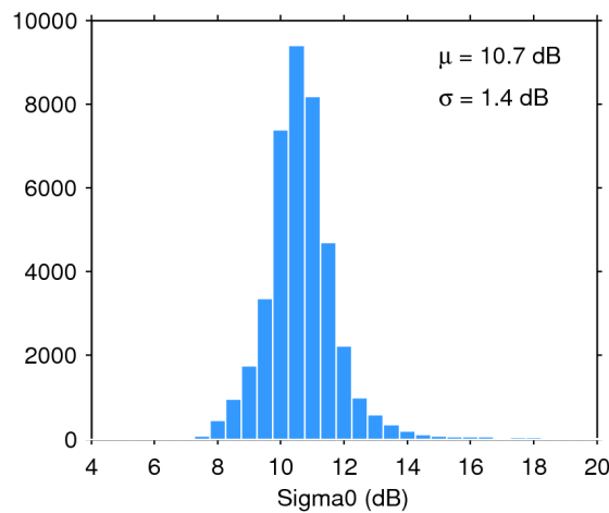
Figure 28. Histogram of science-valid sigma0 over oceans and lakes for 11/02/2020. The mean ( \mu ) and standard deviation ( \sigma ) are also shown. Note that values outside [4 20] dB are excluded from the histogram for the sake of readability but not from the computation of \mu and \sigma .
