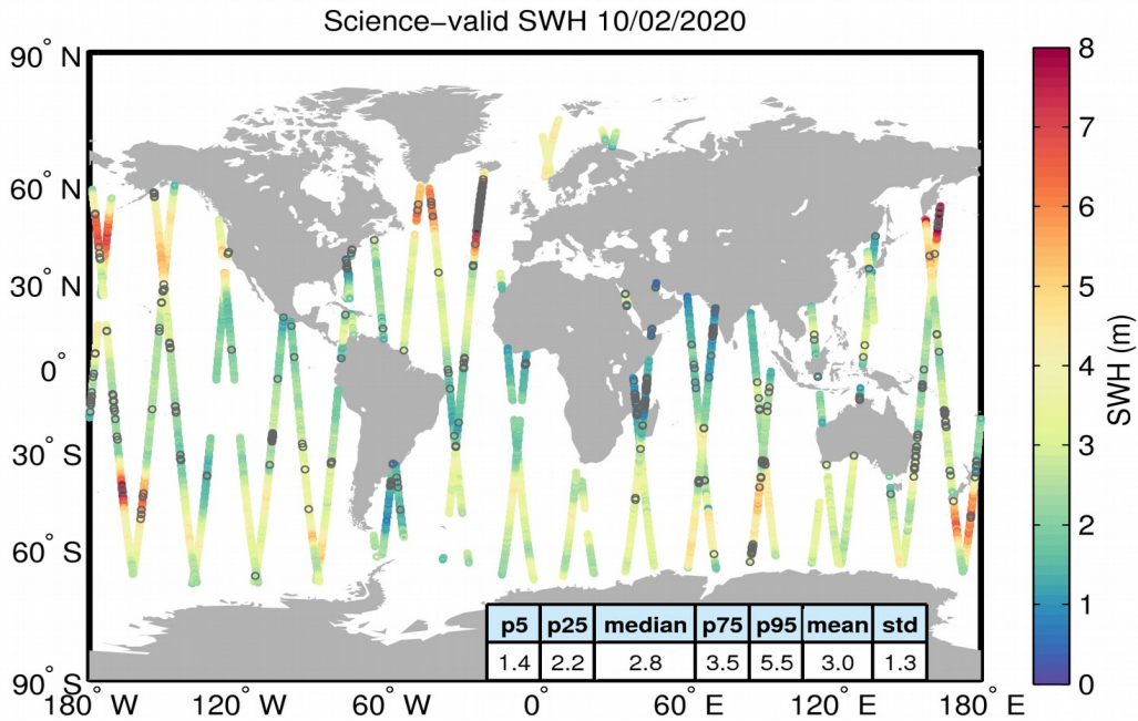
Figure 19. Geographical distribution of science-valid SWH data over oceans and lakes for 10/02/2020. The statistical values shown in the table refer to the SWH in m and are calculated over all measurements shown in the figure. Gray circles denote records that have been rejected based on the editing criteria described in Table 3.
