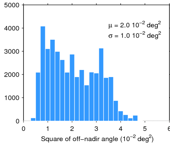
Figure 39. Histogram of flag-valid mispointing over oceans and lakes for 10/02/2020. The mean ( \mu ) and standard deviation ( \sigma ) are also shown. Note that values larger than 6 \cdot 10^{-2} \text{ deg}^2 are excluded from the histogram for the sake of readability but not from the computation of \mu and \sigma .
