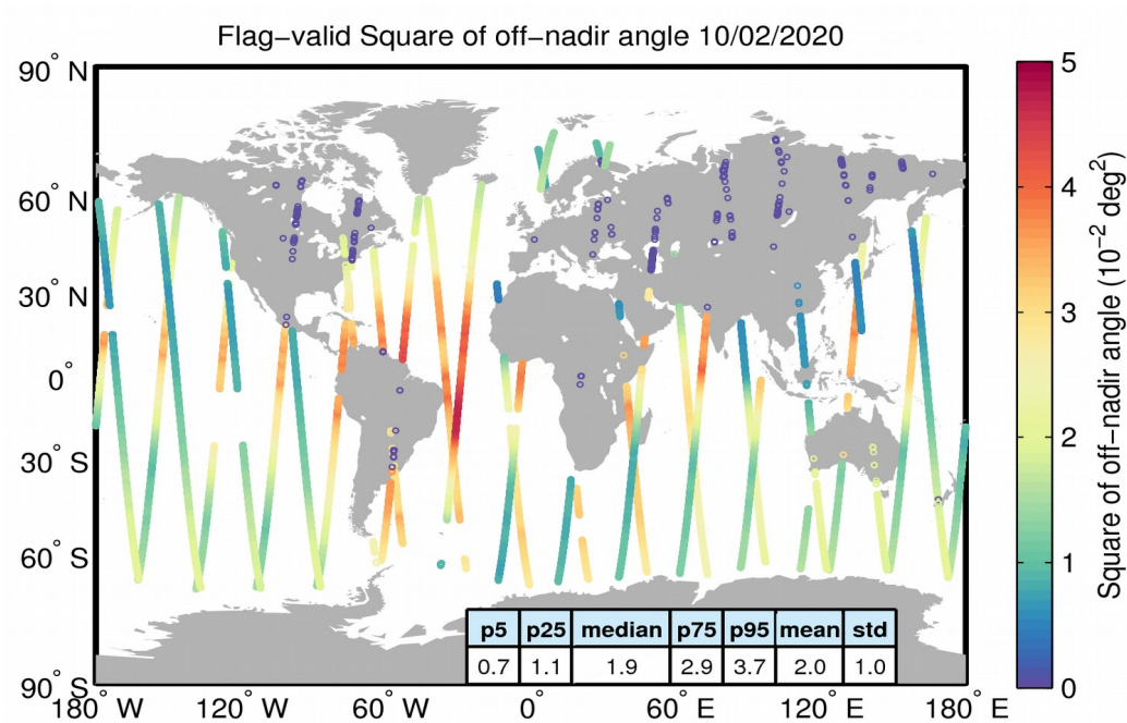
Figure 37. Geographical distribution of flag-valid mispointing data over oceans and lakes for 10/02/2020. The statistical values shown in the table refer to the mispointing in 10^{-2} \text{ deg}^2 and are calculated over all measurements shown in the figure.
