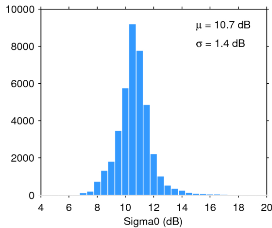
Figure 28. Histogram of science-valid sigma0 over oceans and lakes for 10/02/2020. The mean ( \mu ) and standard deviation ( \sigma ) are also shown. Note that values outside [4 20] dB are excluded from the histogram for the sake of readability but not from the computation of \mu and \sigma .
