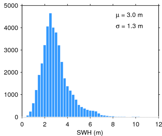
Figure 20. Histogram of science-valid SWH over oceans and lakes for 10/02/2020. The mean ( \mu ) and standard deviation ( \sigma ) are also shown. Note that values larger than 12 m are excluded from the histogram for the sake of readability but not from the computation of \mu and \sigma .
