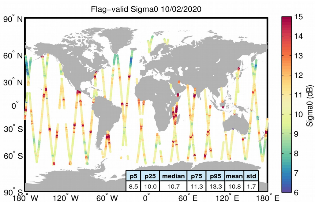
Figure 23. Geographical distribution of flag-valid sigma0 data over oceans and lakes for 10/02/2020. The statistical values shown in the table refer to the sigma0 in dB and are calculated over all measurements shown in the figure.
