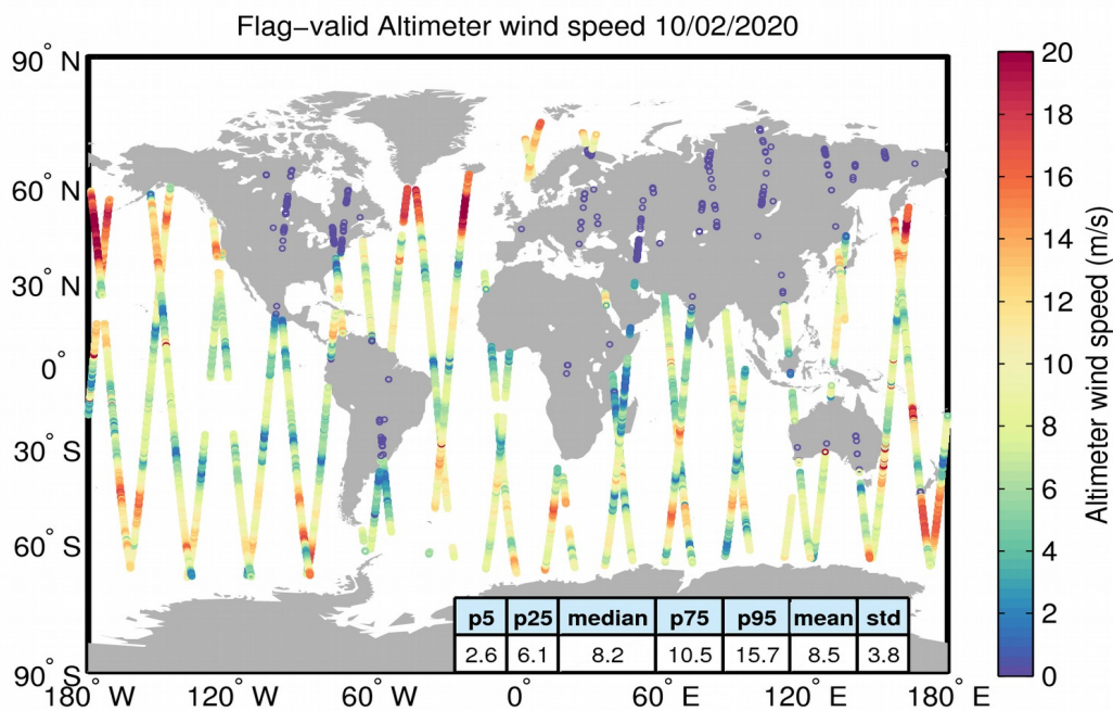
Figure 31. Geographical distribution of flag-valid wind data over oceans and lakes for 10/02/2020. The statistical values shown in the table refer to the wind in m/s and are calculated over all measurements shown in the figure.
