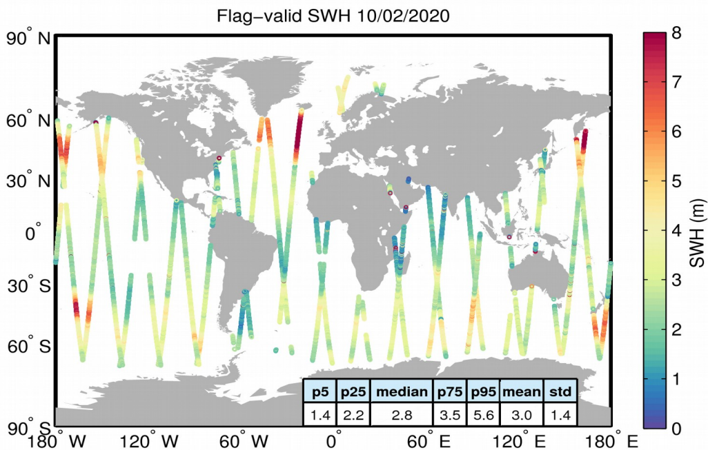
Figure 15. Geographical distribution of flag-valid SWH data over oceans and lakes for 10/02/2020. The statistical values shown in the table refer to the SWH in m and are calculated over all measurements shown in the figure.
