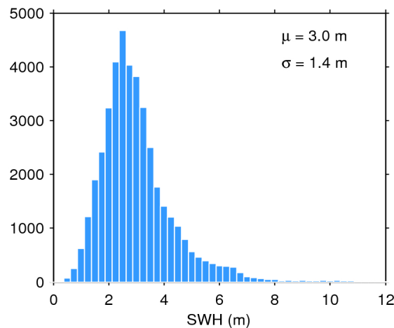
Figure 17. Histogram of flag-valid SWH over oceans and lakes for 10/02/2020. The mean ( \mu ) and standard deviation ( \sigma ) are also shown. Note that values larger than 12 m are excluded from the histogram for the sake of readability but not from the computation of \mu and \sigma .
