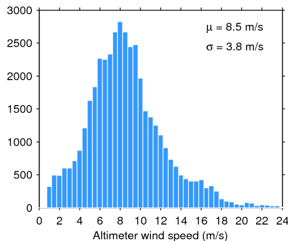
Figure 35. Histogram of science-valid wind over oceans and lakes for 10/02/2020. The mean ( \mu ) and standard deviation ( \sigma ) are also shown. Note that values larger than 24 m/s are excluded from the histogram for the sake of readability but not from the computation of \mu and \sigma .
