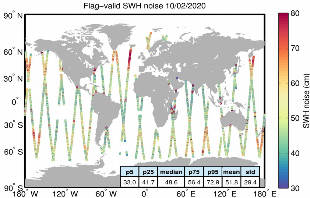
Figure 18. Geographical distribution of flag-valid 20-Hz SWH measurement noise over oceans and lakes for 10/02/2020. The statistical values shown in the table refer to the SWH noise and are calculated over all measurements shown in the figure.
