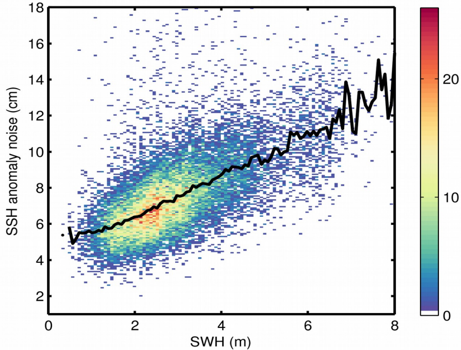
Figure 9. 2D histogram showing flag-valid SSH anomaly noise as a function of SWH for 10/02/2020. The black line denotes the median SSH anomaly noise as a function of SWH.
