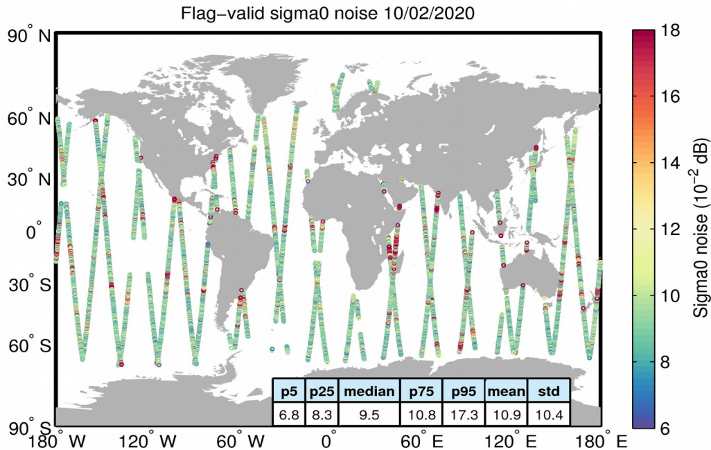
Figure 26. Geographical distribution of flag-valid 20-Hz sigma0 measurement noise over oceans and lakes for 10/02/2020. The statistical values shown in the table refer to the sigma0 noise and are calculated over all measurements shown in the figure.
