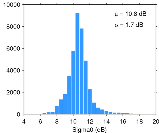
Figure 25. Histogram of flag-valid sigma0 over oceans and lakes for 10/02/2020. The mean ( \mu ) and standard deviation ( \sigma ) are also shown. Note that values outside [4 20] dB are excluded from the histogram for the sake of readability but not from the computation of \mu and \sigma .
