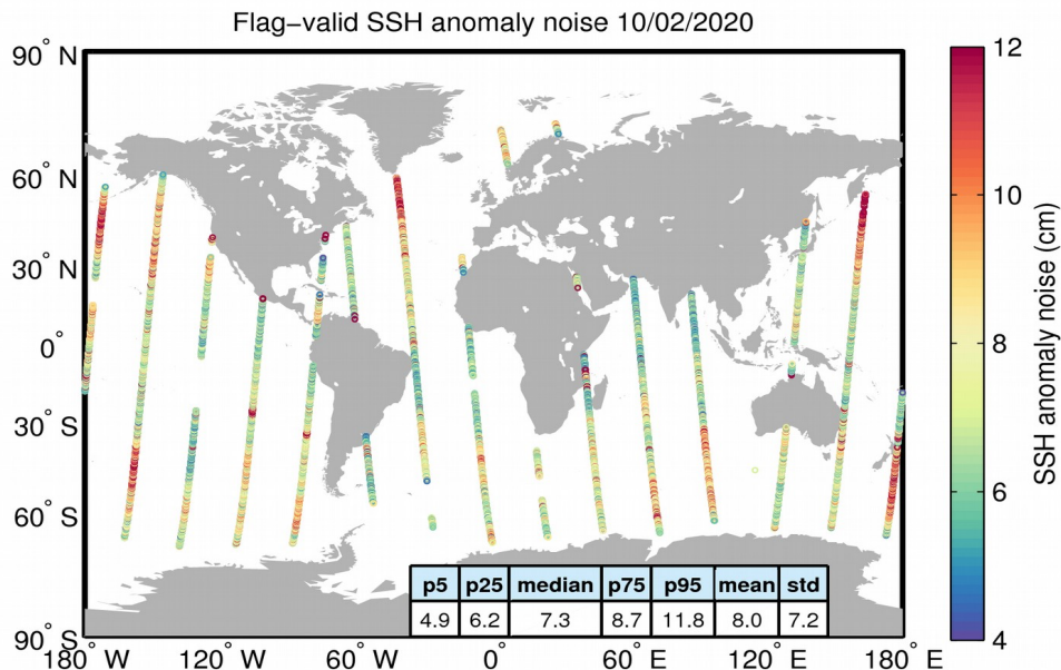
Figure 8. Geographical distribution of flag-valid 20-Hz SSH anomaly measurement noise over oceans and lakes for 10/02/2020. The statistical values shown in the table refer to the SSH anomaly noise and are calculated over all measurements shown in the figure.
