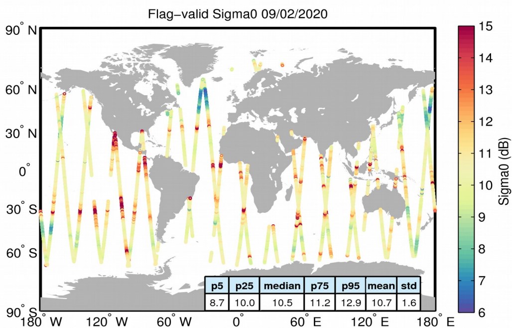
Figure 23. Geographical distribution of flag-valid sigma0 data over oceans and lakes for 09/02/2020. The statistical values shown in the table refer to the sigma0 in dB and are calculated over all measurements shown in the figure.
