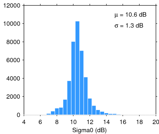
Figure 28. Histogram of science-valid sigma0 over oceans and lakes for 09/02/2020. The mean ( \mu ) and standard deviation ( \sigma ) are also shown. Note that values outside [4 20] dB are excluded from the histogram for the sake of readability but not from the computation of \mu and \sigma .
