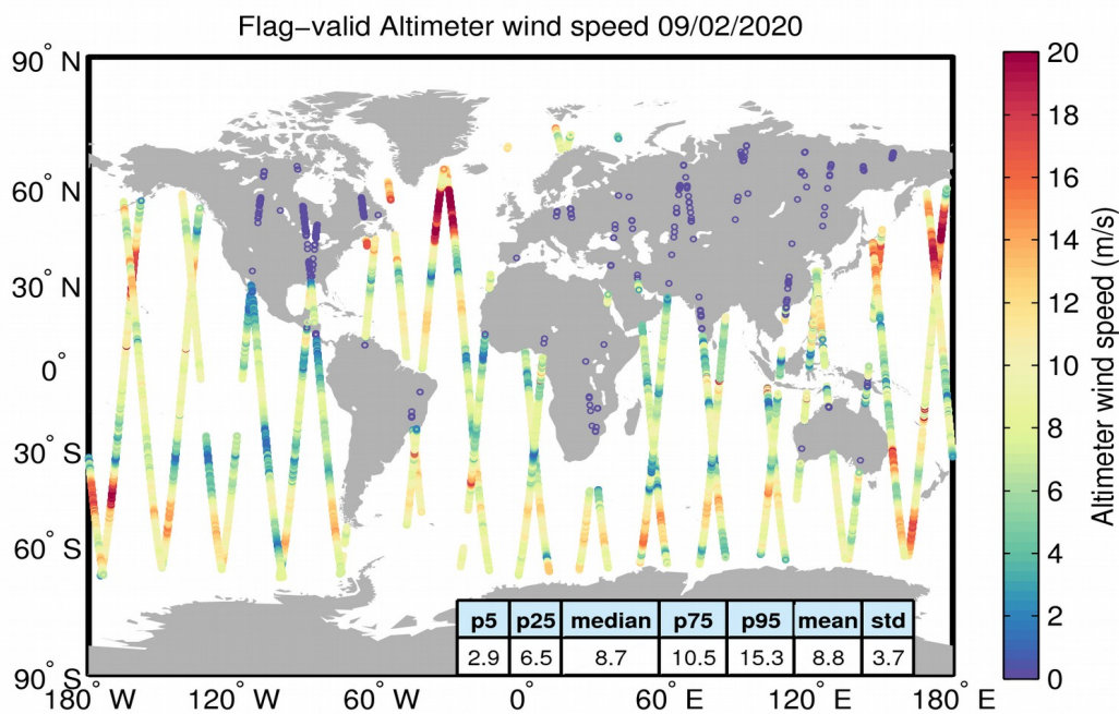
Figure 31. Geographical distribution of flag-valid wind data over oceans and lakes for 09/02/2020. The statistical values shown in the table refer to the wind in m/s and are calculated over all measurements shown in the figure.
