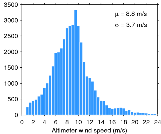
Figure 33. Histogram of flag-valid wind over oceans and lakes for 09/02/2020. The mean ( \mu ) and standard deviation ( \sigma ) are also shown. Note that values larger than 24 m/s are excluded from the histogram for the sake of readability but not from the computation of \mu and \sigma .
