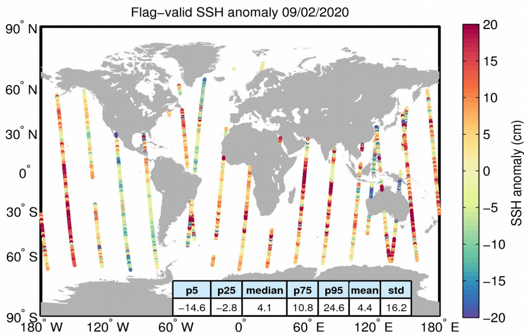
Figure 5. Geographical distribution of flag-valid 1-Hz SSH anomaly data over oceans and lakes for 09/02/2020. The statistical values shown in the table refer to the SSH anomaly in cm and are calculated over all measurements shown in the figure.
