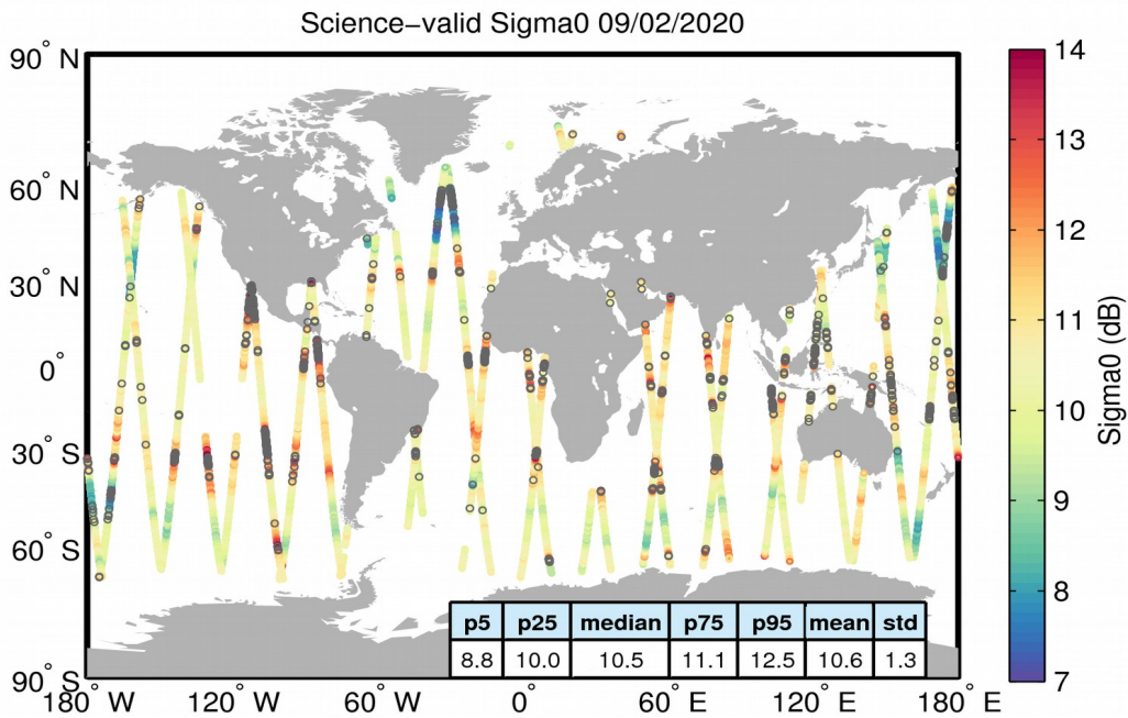
Figure 27. Geographical distribution of science-valid sigma0 data over oceans and lakes for 09/02/2020. The statistical values shown in the table refer to the sigma0 in dB and are calculated over all measurements shown in the figure. Gray circles denote records that have been rejected based on the editing criteria described in Table 4.
