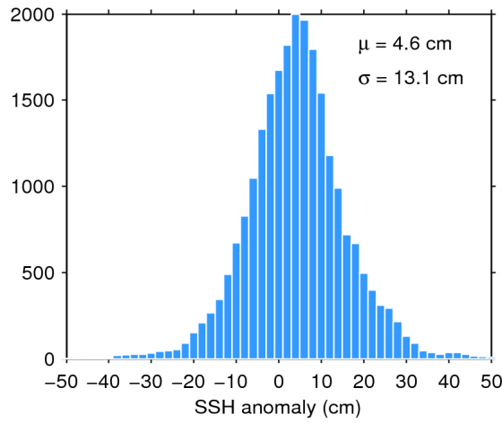
Figure 11. Histogram of science-valid SSH anomaly over oceans and lakes for 09/02/2020. The mean ( \mu ) and standard deviation ( \sigma ) are also shown. Note that values outside [-50 50] cm are excluded from the histogram for the sake of readability but not from the computation of \mu and \sigma .
