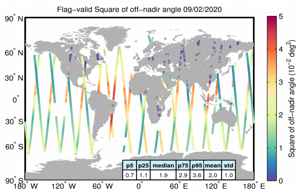
Figure 37. Geographical distribution of flag-valid mispointing data over oceans and lakes for 09/02/2020. The statistical values shown in the table refer to the mispointing in 10^{-2} \text{deg}^2 and are calculated over all measurements shown in the figure.
