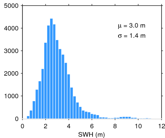
Figure 17. Histogram of flag-valid SWH over oceans and lakes for 09/02/2020. The mean ( \mu ) and standard deviation ( \sigma ) are also shown. Note that values larger than 12 m are excluded from the histogram for the sake of readability but not from the computation of \mu and \sigma .
