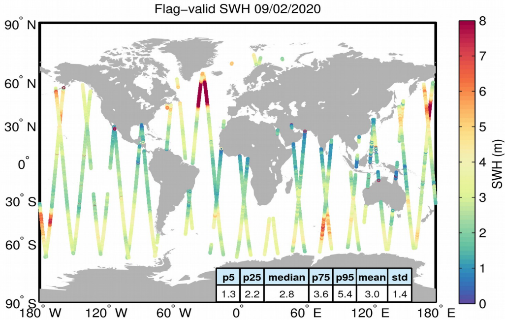
Figure 15. Geographical distribution of flag-valid SWH data over oceans and lakes for 09/02/2020. The statistical values shown in the table refer to the SWH in m and are calculated over all measurements shown in the figure.
