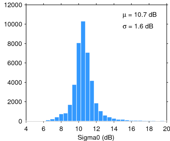
Figure 25. Histogram of flag-valid sigma0 over oceans and lakes for 09/02/2020. The mean ( \mu ) and standard deviation ( \sigma ) are also shown. Note that values outside [4 20] dB are excluded from the histogram for the sake of readability but not from the computation of \mu and \sigma .
