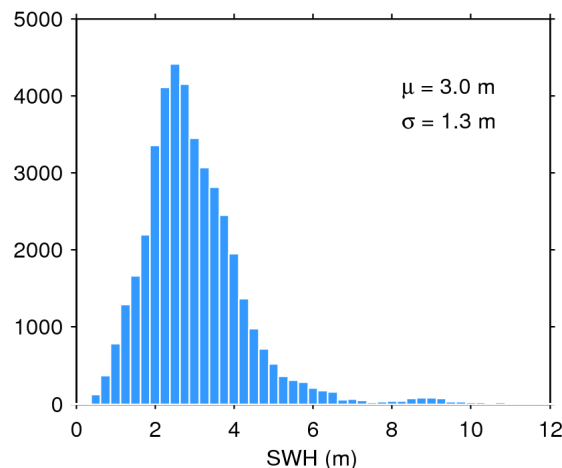
Figure 20. Histogram of science-valid SWH over oceans and lakes for 09/02/2020. The mean ( \mu ) and standard deviation ( \sigma ) are also shown. Note that values larger than 12 m are excluded from the histogram for the sake of readability but not from the computation of \mu and \sigma .
