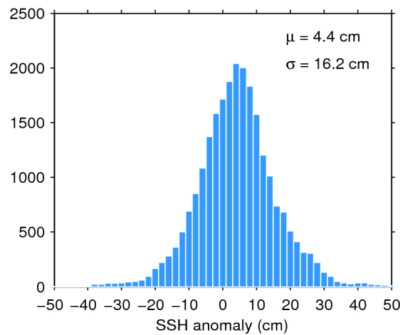
Figure 7. Histogram of flag-valid SSH anomaly over oceans and lakes for 09/02/2020. The mean ( \mu ) and standard deviation ( \sigma ) are also shown. Note that values outside [-50 50] cm are excluded from the histogram for the sake of readability but not from the computation of \mu and \sigma .
