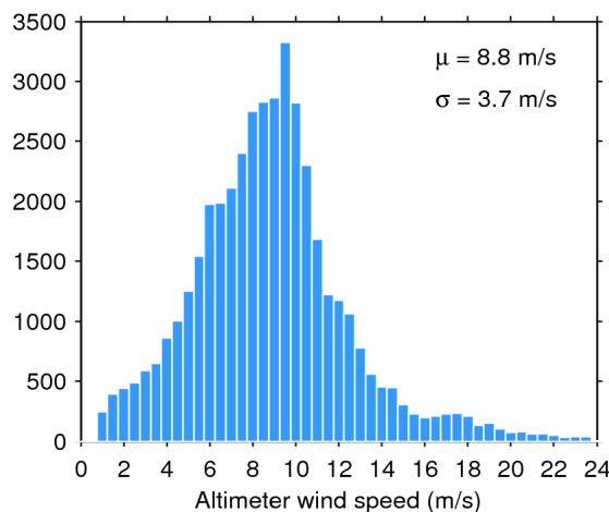
Figure 35. Histogram of science-valid wind over oceans and lakes for 09/02/2020. The mean ( \mu ) and standard deviation ( \sigma ) are also shown. Note that values larger than 24 m/s are excluded from the histogram for the sake of readability but not from the computation of \mu and \sigma .
