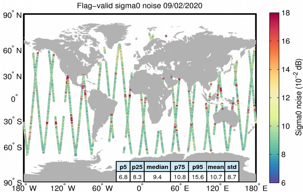
Figure 26. Geographical distribution of flag-valid 20-Hz sigma0 measurement noise over oceans and lakes for 09/02/2020. The statistical values shown in the table refer to the sigma0 noise and are calculated over all measurements shown in the figure.
