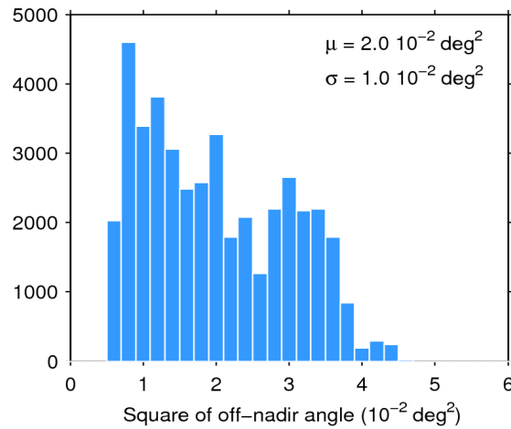
Figure 39. Histogram of flag-valid mispointing over oceans and lakes for 09/02/2020. The mean ( \mu ) and standard deviation ( \sigma ) are also shown. Note that values larger than 6 \cdot 10^{-2} \text{ deg}^2 are excluded from the histogram for the sake of readability but not from the computation of \mu and \sigma .
