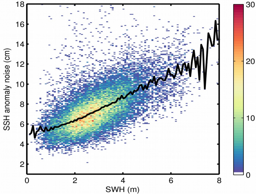
Figure 9. 2D histogram showing flag-valid SSH anomaly noise as a function of SWH for 09/02/2020. The black line denotes the median SSH anomaly noise as a function of SWH.
