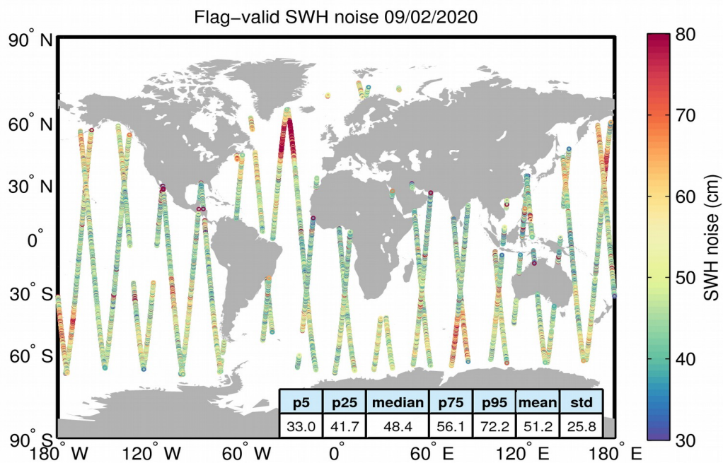
Figure 18. Geographical distribution of flag-valid 20-Hz SWH measurement noise over oceans and lakes for 09/02/2020. The statistical values shown in the figure refer to the SWH noise and are calculated over all measurements shown in the figure.
