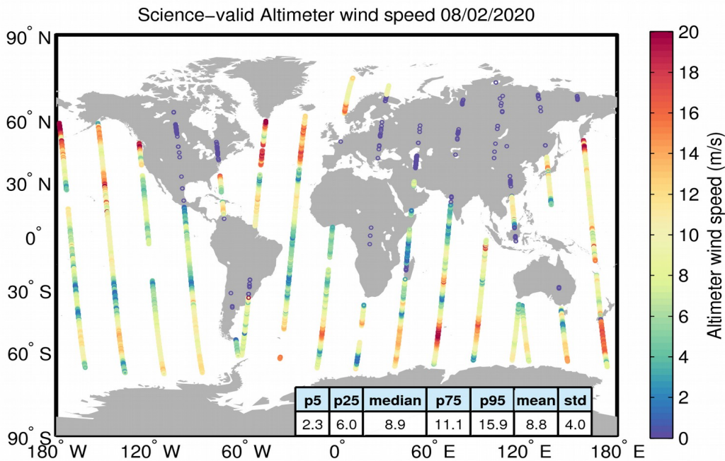
Figure 34. Geographical distribution of science-valid wind data over oceans and lakes for 08/02/2020. The statistical values shown in the table refer to the wind in m/s and are calculated over all measurements shown in the figure. Gray circles denote records that have been rejected based on the editing criteria described in Table 5.
