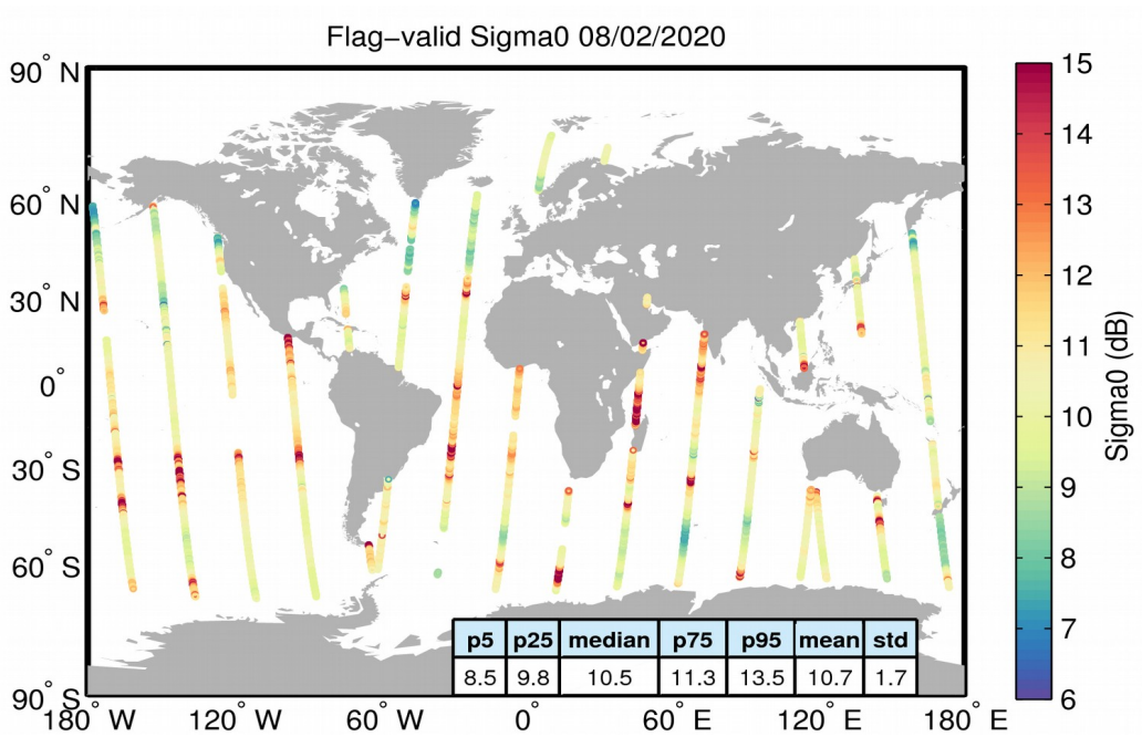
Figure 23. Geographical distribution of flag-valid sigma0 data over oceans and lakes for 08/02/2020. The statistical values shown in the table refer to the sigma0 in dB and are calculated over all measurements shown in the figure.
