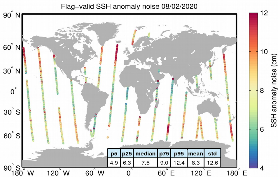
Figure 8. Geographical distribution of flag-valid 20-Hz SSH anomaly measurement noise over oceans and lakes for 08/02/2020. The statistical values shown in the table refer to the SSH anomaly noise and are calculated over all measurements shown in the figure.
