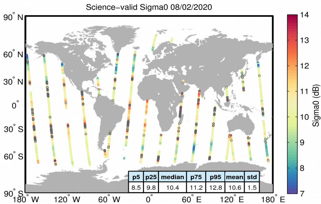
Figure 27. Geographical distribution of science-valid sigma0 data over oceans and lakes for 08/02/2020. The statistical values shown in the table refer to the sigma0 in dB and are calculated over all measurements shown in the figure. Gray circles denote records that have been rejected based on the editing criteria described in Table 4.
