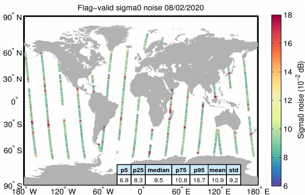
Figure 26. Geographical distribution of flag-valid 20-Hz sigma0 measurement noise over oceans and lakes for 08/02/2020. The statistical values shown in the table refer to the sigma0 noise and are calculated over all measurements shown in the figure.
