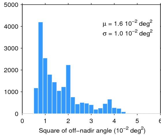
Figure 39. Histogram of flag-valid mispointing over oceans and lakes for 08/02/2020. The mean ( \mu ) and standard deviation ( \sigma ) are also shown. Note that values larger than 6 \cdot 10^{-2} \text{ deg}^2 are excluded from the histogram for the sake of readability but not from the computation of \mu and \sigma .
