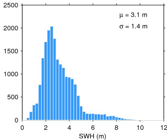
Figure 20. Histogram of science-valid SWH over oceans and lakes for 08/02/2020. The mean ( \mu ) and standard deviation ( \sigma ) are also shown. Note that values larger than 12 m are excluded from the histogram for the sake of readability but not from the computation of \mu and \sigma .
