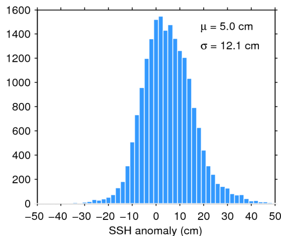
Figure 11. Histogram of science-valid SSH anomaly over oceans and lakes for 08/02/2020. The mean ( \mu ) and standard deviation ( \sigma ) are also shown. Note that values outside [-50 50] cm are excluded from the histogram for the sake of readability but not from the computation of \mu and \sigma .
