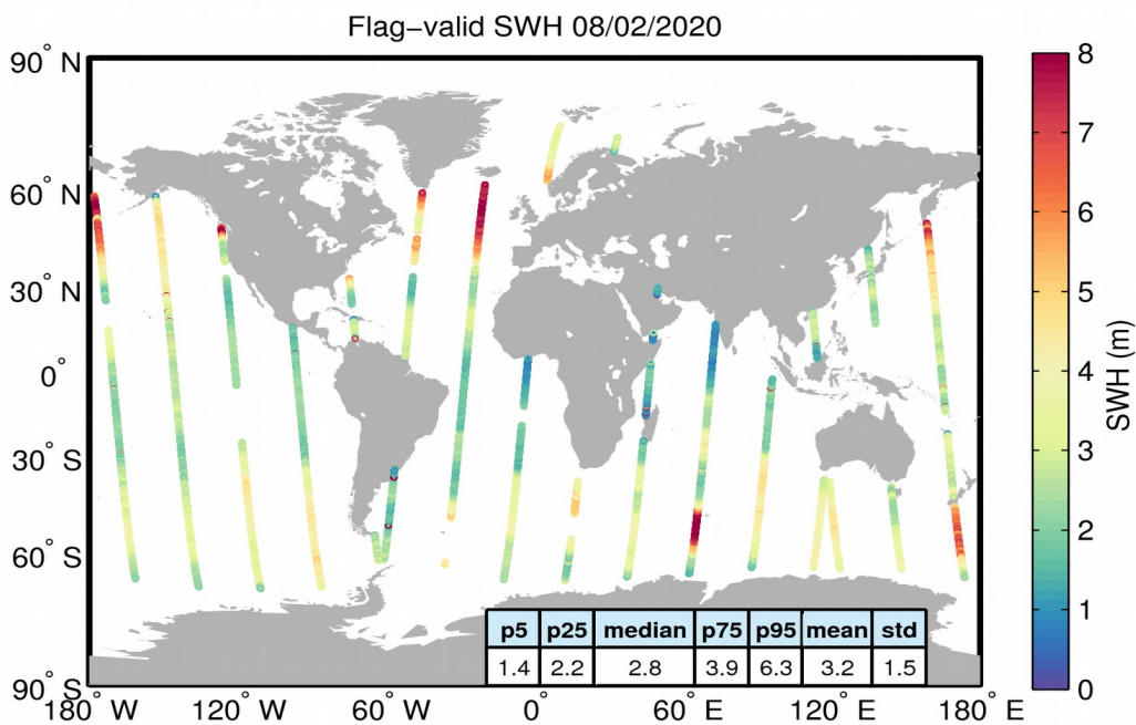
Figure 15. Geographical distribution of flag-valid SWH data over oceans and lakes for 08/02/2020. The statistical values shown in the table refer to the SWH in m and are calculated over all measurements shown in the figure.
