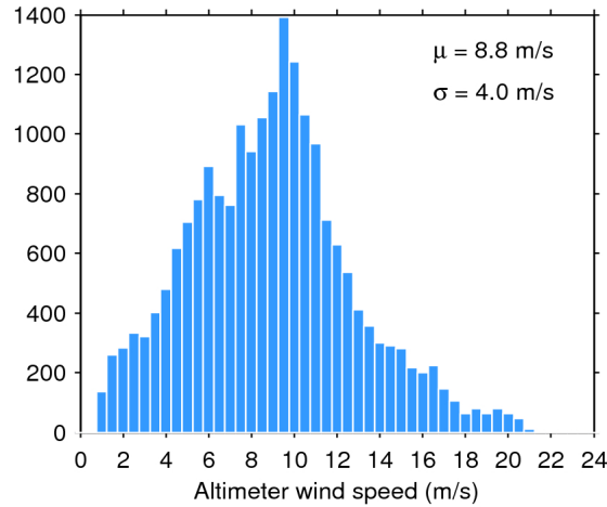
Figure 33. Histogram of flag-valid wind over oceans and lakes for 08/02/2020. The mean ( \mu ) and standard deviation ( \sigma ) are also shown. Note that values larger than 24 m/s are excluded from the histogram for the sake of readability but not from the computation of \mu and \sigma .
