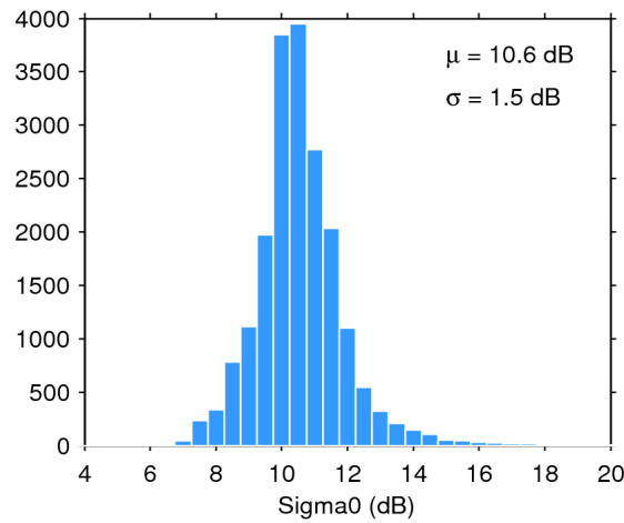
Figure 28. Histogram of science-valid sigma0 over oceans and lakes for 08/02/2020. The mean ( \mu ) and standard deviation ( \sigma ) are also shown. Note that values outside [4 20] dB are excluded from the histogram for the sake of readability but not from the computation of \mu and \sigma .
