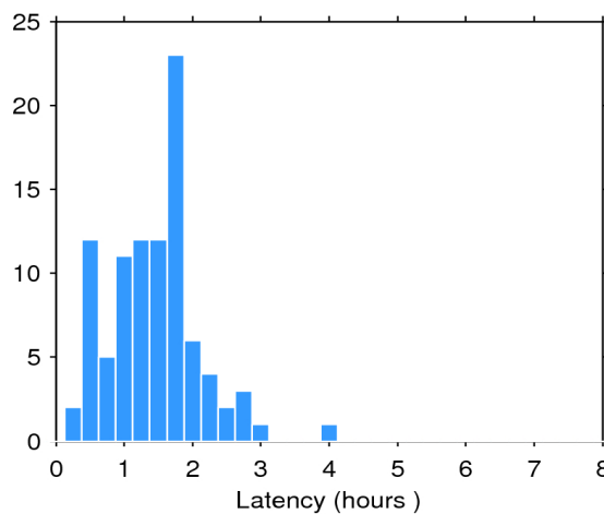
Figure 2. Histogram of the data latency for 08/02/2020. The y-axis denotes the number of files that are made available with a delay of x-hours with respect to the mean time of the records stored in the file.
