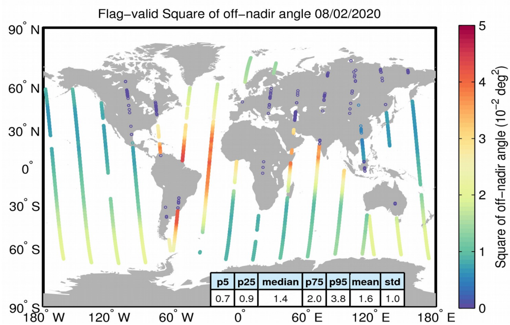
Figure 37. Geographical distribution of flag-valid mispointing data over oceans and lakes for 08/02/2020. The statistical values shown in the table refer to the mispointing in 10^{-2} \text{ deg}^2 and are calculated over all measurements shown in the figure.
