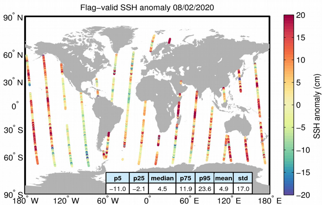
Figure 5. Geographical distribution of flag-valid 1-Hz SSH anomaly data over oceans and lakes for 08/02/2020. The statistical values shown in the table refer to the SSH anomaly in cm and are calculated over all measurements shown in the figure.
