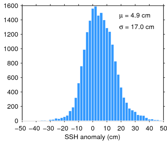
Figure 7. Histogram of flag-valid SSH anomaly over oceans and lakes for 08/02/2020. The mean ( \mu ) and standard deviation ( \sigma ) are also shown. Note that values outside [-50 50] cm are excluded from the histogram for the sake of readability but not from the computation of \mu and \sigma .
