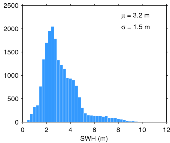
Figure 17. Histogram of flag-valid SWH over oceans and lakes for 08/02/2020. The mean ( \mu ) and standard deviation ( \sigma ) are also shown. Note that values larger than 12 m are excluded from the histogram for the sake of readability but not from the computation of \mu and \sigma .
