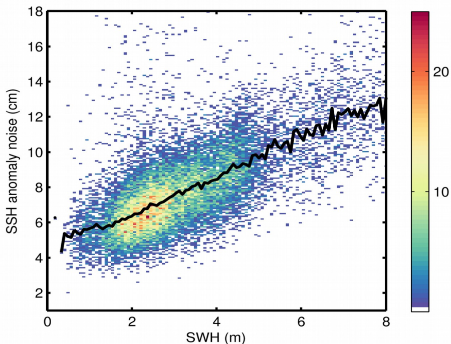
Figure 9. 2D histogram showing flag-valid SSH anomaly noise as a function of SWH for 08/02/2020. The black line denotes the median SSH anomaly noise as a function of SWH.
