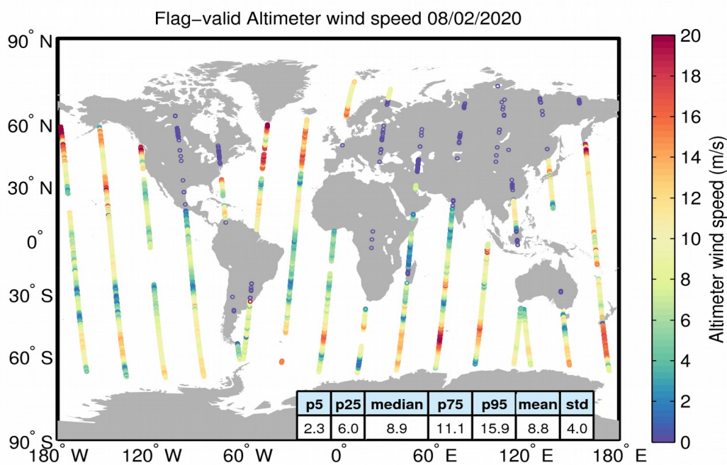
Figure 31. Geographical distribution of flag-valid wind data over oceans and lakes for 08/02/2020. The statistical values shown in the table refer to the wind in m/s and are calculated over all measurements shown in the figure.
