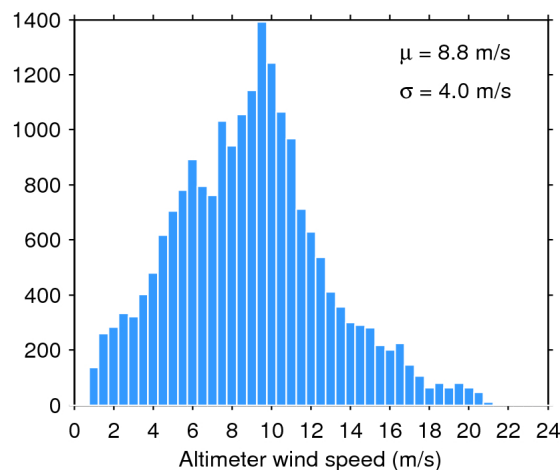
Figure 35. Histogram of science-valid wind over oceans and lakes for 08/02/2020. The mean ( \mu ) and standard deviation ( \sigma ) are also shown. Note that values larger than 24 m/s are excluded from the histogram for the sake of readability but not from the computation of \mu and \sigma .
