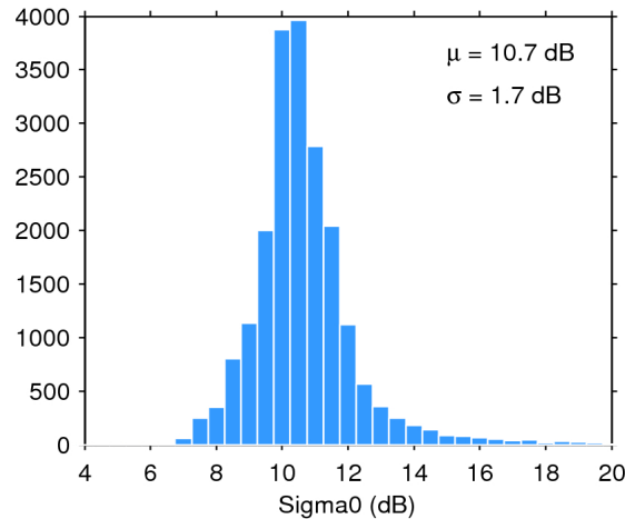
Figure 25. Histogram of flag-valid sigma0 over oceans and lakes for 08/02/2020. The mean ( \mu ) and standard deviation ( \sigma ) are also shown. Note that values outside [4 20] dB are excluded from the histogram for the sake of readability but not from the computation of \mu and \sigma .
