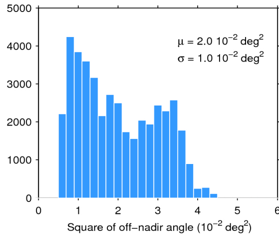
Figure 39. Histogram of flag-valid mispointing over oceans and lakes for 07/02/2020. The mean ( \mu ) and standard deviation ( \sigma ) are also shown. Note that values larger than 6 \cdot 10^{-2} \text{ deg}^2 are excluded from the histogram for the sake of readability but not from the computation of \mu and \sigma .
