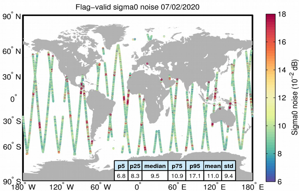
Figure 26. Geographical distribution of flag-valid 20-Hz sigma0 measurement noise over oceans and lakes for 07/02/2020. The statistical values shown in the table refer to the sigma0 noise and are calculated over all measurements shown in the figure.
