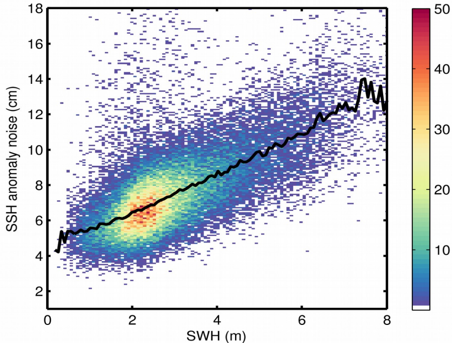
Figure 9. 2D histogram showing flag-valid SSH anomaly noise as a function of SWH for 07/02/2020. The black line denotes the median SSH anomaly noise as a function of SWH.
