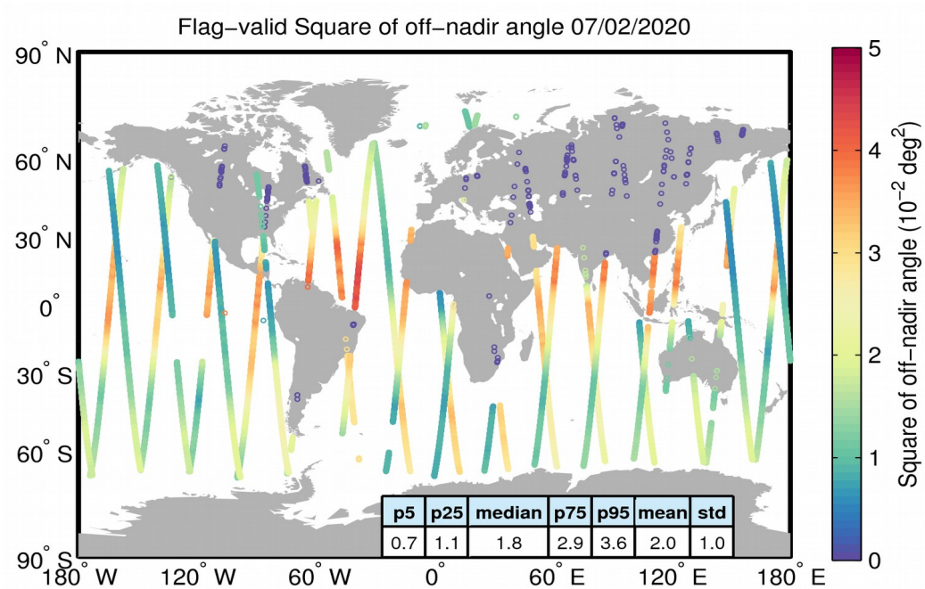
Figure 37. Geographical distribution of flag-valid mispointing data over oceans and lakes for 07/02/2020. The statistical values shown in the table refer to the mispointing in 10^{-2} deg 2 and are calculated over all measurements shown in the figure.
