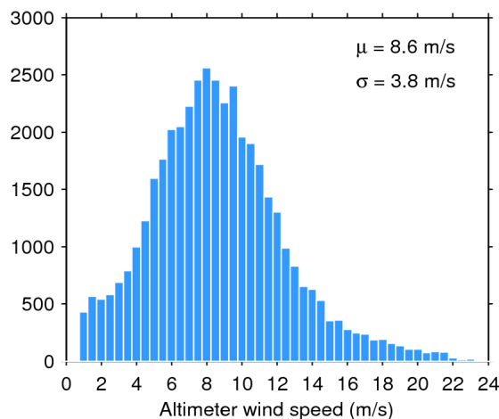
Figure 35. Histogram of science-valid wind over oceans and lakes for 07/02/2020. The mean ( \mu ) and standard deviation ( \sigma ) are also shown. Note that values larger than 24 m/s are excluded from the histogram for the sake of readability but not from the computation of \mu and \sigma .
