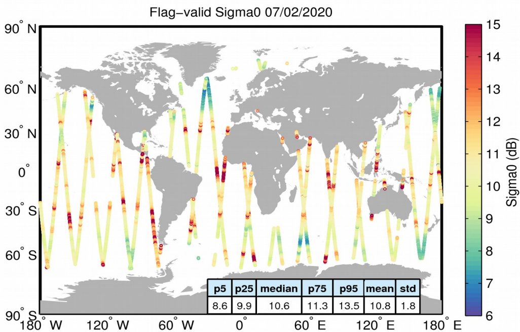
Figure 23. Geographical distribution of flag-valid sigma0 data over oceans and lakes for 07/02/2020. The statistical values shown in the table refer to the sigma0 in dB and are calculated over all measurements shown in the figure.
