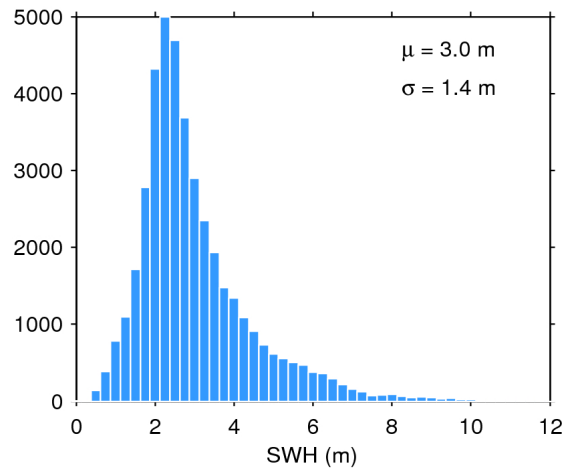
Figure 20. Histogram of science-valid SWH over oceans and lakes for 07/02/2020. The mean ( \mu ) and standard deviation ( \sigma ) are also shown. Note that values larger than 12 m are excluded from the histogram for the sake of readability but not from the computation of \mu and \sigma .
