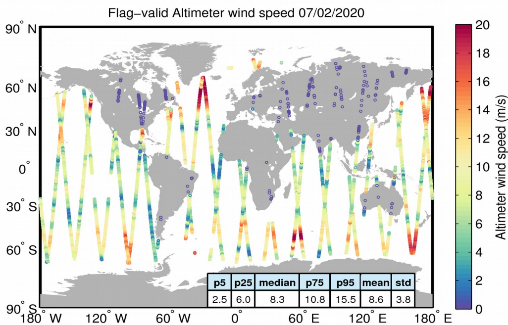
Figure 31. Geographical distribution of flag-valid wind data over oceans and lakes for 07/02/2020. The statistical values shown in the table refer to the wind in m/s and are calculated over all measurements shown in the figure.
