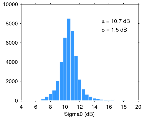
Figure 28. Histogram of science-valid sigma0 over oceans and lakes for 07/02/2020. The mean ( \mu ) and standard deviation ( \sigma ) are also shown. Note that values outside [4 20] dB are excluded from the histogram for the sake of readability but not from the computation of \mu and \sigma .
