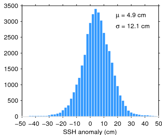
Figure 11. Histogram of science-valid SSH anomaly over oceans and lakes for 07/02/2020. The mean ( \mu ) and standard deviation ( \sigma ) are also shown. Note that values outside [-50 50] cm are excluded from the histogram for the sake of readability but not from the computation of \mu and \sigma .
