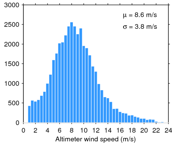
Figure 33. Histogram of flag-valid wind over oceans and lakes for 07/02/2020. The mean ( \mu ) and standard deviation ( \sigma ) are also shown. Note that values larger than 24 m/s are excluded from the histogram for the sake of readability but not from the computation of \mu and \sigma .
