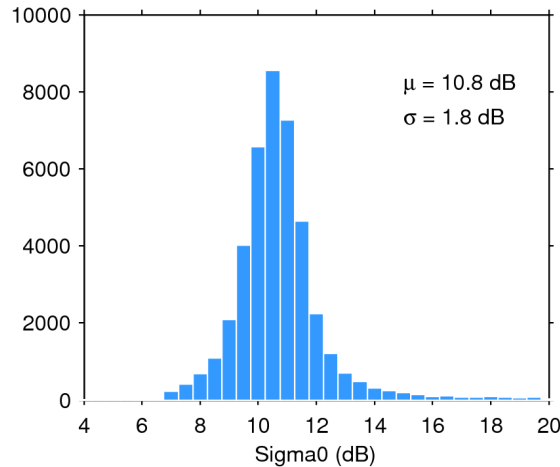
Figure 25. Histogram of flag-valid sigma0 over oceans and lakes for 07/02/2020. The mean ( \mu ) and standard deviation ( \sigma ) are also shown. Note that values outside [4 20] dB are excluded from the histogram for the sake of readability but not from the computation of \mu and \sigma .
