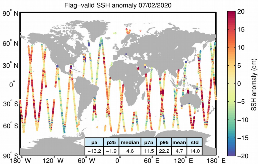
Figure 5. Geographical distribution of flag-valid 1-Hz SSH anomaly data over oceans and lakes for 07/02/2020. The statistical values shown in the table refer to the SSH anomaly in cm and are calculated over all measurements shown in the figure.
