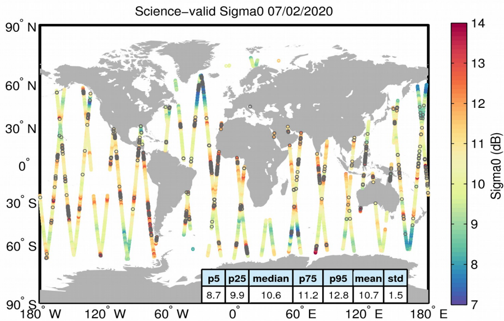
Figure 27. Geographical distribution of science-valid sigma0 data over oceans and lakes for 07/02/2020. The statistical values shown in the table refer to the sigma0 in dB and are calculated over all measurements shown in the figure. Gray circles denote records that have been rejected based on the editing criteria described in Table 4.
