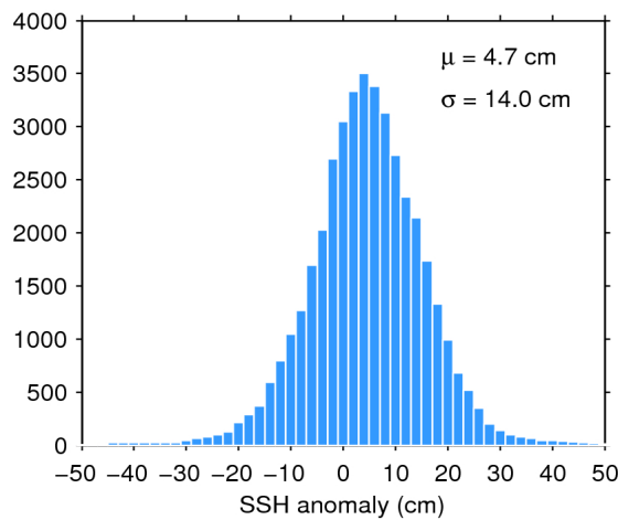
Figure 7. Histogram of flag-valid SSH anomaly over oceans and lakes for 07/02/2020. The mean ( \mu ) and standard deviation ( \sigma ) are also shown. Note that values outside [-50\ 50] cm are excluded from the histogram for the sake of readability but not from the computation of \mu and \sigma .
