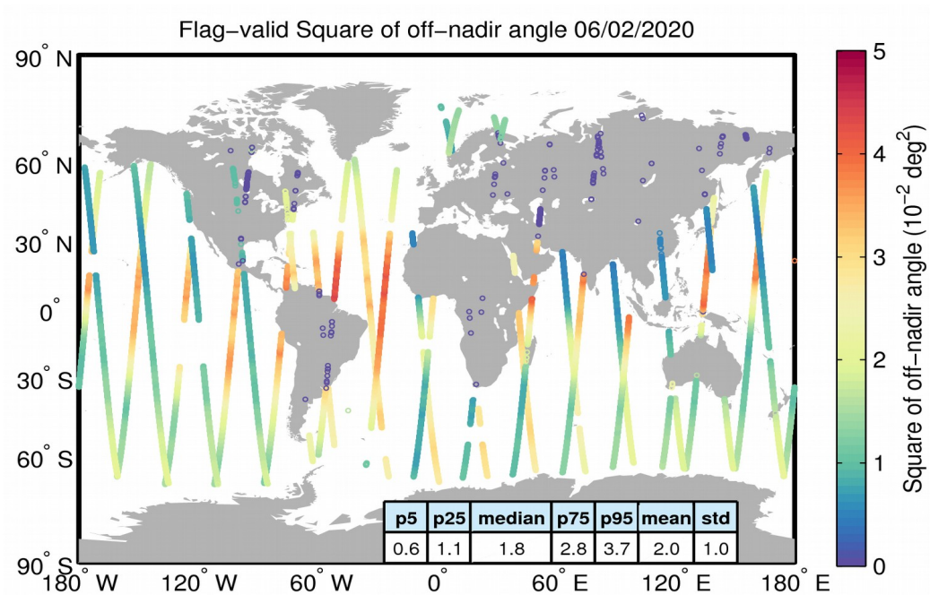
Figure 37. Geographical distribution of flag-valid mispointing data over oceans and lakes for 06/02/2020. The statistical values shown in the table refer to the mispointing in 10^{-2} \text{ deg}^2 and are calculated over all measurements shown in the figure.
