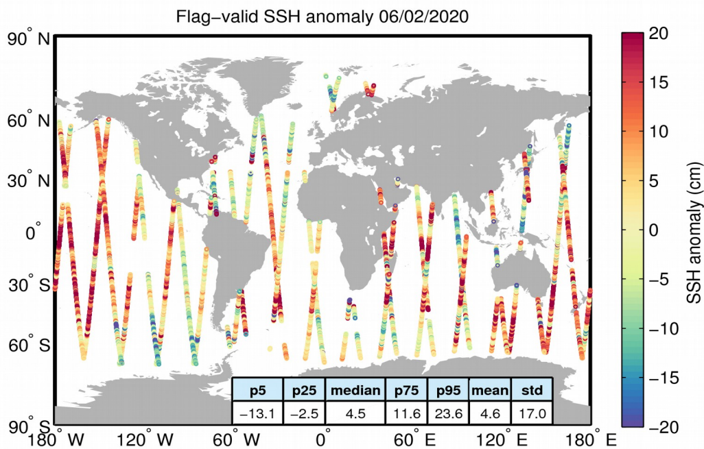
Figure 5. Geographical distribution of flag-valid 1-Hz SSH anomaly data over oceans and lakes for 06/02/2020. The statistical values shown in the table refer to the SSH anomaly in cm and are calculated over all measurements shown in the figure.
