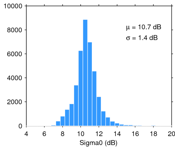
Figure 28. Histogram of science-valid sigma0 over oceans and lakes for 06/02/2020. The mean ( \mu ) and standard deviation ( \sigma ) are also shown. Note that values outside [4 20] dB are excluded from the histogram for the sake of readability but not from the computation of \mu and \sigma .
