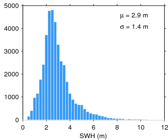
Figure 17. Histogram of flag-valid SWH over oceans and lakes for 06/02/2020. The mean ( \mu ) and standard deviation ( \sigma ) are also shown. Note that values larger than 12 m are excluded from the histogram for the sake of readability but not from the computation of \mu and \sigma .
