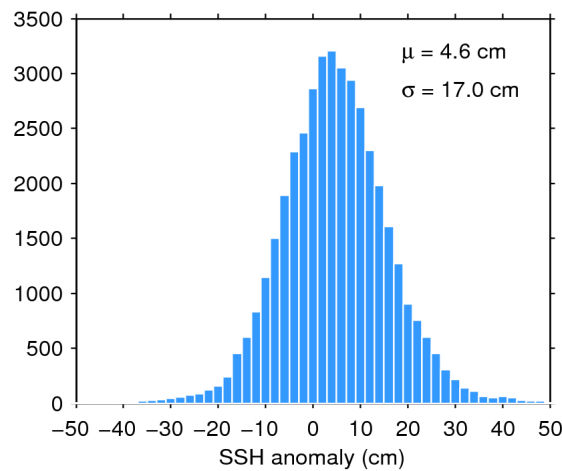
Figure 7. Histogram of flag-valid SSH anomaly over oceans and lakes for 06/02/2020. The mean ( \mu ) and standard deviation ( \sigma ) are also shown. Note that values outside [-50 50] cm are excluded from the histogram for the sake of readability but not from the computation of \mu and \sigma .
