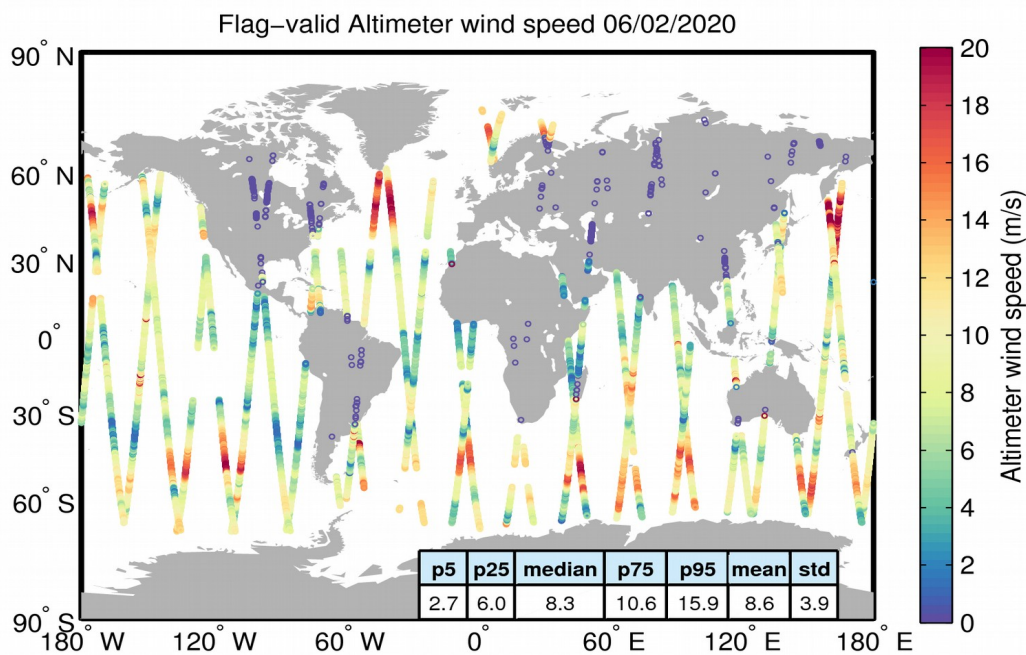
Figure 31. Geographical distribution of flag-valid wind data over oceans and lakes for 06/02/2020. The statistical values shown in the table refer to the wind in m/s and are calculated over all measurements shown in the figure.
