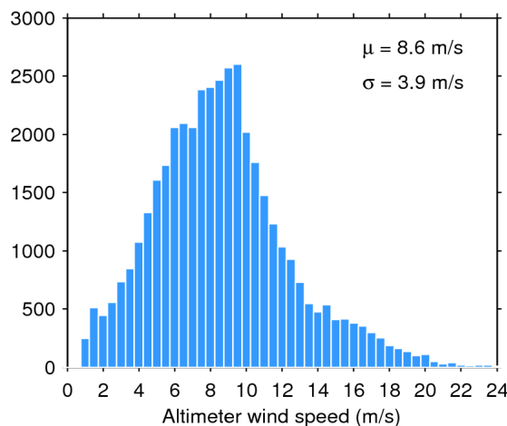
Figure 35. Histogram of science-valid wind over oceans and lakes for 06/02/2020. The mean ( \mu ) and standard deviation ( \sigma ) are also shown. Note that values larger than 24 m/s are excluded from the histogram for the sake of readability but not from the computation of \mu and \sigma .
