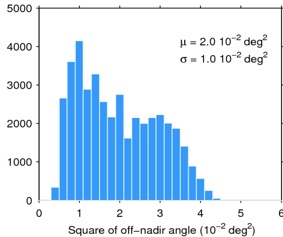
Figure 39. Histogram of flag-valid mispointing over oceans and lakes for 06/02/2020. The mean ( \mu ) and standard deviation ( \sigma ) are also shown. Note that values larger than 6 \cdot 10^{-2} \text{ deg}^2 are excluded from the histogram for the sake of readability but not from the computation of \mu and \sigma .
