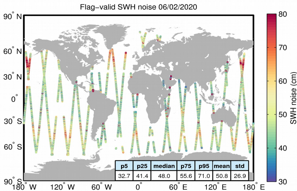
Figure 18. Geographical distribution of flag-valid 20-Hz SWH measurement noise over oceans and lakes for 06/02/2020. The statistical values shown in the figure refer to the SWH noise and are calculated over all measurements shown in the figure.
