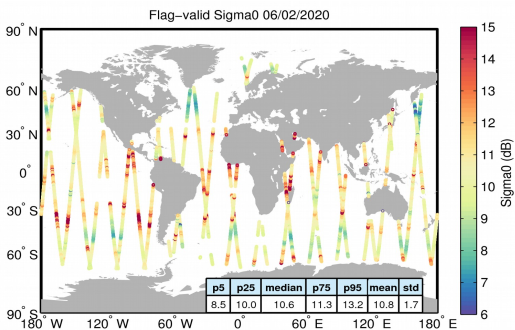
Figure 23. Geographical distribution of flag-valid sigma0 data over oceans and lakes for 06/02/2020. The statistical values shown in the table refer to the sigma0 in dB and are calculated over all measurements shown in the figure.
