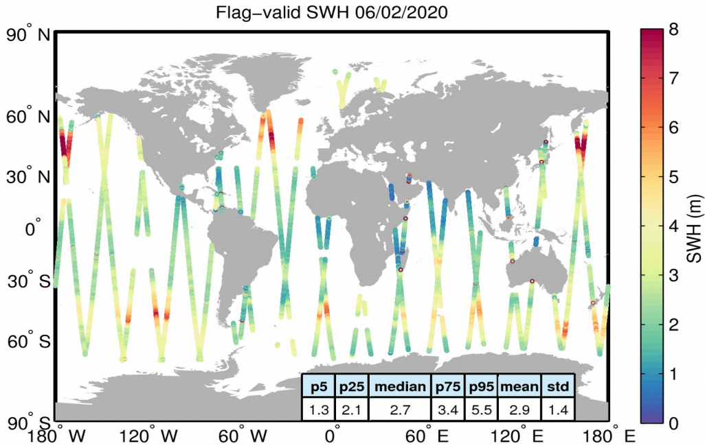
Figure 15. Geographical distribution of flag-valid SWH data over oceans and lakes for 06/02/2020. The statistical values shown in the table refer to the SWH in m and are calculated over all measurements shown in the figure.
