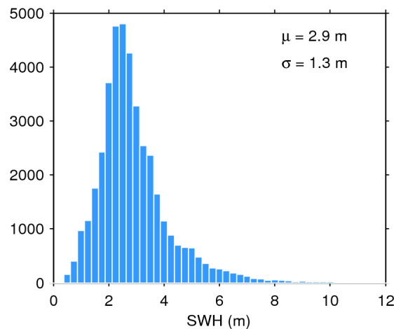
Figure 20. Histogram of science-valid SWH over oceans and lakes for 06/02/2020. The mean ( \mu ) and standard deviation ( \sigma ) are also shown. Note that values larger than 12 m are excluded from the histogram for the sake of readability but not from the computation of \mu and \sigma .
