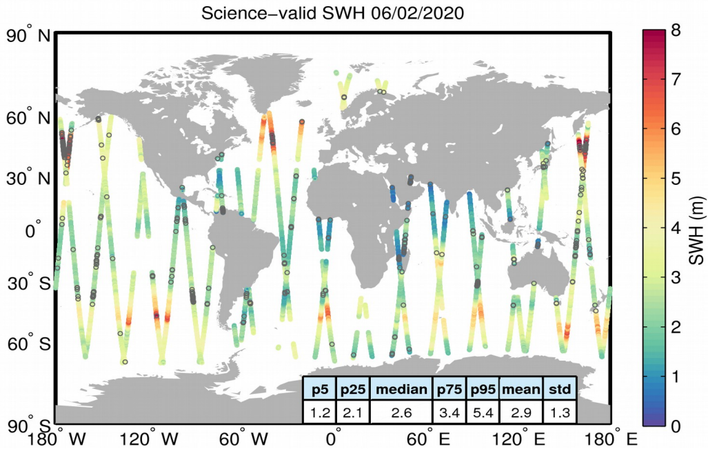
Figure 19. Geographical distribution of science-valid SWH data over oceans and lakes for 06/02/2020. The statistical values shown in the table refer to the SWH in m and are calculated over all measurements shown in the figure. Gray circles denote records that have been rejected based on the editing criteria described in Table 3.
