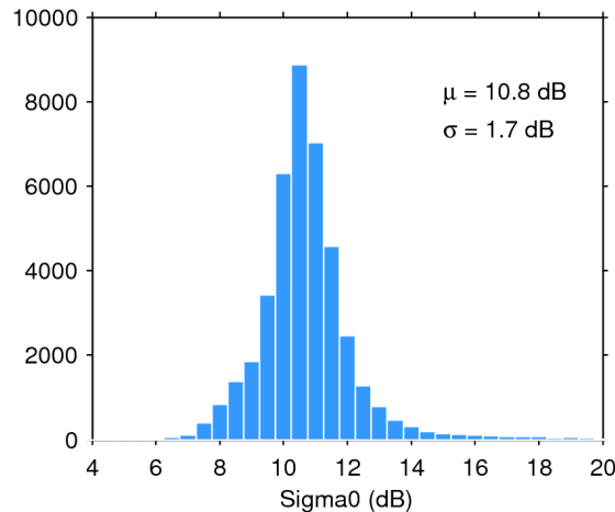
Figure 25. Histogram of flag-valid sigma0 over oceans and lakes for 06/02/2020. The mean ( \mu ) and standard deviation ( \sigma ) are also shown. Note that values outside [4 20] dB are excluded from the histogram for the sake of readability but not from the computation of \mu and \sigma .
