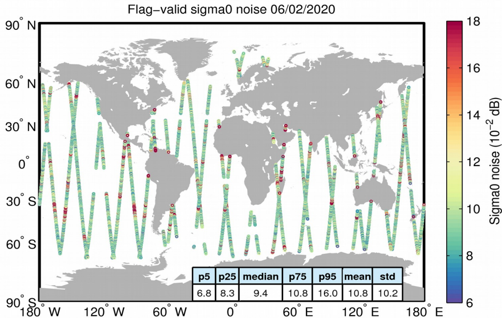
Figure 26. Geographical distribution of flag-valid 20-Hz sigma0 measurement noise over oceans and lakes for 06/02/2020. The statistical values shown in the table refer to the sigma0 noise and are calculated over all measurements shown in the figure.
