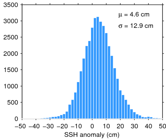
Figure 11. Histogram of science-valid SSH anomaly over oceans and lakes for 06/02/2020. The mean ( \mu ) and standard deviation ( \sigma ) are also shown. Note that values outside [-50 50] cm are excluded from the histogram for the sake of readability but not from the computation of \mu and \sigma .
