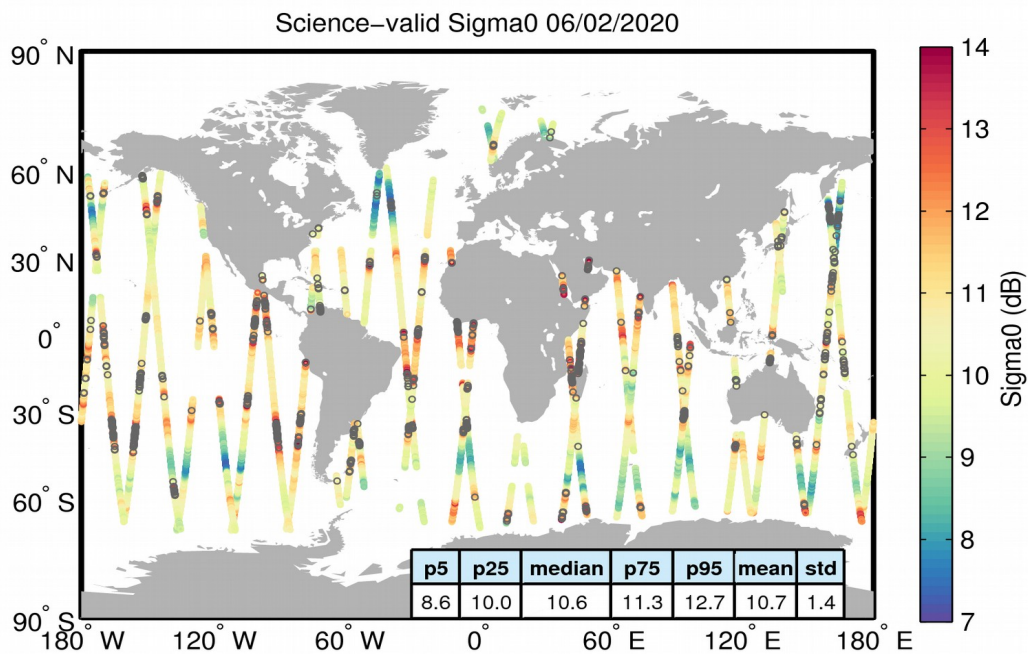
Figure 27. Geographical distribution of science-valid sigma0 data over oceans and lakes for 06/02/2020. The statistical values shown in the table refer to the sigma0 in dB and are calculated over all measurements shown in the figure. Gray circles denote records that have been rejected based on the editing criteria described in Table 4.
