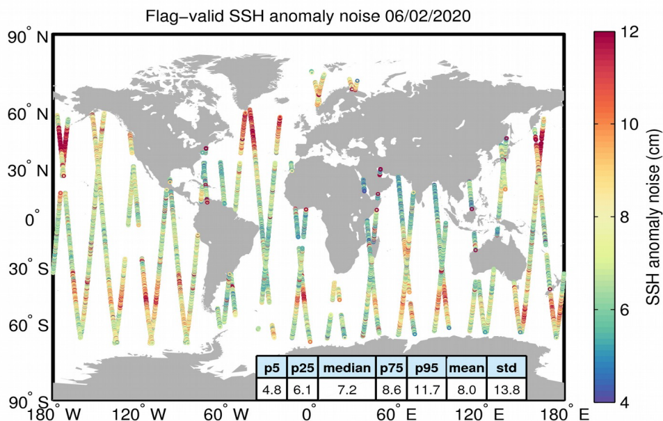
Figure 8. Geographical distribution of flag-valid 20-Hz SSH anomaly measurement noise over oceans and lakes for 06/02/2020. The statistical values shown in the table refer to the SSH anomaly noise and are calculated over all measurements shown in the figure.
