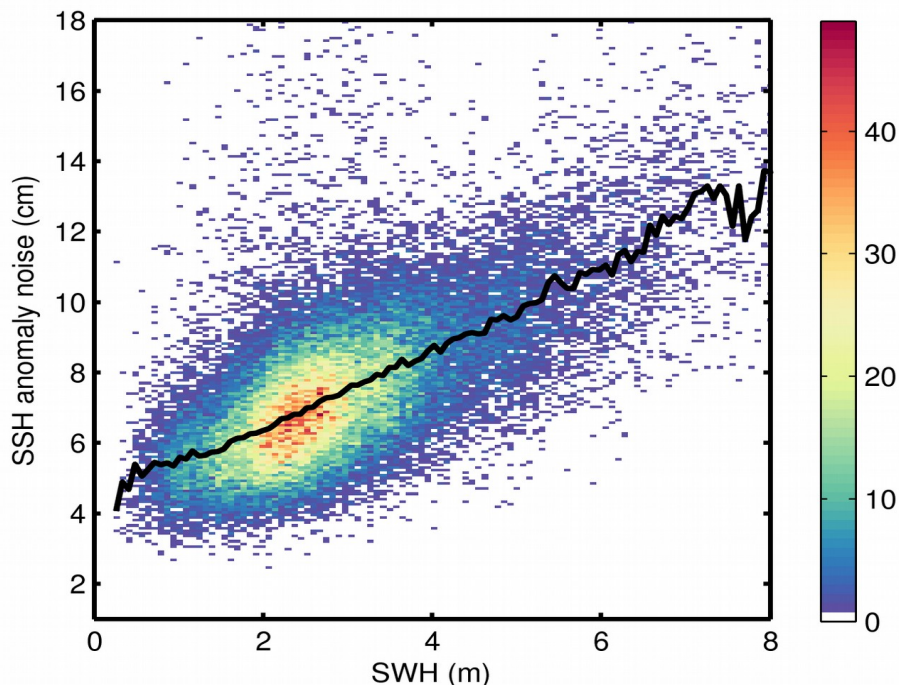
Figure 9. 2D histogram showing flag-valid SSH anomaly noise as a function of SWH for 06/02/2020. The black line denotes the median SSH anomaly noise as a function of SWH.
