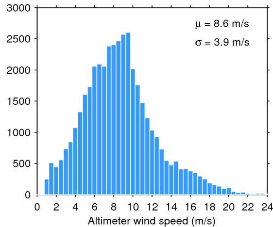
Figure 33. Histogram of flag-valid wind over oceans and lakes for 06/02/2020. The mean ( \mu ) and standard deviation ( \sigma ) are also shown. Note that values larger than 24 m/s are excluded from the histogram for the sake of readability but not from the computation of \mu and \sigma .
