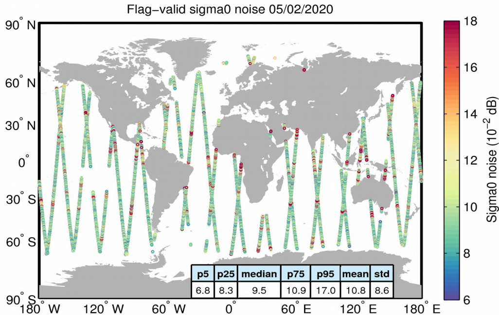
Figure 26. Geographical distribution of flag-valid 20-Hz sigma0 measurement noise over oceans and lakes for 05/02/2020. The statistical values shown in the table refer to the sigma0 noise and are calculated over all measurements shown in the figure.
