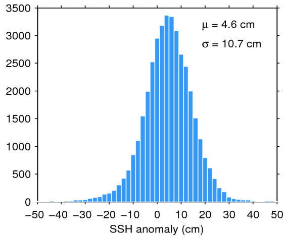
Figure 11. Histogram of science-valid SSH anomaly over oceans and lakes for 05/02/2020. The mean ( \mu ) and standard deviation ( \sigma ) are also shown. Note that values outside [-50 50] cm are excluded from the histogram for the sake of readability but not from the computation of \mu and \sigma .
