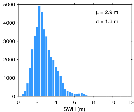
Figure 17. Histogram of flag-valid SWH over oceans and lakes for 05/02/2020. The mean ( \mu ) and standard deviation ( \sigma ) are also shown. Note that values larger than 12 m are excluded from the histogram for the sake of readability but not from the computation of \mu and \sigma .
