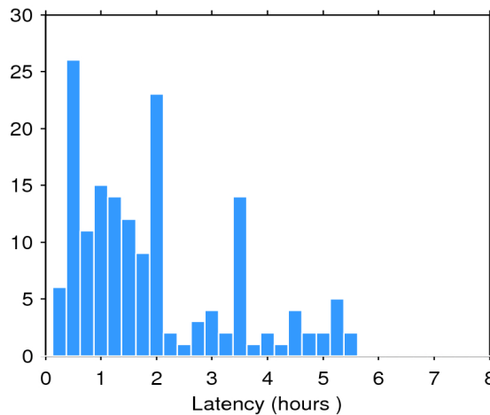
Figure 2. Histogram of the data latency for 05/02/2020. The y-axis denotes the number of files that are made available with a delay of x-hours with respect to the mean time of the records stored in the file.
