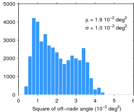
Figure 39. Histogram of flag-valid mispointing over oceans and lakes for 05/02/2020. The mean ( \mu ) and standard deviation ( \sigma ) are also shown. Note that values larger than 6 \cdot 10^{-2} \text{ deg}^2 are excluded from the histogram for the sake of readability but not from the computation of \mu and \sigma .
