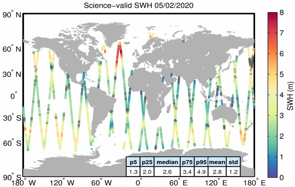
Figure 19. Geographical distribution of science-valid SWH data over oceans and lakes for 05/02/2020. The statistical values shown in the table refer to the SWH in m and are calculated over all measurements shown in the figure. Gray circles denote records that have been rejected based on the editing criteria described in Table 3.
