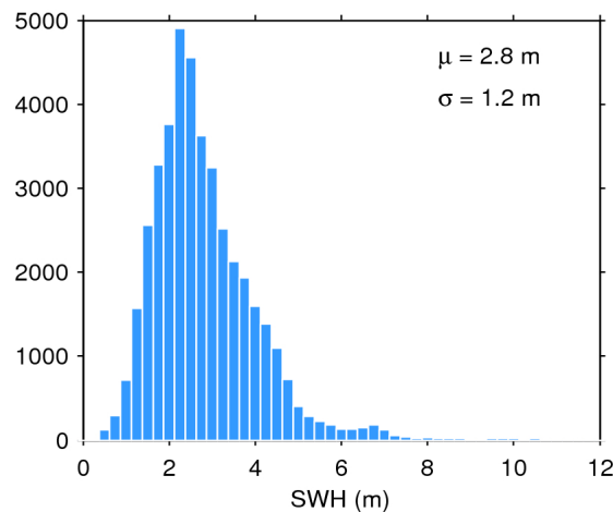
Figure 20. Histogram of science-valid SWH over oceans and lakes for 05/02/2020. The mean ( \mu ) and standard deviation ( \sigma ) are also shown. Note that values larger than 12 m are excluded from the histogram for the sake of readability but not from the computation of \mu and \sigma .
