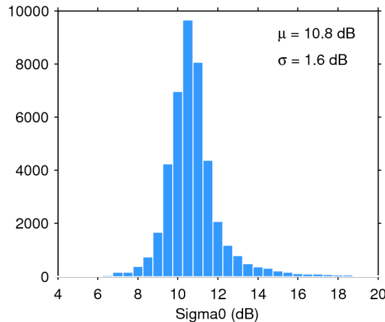
Figure 25. Histogram of flag-valid sigma0 over oceans and lakes for 05/02/2020. The mean ( \mu ) and standard deviation ( \sigma ) are also shown. Note that values outside [4 20] dB are excluded from the histogram for the sake of readability but not from the computation of \mu and \sigma .
