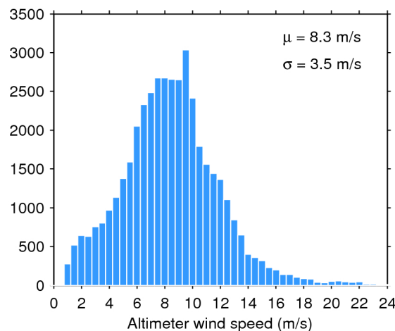
Figure 35. Histogram of science-valid wind over oceans and lakes for 05/02/2020. The mean ( \mu ) and standard deviation ( \sigma ) are also shown. Note that values larger than 24 m/s are excluded from the histogram for the sake of readability but not from the computation of \mu and \sigma .
