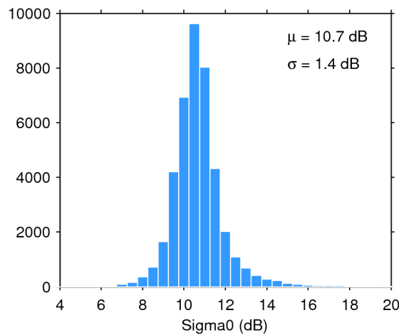
Figure 28. Histogram of science-valid sigma0 over oceans and lakes for 05/02/2020. The mean ( \mu ) and standard deviation ( \sigma ) are also shown. Note that values outside [4 20] dB are excluded from the histogram for the sake of readability but not from the computation of \mu and \sigma .
