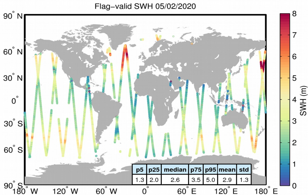
Figure 15. Geographical distribution of flag-valid SWH data over oceans and lakes for 05/02/2020. The statistical values shown in the table refer to the SWH in m and are calculated over all measurements shown in the figure.
