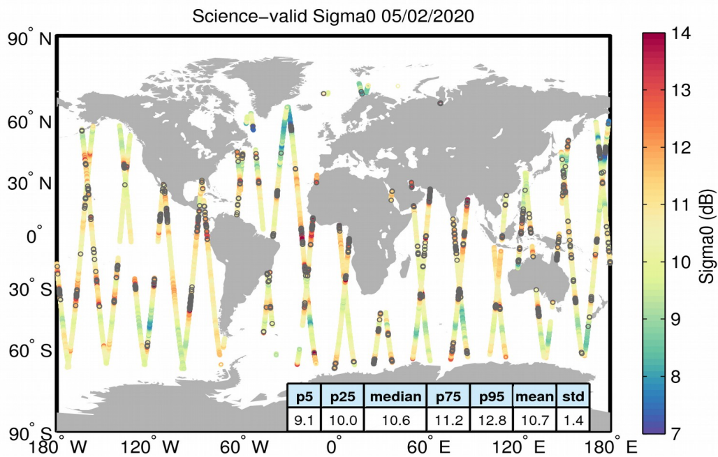
Figure 27. Geographical distribution of science-valid sigma0 data over oceans and lakes for 05/02/2020. The statistical values shown in the table refer to the sigma0 in dB and are calculated over all measurements shown in the figure. Gray circles denote records that have been rejected based on the editing criteria described in Table 4.
