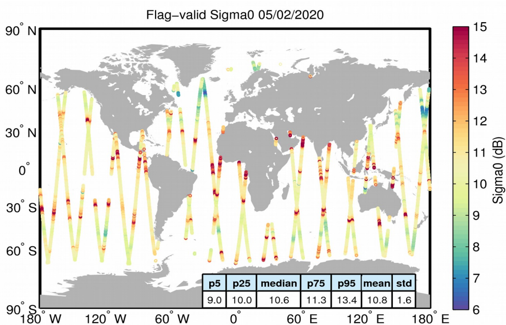
Figure 23. Geographical distribution of flag-valid sigma0 data over oceans and lakes for 05/02/2020. The statistical values shown in the table refer to the sigma0 in dB and are calculated over all measurements shown in the figure.
