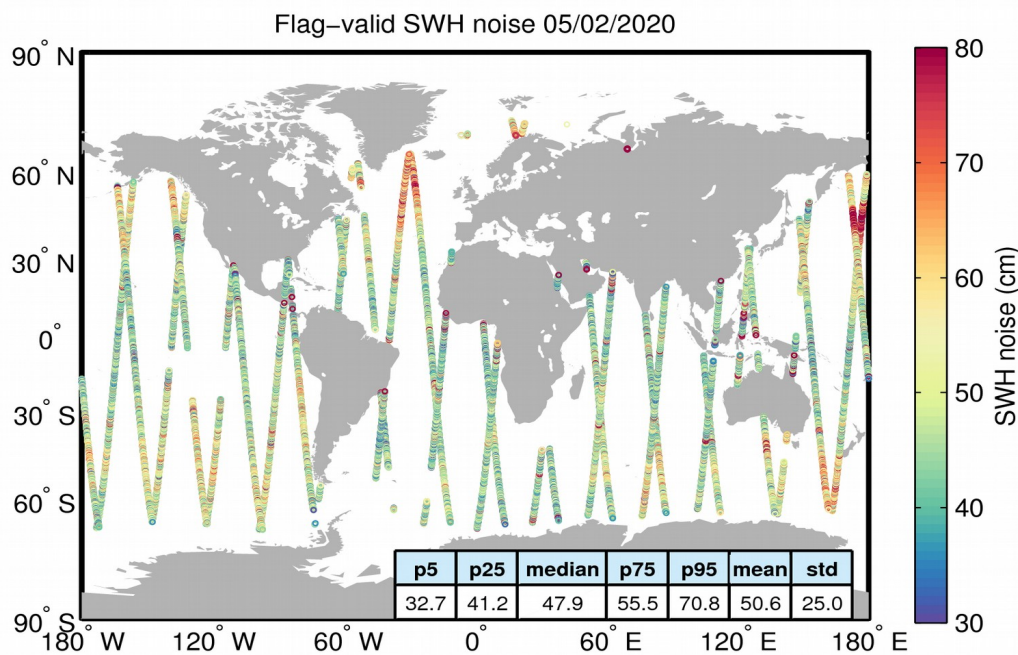
Figure 18. Geographical distribution of flag-valid 20-Hz SWH measurement noise over oceans and lakes for 05/02/2020. The statistical values shown in the figure refer to the SWH noise and are calculated over all measurements shown in the figure.
