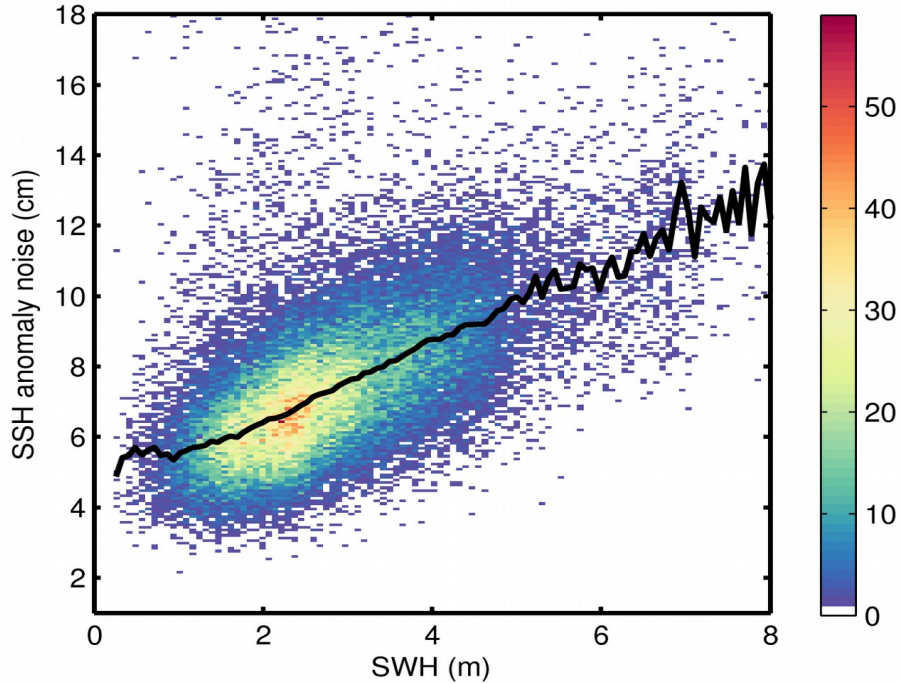
Figure 9. 2D histogram showing flag-valid SSH anomaly noise as a function of SWH for 05/02/2020. The black line denotes the median SSH anomaly noise as a function of SWH.
