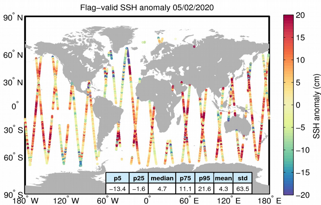
Figure 5. Geographical distribution of flag-valid 1-Hz SSH anomaly data over oceans and lakes for 05/02/2020. The statistical values shown in the table refer to the SSH anomaly in cm and are calculated over all measurements shown in the figure.
