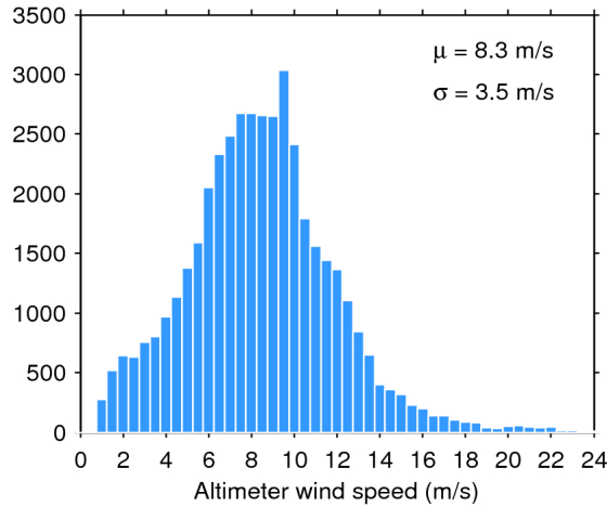
Figure 33. Histogram of flag-valid wind over oceans and lakes for 05/02/2020. The mean ( \mu ) and standard deviation ( \sigma ) are also shown. Note that values larger than 24 m/s are excluded from the histogram for the sake of readability but not from the computation of \mu and \sigma .
