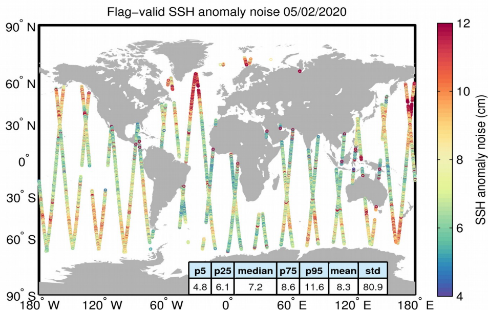
Figure 8. Geographical distribution of flag-valid 20-Hz SSH anomaly measurement noise over oceans and lakes for 05/02/2020. The statistical values shown in the table refer to the SSH anomaly noise and are calculated over all measurements shown in the figure.
