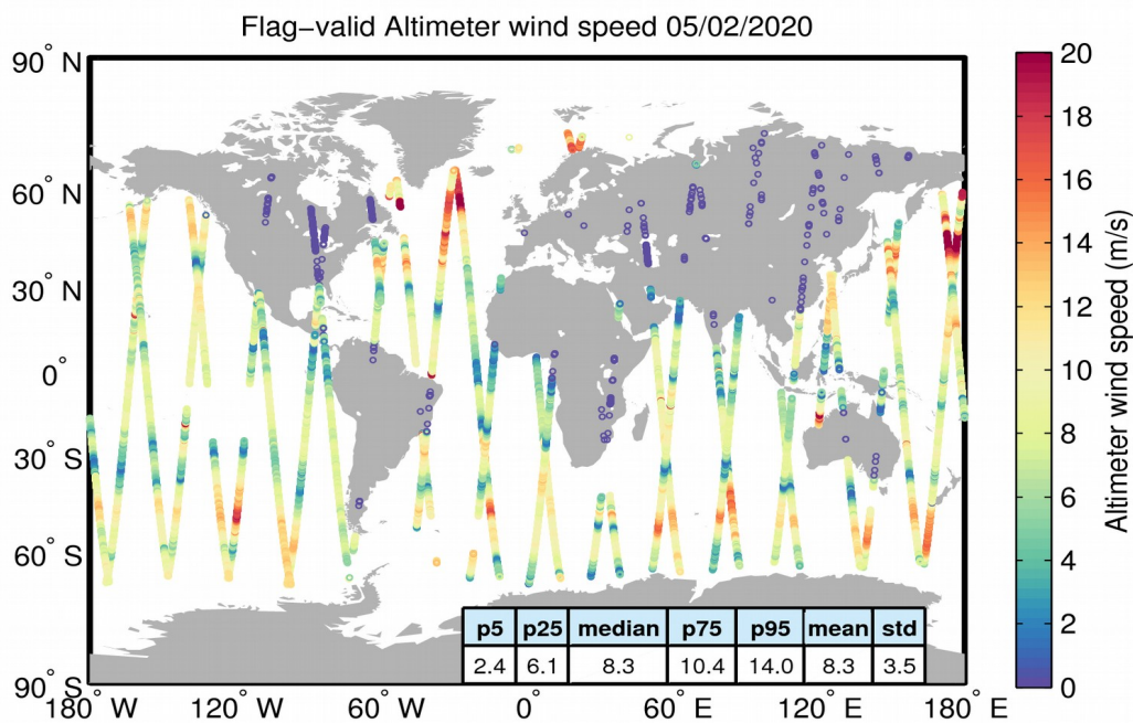
Figure 31. Geographical distribution of flag-valid wind data over oceans and lakes for 05/02/2020. The statistical values shown in the table refer to the wind in m/s and are calculated over all measurements shown in the figure.
