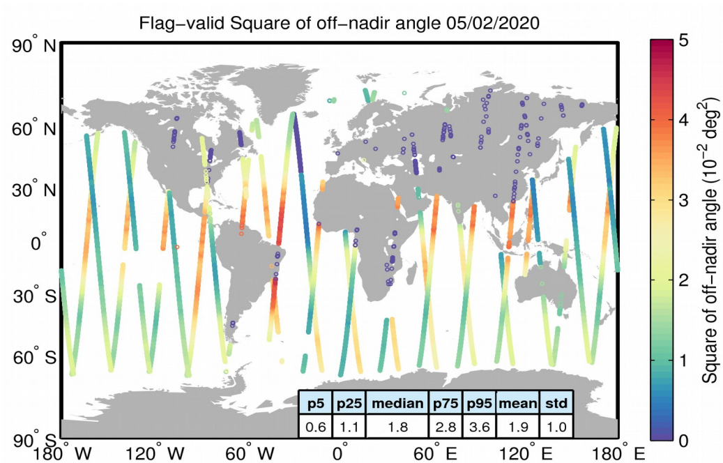
Figure 37. Geographical distribution of flag-valid mispointing data over oceans and lakes for 05/02/2020. The statistical values shown in the table refer to the mispointing in 10^{-2} deg 2 and are calculated over all measurements shown in the figure.
