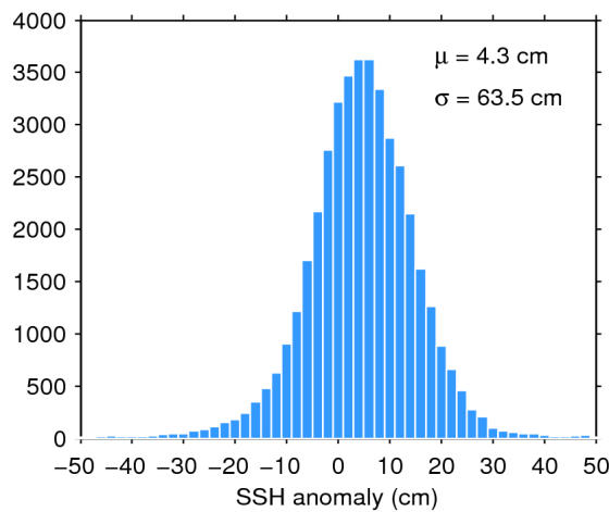
Figure 7. Histogram of flag-valid SSH anomaly over oceans and lakes for 05/02/2020. The mean ( \mu ) and standard deviation ( \sigma ) are also shown. Note that values outside [-50 50] cm are excluded from the histogram for the sake of readability but not from the computation of \mu and \sigma .
