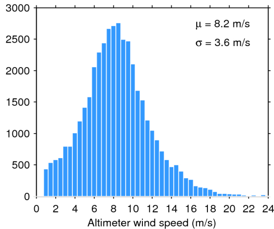
Figure 33. Histogram of flag-valid wind over oceans and lakes for 04/02/2020. The mean ( \mu ) and standard deviation ( \sigma ) are also shown. Note that values larger than 24 m/s are excluded from the histogram for the sake of readability but not from the computation of \mu and \sigma .
