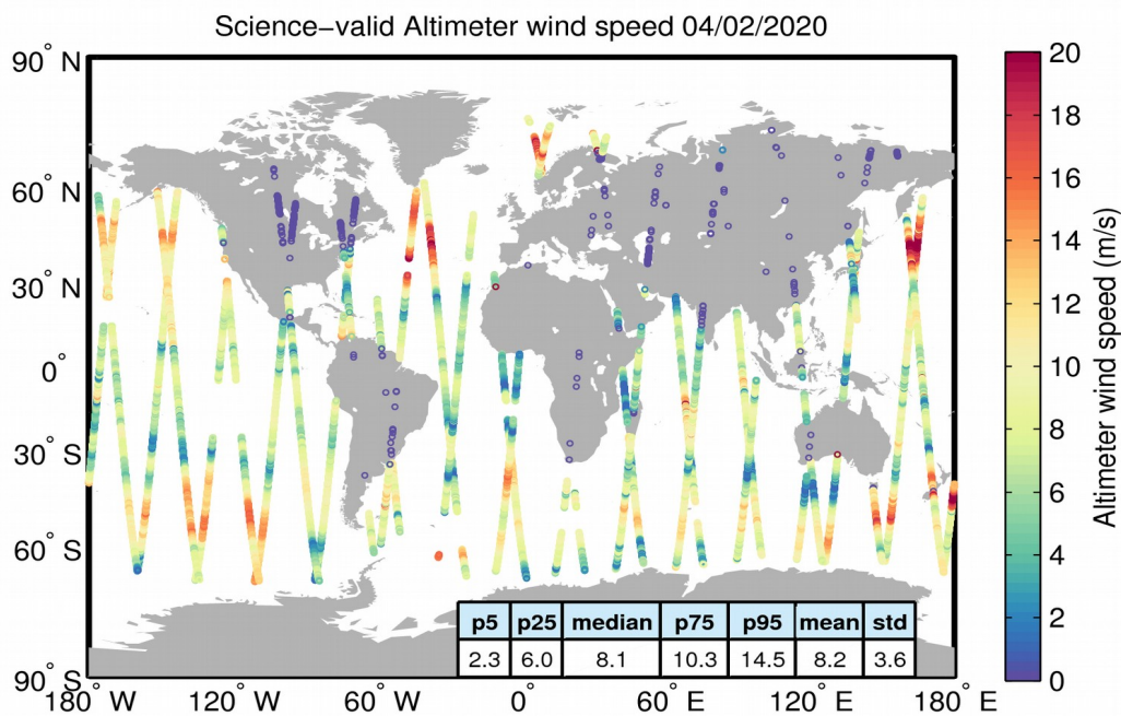
Figure 34. Geographical distribution of science-valid wind data over oceans and lakes for 04/02/2020. The statistical values shown in the table refer to the wind in m/s and are calculated over all measurements shown in the figure. Gray circles denote records that have been rejected based on the editing criteria described in Table 5.
