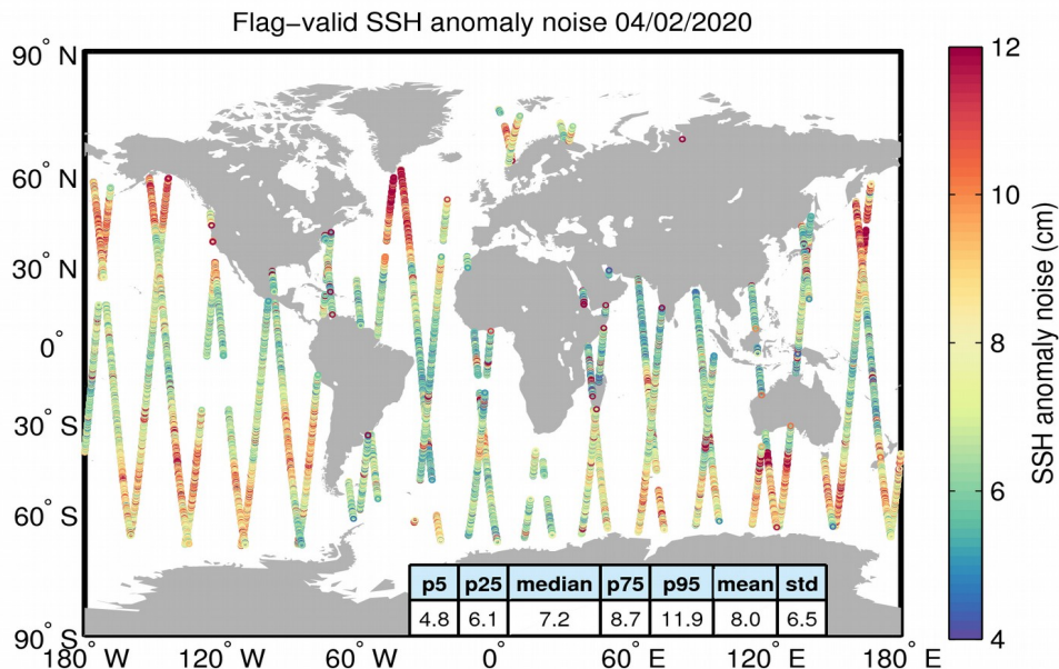
Figure 8. Geographical distribution of flag-valid 20-Hz SSH anomaly measurement noise over oceans and lakes for 04/02/2020. The statistical values shown in the table refer to the SSH anomaly noise and are calculated over all measurements shown in the figure.
