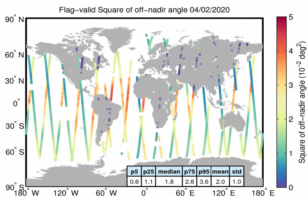
Figure 37. Geographical distribution of flag-valid mispointing data over oceans and lakes for 04/02/2020. The statistical values shown in the table refer to the mispointing in 10^{-2} deg 2 and are calculated over all measurements shown in the figure.
