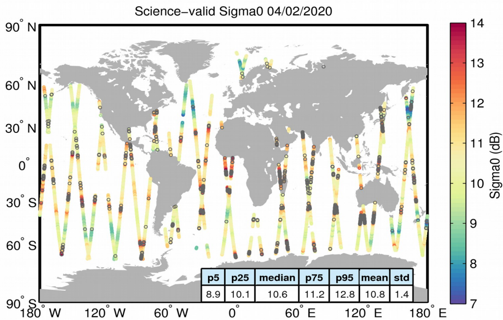
Figure 27. Geographical distribution of science-valid sigma0 data over oceans and lakes for 04/02/2020. The statistical values shown in the table refer to the sigma0 in dB and are calculated over all measurements shown in the figure. Gray circles denote records that have been rejected based on the editing criteria described in Table 4.
