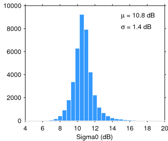
Figure 28. Histogram of science-valid sigma0 over oceans and lakes for 04/02/2020. The mean ( \mu ) and standard deviation ( \sigma ) are also shown. Note that values outside [4 20] dB are excluded from the histogram for the sake of readability but not from the computation of \mu and \sigma .
