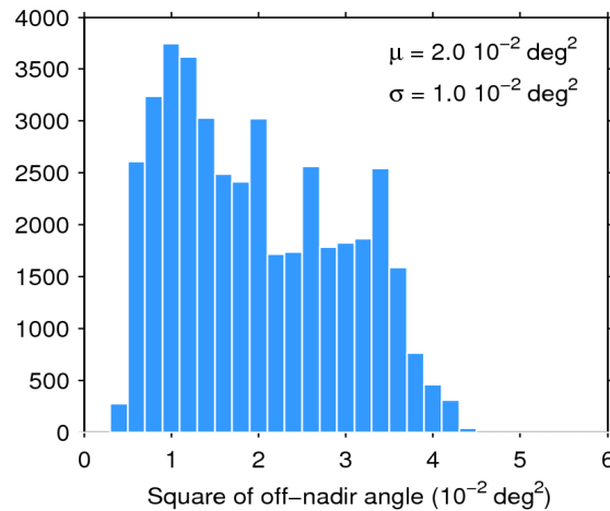
Figure 39. Histogram of flag-valid mispointing over oceans and lakes for 04/02/2020. The mean ( \mu ) and standard deviation ( \sigma ) are also shown. Note that values larger than 6 \cdot 10^{-2} \text{ deg}^2 are excluded from the histogram for the sake of readability but not from the computation of \mu and \sigma .
