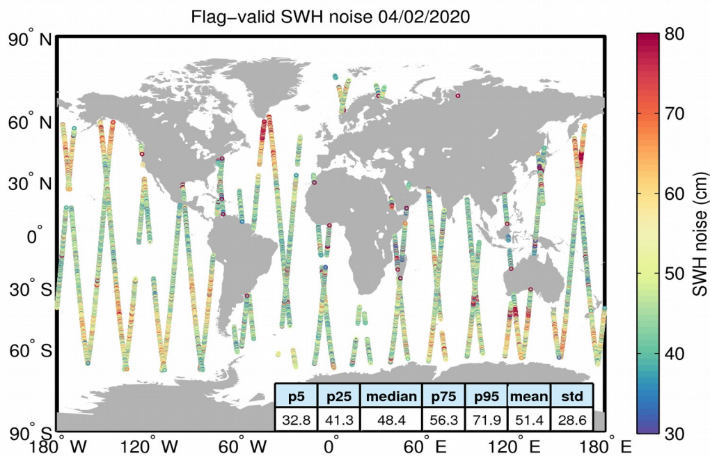
Figure 18. Geographical distribution of flag-valid 20-Hz SWH measurement noise over oceans and lakes for 04/02/2020. The statistical values shown in the figure refer to the SWH noise and are calculated over all measurements shown in the figure.
