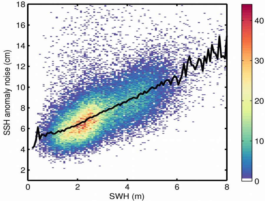
Figure 9. 2D histogram showing flag-valid SSH anomaly noise as a function of SWH for 04/02/2020. The black line denotes the median SSH anomaly noise as a function of SWH.
