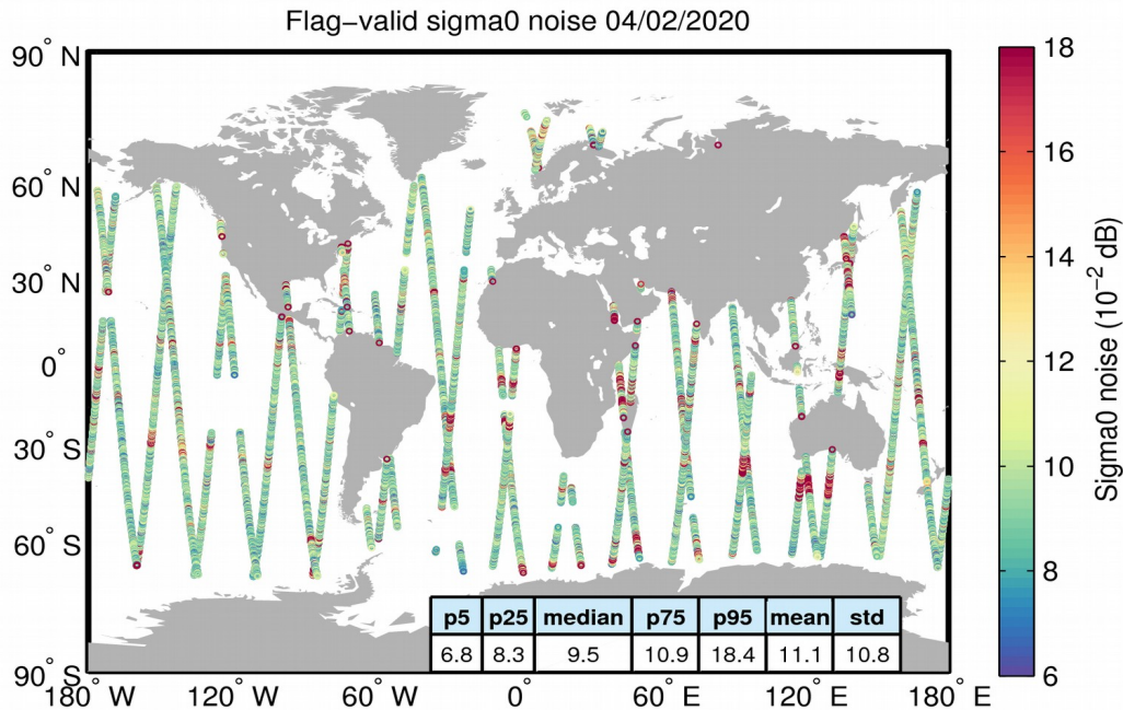
Figure 26. Geographical distribution of flag-valid 20-Hz sigma0 measurement noise over oceans and lakes for 04/02/2020. The statistical values shown in the table refer to the sigma0 noise and are calculated over all measurements shown in the figure.
