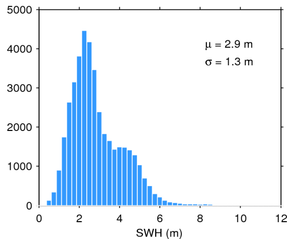
Figure 17. Histogram of flag-valid SWH over oceans and lakes for 04/02/2020. The mean ( \mu ) and standard deviation ( \sigma ) are also shown. Note that values larger than 12 m are excluded from the histogram for the sake of readability but not from the computation of \mu and \sigma .
