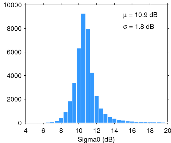
Figure 25. Histogram of flag-valid sigma0 over oceans and lakes for 04/02/2020. The mean ( \mu ) and standard deviation ( \sigma ) are also shown. Note that values outside [4 20] dB are excluded from the histogram for the sake of readability but not from the computation of \mu and \sigma .
