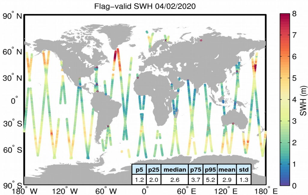
Figure 15. Geographical distribution of flag-valid SWH data over oceans and lakes for 04/02/2020. The statistical values shown in the table refer to the SWH in m and are calculated over all measurements shown in the figure.
