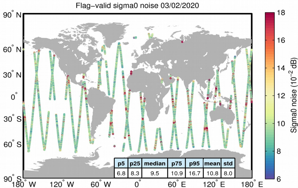
Figure 26. Geographical distribution of flag-valid 20-Hz sigma0 measurement noise over oceans and lakes for 03/02/2020. The statistical values shown in the table refer to the sigma0 noise and are calculated over all measurements shown in the figure.
