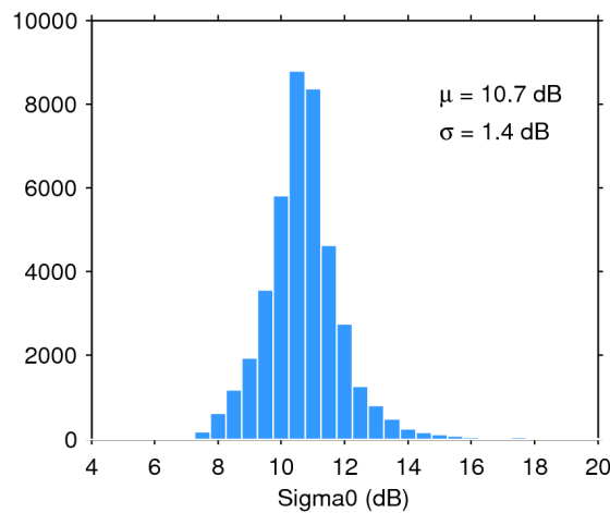
Figure 28. Histogram of science-valid sigma0 over oceans and lakes for 03/02/2020. The mean ( \mu ) and standard deviation ( \sigma ) are also shown. Note that values outside [4 20] dB are excluded from the histogram for the sake of readability but not from the computation of \mu and \sigma .
