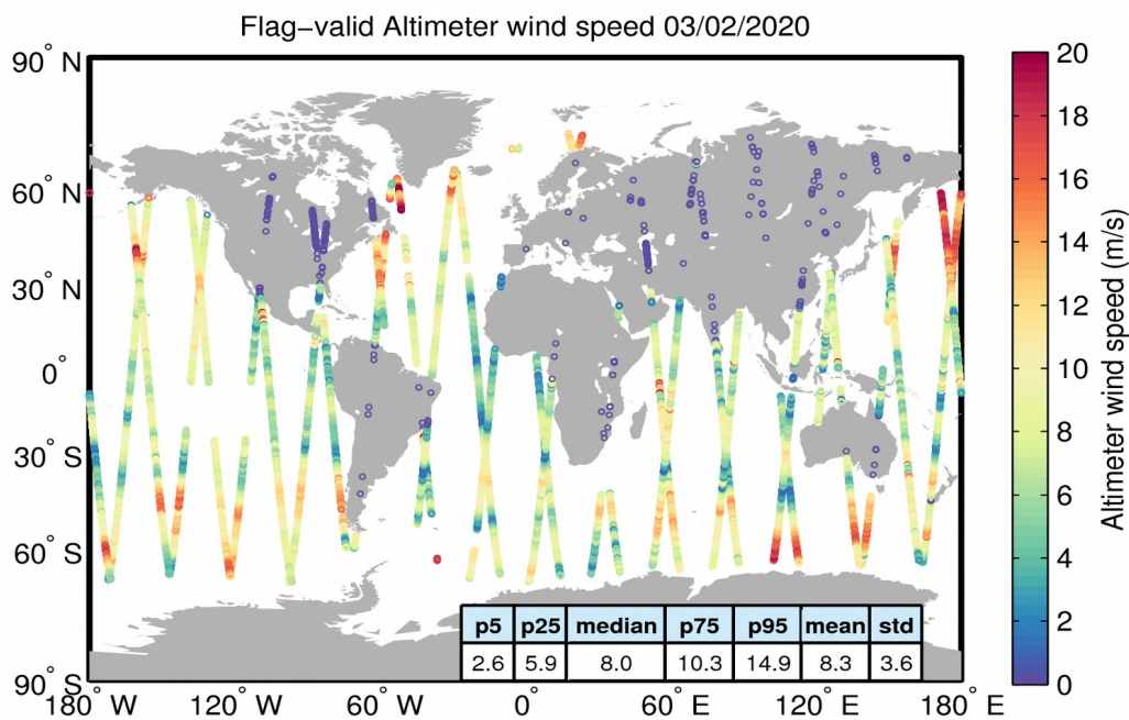
Figure 31. Geographical distribution of flag-valid wind data over oceans and lakes for 03/02/2020. The statistical values shown in the table refer to the wind in m/s and are calculated over all measurements shown in the figure.
