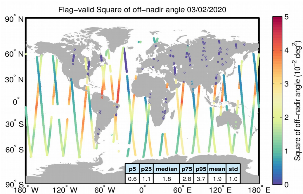
Figure 37. Geographical distribution of flag-valid mispointing data over oceans and lakes for 03/02/2020. The statistical values shown in the table refer to the mispointing in 10^{-2} \text{deg}^2 and are calculated over all measurements shown in the figure.
