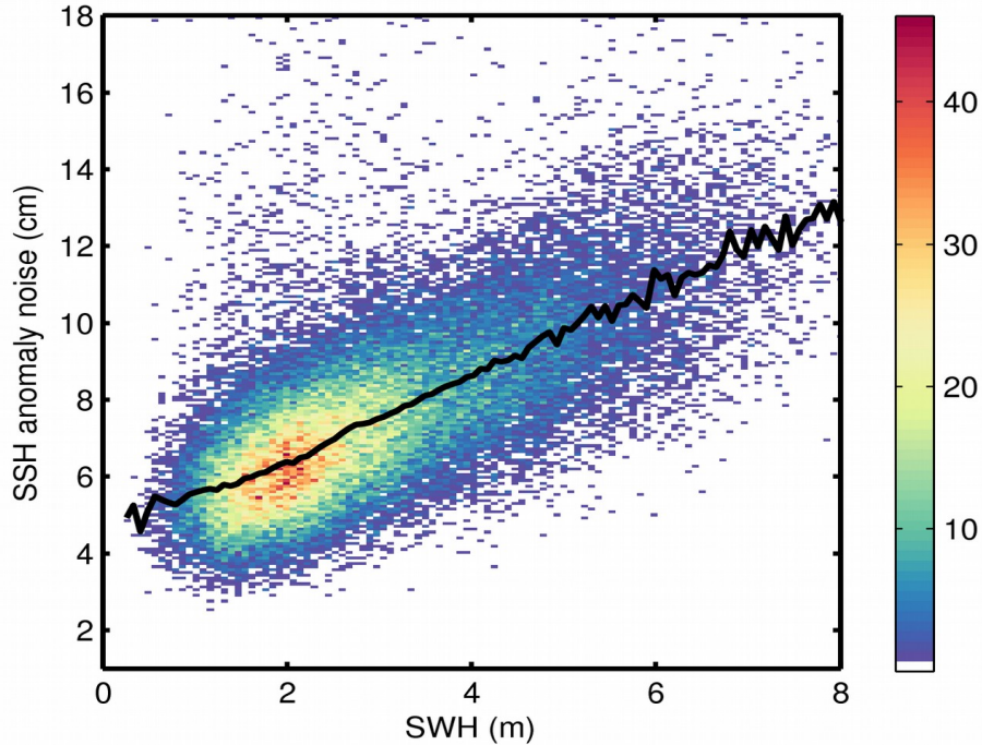
Figure 9. 2D histogram showing flag-valid SSH anomaly noise as a function of SWH for 03/02/2020. The black line denotes the median SSH anomaly noise as a function of SWH.
