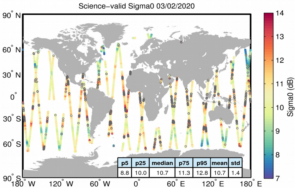
Figure 27. Geographical distribution of science-valid sigma0 data over oceans and lakes for 03/02/2020. The statistical values shown in the table refer to the sigma0 in dB and are calculated over all measurements shown in the figure. Gray circles denote records that have been rejected based on the editing criteria described in Table 4.
