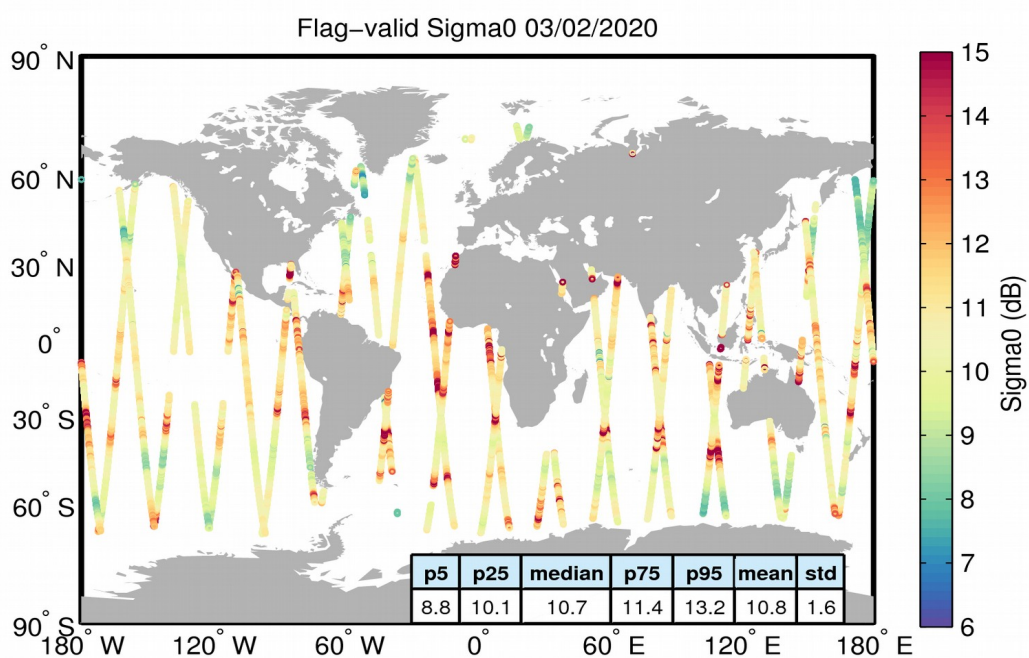
Figure 23. Geographical distribution of flag-valid sigma0 data over oceans and lakes for 03/02/2020. The statistical values shown in the table refer to the sigma0 in dB and are calculated over all measurements shown in the figure.
