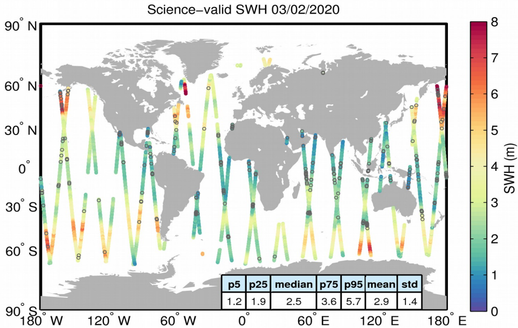
Figure 19. Geographical distribution of science-valid SWH data over oceans and lakes for 03/02/2020. The statistical values shown in the table refer to the SWH in m and are calculated over all measurements shown in the figure. Gray circles denote records that have been rejected based on the editing criteria described in Table 3.
