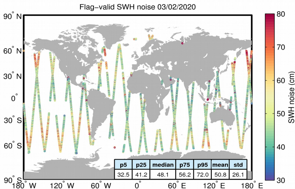
Figure 18. Geographical distribution of flag-valid 20-Hz SWH measurement noise over oceans and lakes for 03/02/2020. The statistical values shown in the table refer to the SWH noise and are calculated over all measurements shown in the figure.
