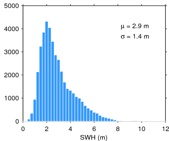
Figure 20. Histogram of science-valid SWH over oceans and lakes for 03/02/2020. The mean ( \mu ) and standard deviation ( \sigma ) are also shown. Note that values larger than 12 m are excluded from the histogram for the sake of readability but not from the computation of \mu and \sigma .
