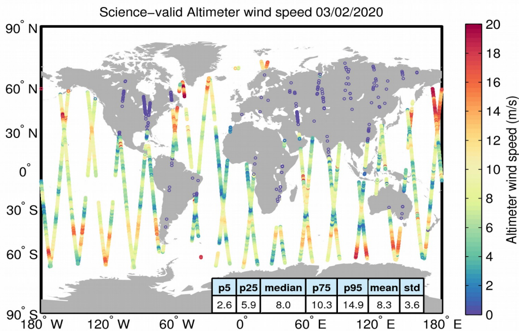
Figure 34. Geographical distribution of science-valid wind data over oceans and lakes for 03/02/2020. The statistical values shown in the table refer to the wind in m/s and are calculated over all measurements shown in the figure. Gray circles denote records that have been rejected based on the editing criteria described in Table 5.
