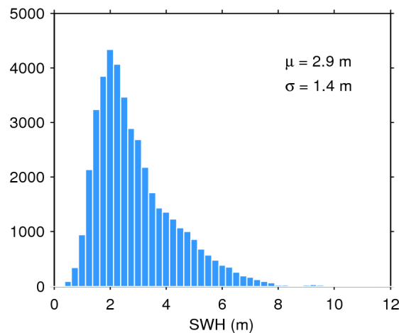
Figure 17. Histogram of flag-valid SWH over oceans and lakes for 03/02/2020. The mean ( \mu ) and standard deviation ( \sigma ) are also shown. Note that values larger than 12 m are excluded from the histogram for the sake of readability but not from the computation of \mu and \sigma .
