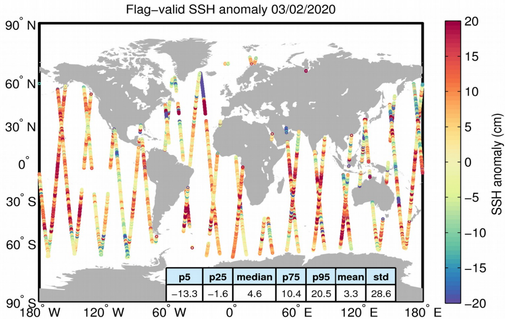
Figure 5. Geographical distribution of flag-valid 1-Hz SSH anomaly data over oceans and lakes for 03/02/2020. The statistical values shown in the table refer to the SSH anomaly in cm and are calculated over all measurements shown in the figure.
