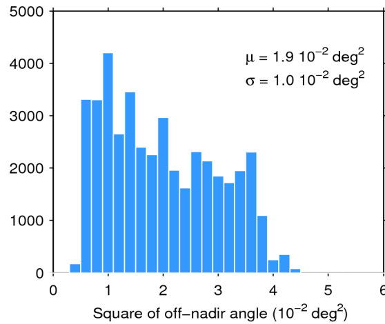
Figure 39. Histogram of flag-valid mispointing over oceans and lakes for 03/02/2020. The mean ( \mu ) and standard deviation ( \sigma ) are also shown. Note that values larger than 6 \cdot 10^{-2} \text{ deg}^2 are excluded from the histogram for the sake of readability but not from the computation of \mu and \sigma .
