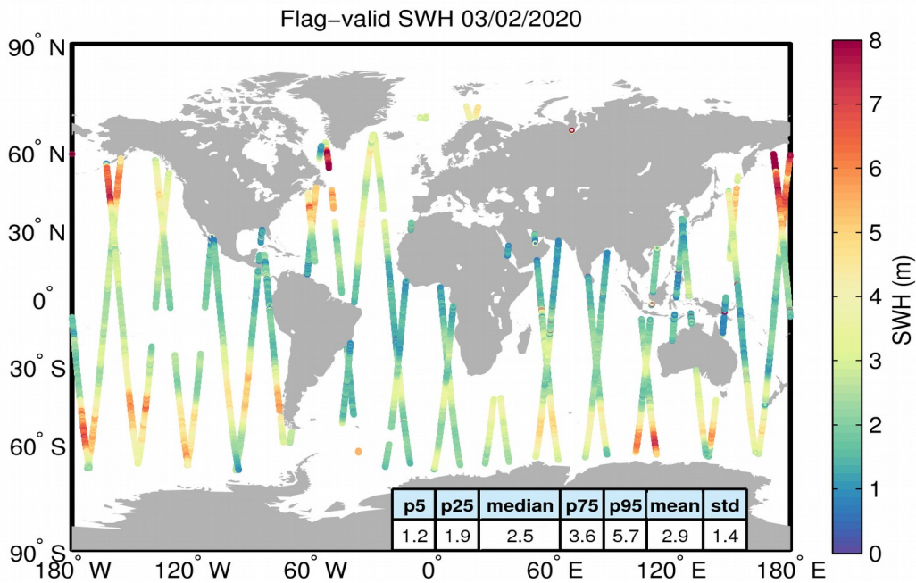
Figure 15. Geographical distribution of flag-valid SWH data over oceans and lakes for 03/02/2020. The statistical values shown in the table refer to the SWH in m and are calculated over all measurements shown in the figure.
