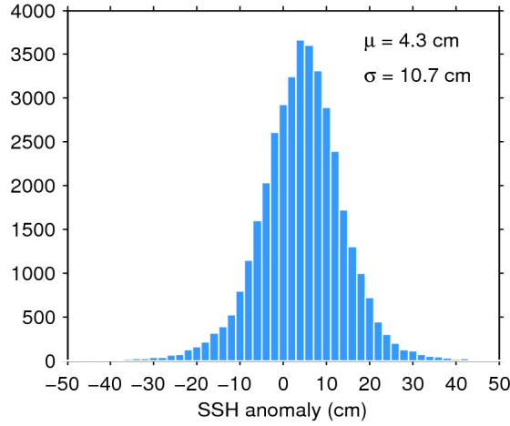
Figure 11. Histogram of science-valid SSH anomaly over oceans and lakes for 03/02/2020. The mean ( \mu ) and standard deviation ( \sigma ) are also shown. Note that values outside [-50 50] cm are excluded from the histogram for the sake of readability but not from the computation of \mu and \sigma .
