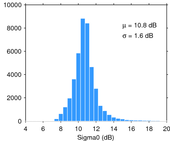
Figure 25. Histogram of flag-valid sigma0 over oceans and lakes for 03/02/2020. The mean ( \mu ) and standard deviation ( \sigma ) are also shown. Note that values outside [4 20] dB are excluded from the histogram for the sake of readability but not from the computation of \mu and \sigma .
