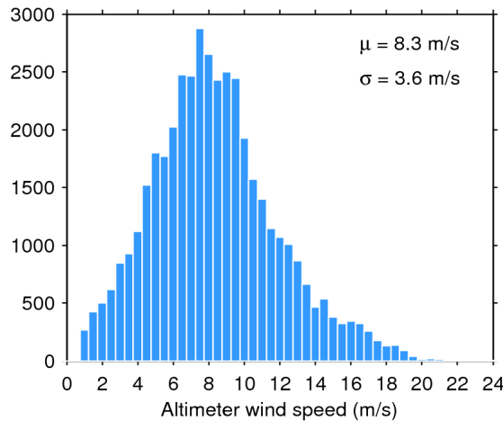
Figure 33. Histogram of flag-valid wind over oceans and lakes for 03/02/2020. The mean ( \mu ) and standard deviation ( \sigma ) are also shown. Note that values larger than 24 m/s are excluded from the histogram for the sake of readability but not from the computation of \mu and \sigma .
