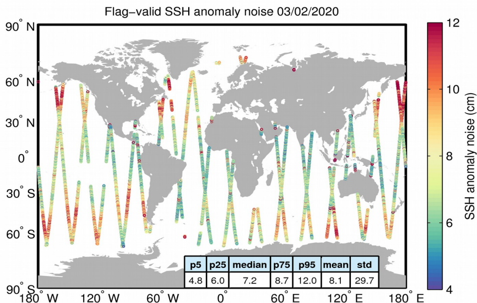
Figure 8. Geographical distribution of flag-valid 20-Hz SSH anomaly measurement noise over oceans and lakes for 03/02/2020. The statistical values shown in the table refer to the SSH anomaly noise and are calculated over all measurements shown in the figure.
