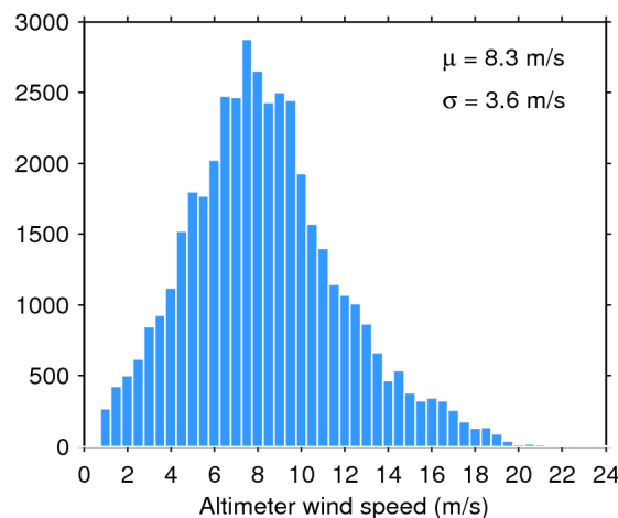
Figure 35. Histogram of science-valid wind over oceans and lakes for 03/02/2020. The mean ( \mu ) and standard deviation ( \sigma ) are also shown. Note that values larger than 24 m/s are excluded from the histogram for the sake of readability but not from the computation of \mu and \sigma .
