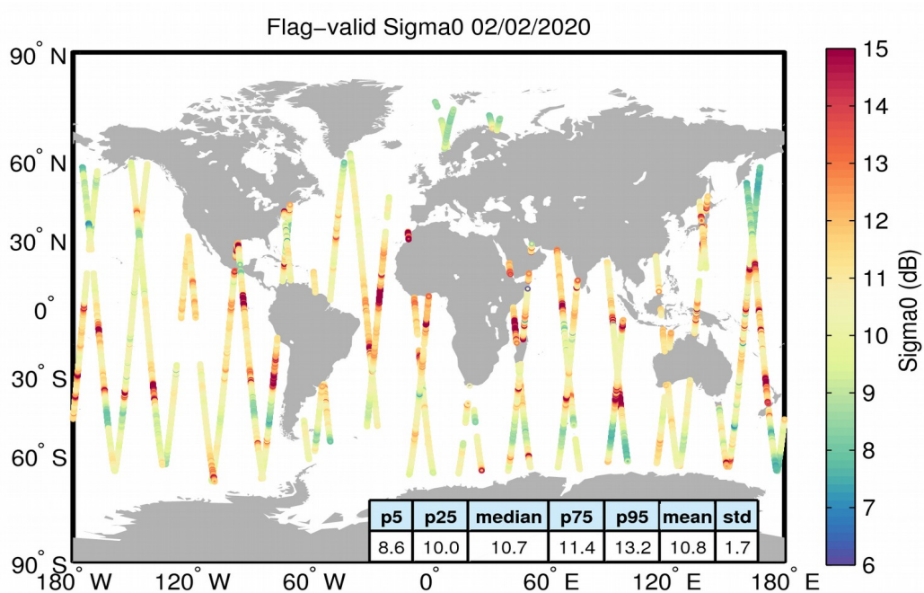
Figure 23. Geographical distribution of flag-valid sigma0 data over oceans and lakes for 02/02/2020. The statistical values shown in the table refer to the sigma0 in dB and are calculated over all measurements shown in the figure.
