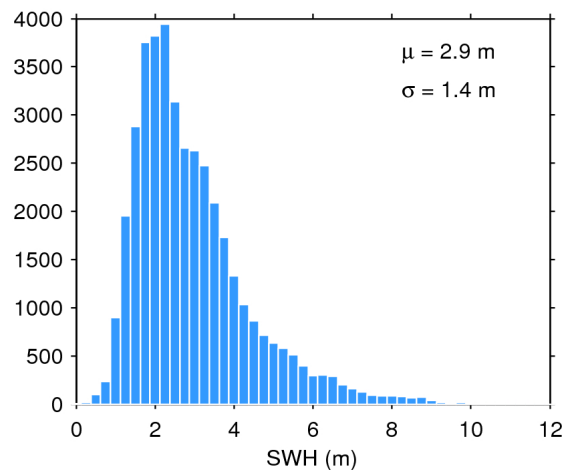
Figure 20. Histogram of science-valid SWH over oceans and lakes for 02/02/2020. The mean ( \mu ) and standard deviation ( \sigma ) are also shown. Note that values larger than 12 m are excluded from the histogram for the sake of readability but not from the computation of \mu and \sigma .
