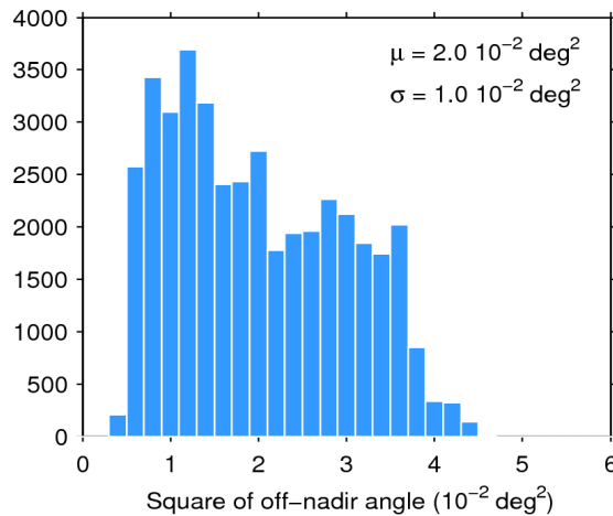
Figure 39. Histogram of flag-valid mispointing over oceans and lakes for 02/02/2020. The mean ( \mu ) and standard deviation ( \sigma ) are also shown. Note that values larger than 6 \cdot 10^{-2} \text{ deg}^2 are excluded from the histogram for the sake of readability but not from the computation of \mu and \sigma .
