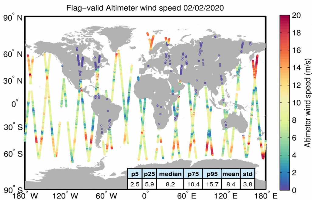
Figure 31. Geographical distribution of flag-valid wind data over oceans and lakes for 02/02/2020. The statistical values shown in the table refer to the wind in m/s and are calculated over all measurements shown in the figure.
