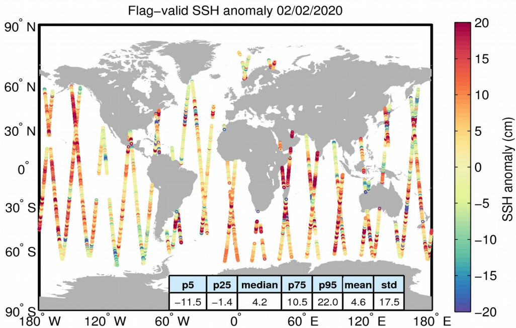
Figure 5. Geographical distribution of flag-valid 1-Hz SSH anomaly data over oceans and lakes for 02/02/2020. The statistical values shown in the table refer to the SSH anomaly in cm and are calculated over all measurements shown in the figure.
