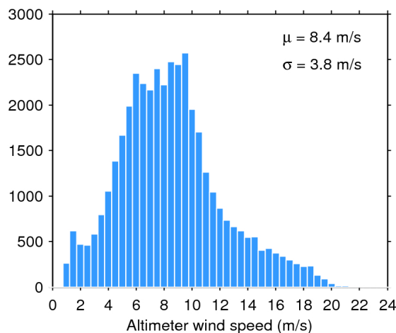
Figure 35. Histogram of science-valid wind over oceans and lakes for 02/02/2020. The mean ( \mu ) and standard deviation ( \sigma ) are also shown. Note that values larger than 24 m/s are excluded from the histogram for the sake of readability but not from the computation of \mu and \sigma .
