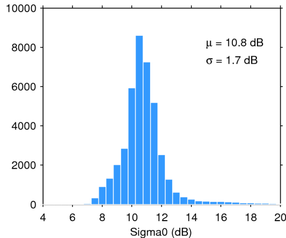
Figure 25. Histogram of flag-valid sigma0 over oceans and lakes for 02/02/2020. The mean ( \mu ) and standard deviation ( \sigma ) are also shown. Note that values outside [4 20] dB are excluded from the histogram for the sake of readability but not from the computation of \mu and \sigma .
