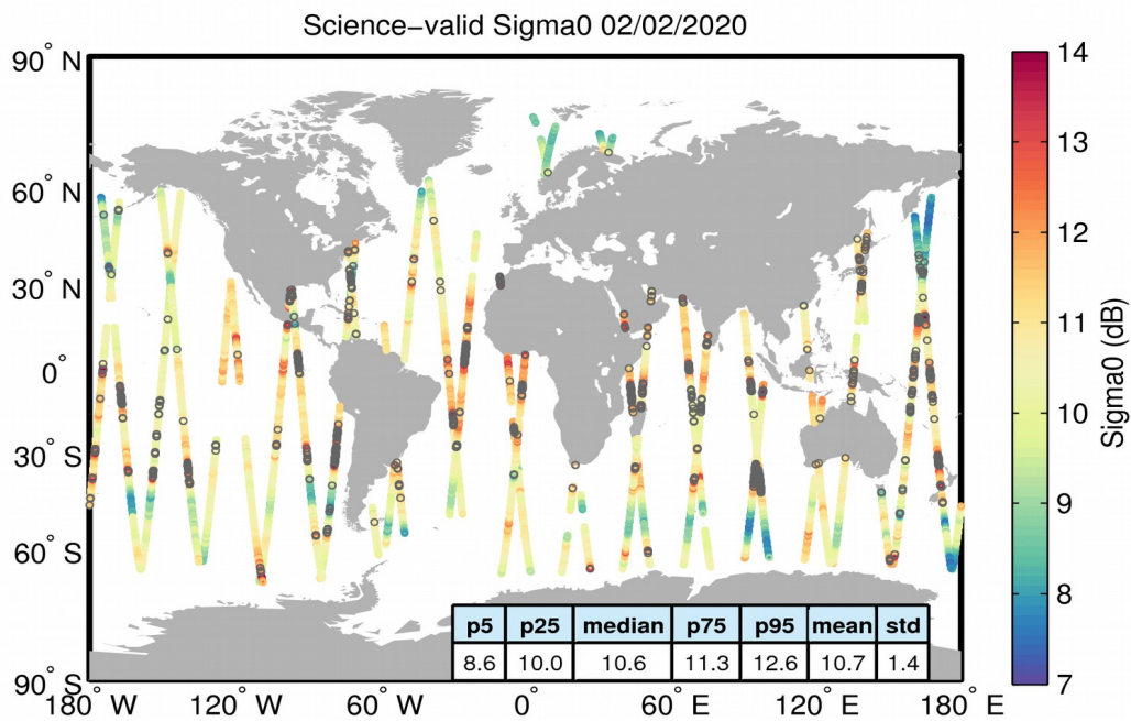
Figure 27. Geographical distribution of science-valid sigma0 data over oceans and lakes for 02/02/2020. The statistical values shown in the table refer to the sigma0 in dB and are calculated over all measurements shown in the figure. Gray circles denote records that have been rejected based on the editing criteria described in Table 4.
