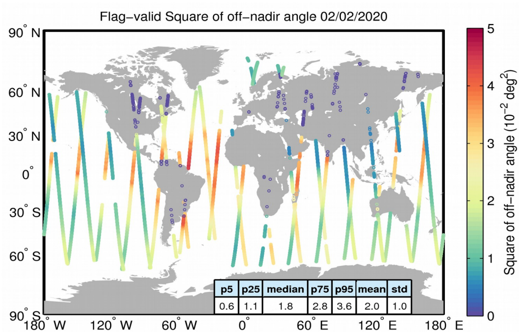
Figure 37. Geographical distribution of flag-valid mispointing data over oceans and lakes for 02/02/2020. The statistical values shown in the table refer to the mispointing in 10^{-2} deg 2 and are calculated over all measurements shown in the figure.
