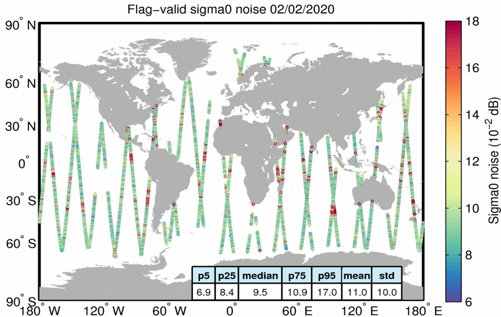
Figure 26. Geographical distribution of flag-valid 20-Hz sigma0 measurement noise over oceans and lakes for 02/02/2020. The statistical values shown in the table refer to the sigma0 noise and are calculated over all measurements shown in the figure.
