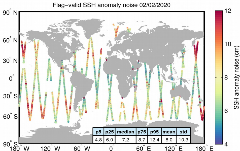
Figure 8. Geographical distribution of flag-valid 20-Hz SSH anomaly measurement noise over oceans and lakes for 02/02/2020. The statistical values shown in the table refer to the SSH anomaly noise and are calculated over all measurements shown in the figure.
