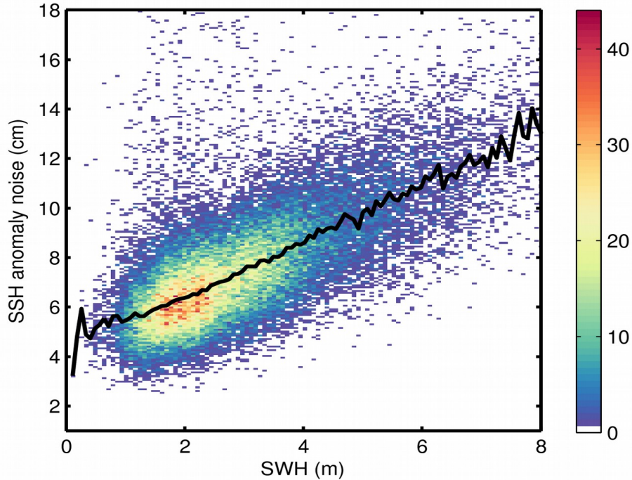
Figure 9. 2D histogram showing flag-valid SSH anomaly noise as a function of SWH for 02/02/2020. The black line denotes the median SSH anomaly noise as a function of SWH.
