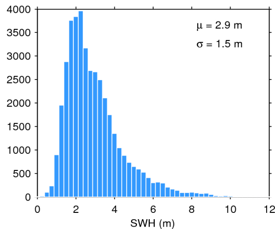
Figure 17. Histogram of flag-valid SWH over oceans and lakes for 02/02/2020. The mean ( \mu ) and standard deviation ( \sigma ) are also shown. Note that values larger than 12 m are excluded from the histogram for the sake of readability but not from the computation of \mu and \sigma .
