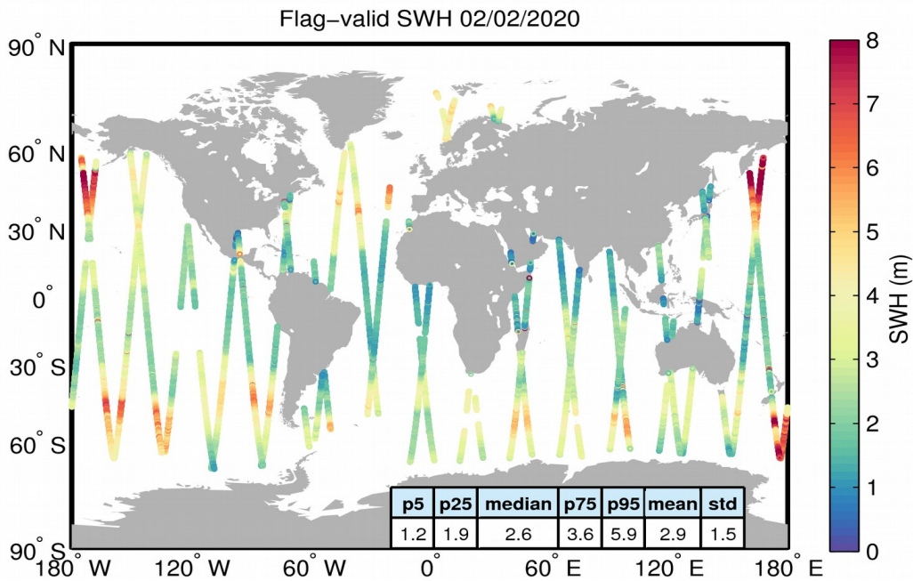
Figure 15. Geographical distribution of flag-valid SWH data over oceans and lakes for 02/02/2020. The statistical values shown in the table refer to the SWH in m and are calculated over all measurements shown in the figure.
