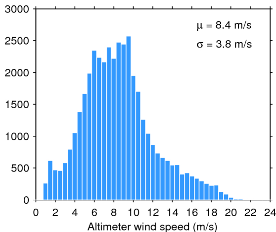
Figure 33. Histogram of flag-valid wind over oceans and lakes for 02/02/2020. The mean ( \mu ) and standard deviation ( \sigma ) are also shown. Note that values larger than 24 m/s are excluded from the histogram for the sake of readability but not from the computation of \mu and \sigma .
