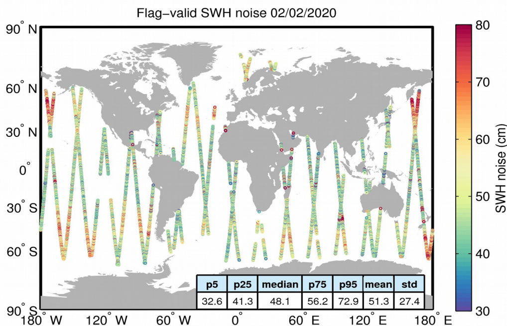
Figure 18. Geographical distribution of flag-valid 20-Hz SWH measurement noise over oceans and lakes for 02/02/2020. The statistical values shown in the figure refer to the SWH noise and are calculated over all measurements shown in the figure.
