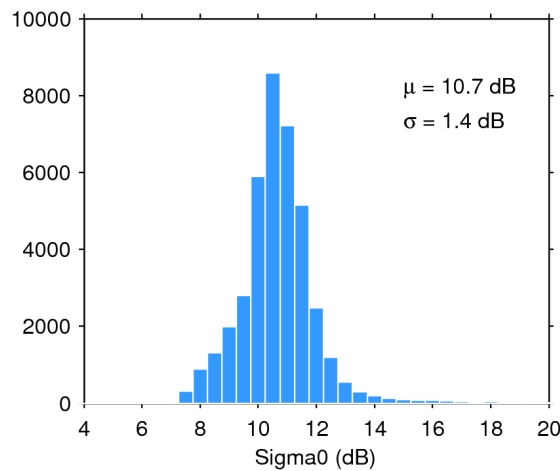
Figure 28. Histogram of science-valid sigma0 over oceans and lakes for 02/02/2020. The mean ( \mu ) and standard deviation ( \sigma ) are also shown. Note that values outside [4 20] dB are excluded from the histogram for the sake of readability but not from the computation of \mu and \sigma .
