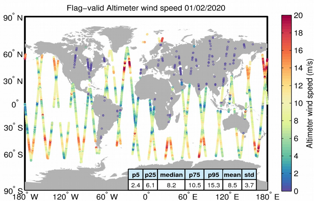
Figure 31. Geographical distribution of flag-valid wind data over oceans and lakes for 01/02/2020. The statistical values shown in the table refer to the wind in m/s and are calculated over all measurements shown in the figure.
