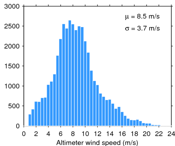
Figure 35. Histogram of science-valid wind over oceans and lakes for 01/02/2020. The mean ( \mu ) and standard deviation ( \sigma ) are also shown. Note that values larger than 24 m/s are excluded from the histogram for the sake of readability but not from the computation of \mu and \sigma .
