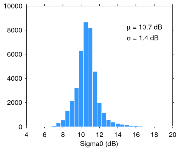
Figure 28. Histogram of science-valid sigma0 over oceans and lakes for 01/02/2020. The mean ( \mu ) and standard deviation ( \sigma ) are also shown. Note that values outside [4 20] dB are excluded from the histogram for the sake of readability but not from the computation of \mu and \sigma .
