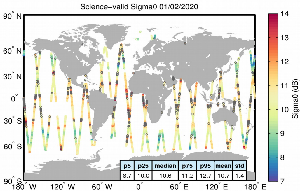
Figure 27. Geographical distribution of science-valid sigma0 data over oceans and lakes for 01/02/2020. The statistical values shown in the table refer to the sigma0 in dB and are calculated over all measurements shown in the figure. Gray circles denote records that have been rejected based on the editing criteria described in Table 4.
