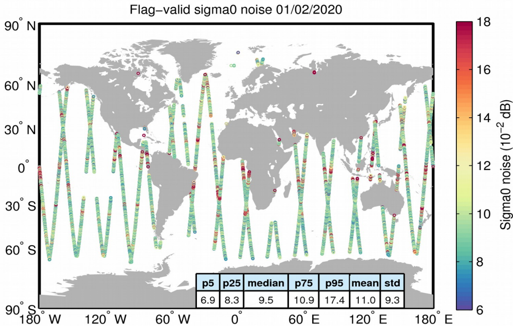
Figure 26. Geographical distribution of flag-valid 20-Hz sigma0 measurement noise over oceans and lakes for 01/02/2020. The statistical values shown in the table refer to the sigma0 noise and are calculated over all measurements shown in the figure.
