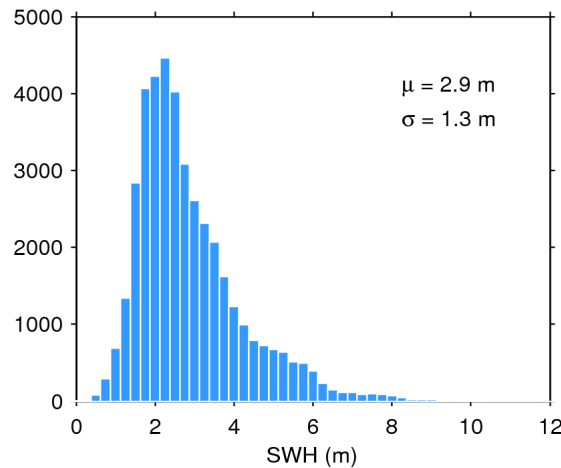
Figure 20. Histogram of science-valid SWH over oceans and lakes for 01/02/2020. The mean ( \mu ) and standard deviation ( \sigma ) are also shown. Note that values larger than 12 m are excluded from the histogram for the sake of readability but not from the computation of \mu and \sigma .
