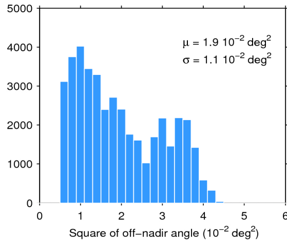
Figure 39. Histogram of flag-valid mispointing over oceans and lakes for 01/02/2020. The mean ( \mu ) and standard deviation ( \sigma ) are also shown. Note that values larger than 6 \cdot 10^{-2} \text{ deg}^2 are excluded from the histogram for the sake of readability but not from the computation of \mu and \sigma .
