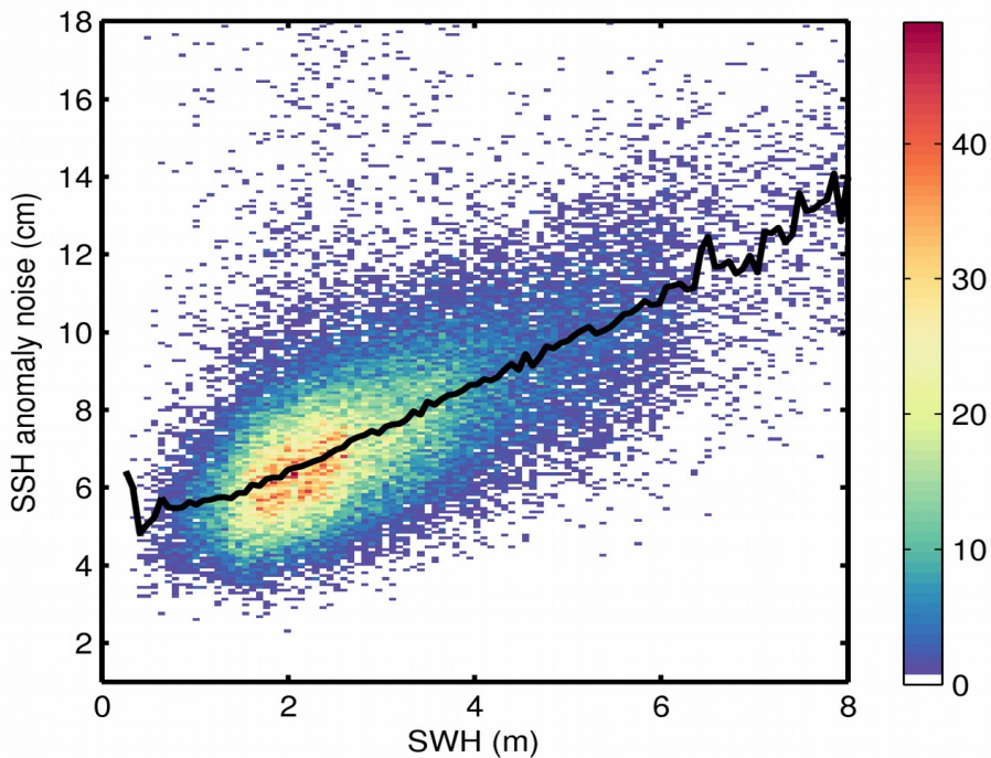
Figure 9. 2D histogram showing flag-valid SSH anomaly noise as a function of SWH for 01/02/2020. The black line denotes the median SSH anomaly noise as a function of SWH.
