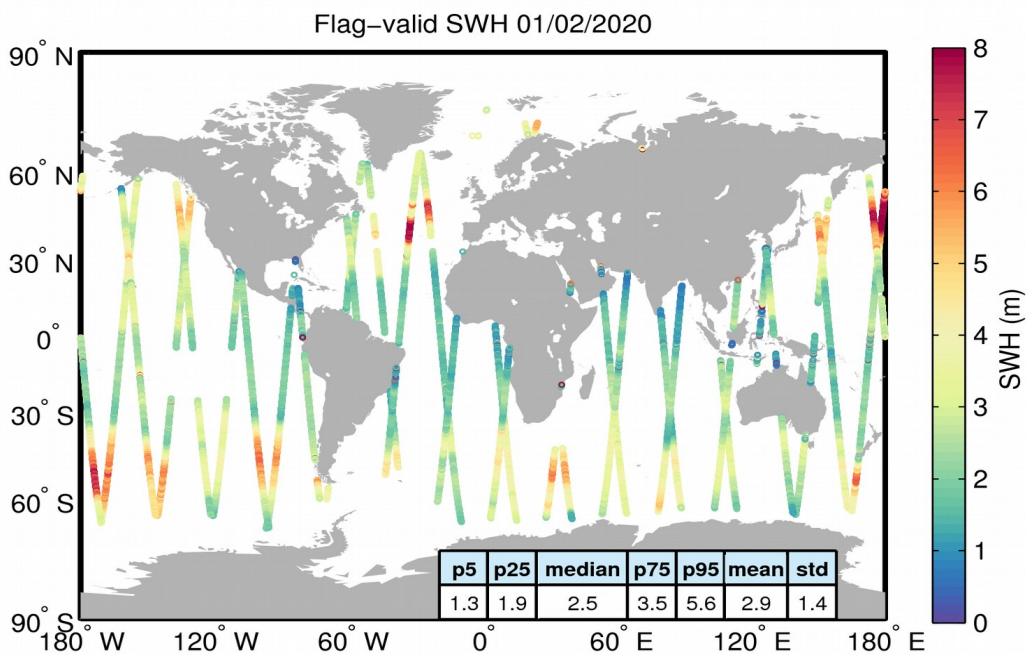
Figure 15. Geographical distribution of flag-valid SWH data over oceans and lakes for 01/02/2020. The statistical values shown in the table refer to the SWH in m and are calculated over all measurements shown in the figure.
