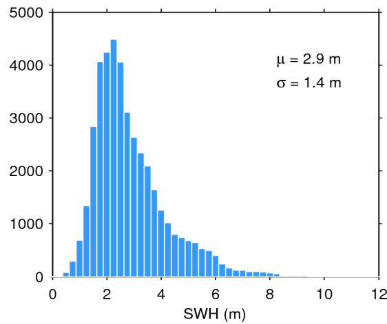
Figure 17. Histogram of flag-valid SWH over oceans and lakes for 01/02/2020. The mean ( \mu ) and standard deviation ( \sigma ) are also shown. Note that values larger than 12 m are excluded from the histogram for the sake of readability but not from the computation of \mu and \sigma .
