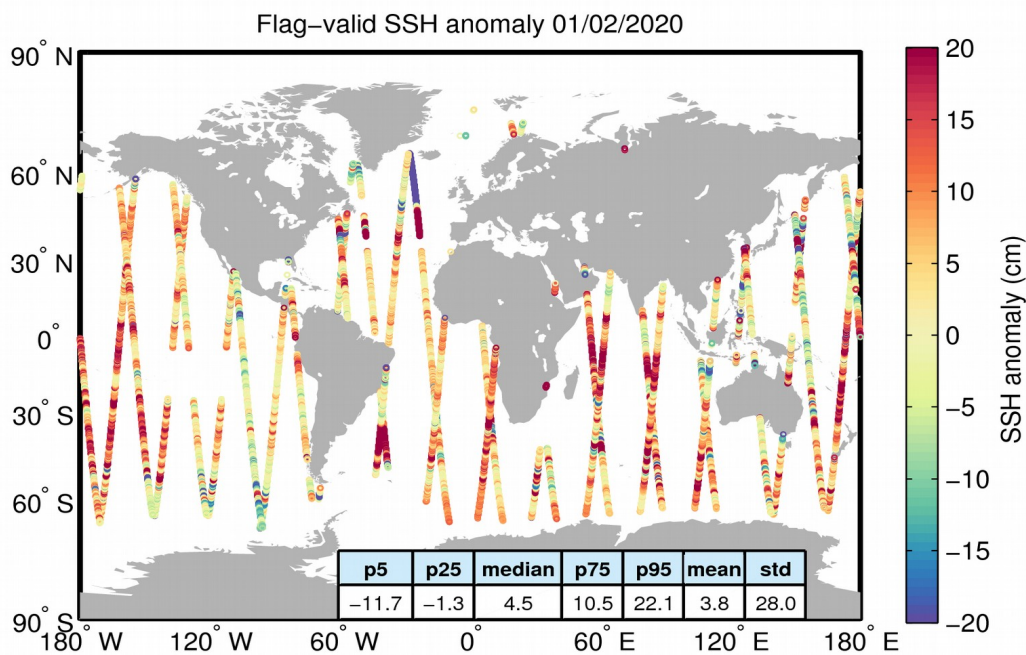
Figure 5. Geographical distribution of flag-valid 1-Hz SSH anomaly data over oceans and lakes for 01/02/2020. The statistical values shown in the table refer to the SSH anomaly in cm and are calculated over all measurements shown in the figure.
