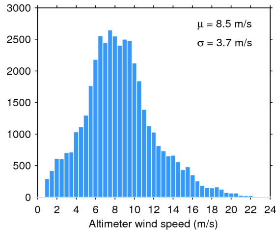
Figure 33. Histogram of flag-valid wind over oceans and lakes for 01/02/2020. The mean ( \mu ) and standard deviation ( \sigma ) are also shown. Note that values larger than 24 m/s are excluded from the histogram for the sake of readability but not from the computation of \mu and \sigma .
