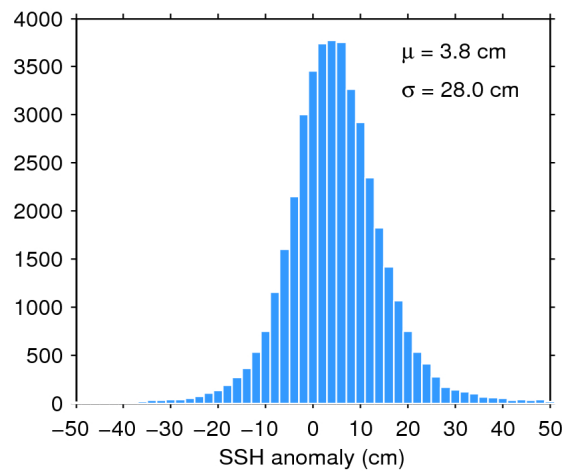
Figure 7. Histogram of flag-valid SSH anomaly over oceans and lakes for 01/02/2020. The mean ( \mu ) and standard deviation ( \sigma ) are also shown. Note that values outside [-50\ 50] cm are excluded from the histogram for the sake of readability but not from the computation of \mu and \sigma .
