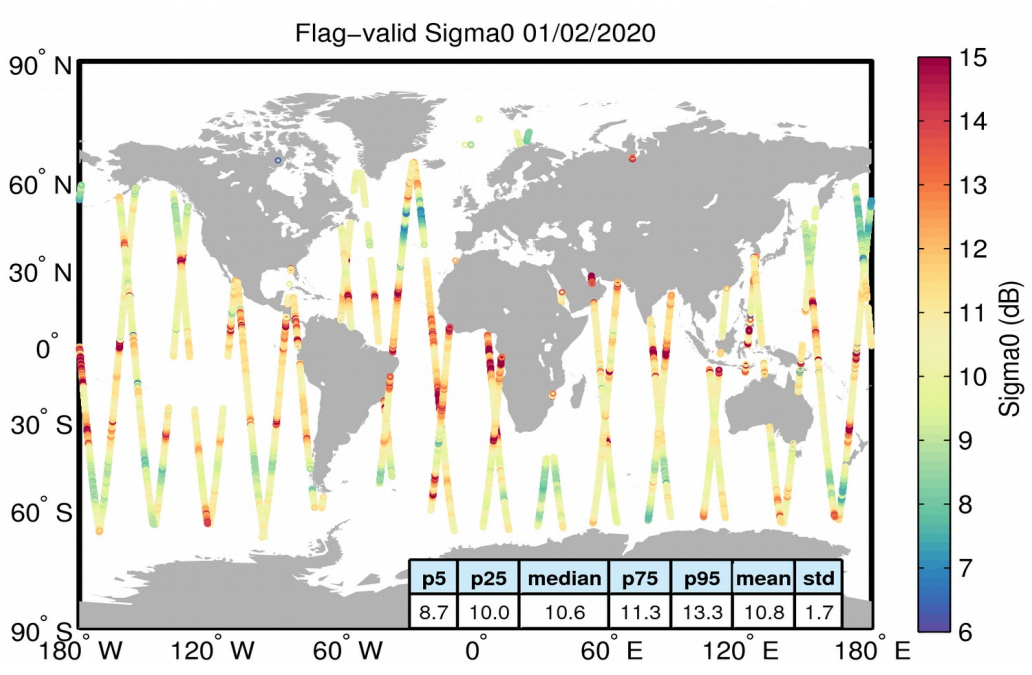
Figure 23. Geographical distribution of flag-valid sigma0 data over oceans and lakes for 01/02/2020. The statistical values shown in the table refer to the sigma0 in dB and are calculated over all measurements shown in the figure.
