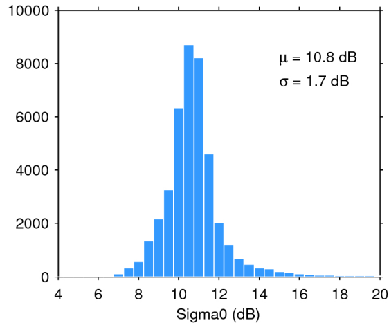
Figure 25. Histogram of flag-valid sigma0 over oceans and lakes for 01/02/2020. The mean ( \mu ) and standard deviation ( \sigma ) are also shown. Note that values outside [4 20] dB are excluded from the histogram for the sake of readability but not from the computation of \mu and \sigma .
