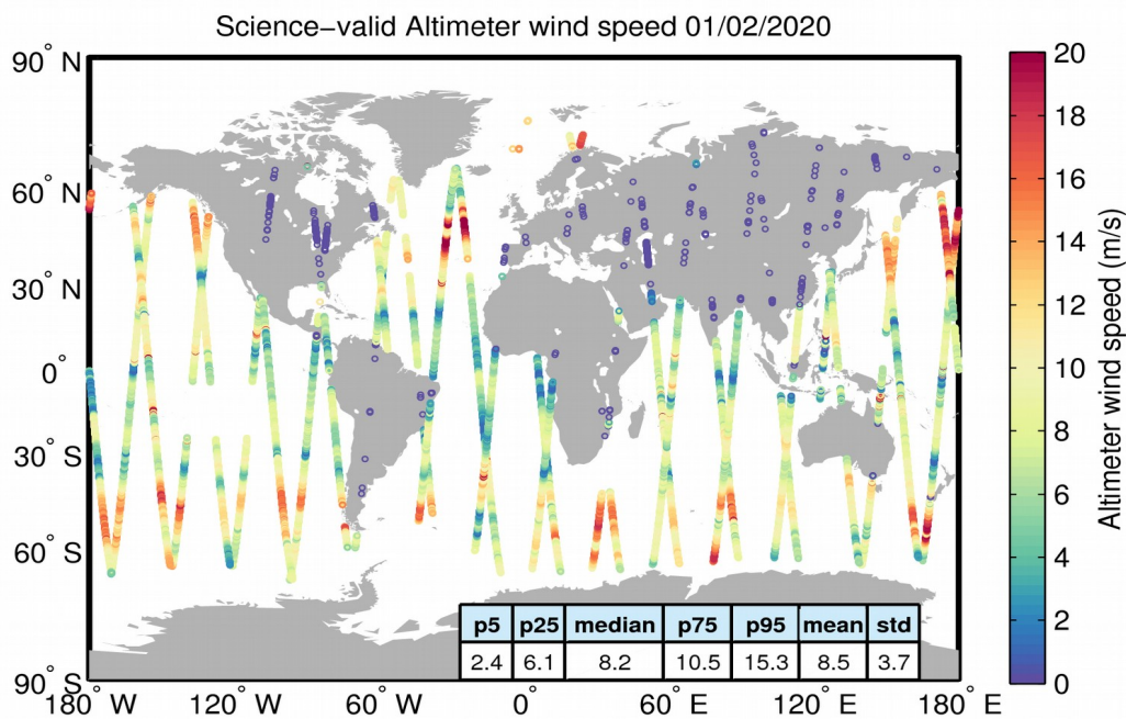
Figure 34. Geographical distribution of science-valid wind data over oceans and lakes for 01/02/2020. The statistical values shown in the table refer to the wind in m/s and are calculated over all measurements shown in the figure. Gray circles denote records that have been rejected based on the editing criteria described in Table 5.
