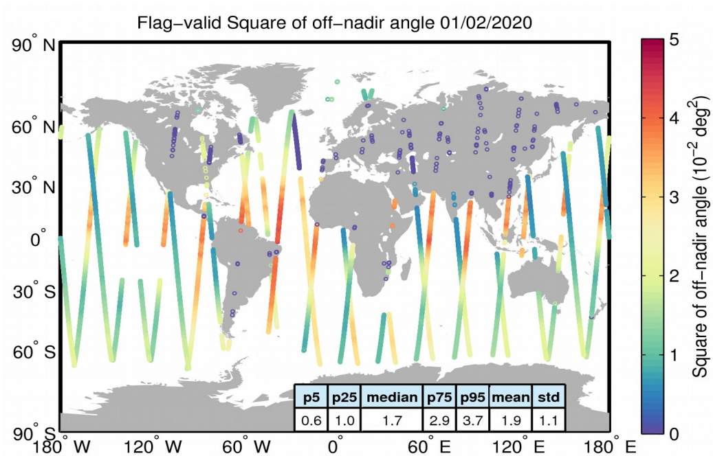
Figure 37. Geographical distribution of flag-valid mispointing data over oceans and lakes for 01/02/2020. The statistical values shown in the table refer to the mispointing in 10^{-2} \text{ deg}^2 and are calculated over all measurements shown in the figure.
