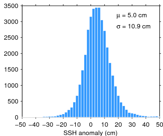
Figure 11. Histogram of science-valid SSH anomaly over oceans and lakes for 01/02/2020. The mean ( \mu ) and standard deviation ( \sigma ) are also shown. Note that values outside [-50 50] cm are excluded from the histogram for the sake of readability but not from the computation of \mu and \sigma .
