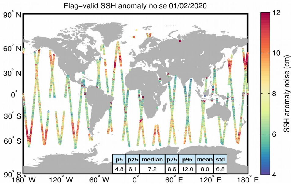
Figure 8. Geographical distribution of flag-valid 20-Hz SSH anomaly measurement noise over oceans and lakes for 01/02/2020. The statistical values shown in the table refer to the SSH anomaly noise and are calculated over all measurements shown in the figure.
