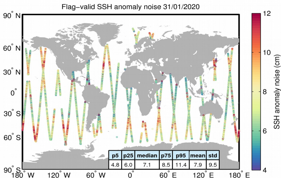
Figure 8. Geographical distribution of flag-valid 20-Hz SSH anomaly measurement noise over oceans and lakes for 31/01/2020. The statistical values shown in the table refer to the SSH anomaly noise and are calculated over all measurements shown in the figure.
