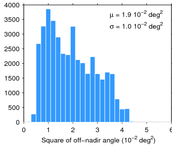
Figure 39. Histogram of flag-valid mispointing over oceans and lakes for 31/01/2020. The mean ( \mu ) and standard deviation ( \sigma ) are also shown. Note that values larger than 6 \cdot 10^{-2} \text{ deg}^2 are excluded from the histogram for the sake of readability but not from the computation of \mu and \sigma .
