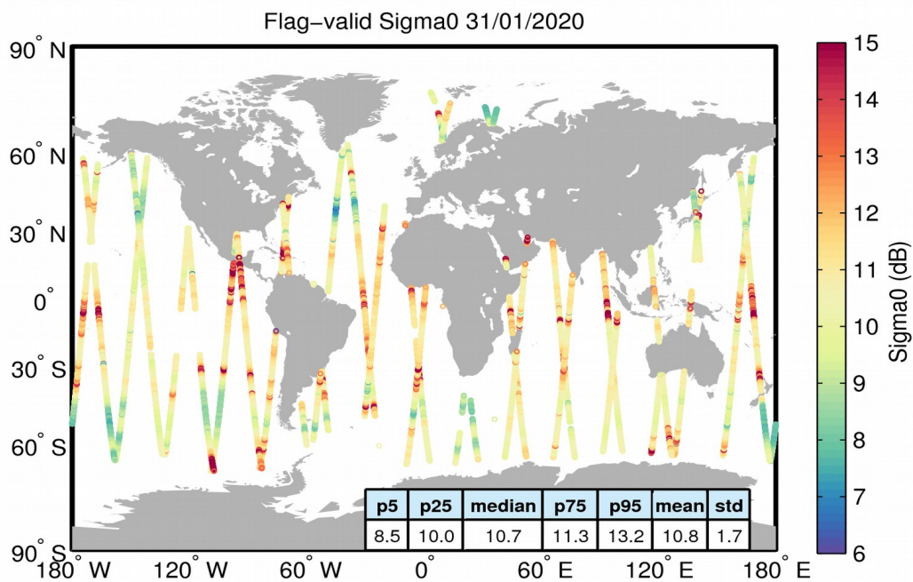
Figure 23. Geographical distribution of flag-valid sigma0 data over oceans and lakes for 31/01/2020. The statistical values shown in the table refer to the sigma0 in dB and are calculated over all measurements shown in the figure.
