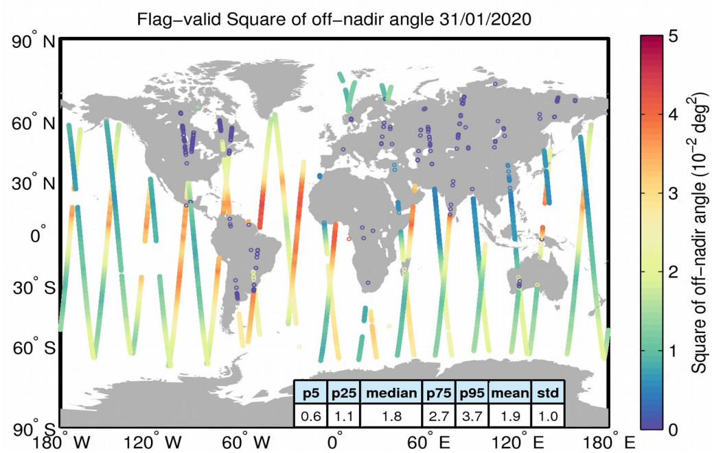
Figure 37. Geographical distribution of flag-valid mispointing data over oceans and lakes for 31/01/2020. The statistical values shown in the table refer to the mispointing in 10^{-2} \text{ deg}^2 and are calculated over all measurements shown in the figure.
