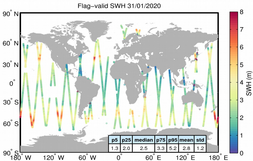
Figure 15. Geographical distribution of flag-valid SWH data over oceans and lakes for 31/01/2020. The statistical values shown in the table refer to the SWH in m and are calculated over all measurements shown in the figure.
