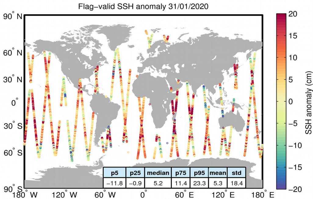
Figure 5. Geographical distribution of flag-valid 1-Hz SSH anomaly data over oceans and lakes for 31/01/2020. The statistical values shown in the table refer to the SSH anomaly in cm and are calculated over all measurements shown in the figure.
