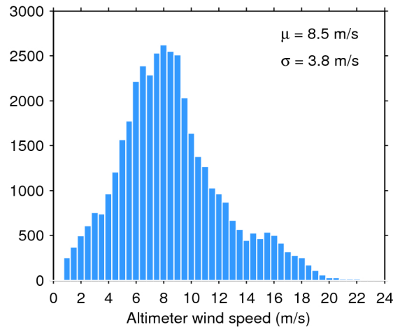
Figure 33. Histogram of flag-valid wind over oceans and lakes for 31/01/2020. The mean ( \mu ) and standard deviation ( \sigma ) are also shown. Note that values larger than 24 m/s are excluded from the histogram for the sake of readability but not from the computation of \mu and \sigma .
