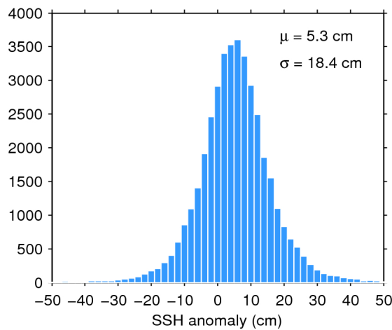
Figure 7. Histogram of flag-valid SSH anomaly over oceans and lakes for 31/01/2020. The mean ( \mu ) and standard deviation ( \sigma ) are also shown. Note that values outside [-50\ 50] cm are excluded from the histogram for the sake of readability but not from the computation of \mu and \sigma .
