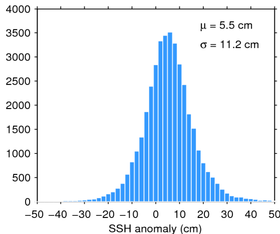
Figure 11. Histogram of science-valid SSH anomaly over oceans and lakes for 31/01/2020. The mean ( \mu ) and standard deviation ( \sigma ) are also shown. Note that values outside [-50 50] cm are excluded from the histogram for the sake of readability but not from the computation of \mu and \sigma .
