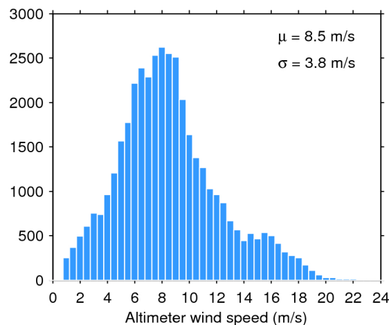
Figure 35. Histogram of science-valid wind over oceans and lakes for 31/01/2020. The mean ( \mu ) and standard deviation ( \sigma ) are also shown. Note that values larger than 24 m/s are excluded from the histogram for the sake of readability but not from the computation of \mu and \sigma .
