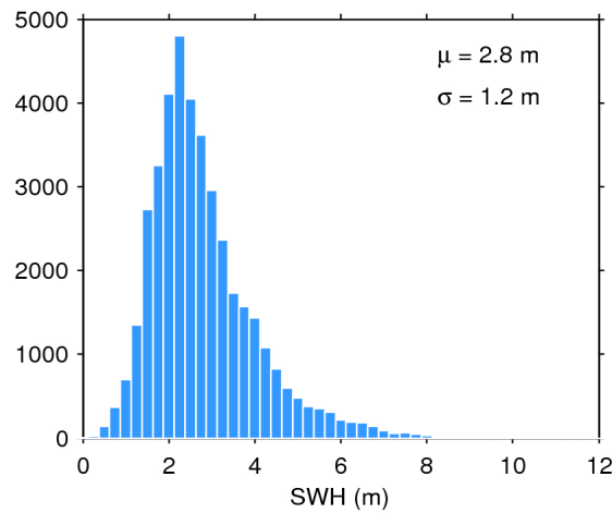
Figure 17. Histogram of flag-valid SWH over oceans and lakes for 31/01/2020. The mean ( \mu ) and standard deviation ( \sigma ) are also shown. Note that values larger than 12 m are excluded from the histogram for the sake of readability but not from the computation of \mu and \sigma .
