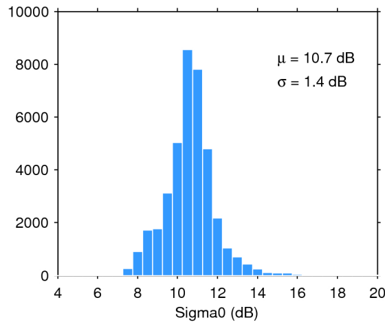
Figure 28. Histogram of science-valid sigma0 over oceans and lakes for 31/01/2020. The mean ( \mu ) and standard deviation ( \sigma ) are also shown. Note that values outside [4 20] dB are excluded from the histogram for the sake of readability but not from the computation of \mu and \sigma .
