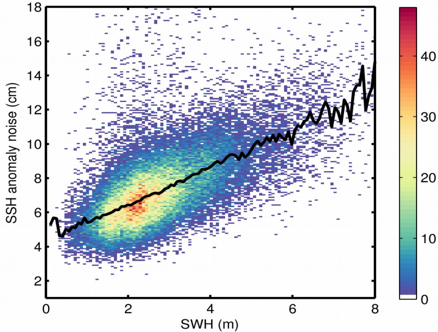
Figure 9. 2D histogram showing flag-valid SSH anomaly noise as a function of SWH for 31/01/2020. The black line denotes the median SSH anomaly noise as a function of SWH.
