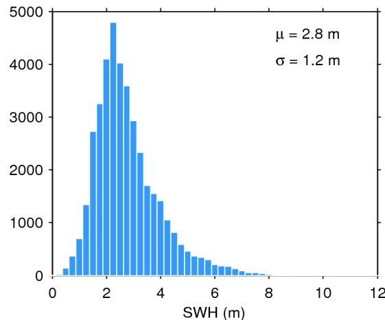
Figure 20. Histogram of science-valid SWH over oceans and lakes for 31/01/2020. The mean ( \mu ) and standard deviation ( \sigma ) are also shown. Note that values larger than 12 m are excluded from the histogram for the sake of readability but not from the computation of \mu and \sigma .
