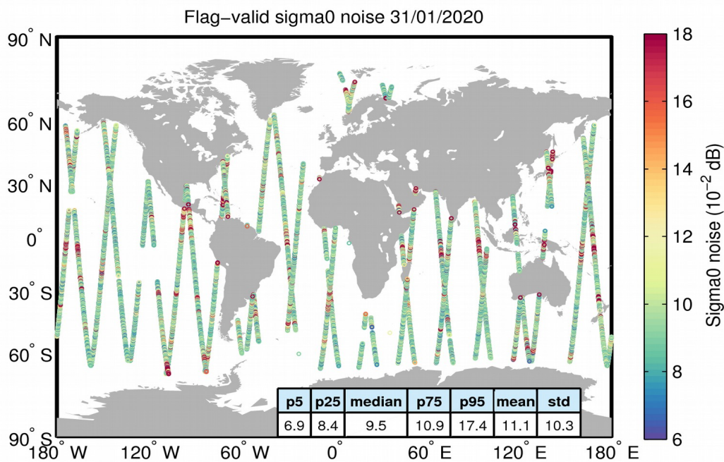
Figure 26. Geographical distribution of flag-valid 20-Hz sigma0 measurement noise over oceans and lakes for 31/01/2020. The statistical values shown in the table refer to the sigma0 noise and are calculated over all measurements shown in the figure.
