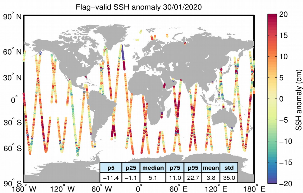
Figure 5. Geographical distribution of flag-valid 1-Hz SSH anomaly data over oceans and lakes for 30/01/2020. The statistical values shown in the table refer to the SSH anomaly in cm and are calculated over all measurements shown in the figure.
