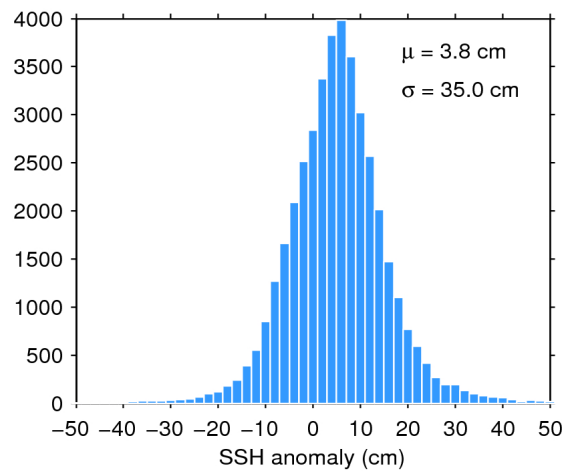
Figure 7. Histogram of flag-valid SSH anomaly over oceans and lakes for 30/01/2020. The mean ( \mu ) and standard deviation ( \sigma ) are also shown. Note that values outside [-50\ 50] cm are excluded from the histogram for the sake of readability but not from the computation of \mu and \sigma .
