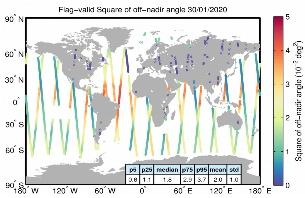
Figure 37. Geographical distribution of flag-valid mispointing data over oceans and lakes for 30/01/2020. The statistical values shown in the table refer to the mispointing in 10^{-2} deg 2 and are calculated over all measurements shown in the figure.
