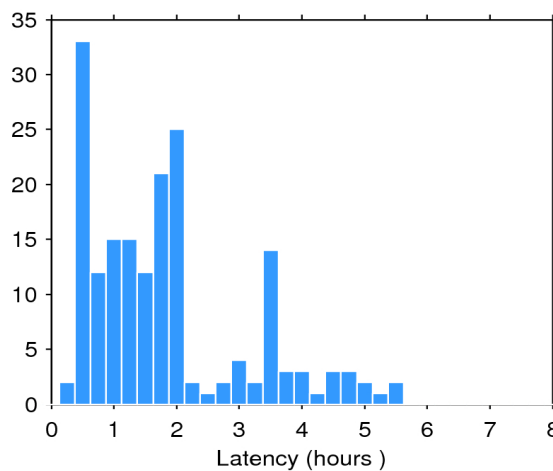
Figure 2. Histogram of the data latency for 30/01/2020. The y-axis denotes the number of files that are made available with a delay of x-hours with respect to the mean time of the records stored in the file.
