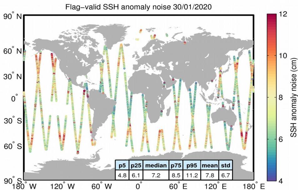
Figure 8. Geographical distribution of flag-valid 20-Hz SSH anomaly measurement noise over oceans and lakes for 30/01/2020. The statistical values shown in the table refer to the SSH anomaly noise and are calculated over all measurements shown in the figure.
