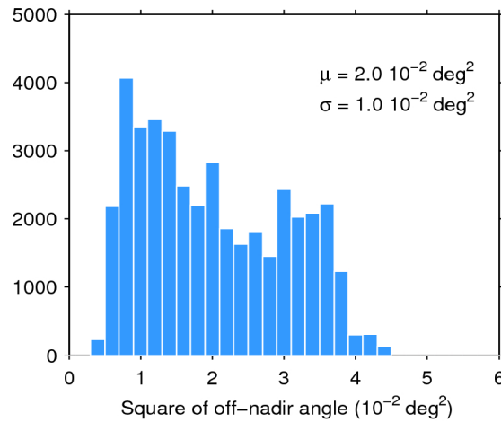
Figure 39. Histogram of flag-valid mispointing over oceans and lakes for 30/01/2020. The mean ( \mu ) and standard deviation ( \sigma ) are also shown. Note that values larger than 6 \cdot 10^{-2} \text{ deg}^2 are excluded from the histogram for the sake of readability but not from the computation of \mu and \sigma .
