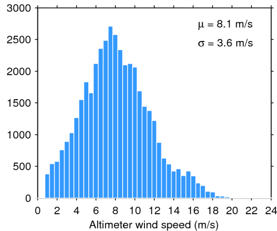
Figure 33. Histogram of flag-valid wind over oceans and lakes for 30/01/2020. The mean ( \mu ) and standard deviation ( \sigma ) are also shown. Note that values larger than 24 m/s are excluded from the histogram for the sake of readability but not from the computation of \mu and \sigma .
