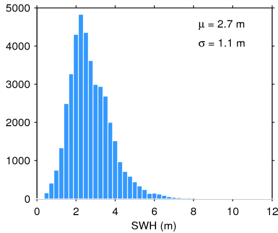
Figure 17. Histogram of flag-valid SWH over oceans and lakes for 30/01/2020. The mean ( \mu ) and standard deviation ( \sigma ) are also shown. Note that values larger than 12 m are excluded from the histogram for the sake of readability but not from the computation of \mu and \sigma .
