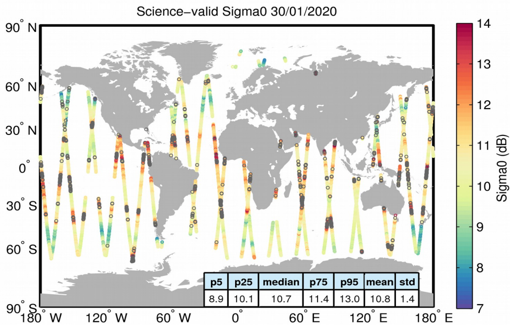
Figure 27. Geographical distribution of science-valid sigma0 data over oceans and lakes for 30/01/2020. The statistical values shown in the table refer to the sigma0 in dB and are calculated over all measurements shown in the figure. Gray circles denote records that have been rejected based on the editing criteria described in Table 4.
