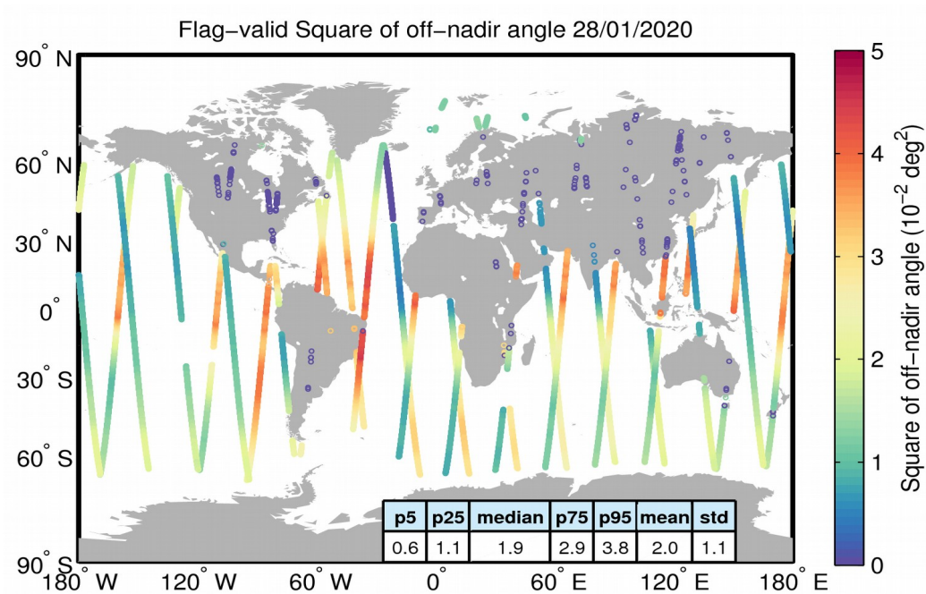
Figure 37. Geographical distribution of flag-valid mispointing data over oceans and lakes for 28/01/2020. The statistical values shown in the table refer to the mispointing in 10^{-2} deg 2 and are calculated over all measurements shown in the figure.
