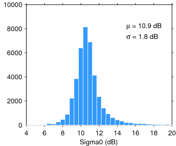
Figure 25. Histogram of flag-valid sigma0 over oceans and lakes for 28/01/2020. The mean ( \mu ) and standard deviation ( \sigma ) are also shown. Note that values outside [4 20] dB are excluded from the histogram for the sake of readability but not from the computation of \mu and \sigma .
