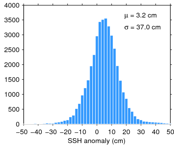
Figure 7. Histogram of flag-valid SSH anomaly over oceans and lakes for 28/01/2020. The mean ( \mu ) and standard deviation ( \sigma ) are also shown. Note that values outside [-50 50] cm are excluded from the histogram for the sake of readability but not from the computation of \mu and \sigma .
