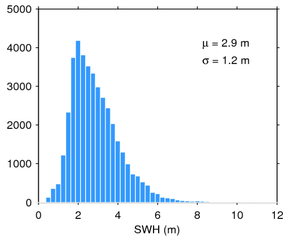
Figure 17. Histogram of flag-valid SWH over oceans and lakes for 28/01/2020. The mean ( \mu ) and standard deviation ( \sigma ) are also shown. Note that values larger than 12 m are excluded from the histogram for the sake of readability but not from the computation of \mu and \sigma .
