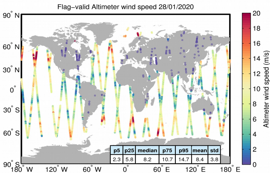
Figure 31. Geographical distribution of flag-valid wind data over oceans and lakes for 28/01/2020. The statistical values shown in the table refer to the wind in m/s and are calculated over all measurements shown in the figure.
