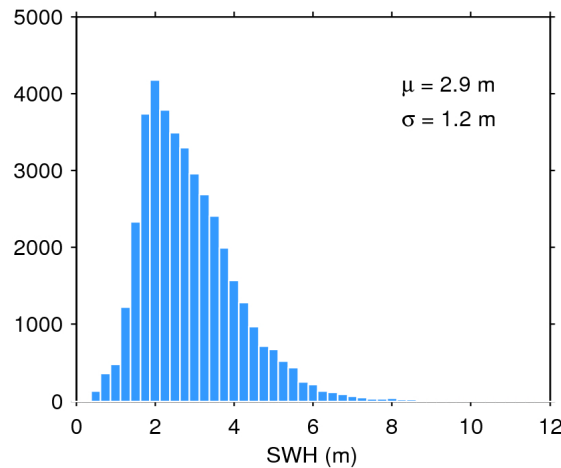
Figure 20. Histogram of science-valid SWH over oceans and lakes for 28/01/2020. The mean ( \mu ) and standard deviation ( \sigma ) are also shown. Note that values larger than 12 m are excluded from the histogram for the sake of readability but not from the computation of \mu and \sigma .
