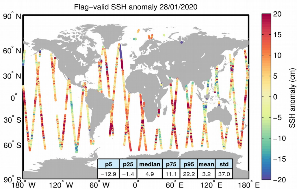
Figure 5. Geographical distribution of flag-valid 1-Hz SSH anomaly data over oceans and lakes for 28/01/2020. The statistical values shown in the table refer to the SSH anomaly in cm and are calculated over all measurements shown in the figure.
