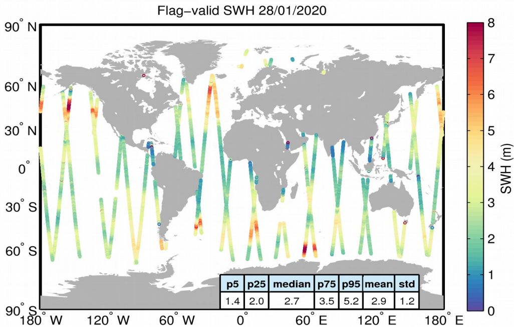
Figure 15. Geographical distribution of flag-valid SWH data over oceans and lakes for 28/01/2020. The statistical values shown in the table refer to the SWH in m and are calculated over all measurements shown in the figure.
