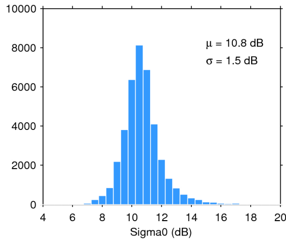
Figure 28. Histogram of science-valid sigma0 over oceans and lakes for 28/01/2020. The mean ( \mu ) and standard deviation ( \sigma ) are also shown. Note that values outside [4 20] dB are excluded from the histogram for the sake of readability but not from the computation of \mu and \sigma .
