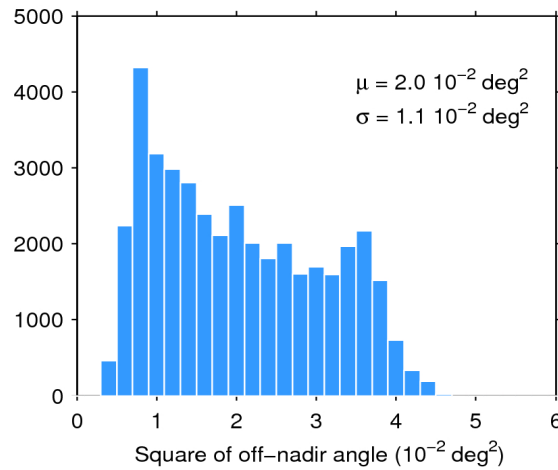
Figure 39. Histogram of flag-valid mispointing over oceans and lakes for 28/01/2020. The mean ( \mu ) and standard deviation ( \sigma ) are also shown. Note that values larger than 6 \cdot 10^{-2} \text{ deg}^2 are excluded from the histogram for the sake of readability but not from the computation of \mu and \sigma .
