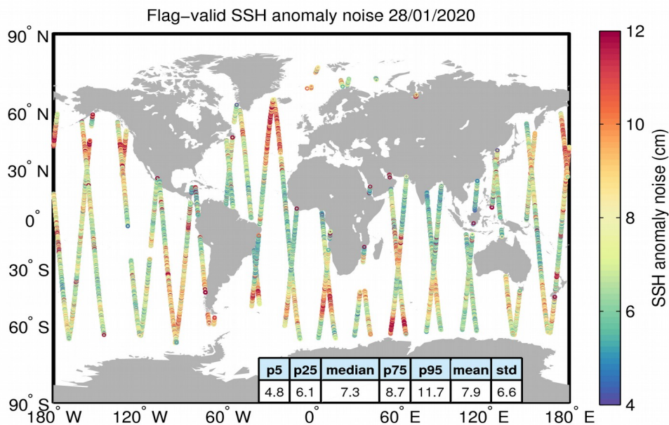
Figure 8. Geographical distribution of flag-valid 20-Hz SSH anomaly measurement noise over oceans and lakes for 28/01/2020. The statistical values shown in the table refer to the SSH anomaly noise and are calculated over all measurements shown in the figure.
