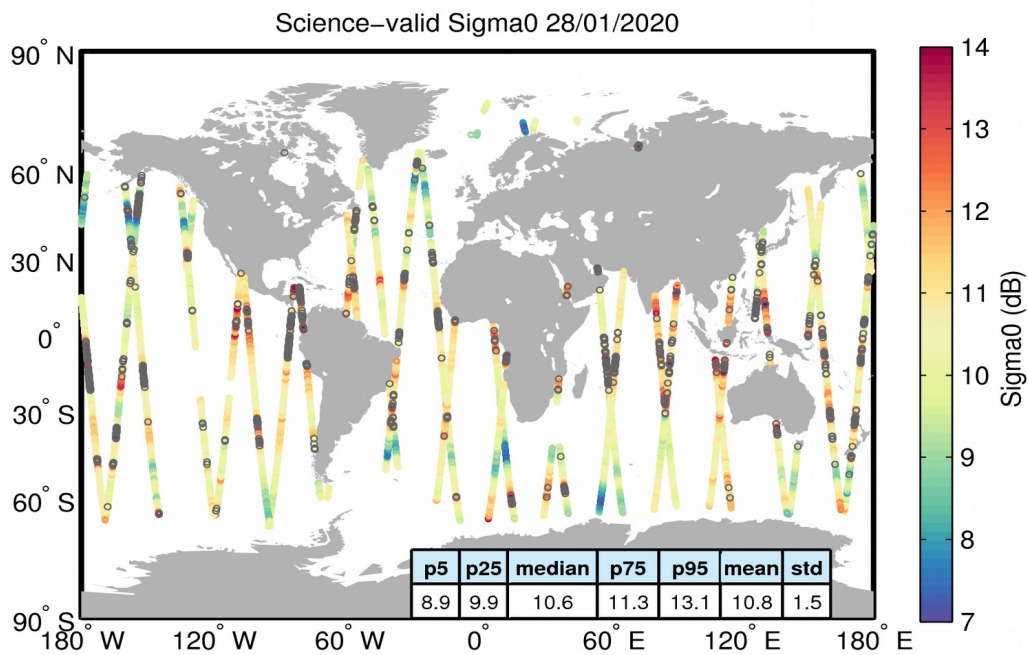
Figure 27. Geographical distribution of science-valid sigma0 data over oceans and lakes for 28/01/2020. The statistical values shown in the table refer to the sigma0 in dB and are calculated over all measurements shown in the figure. Gray circles denote records that have been rejected based on the editing criteria described in Table 4.
