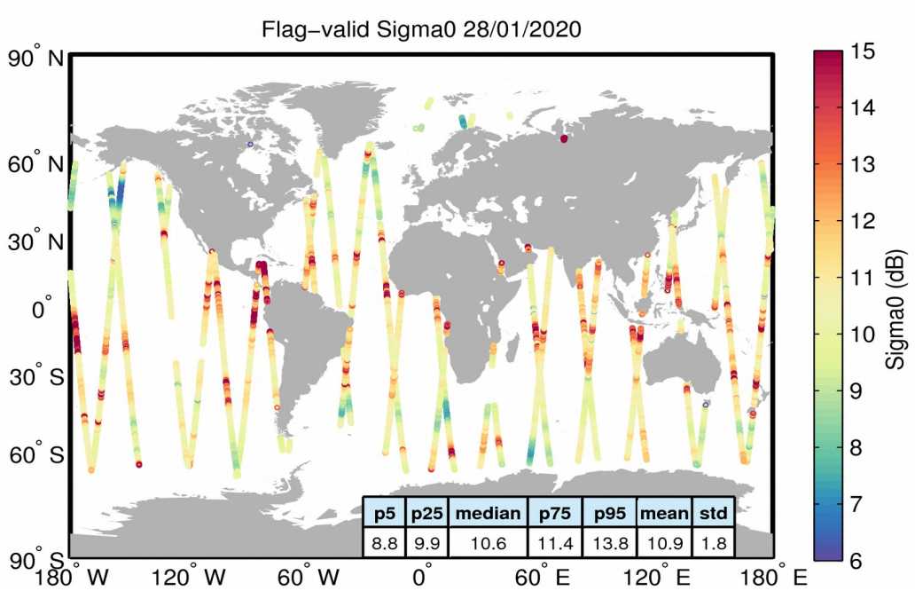
Figure 23. Geographical distribution of flag-valid sigma0 data over oceans and lakes for 28/01/2020. The statistical values shown in the table refer to the sigma0 in dB and are calculated over all measurements shown in the figure.
