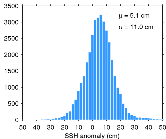
Figure 11. Histogram of science-valid SSH anomaly over oceans and lakes for 28/01/2020. The mean ( \mu ) and standard deviation ( \sigma ) are also shown. Note that values outside [-50 50] cm are excluded from the histogram for the sake of readability but not from the computation of \mu and \sigma .
