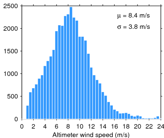
Figure 35. Histogram of science-valid wind over oceans and lakes for 28/01/2020. The mean ( \mu ) and standard deviation ( \sigma ) are also shown. Note that values larger than 24 m/s are excluded from the histogram for the sake of readability but not from the computation of \mu and \sigma .
