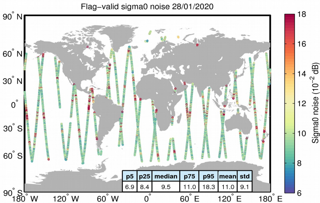
Figure 26. Geographical distribution of flag-valid 20-Hz sigma0 measurement noise over oceans and lakes for 28/01/2020. The statistical values shown in the table refer to the sigma0 noise and are calculated over all measurements shown in the figure.
