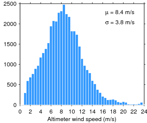
Figure 33. Histogram of flag-valid wind over oceans and lakes for 28/01/2020. The mean ( \mu ) and standard deviation ( \sigma ) are also shown. Note that values larger than 24 m/s are excluded from the histogram for the sake of readability but not from the computation of \mu and \sigma .
