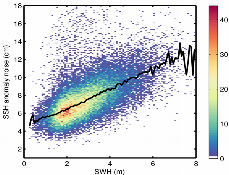
Figure 9. 2D histogram showing flag-valid SSH anomaly noise as a function of SWH for 28/01/2020. The black line denotes the median SSH anomaly noise as a function of SWH.
