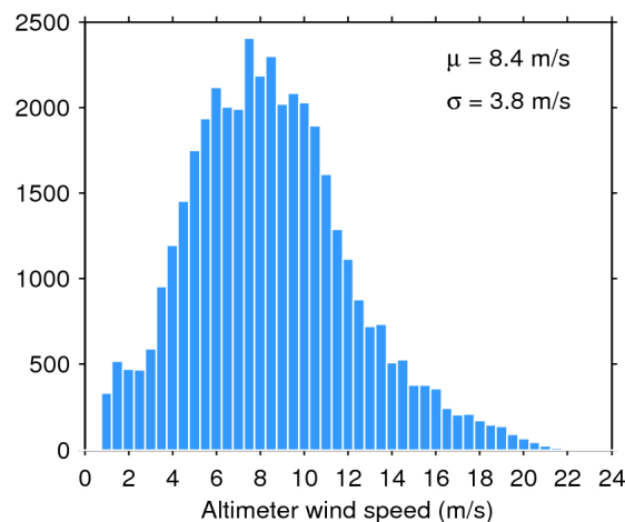
Figure 35. Histogram of science-valid wind over oceans and lakes for 27/01/2020. The mean ( \mu ) and standard deviation ( \sigma ) are also shown. Note that values larger than 24 m/s are excluded from the histogram for the sake of readability but not from the computation of \mu and \sigma .
