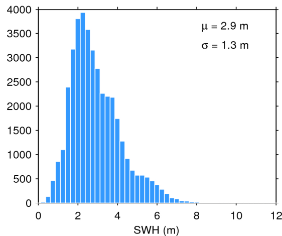
Figure 20. Histogram of science-valid SWH over oceans and lakes for 27/01/2020. The mean ( \mu ) and standard deviation ( \sigma ) are also shown. Note that values larger than 12 m are excluded from the histogram for the sake of readability but not from the computation of \mu and \sigma .
