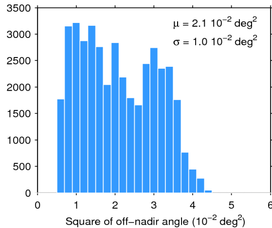
Figure 39. Histogram of flag-valid mispointing over oceans and lakes for 27/01/2020. The mean ( \mu ) and standard deviation ( \sigma ) are also shown. Note that values larger than 6 \cdot 10^{-2} \text{ deg}^2 are excluded from the histogram for the sake of readability but not from the computation of \mu and \sigma .
