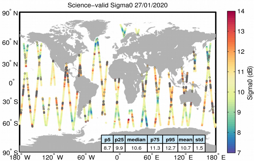
Figure 27. Geographical distribution of science-valid sigma0 data over oceans and lakes for 27/01/2020. The statistical values shown in the table refer to the sigma0 in dB and are calculated over all measurements shown in the figure. Gray circles denote records that have been rejected based on the editing criteria described in Table 4.
