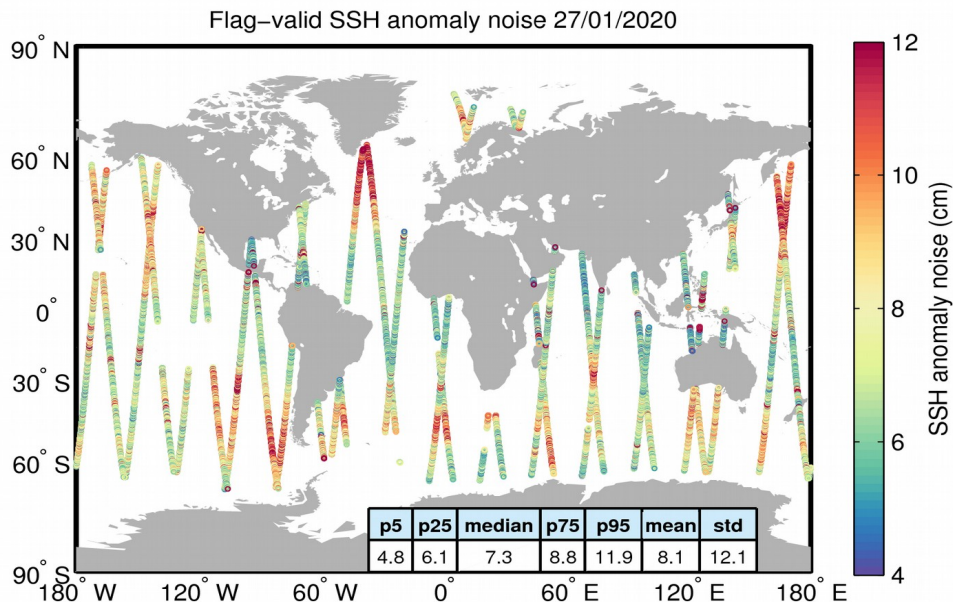
Figure 8. Geographical distribution of flag-valid 20-Hz SSH anomaly measurement noise over oceans and lakes for 27/01/2020. The statistical values shown in the table refer to the SSH anomaly noise and are calculated over all measurements shown in the figure.
