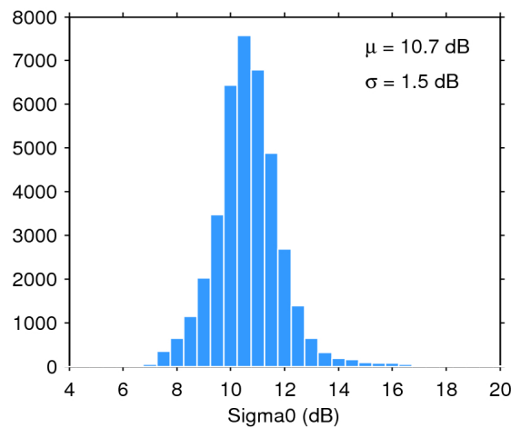
Figure 28. Histogram of science-valid sigma0 over oceans and lakes for 27/01/2020. The mean ( \mu ) and standard deviation ( \sigma ) are also shown. Note that values outside [4 20] dB are excluded from the histogram for the sake of readability but not from the computation of \mu and \sigma .
