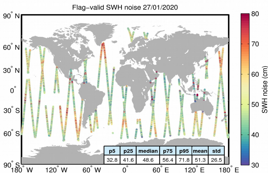
Figure 18. Geographical distribution of flag-valid 20-Hz SWH measurement noise over oceans and lakes for 27/01/2020. The statistical values shown in the figure refer to the SWH noise and are calculated over all measurements shown in the figure.
