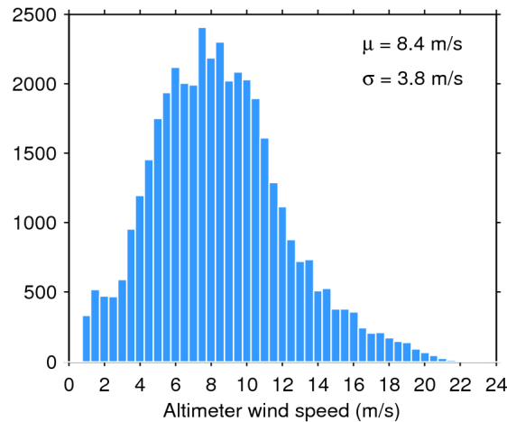
Figure 33. Histogram of flag-valid wind over oceans and lakes for 27/01/2020. The mean ( \mu ) and standard deviation ( \sigma ) are also shown. Note that values larger than 24 m/s are excluded from the histogram for the sake of readability but not from the computation of \mu and \sigma .
