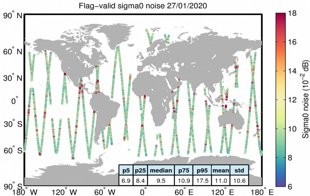
Figure 26. Geographical distribution of flag-valid 20-Hz sigma0 measurement noise over oceans and lakes for 27/01/2020. The statistical values shown in the table refer to the sigma0 noise and are calculated over all measurements shown in the figure.
