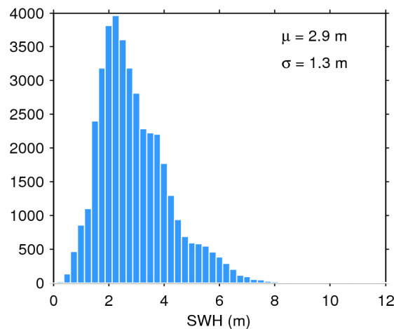
Figure 17. Histogram of flag-valid SWH over oceans and lakes for 27/01/2020. The mean ( \mu ) and standard deviation ( \sigma ) are also shown. Note that values larger than 12 m are excluded from the histogram for the sake of readability but not from the computation of \mu and \sigma .
