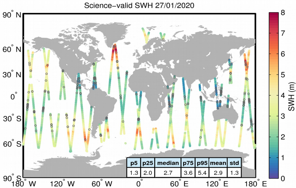
Figure 19. Geographical distribution of science-valid SWH data over oceans and lakes for 27/01/2020. The statistical values shown in the table refer to the SWH in m and are calculated over all measurements shown in the figure. Gray circles denote records that have been rejected based on the editing criteria described in Table 3.
