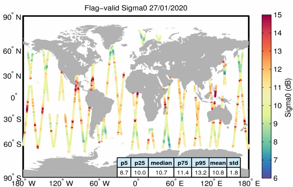
Figure 23. Geographical distribution of flag-valid sigma0 data over oceans and lakes for 27/01/2020. The statistical values shown in the table refer to the sigma0 in dB and are calculated over all measurements shown in the figure.
