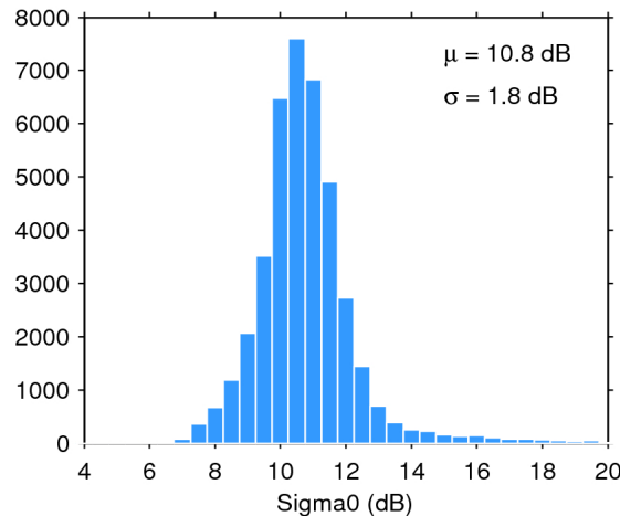
Figure 25. Histogram of flag-valid sigma0 over oceans and lakes for 27/01/2020. The mean ( \mu ) and standard deviation ( \sigma ) are also shown. Note that values outside [4 20] dB are excluded from the histogram for the sake of readability but not from the computation of \mu and \sigma .
