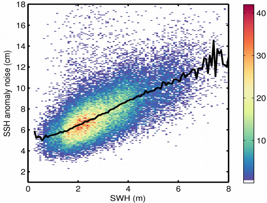
Figure 9. 2D histogram showing flag-valid SSH anomaly noise as a function of SWH for 27/01/2020. The black line denotes the median SSH anomaly noise as a function of SWH.
