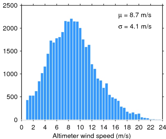
Figure 33. Histogram of flag-valid wind over oceans and lakes for 26/01/2020. The mean ( \mu ) and standard deviation ( \sigma ) are also shown. Note that values larger than 24 m/s are excluded from the histogram for the sake of readability but not from the computation of \mu and \sigma .
