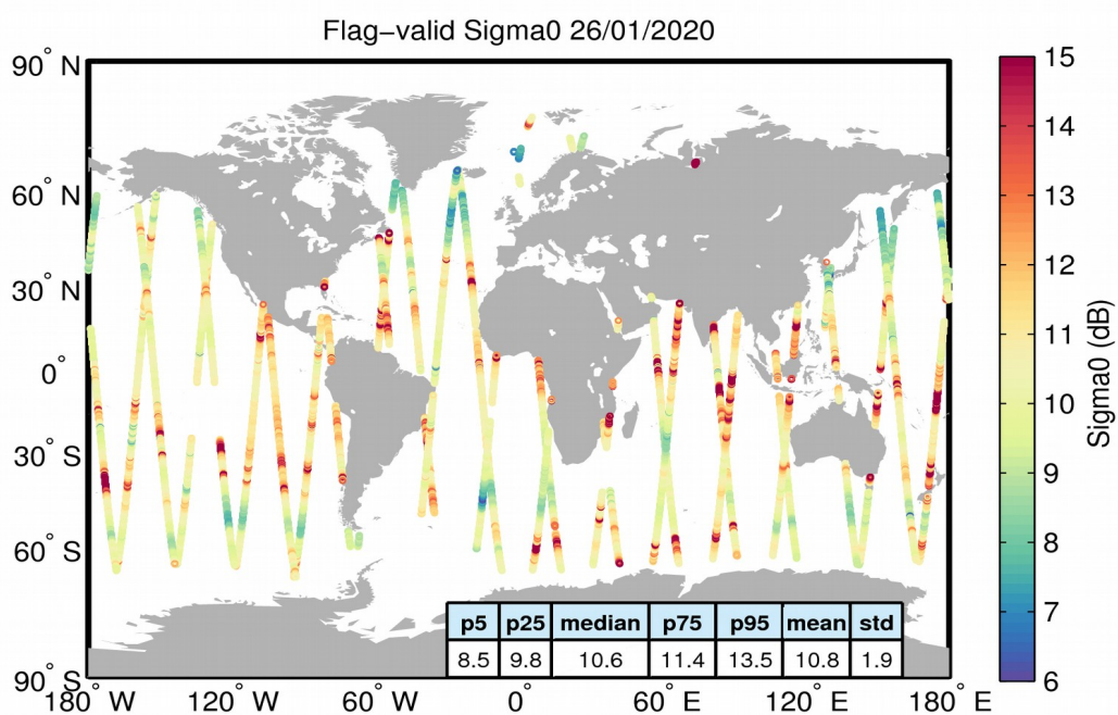
Figure 23. Geographical distribution of flag-valid sigma0 data over oceans and lakes for 26/01/2020. The statistical values shown in the table refer to the sigma0 in dB and are calculated over all measurements shown in the figure.
