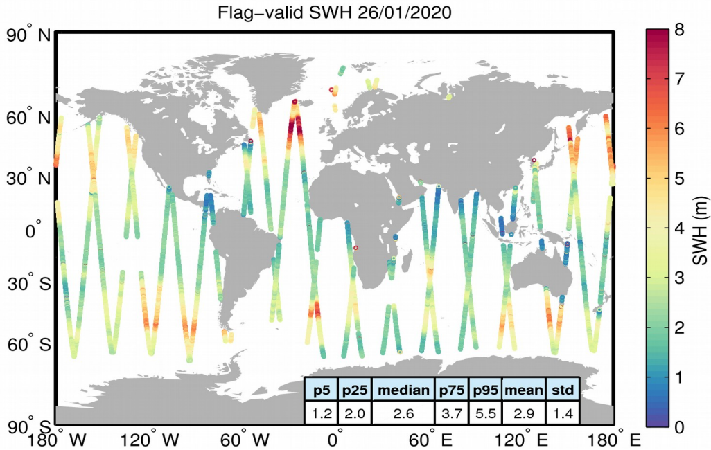
Figure 15. Geographical distribution of flag-valid SWH data over oceans and lakes for 26/01/2020. The statistical values shown in the table refer to the SWH in m and are calculated over all measurements shown in the figure.
