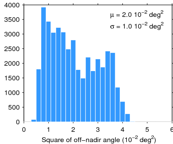
Figure 39. Histogram of flag-valid mispointing over oceans and lakes for 26/01/2020. The mean ( \mu ) and standard deviation ( \sigma ) are also shown. Note that values larger than 6 \cdot 10^{-2} \text{ deg}^2 are excluded from the histogram for the sake of readability but not from the computation of \mu and \sigma .
