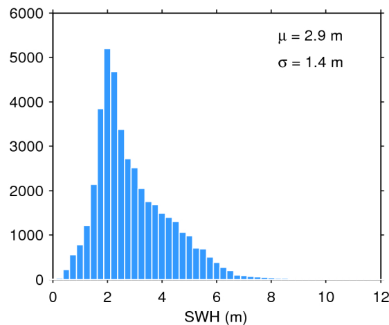
Figure 17. Histogram of flag-valid SWH over oceans and lakes for 26/01/2020. The mean ( \mu ) and standard deviation ( \sigma ) are also shown. Note that values larger than 12 m are excluded from the histogram for the sake of readability but not from the computation of \mu and \sigma .
