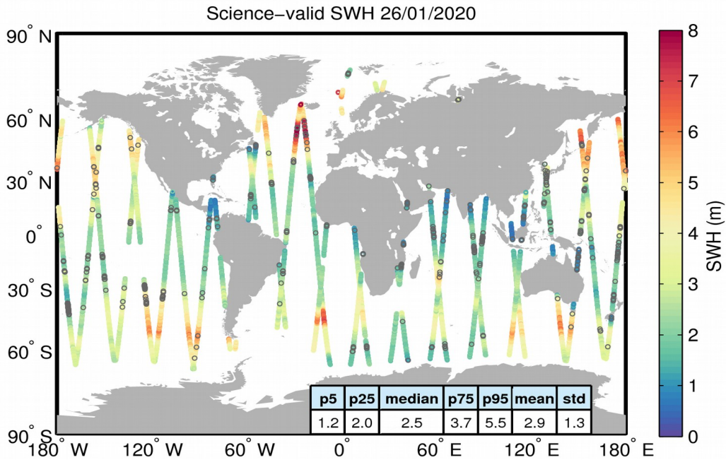
Figure 19. Geographical distribution of science-valid SWH data over oceans and lakes for 26/01/2020. The statistical values shown in the table refer to the SWH in m and are calculated over all measurements shown in the figure. Gray circles denote records that have been rejected based on the editing criteria described in Table 3.
