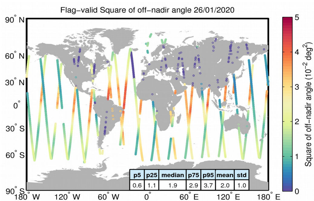
Figure 37. Geographical distribution of flag-valid mispointing data over oceans and lakes for 26/01/2020. The statistical values shown in the table refer to the mispointing in 10^{-2} \text{ deg}^2 and are calculated over all measurements shown in the figure.
