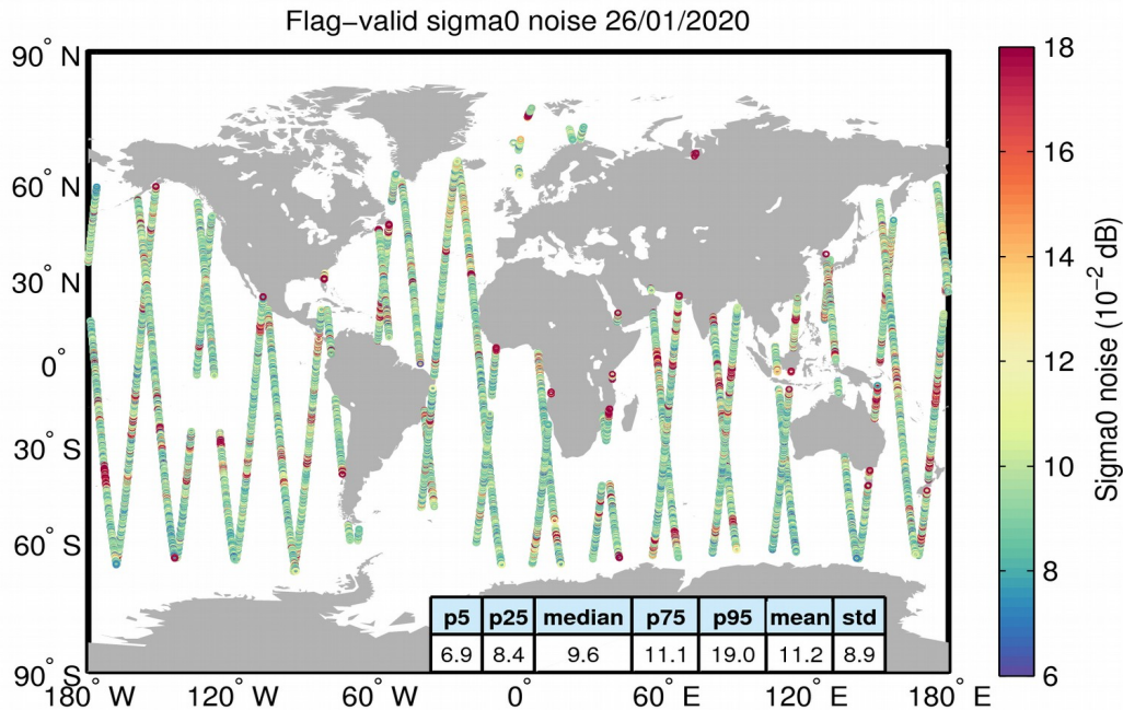
Figure 26. Geographical distribution of flag-valid 20-Hz sigma0 measurement noise over oceans and lakes for 26/01/2020. The statistical values shown in the table refer to the sigma0 noise and are calculated over all measurements shown in the figure.
