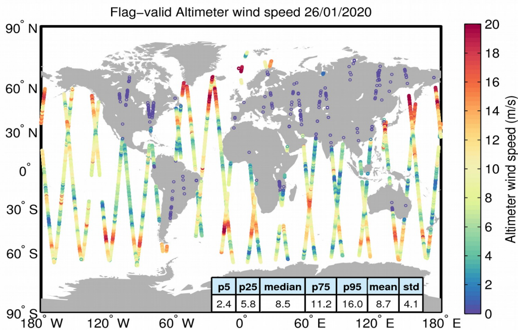
Figure 31. Geographical distribution of flag-valid wind data over oceans and lakes for 26/01/2020. The statistical values shown in the table refer to the wind in m/s and are calculated over all measurements shown in the figure.
