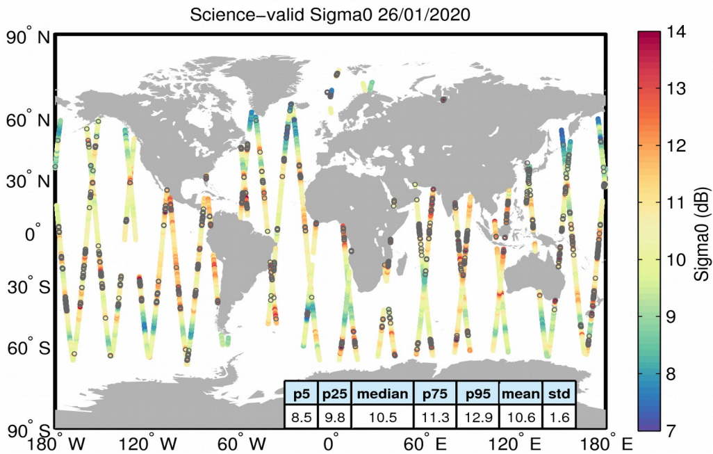
Figure 27. Geographical distribution of science-valid sigma0 data over oceans and lakes for 26/01/2020. The statistical values shown in the table refer to the sigma0 in dB and are calculated over all measurements shown in the figure. Gray circles denote records that have been rejected based on the editing criteria described in Table 4.
