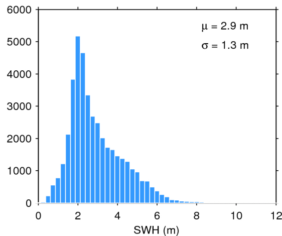
Figure 20. Histogram of science-valid SWH over oceans and lakes for 26/01/2020. The mean ( \mu ) and standard deviation ( \sigma ) are also shown. Note that values larger than 12 m are excluded from the histogram for the sake of readability but not from the computation of \mu and \sigma .
