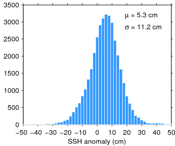
Figure 11. Histogram of science-valid SSH anomaly over oceans and lakes for 26/01/2020. The mean ( \mu ) and standard deviation ( \sigma ) are also shown. Note that values outside [-50 50] cm are excluded from the histogram for the sake of readability but not from the computation of \mu and \sigma .
