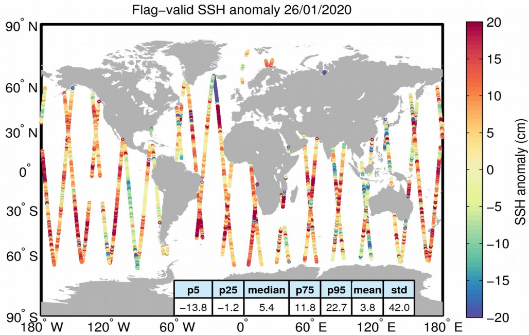
Figure 5. Geographical distribution of flag-valid 1-Hz SSH anomaly data over oceans and lakes for 26/01/2020. The statistical values shown in the table refer to the SSH anomaly in cm and are calculated over all measurements shown in the figure.
