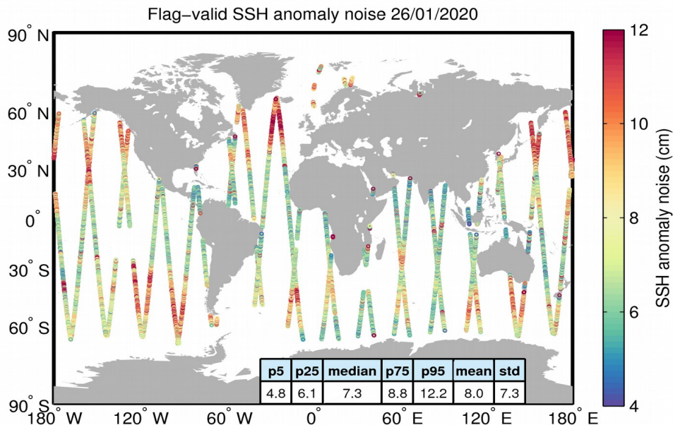
Figure 8. Geographical distribution of flag-valid 20-Hz SSH anomaly measurement noise over oceans and lakes for 26/01/2020. The statistical values shown in the table refer to the SSH anomaly noise and are calculated over all measurements shown in the figure.
