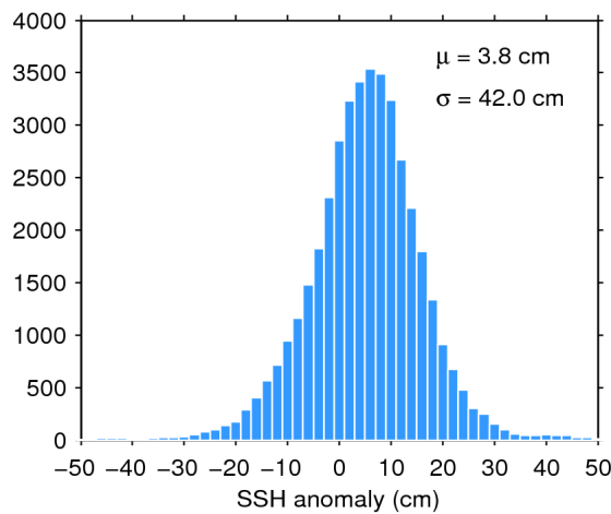
Figure 7. Histogram of flag-valid SSH anomaly over oceans and lakes for 26/01/2020. The mean ( \mu ) and standard deviation ( \sigma ) are also shown. Note that values outside [-50 50] cm are excluded from the histogram for the sake of readability but not from the computation of \mu and \sigma .
