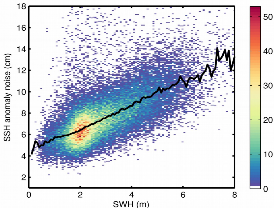
Figure 9. 2D histogram showing flag-valid SSH anomaly noise as a function of SWH for 26/01/2020. The black line denotes the median SSH anomaly noise as a function of SWH.
