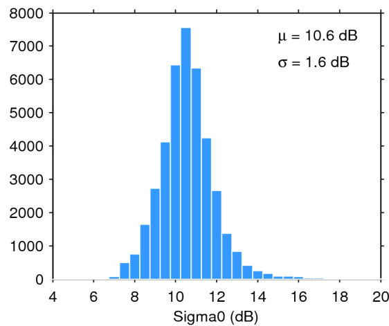
Figure 28. Histogram of science-valid sigma0 over oceans and lakes for 26/01/2020. The mean ( \mu ) and standard deviation ( \sigma ) are also shown. Note that values outside [4 20] dB are excluded from the histogram for the sake of readability but not from the computation of \mu and \sigma .
