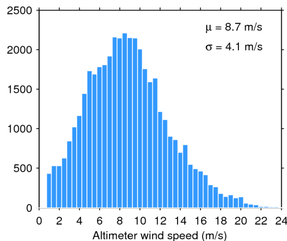
Figure 35. Histogram of science-valid wind over oceans and lakes for 26/01/2020. The mean ( \mu ) and standard deviation ( \sigma ) are also shown. Note that values larger than 24 m/s are excluded from the histogram for the sake of readability but not from the computation of \mu and \sigma .
