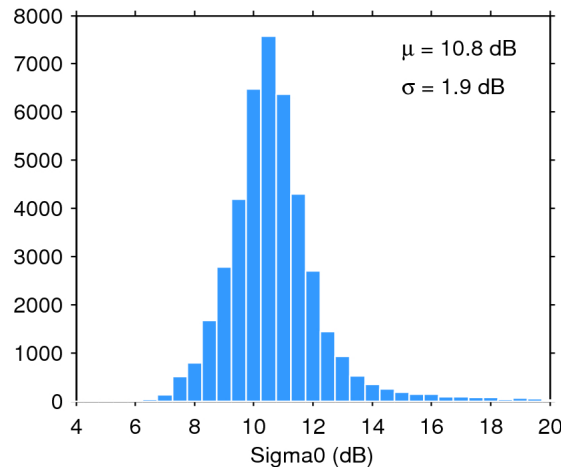
Figure 25. Histogram of flag-valid sigma0 over oceans and lakes for 26/01/2020. The mean ( \mu ) and standard deviation ( \sigma ) are also shown. Note that values outside [4 20] dB are excluded from the histogram for the sake of readability but not from the computation of \mu and \sigma .
