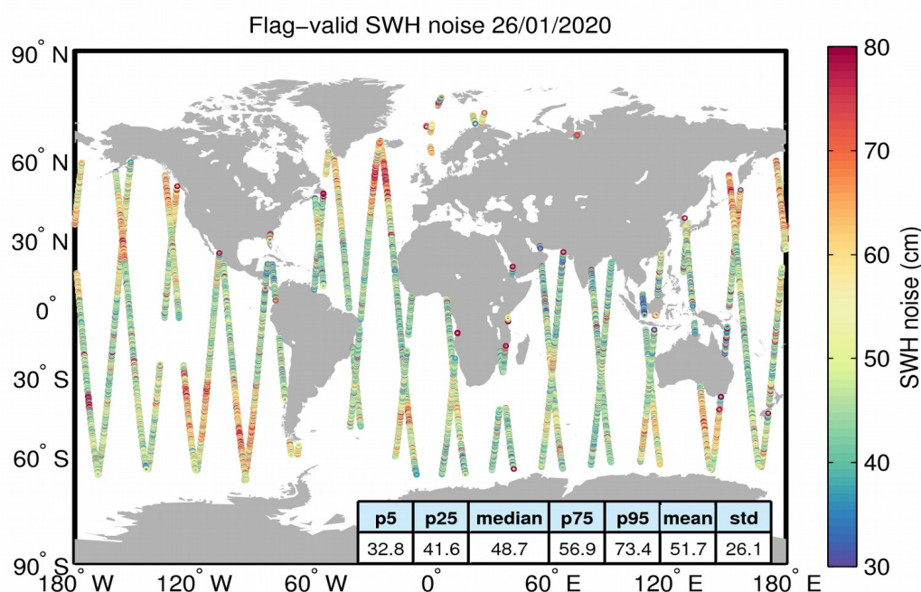
Figure 18. Geographical distribution of flag-valid 20-Hz SWH measurement noise over oceans and lakes for 26/01/2020. The statistical values shown in the table refer to the SWH noise and are calculated over all measurements shown in the figure.
