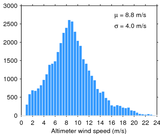
Figure 35. Histogram of science-valid wind over oceans and lakes for 25/01/2020. The mean ( \mu ) and standard deviation ( \sigma ) are also shown. Note that values larger than 24 m/s are excluded from the histogram for the sake of readability but not from the computation of \mu and \sigma .
