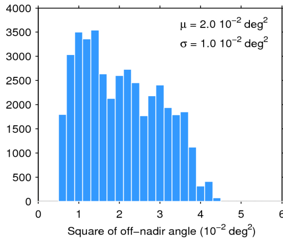
Figure 39. Histogram of flag-valid mispointing over oceans and lakes for 25/01/2020. The mean ( \mu ) and standard deviation ( \sigma ) are also shown. Note that values larger than 6 \cdot 10^{-2} \text{ deg}^2 are excluded from the histogram for the sake of readability but not from the computation of \mu and \sigma .
