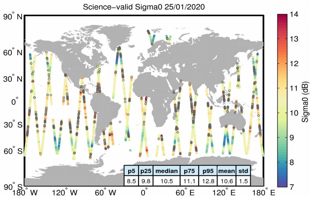
Figure 27. Geographical distribution of science-valid sigma0 data over oceans and lakes for 25/01/2020. The statistical values shown in the table refer to the sigma0 in dB and are calculated over all measurements shown in the figure. Gray circles denote records that have been rejected based on the editing criteria described in Table 4.
