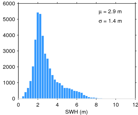
Figure 20. Histogram of science-valid SWH over oceans and lakes for 25/01/2020. The mean ( \mu ) and standard deviation ( \sigma ) are also shown. Note that values larger than 12 m are excluded from the histogram for the sake of readability but not from the computation of \mu and \sigma .
