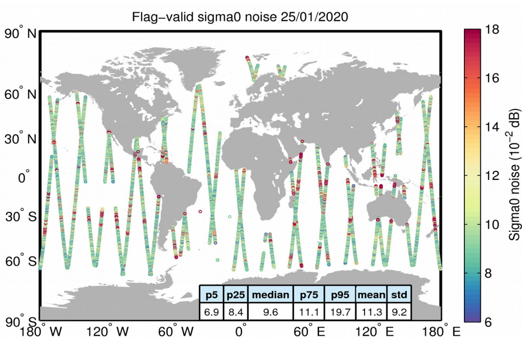
Figure 26. Geographical distribution of flag-valid 20-Hz sigma0 measurement noise over oceans and lakes for 25/01/2020. The statistical values shown in the table refer to the sigma0 noise and are calculated over all measurements shown in the figure.
