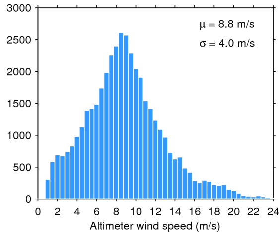
Figure 33. Histogram of flag-valid wind over oceans and lakes for 25/01/2020. The mean ( \mu ) and standard deviation ( \sigma ) are also shown. Note that values larger than 24 m/s are excluded from the histogram for the sake of readability but not from the computation of \mu and \sigma .
