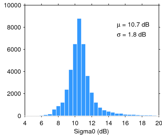
Figure 25. Histogram of flag-valid sigma0 over oceans and lakes for 25/01/2020. The mean ( \mu ) and standard deviation ( \sigma ) are also shown. Note that values outside [4 20] dB are excluded from the histogram for the sake of readability but not from the computation of \mu and \sigma .
