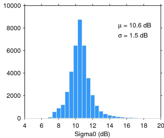
Figure 28. Histogram of science-valid sigma0 over oceans and lakes for 25/01/2020. The mean ( \mu ) and standard deviation ( \sigma ) are also shown. Note that values outside [4 20] dB are excluded from the histogram for the sake of readability but not from the computation of \mu and \sigma .
