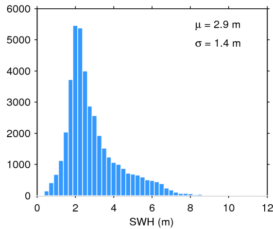
Figure 17. Histogram of flag-valid SWH over oceans and lakes for 25/01/2020. The mean ( \mu ) and standard deviation ( \sigma ) are also shown. Note that values larger than 12 m are excluded from the histogram for the sake of readability but not from the computation of \mu and \sigma .
