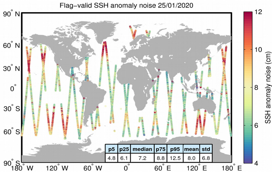
Figure 8. Geographical distribution of flag-valid 20-Hz SSH anomaly measurement noise over oceans and lakes for 25/01/2020. The statistical values shown in the table refer to the SSH anomaly noise and are calculated over all measurements shown in the figure.
