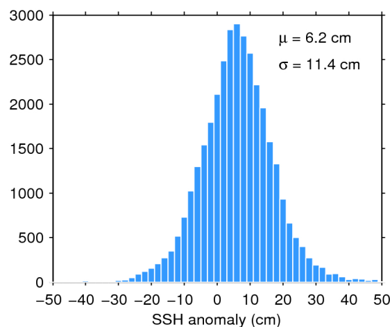
Figure 11. Histogram of science-valid SSH anomaly over oceans and lakes for 25/01/2020. The mean ( \mu ) and standard deviation ( \sigma ) are also shown. Note that values outside [-50 50] cm are excluded from the histogram for the sake of readability but not from the computation of \mu and \sigma .
