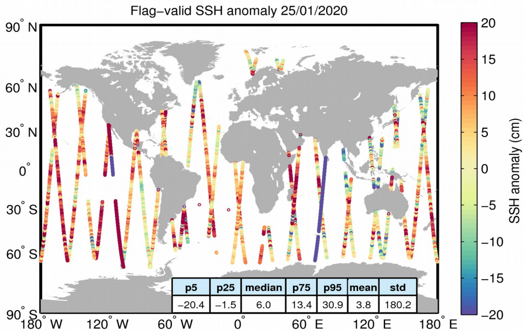
Figure 5. Geographical distribution of flag-valid 1-Hz SSH anomaly data over oceans and lakes for 25/01/2020. The statistical values shown in the table refer to the SSH anomaly in cm and are calculated over all measurements shown in the figure.
