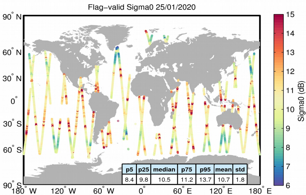
Figure 23. Geographical distribution of flag-valid sigma0 data over oceans and lakes for 25/01/2020. The statistical values shown in the table refer to the sigma0 in dB and are calculated over all measurements shown in the figure.
