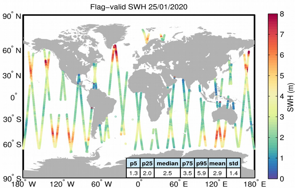
Figure 15. Geographical distribution of flag-valid SWH data over oceans and lakes for 25/01/2020. The statistical values shown in the table refer to the SWH in m and are calculated over all measurements shown in the figure.
