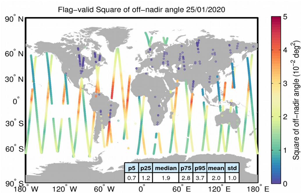
Figure 37. Geographical distribution of flag-valid mispointing data over oceans and lakes for 25/01/2020. The statistical values shown in the table refer to the mispointing in 10^{-2} deg 2 and are calculated over all measurements shown in the figure.
