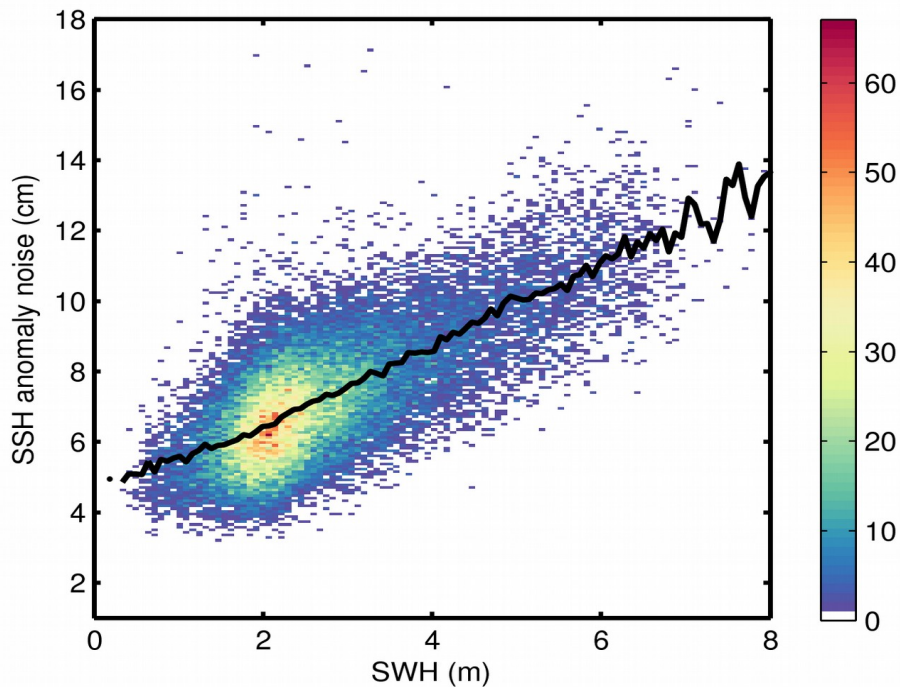
Figure 9. 2D histogram showing flag-valid SSH anomaly noise as a function of SWH for 25/01/2020. The black line denotes the median SSH anomaly noise as a function of SWH.
