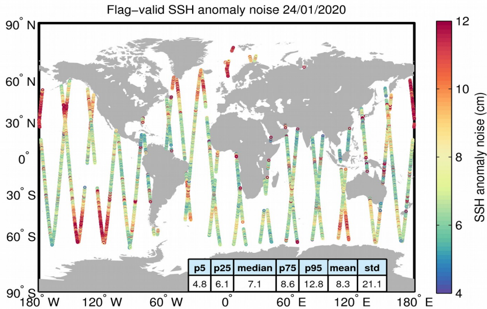
Figure 8. Geographical distribution of flag-valid 20-Hz SSH anomaly measurement noise over oceans and lakes for 24/01/2020. The statistical values shown in the table refer to the SSH anomaly noise and are calculated over all measurements shown in the figure.
