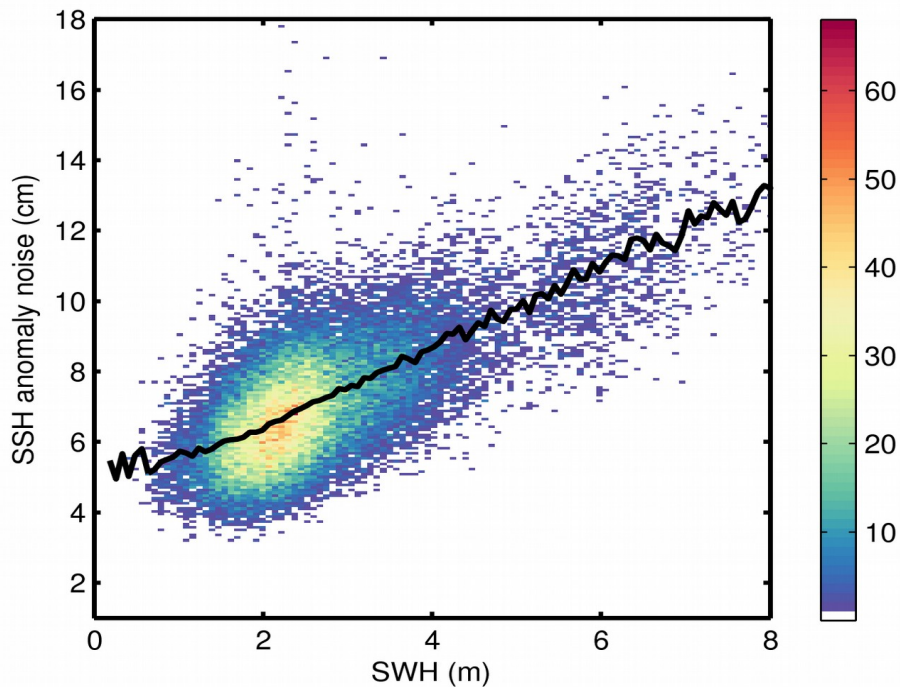
Figure 9. 2D histogram showing flag-valid SSH anomaly noise as a function of SWH for 24/01/2020. The black line denotes the median SSH anomaly noise as a function of SWH.
