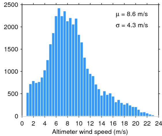
Figure 33. Histogram of flag-valid wind over oceans and lakes for 24/01/2020. The mean ( \mu ) and standard deviation ( \sigma ) are also shown. Note that values larger than 24 m/s are excluded from the histogram for the sake of readability but not from the computation of \mu and \sigma .
