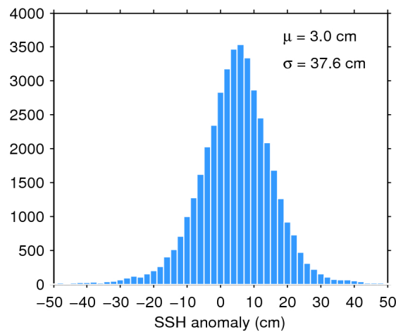
Figure 7. Histogram of flag-valid SSH anomaly over oceans and lakes for 24/01/2020. The mean ( \mu ) and standard deviation ( \sigma ) are also shown. Note that values outside [-50 50] cm are excluded from the histogram for the sake of readability but not from the computation of \mu and \sigma .
