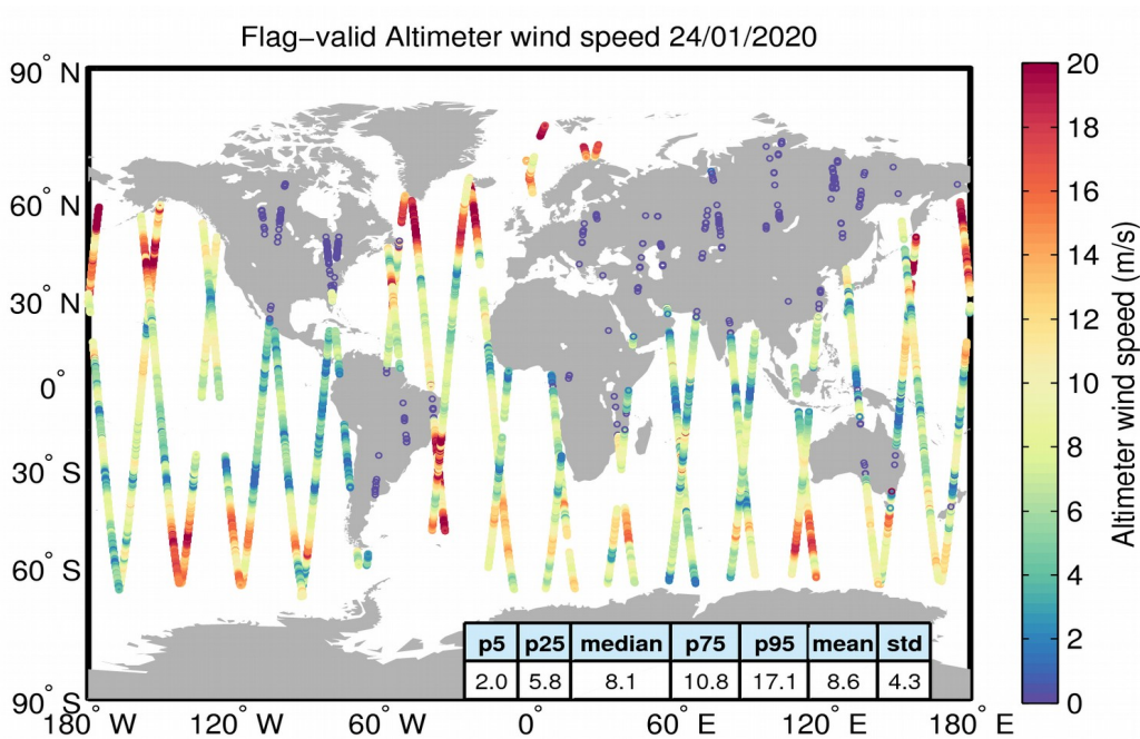
Figure 31. Geographical distribution of flag-valid wind data over oceans and lakes for 24/01/2020. The statistical values shown in the table refer to the wind in m/s and are calculated over all measurements shown in the figure.
