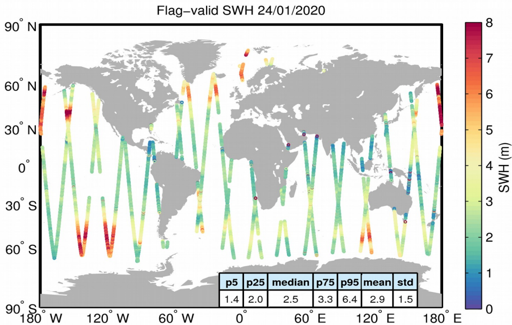
Figure 15. Geographical distribution of flag-valid SWH data over oceans and lakes for 24/01/2020. The statistical values shown in the table refer to the SWH in m and are calculated over all measurements shown in the figure.
