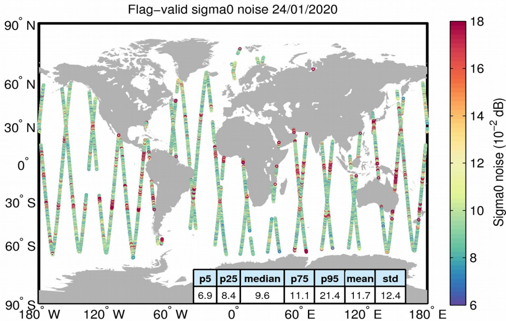
Figure 26. Geographical distribution of flag-valid 20-Hz sigma0 measurement noise over oceans and lakes for 24/01/2020. The statistical values shown in the table refer to the sigma0 noise and are calculated over all measurements shown in the figure.
