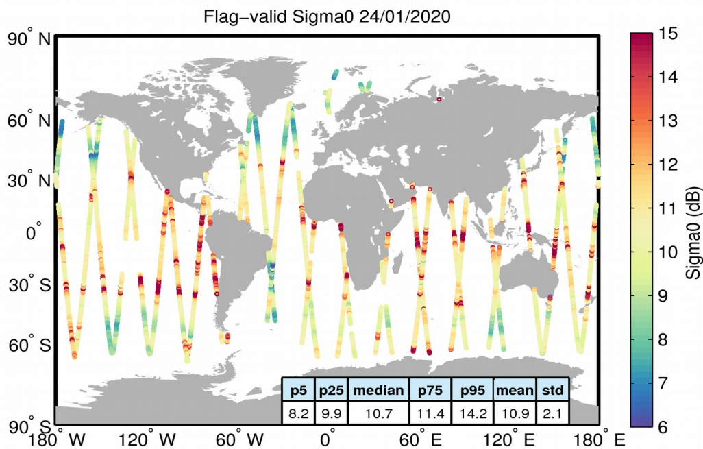
Figure 23. Geographical distribution of flag-valid sigma0 data over oceans and lakes for 24/01/2020. The statistical values shown in the table refer to the sigma0 in dB and are calculated over all measurements shown in the figure.
