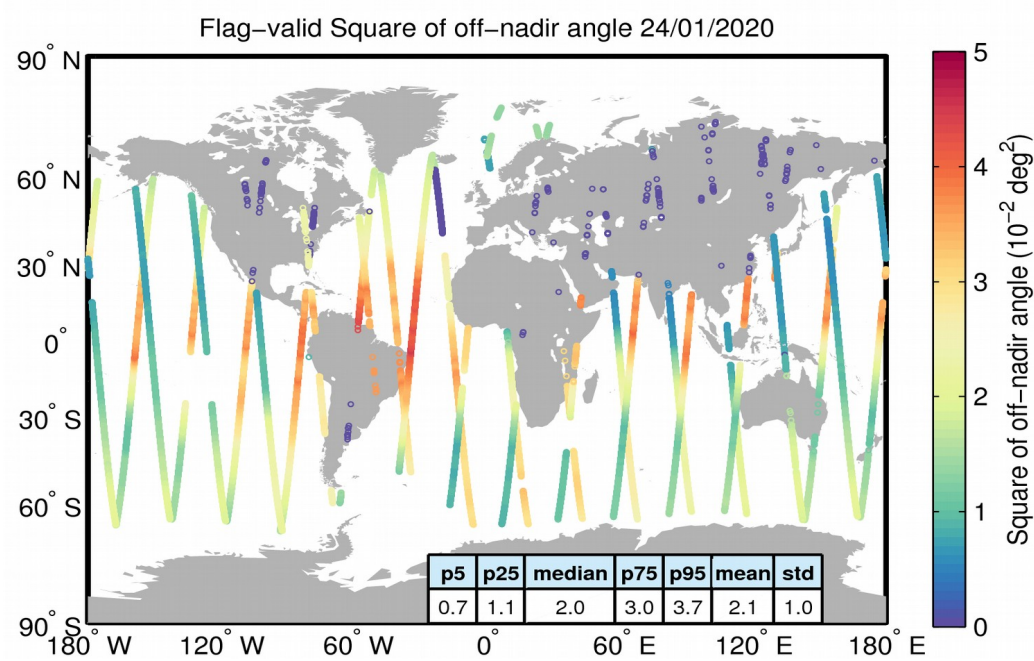
Figure 37. Geographical distribution of flag-valid mispointing data over oceans and lakes for 24/01/2020. The statistical values shown in the table refer to the mispointing in 10^{-2} \text{deg}^2 and are calculated over all measurements shown in the figure.
