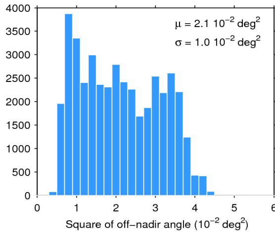
Figure 39. Histogram of flag-valid mispointing over oceans and lakes for 24/01/2020. The mean ( \mu ) and standard deviation ( \sigma ) are also shown. Note that values larger than 6 \cdot 10^{-2} \text{ deg}^2 are excluded from the histogram for the sake of readability but not from the computation of \mu and \sigma .
