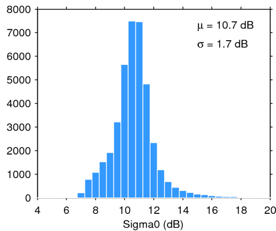
Figure 28. Histogram of science-valid sigma0 over oceans and lakes for 24/01/2020. The mean ( \mu ) and standard deviation ( \sigma ) are also shown. Note that values outside [4 20] dB are excluded from the histogram for the sake of readability but not from the computation of \mu and \sigma .
