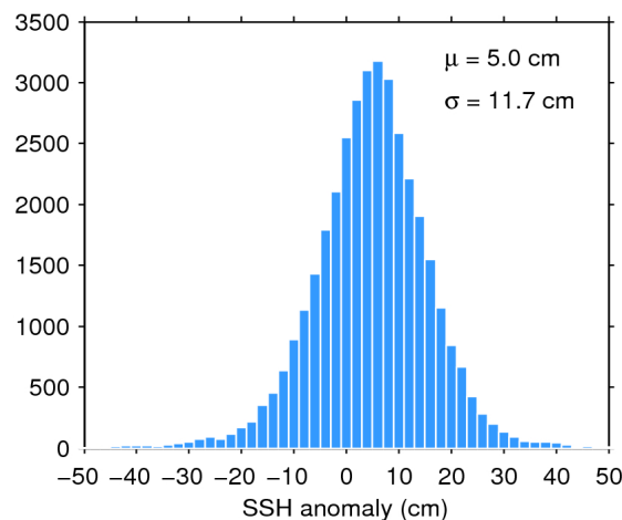
Figure 11. Histogram of science-valid SSH anomaly over oceans and lakes for 24/01/2020. The mean ( \mu ) and standard deviation ( \sigma ) are also shown. Note that values outside [-50 50] cm are excluded from the histogram for the sake of readability but not from the computation of \mu and \sigma .
