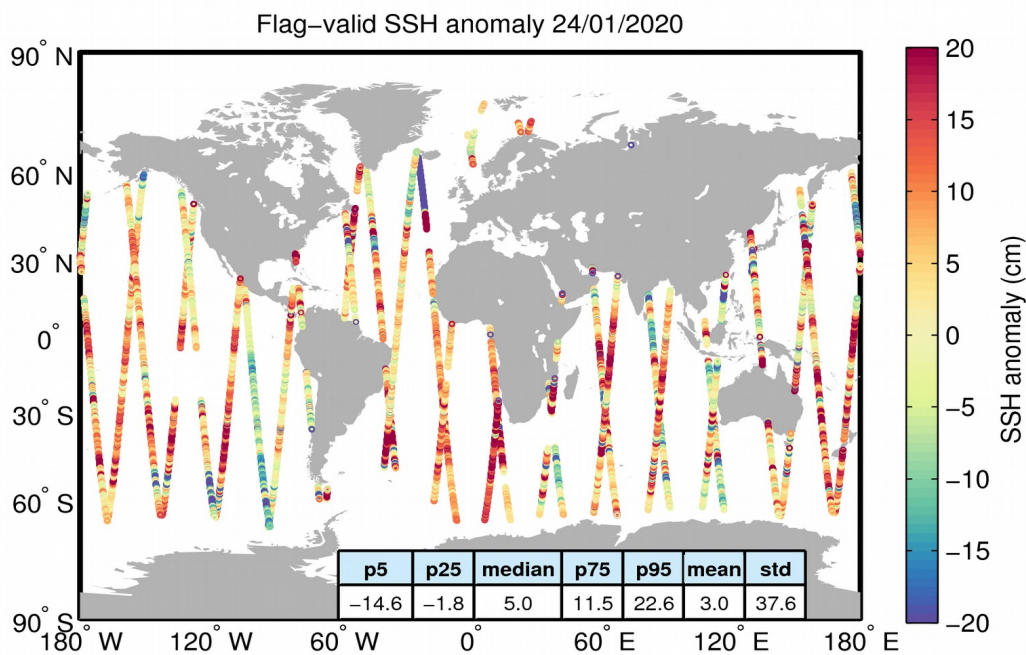
Figure 5. Geographical distribution of flag-valid 1-Hz SSH anomaly data over oceans and lakes for 24/01/2020. The statistical values shown in the table refer to the SSH anomaly in cm and are calculated over all measurements shown in the figure.
