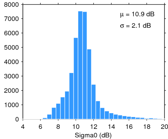
Figure 25. Histogram of flag-valid sigma0 over oceans and lakes for 24/01/2020. The mean ( \mu ) and standard deviation ( \sigma ) are also shown. Note that values outside [4 20] dB are excluded from the histogram for the sake of readability but not from the computation of \mu and \sigma .
