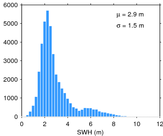
Figure 20. Histogram of science-valid SWH over oceans and lakes for 24/01/2020. The mean ( \mu ) and standard deviation ( \sigma ) are also shown. Note that values larger than 12 m are excluded from the histogram for the sake of readability but not from the computation of \mu and \sigma .
