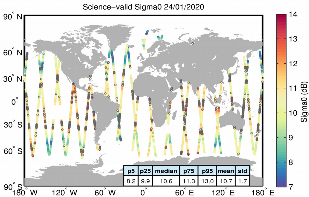
Figure 27. Geographical distribution of science-valid sigma0 data over oceans and lakes for 24/01/2020. The statistical values shown in the table refer to the sigma0 in dB and are calculated over all measurements shown in the figure. Gray circles denote records that have been rejected based on the editing criteria described in Table 4.
