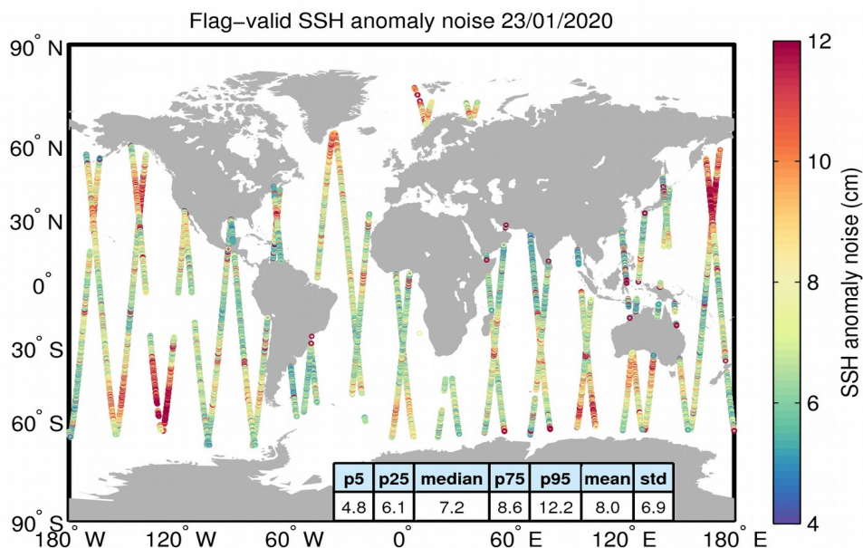
Figure 8. Geographical distribution of flag-valid 20-Hz SSH anomaly measurement noise over oceans and lakes for 23/01/2020. The statistical values shown in the table refer to the SSH anomaly noise and are calculated over all measurements shown in the figure.
