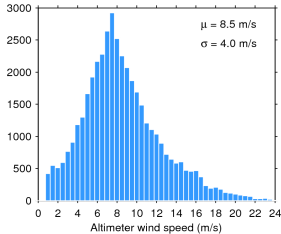
Figure 33. Histogram of flag-valid wind over oceans and lakes for 23/01/2020. The mean ( \mu ) and standard deviation ( \sigma ) are also shown. Note that values larger than 24 m/s are excluded from the histogram for the sake of readability but not from the computation of \mu and \sigma .
