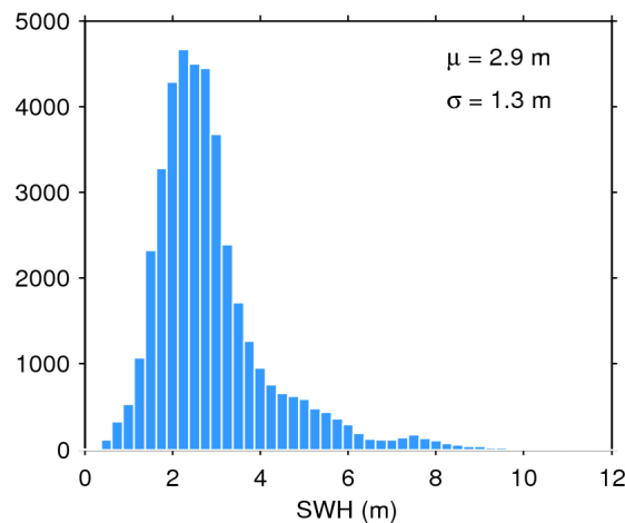
Figure 20. Histogram of science-valid SWH over oceans and lakes for 23/01/2020. The mean ( \mu ) and standard deviation ( \sigma ) are also shown. Note that values larger than 12 m are excluded from the histogram for the sake of readability but not from the computation of \mu and \sigma .
