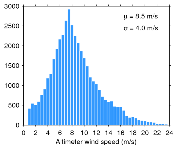
Figure 35. Histogram of science-valid wind over oceans and lakes for 23/01/2020. The mean ( \mu ) and standard deviation ( \sigma ) are also shown. Note that values larger than 24 m/s are excluded from the histogram for the sake of readability but not from the computation of \mu and \sigma .
