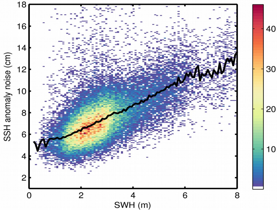
Figure 9. 2D histogram showing flag-valid SSH anomaly noise as a function of SWH for 23/01/2020. The black line denotes the median SSH anomaly noise as a function of SWH.
