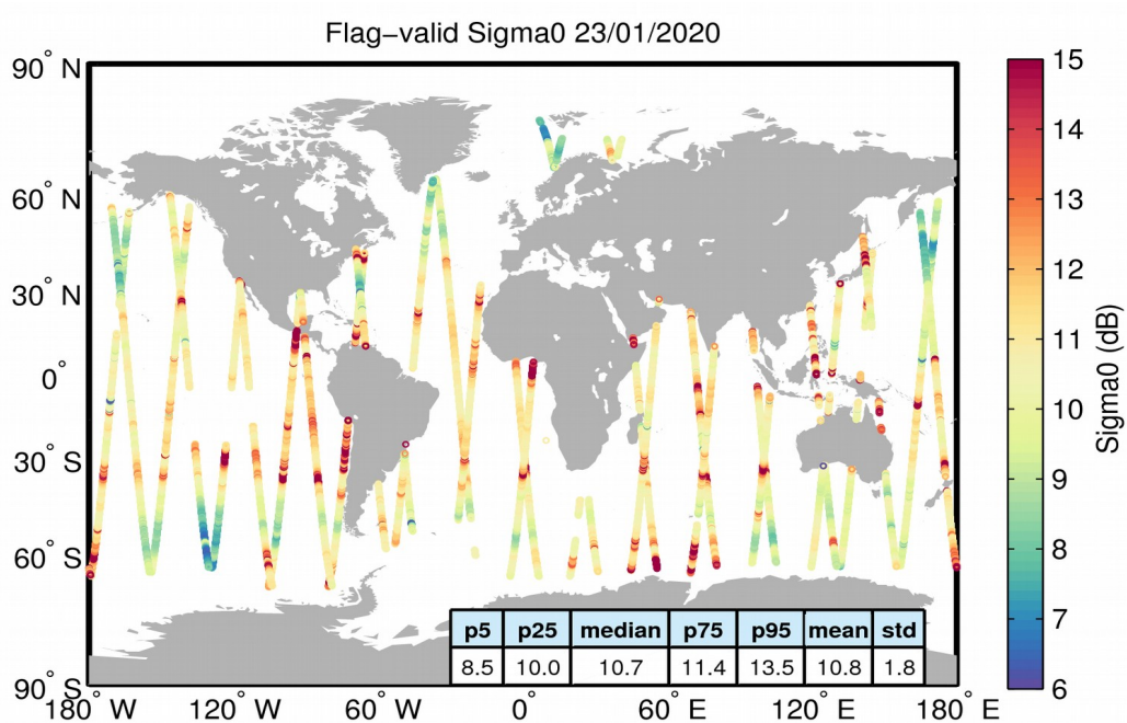
Figure 23. Geographical distribution of flag-valid sigma0 data over oceans and lakes for 23/01/2020. The statistical values shown in the table refer to the sigma0 in dB and are calculated over all measurements shown in the figure.
