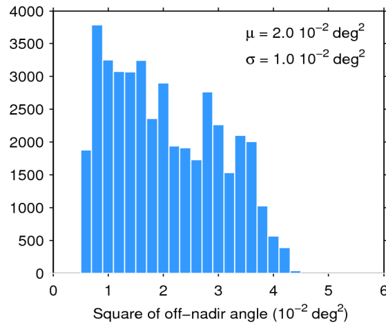
Figure 39. Histogram of flag-valid mispointing over oceans and lakes for 23/01/2020. The mean ( \mu ) and standard deviation ( \sigma ) are also shown. Note that values larger than 6 \cdot 10^{-2} \text{ deg}^2 are excluded from the histogram for the sake of readability but not from the computation of \mu and \sigma .
