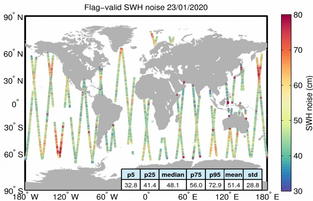
Figure 18. Geographical distribution of flag-valid 20-Hz SWH measurement noise over oceans and lakes for 23/01/2020. The statistical values shown in the table refer to the SWH noise and are calculated over all measurements shown in the figure.
