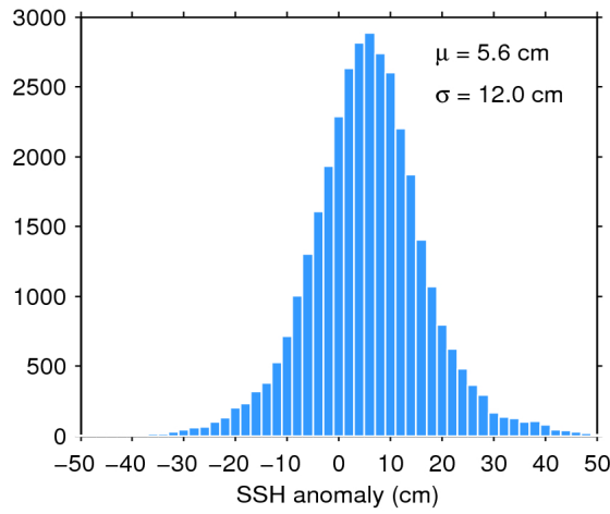
Figure 11. Histogram of science-valid SSH anomaly over oceans and lakes for 23/01/2020. The mean ( \mu ) and standard deviation ( \sigma ) are also shown. Note that values outside [-50 50] cm are excluded from the histogram for the sake of readability but not from the computation of \mu and \sigma .
