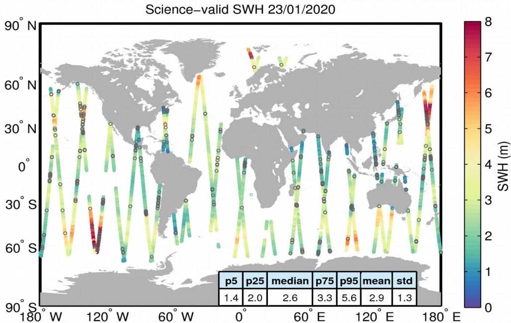
Figure 19. Geographical distribution of science-valid SWH data over oceans and lakes for 23/01/2020. The statistical values shown in the table refer to the SWH in m and are calculated over all measurements shown in the figure. Gray circles denote records that have been rejected based on the editing criteria described in Table 3.
