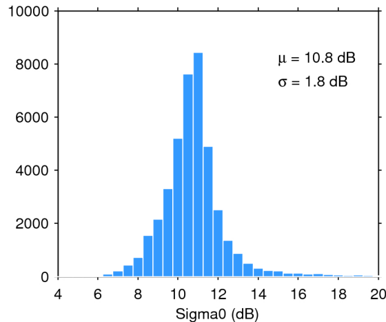
Figure 25. Histogram of flag-valid sigma0 over oceans and lakes for 23/01/2020. The mean ( \mu ) and standard deviation ( \sigma ) are also shown. Note that values outside [4 20] dB are excluded from the histogram for the sake of readability but not from the computation of \mu and \sigma .
