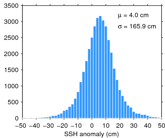
Figure 7. Histogram of flag-valid SSH anomaly over oceans and lakes for 23/01/2020. The mean ( \mu ) and standard deviation ( \sigma ) are also shown. Note that values outside [-50\ 50] cm are excluded from the histogram for the sake of readability but not from the computation of \mu and \sigma .
