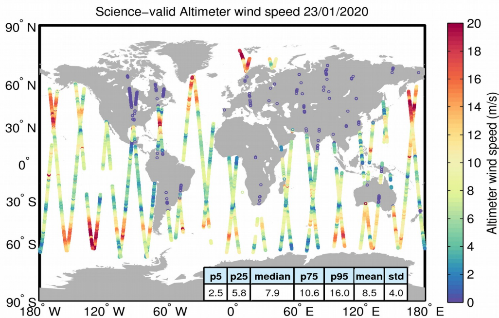
Figure 34. Geographical distribution of science-valid wind data over oceans and lakes for 23/01/2020. The statistical values shown in the table refer to the wind in m/s and are calculated over all measurements shown in the figure. Gray circles denote records that have been rejected based on the editing criteria described in Table 5.
