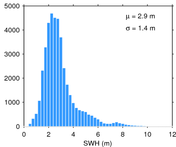
Figure 17. Histogram of flag-valid SWH over oceans and lakes for 23/01/2020. The mean ( \mu ) and standard deviation ( \sigma ) are also shown. Note that values larger than 12 m are excluded from the histogram for the sake of readability but not from the computation of \mu and \sigma .
