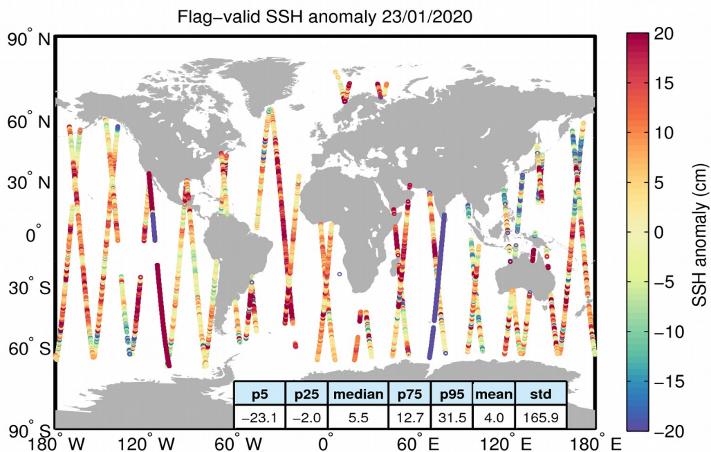
Figure 5. Geographical distribution of flag-valid 1-Hz SSH anomaly data over oceans and lakes for 23/01/2020. The statistical values shown in the table refer to the SSH anomaly in cm and are calculated over all measurements shown in the figure.
