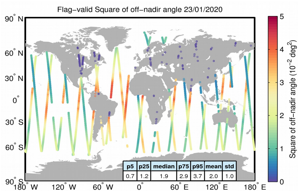
Figure 37. Geographical distribution of flag-valid mispointing data over oceans and lakes for 23/01/2020. The statistical values shown in the table refer to the mispointing in 10^{-2} \text{ deg}^2 and are calculated over all measurements shown in the figure.
