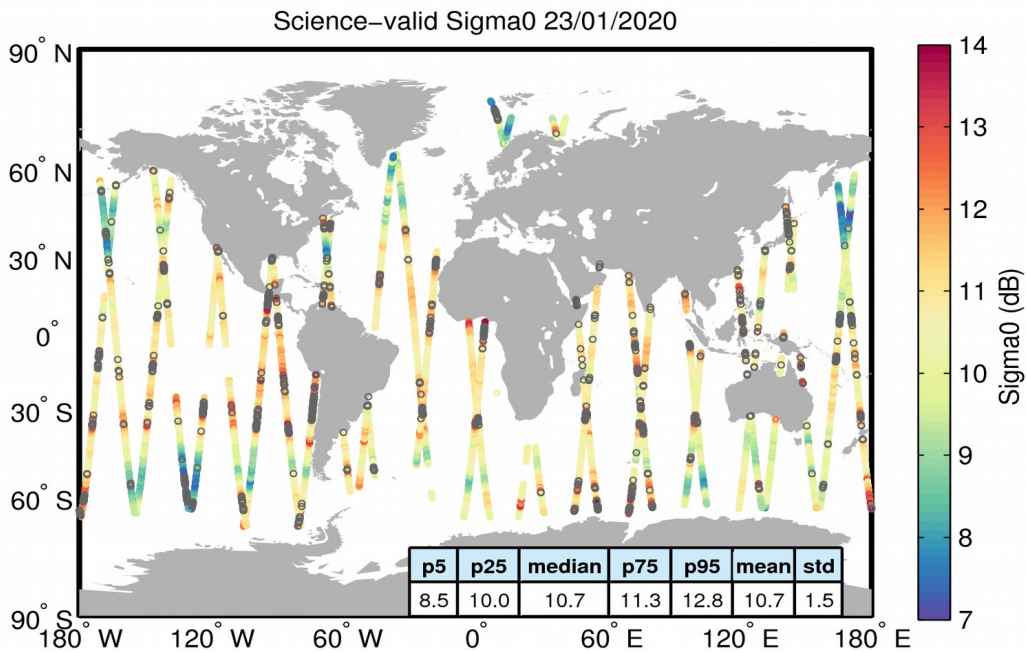
Figure 27. Geographical distribution of science-valid sigma0 data over oceans and lakes for 23/01/2020. The statistical values shown in the table refer to the sigma0 in dB and are calculated over all measurements shown in the figure. Gray circles denote records that have been rejected based on the editing criteria described in Table 4.
