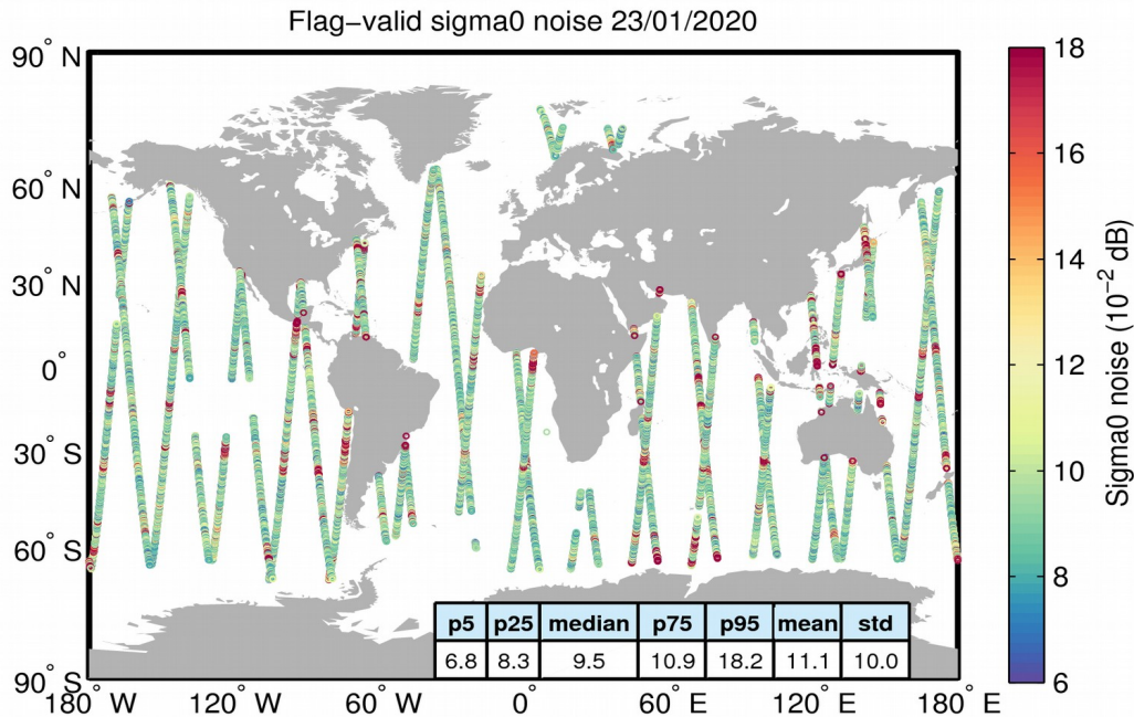
Figure 26. Geographical distribution of flag-valid 20-Hz sigma0 measurement noise over oceans and lakes for 23/01/2020. The statistical values shown in the table refer to the sigma0 noise and are calculated over all measurements shown in the figure.
