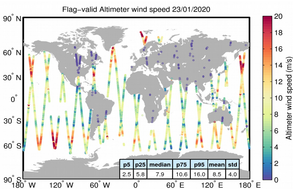
Figure 31. Geographical distribution of flag-valid wind data over oceans and lakes for 23/01/2020. The statistical values shown in the table refer to the wind in m/s and are calculated over all measurements shown in the figure.
