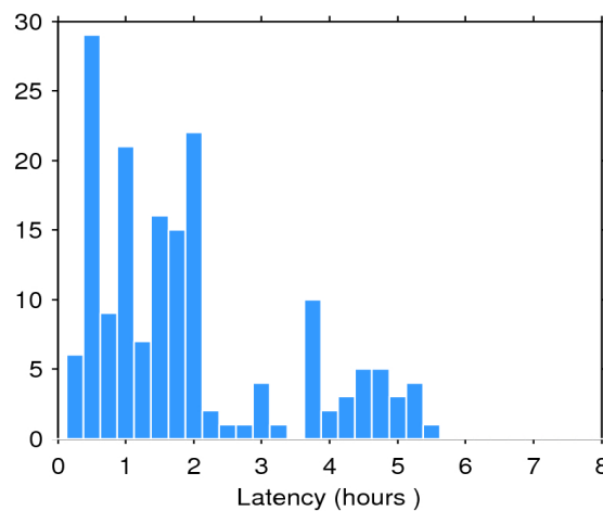
Figure 2. Histogram of the data latency for 23/01/2020. The y-axis denotes the number of files that are made available with a delay of x-hours with respect to the mean time of the records stored in the file.
