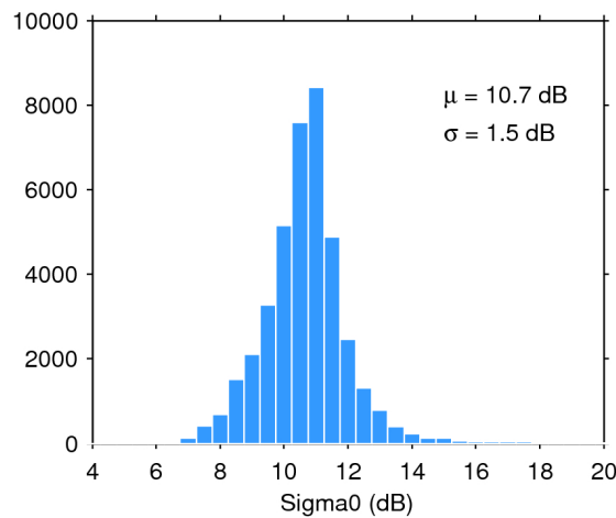
Figure 28. Histogram of science-valid sigma0 over oceans and lakes for 23/01/2020. The mean ( \mu ) and standard deviation ( \sigma ) are also shown. Note that values outside [4 20] dB are excluded from the histogram for the sake of readability but not from the computation of \mu and \sigma .
