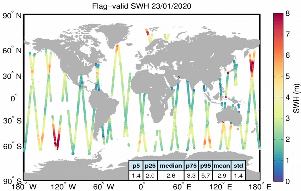
Figure 15. Geographical distribution of flag-valid SWH data over oceans and lakes for 23/01/2020. The statistical values shown in the table refer to the SWH in m and are calculated over all measurements shown in the figure.
