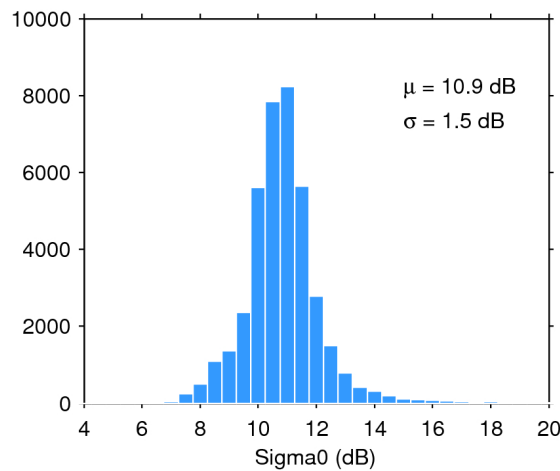
Figure 28. Histogram of science-valid sigma0 over oceans and lakes for 21/01/2020. The mean ( \mu ) and standard deviation ( \sigma ) are also shown. Note that values outside [4 20] dB are excluded from the histogram for the sake of readability but not from the computation of \mu and \sigma .
