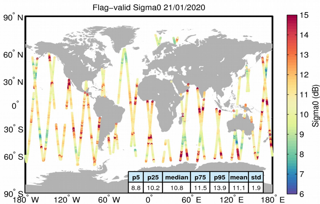
Figure 23. Geographical distribution of flag-valid sigma0 data over oceans and lakes for 21/01/2020. The statistical values shown in the table refer to the sigma0 in dB and are calculated over all measurements shown in the figure.
