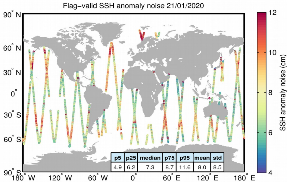
Figure 8. Geographical distribution of flag-valid 20-Hz SSH anomaly measurement noise over oceans and lakes for 21/01/2020. The statistical values shown in the table refer to the SSH anomaly noise and are calculated over all measurements shown in the figure.
