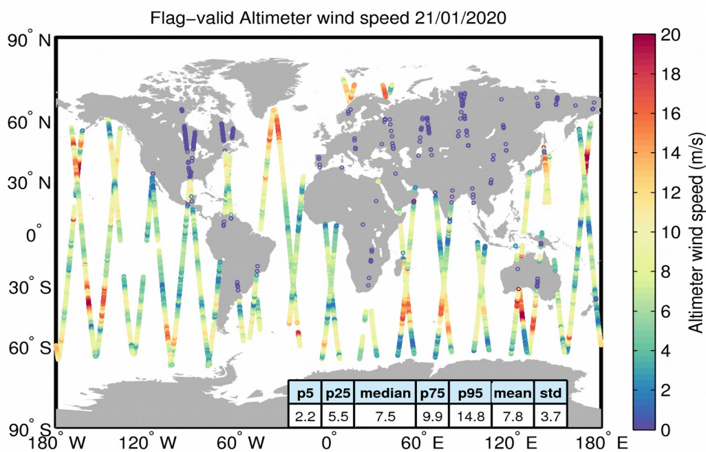
Figure 31. Geographical distribution of flag-valid wind data over oceans and lakes for 21/01/2020. The statistical values shown in the table refer to the wind in m/s and are calculated over all measurements shown in the figure.
