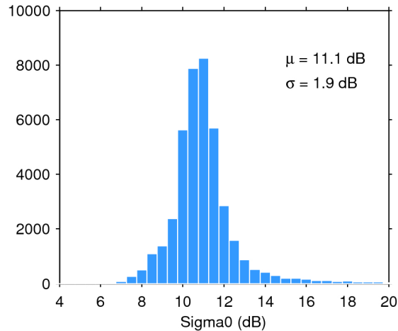
Figure 25. Histogram of flag-valid sigma0 over oceans and lakes for 21/01/2020. The mean ( \mu ) and standard deviation ( \sigma ) are also shown. Note that values outside [4 20] dB are excluded from the histogram for the sake of readability but not from the computation of \mu and \sigma .
