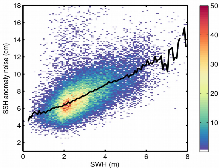
Figure 9. 2D histogram showing flag-valid SSH anomaly noise as a function of SWH for 21/01/2020. The black line denotes the median SSH anomaly noise as a function of SWH.
