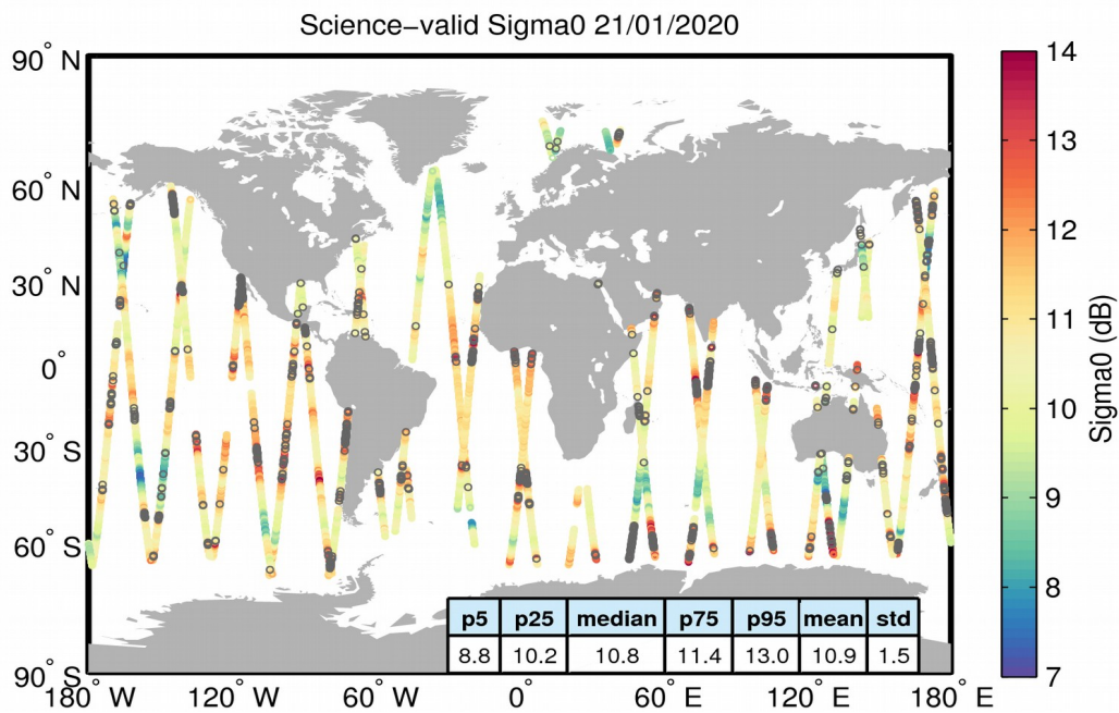
Figure 27. Geographical distribution of science-valid sigma0 data over oceans and lakes for 21/01/2020. The statistical values shown in the table refer to the sigma0 in dB and are calculated over all measurements shown in the figure. Gray circles denote records that have been rejected based on the editing criteria described in Table 4.
