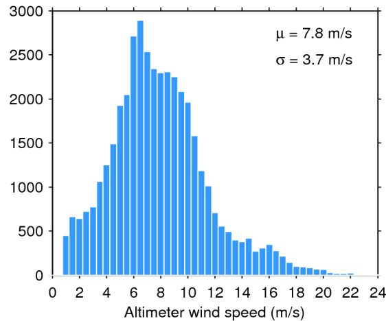
Figure 33. Histogram of flag-valid wind over oceans and lakes for 21/01/2020. The mean ( \mu ) and standard deviation ( \sigma ) are also shown. Note that values larger than 24 m/s are excluded from the histogram for the sake of readability but not from the computation of \mu and \sigma .
