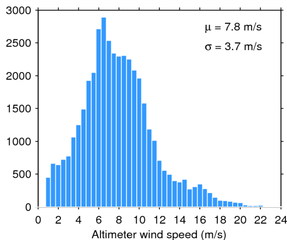
Figure 35. Histogram of science-valid wind over oceans and lakes for 21/01/2020. The mean ( \mu ) and standard deviation ( \sigma ) are also shown. Note that values larger than 24 m/s are excluded from the histogram for the sake of readability but not from the computation of \mu and \sigma .
