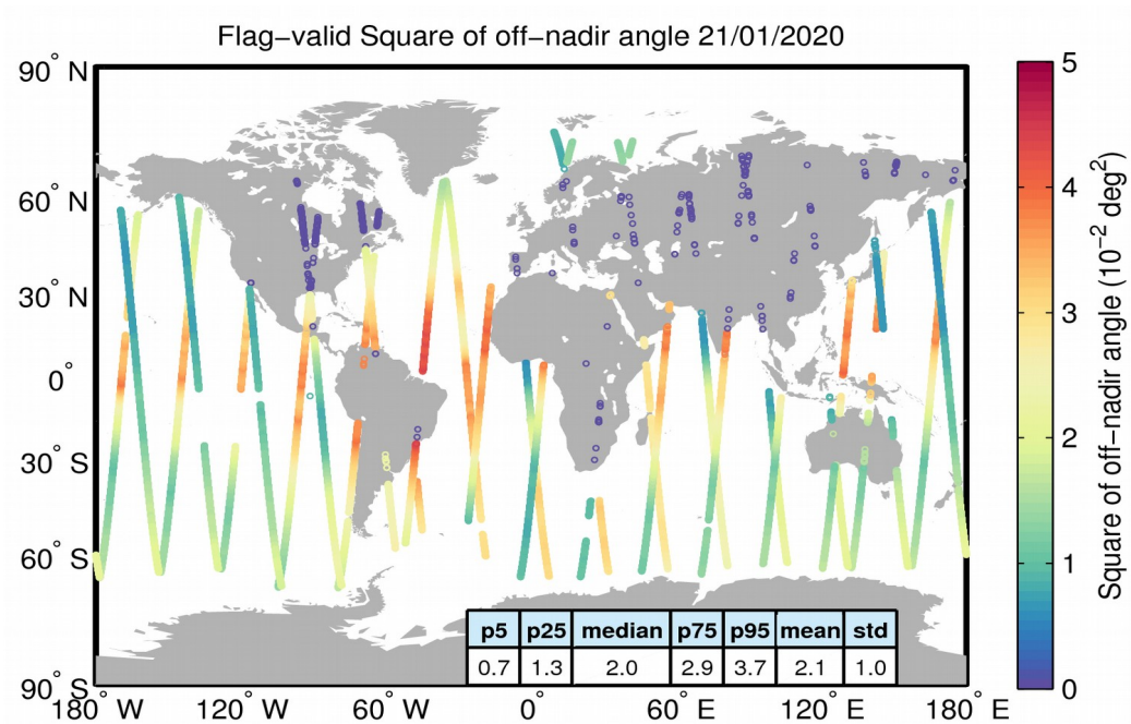
Figure 37. Geographical distribution of flag-valid mispointing data over oceans and lakes for 21/01/2020. The statistical values shown in the table refer to the mispointing in 10^{-2} \text{ deg}^2 and are calculated over all measurements shown in the figure.
