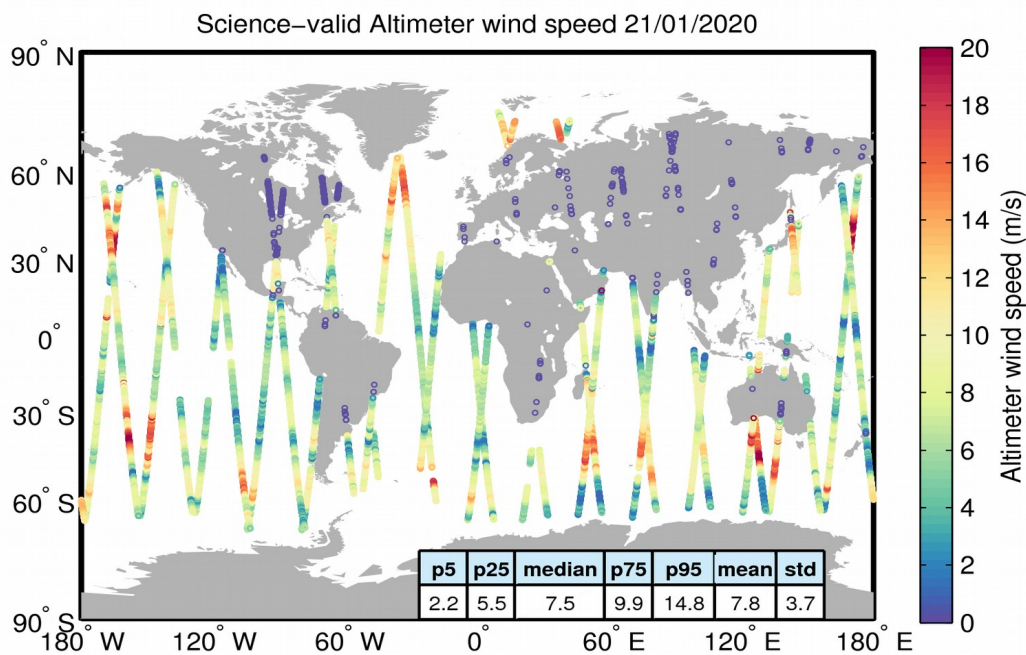
Figure 34. Geographical distribution of science-valid wind data over oceans and lakes for 21/01/2020. The statistical values shown in the table refer to the wind in m/s and are calculated over all measurements shown in the figure. Gray circles denote records that have been rejected based on the editing criteria described in Table 5.
