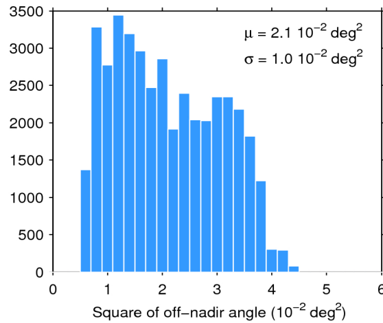
Figure 39. Histogram of flag-valid mispointing over oceans and lakes for 21/01/2020. The mean ( \mu ) and standard deviation ( \sigma ) are also shown. Note that values larger than 6 \cdot 10^{-2} \text{ deg}^2 are excluded from the histogram for the sake of readability but not from the computation of \mu and \sigma .
