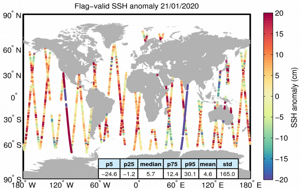
Figure 5. Geographical distribution of flag-valid 1-Hz SSH anomaly data over oceans and lakes for 21/01/2020. The statistical values shown in the table refer to the SSH anomaly in cm and are calculated over all measurements shown in the figure.
