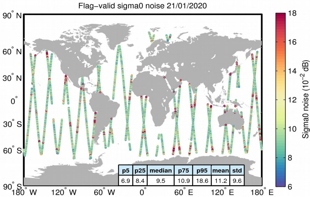
Figure 26. Geographical distribution of flag-valid 20-Hz sigma0 measurement noise over oceans and lakes for 21/01/2020. The statistical values shown in the table refer to the sigma0 noise and are calculated over all measurements shown in the figure.
