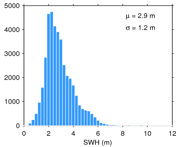
Figure 17. Histogram of flag-valid SWH over oceans and lakes for 21/01/2020. The mean ( \mu ) and standard deviation ( \sigma ) are also shown. Note that values larger than 12 m are excluded from the histogram for the sake of readability but not from the computation of \mu and \sigma .
