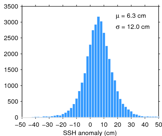
Figure 11. Histogram of science-valid SSH anomaly over oceans and lakes for 21/01/2020. The mean ( \mu ) and standard deviation ( \sigma ) are also shown. Note that values outside [-50 50] cm are excluded from the histogram for the sake of readability but not from the computation of \mu and \sigma .
