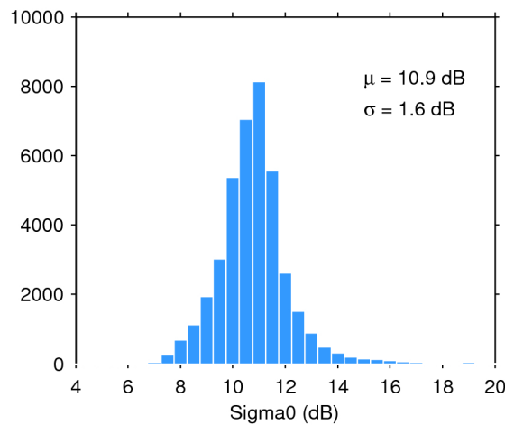
Figure 28. Histogram of science-valid sigma0 over oceans and lakes for 20/01/2020. The mean ( \mu ) and standard deviation ( \sigma ) are also shown. Note that values outside [4 20] dB are excluded from the histogram for the sake of readability but not from the computation of \mu and \sigma .
