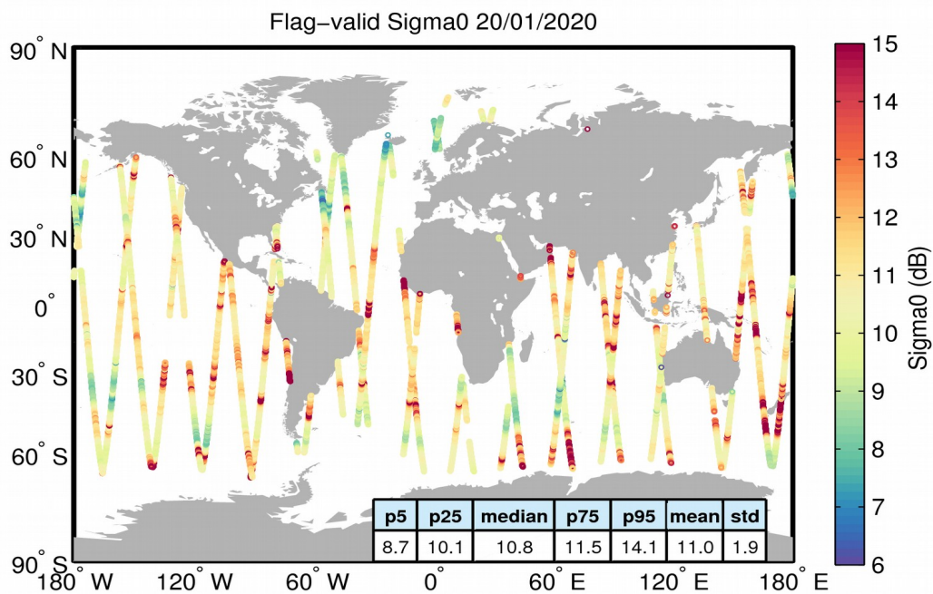
Figure 23. Geographical distribution of flag-valid sigma0 data over oceans and lakes for 20/01/2020. The statistical values shown in the table refer to the sigma0 in dB and are calculated over all measurements shown in the figure.
