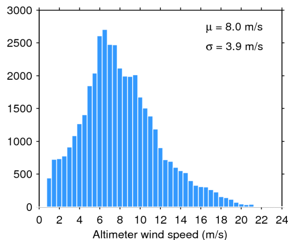
Figure 35. Histogram of science-valid wind over oceans and lakes for 20/01/2020. The mean ( \mu ) and standard deviation ( \sigma ) are also shown. Note that values larger than 24 m/s are excluded from the histogram for the sake of readability but not from the computation of \mu and \sigma .
