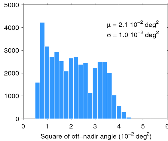
Figure 39. Histogram of flag-valid mispointing over oceans and lakes for 20/01/2020. The mean ( \mu ) and standard deviation ( \sigma ) are also shown. Note that values larger than 6 \cdot 10^{-2} \text{ deg}^2 are excluded from the histogram for the sake of readability but not from the computation of \mu and \sigma .
