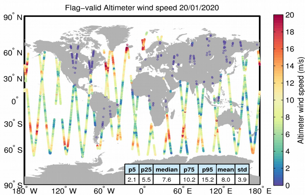
Figure 31. Geographical distribution of flag-valid wind data over oceans and lakes for 20/01/2020. The statistical values shown in the table refer to the wind in m/s and are calculated over all measurements shown in the figure.
