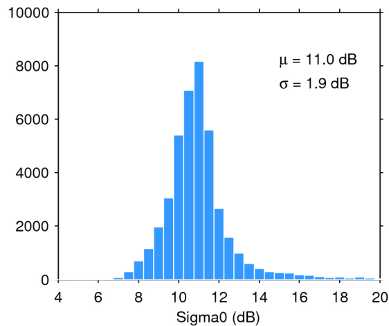
Figure 25. Histogram of flag-valid sigma0 over oceans and lakes for 20/01/2020. The mean ( \mu ) and standard deviation ( \sigma ) are also shown. Note that values outside [4 20] dB are excluded from the histogram for the sake of readability but not from the computation of \mu and \sigma .
