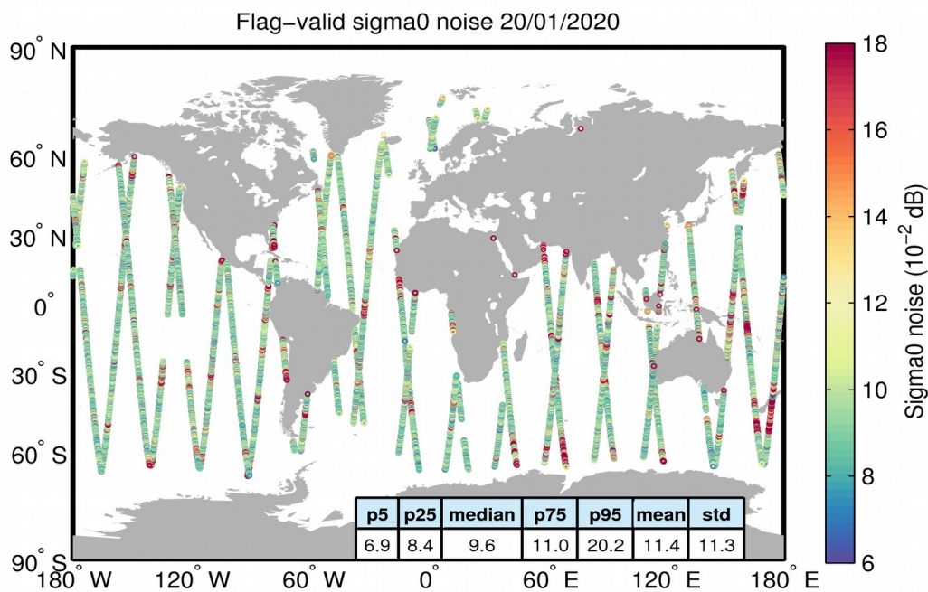
Figure 26. Geographical distribution of flag-valid 20-Hz sigma0 measurement noise over oceans and lakes for 20/01/2020. The statistical values shown in the table refer to the sigma0 noise and are calculated over all measurements shown in the figure.
