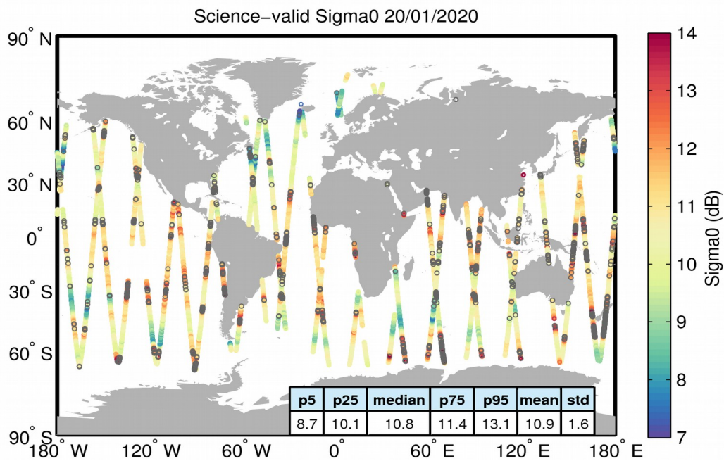
Figure 27. Geographical distribution of science-valid sigma0 data over oceans and lakes for 20/01/2020. The statistical values shown in the table refer to the sigma0 in dB and are calculated over all measurements shown in the figure. Gray circles denote records that have been rejected based on the editing criteria described in Table 4.
