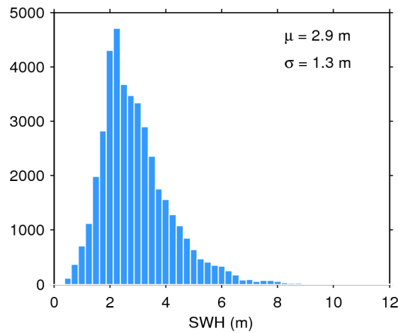
Figure 17. Histogram of flag-valid SWH over oceans and lakes for 20/01/2020. The mean ( \mu ) and standard deviation ( \sigma ) are also shown. Note that values larger than 12 m are excluded from the histogram for the sake of readability but not from the computation of \mu and \sigma .
