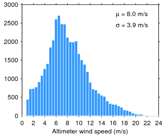
Figure 33. Histogram of flag-valid wind over oceans and lakes for 20/01/2020. The mean ( \mu ) and standard deviation ( \sigma ) are also shown. Note that values larger than 24 m/s are excluded from the histogram for the sake of readability but not from the computation of \mu and \sigma .
