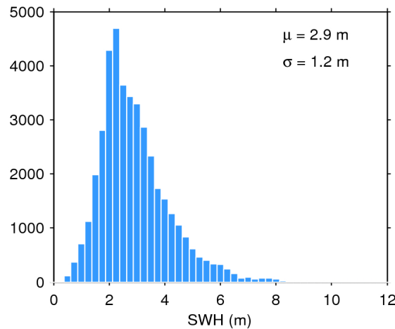
Figure 20. Histogram of science-valid SWH over oceans and lakes for 20/01/2020. The mean ( \mu ) and standard deviation ( \sigma ) are also shown. Note that values larger than 12 m are excluded from the histogram for the sake of readability but not from the computation of \mu and \sigma .
