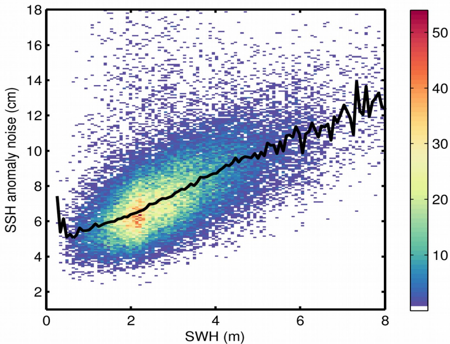
Figure 9. 2D histogram showing flag-valid SSH anomaly noise as a function of SWH for 20/01/2020. The black line denotes the median SSH anomaly noise as a function of SWH.
