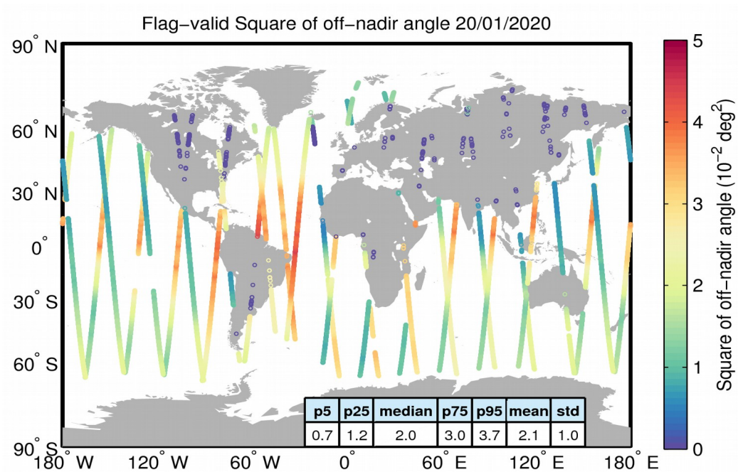
Figure 37. Geographical distribution of flag-valid mispointing data over oceans and lakes for 20/01/2020. The statistical values shown in the table refer to the mispointing in 10^{-2} deg 2 and are calculated over all measurements shown in the figure.
