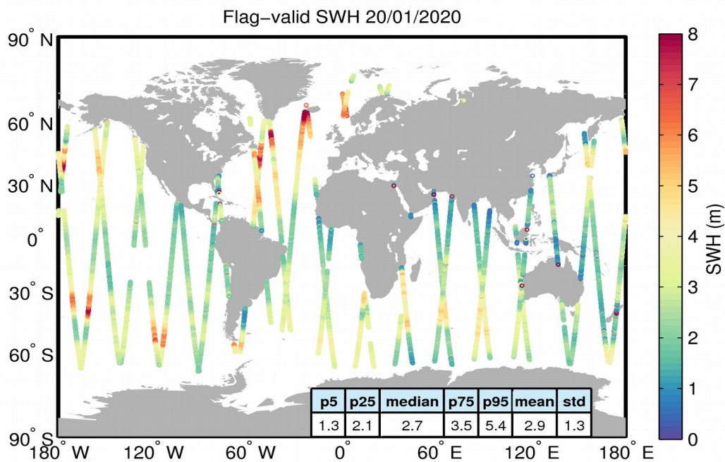
Figure 15. Geographical distribution of flag-valid SWH data over oceans and lakes for 20/01/2020. The statistical values shown in the table refer to the SWH in m and are calculated over all measurements shown in the figure.
