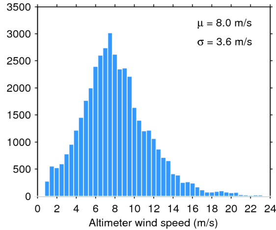
Figure 33. Histogram of flag-valid wind over oceans and lakes for 19/01/2020. The mean ( \mu ) and standard deviation ( \sigma ) are also shown. Note that values larger than 24 m/s are excluded from the histogram for the sake of readability but not from the computation of \mu and \sigma .
