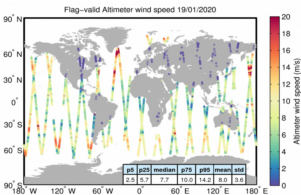
Figure 31. Geographical distribution of flag-valid wind data over oceans and lakes for 19/01/2020. The statistical values shown in the table refer to the wind in m/s and are calculated over all measurements shown in the figure.
