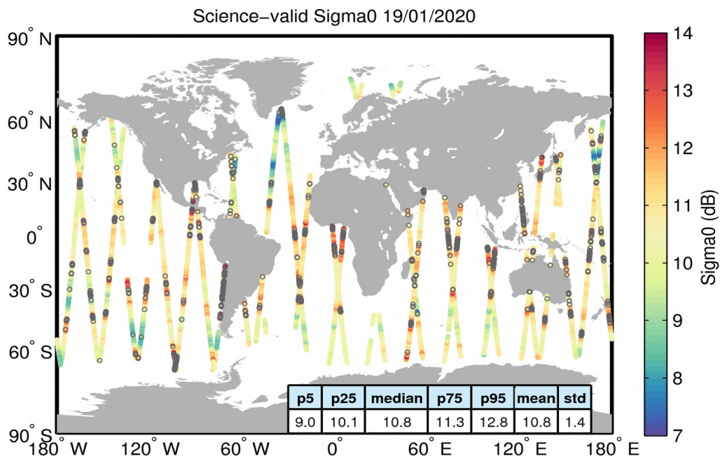
Figure 27. Geographical distribution of science-valid sigma0 data over oceans and lakes for 19/01/2020. The statistical values shown in the table refer to the sigma0 in dB and are calculated over all measurements shown in the figure. Gray circles denote records that have been rejected based on the editing criteria described in Table 4.
