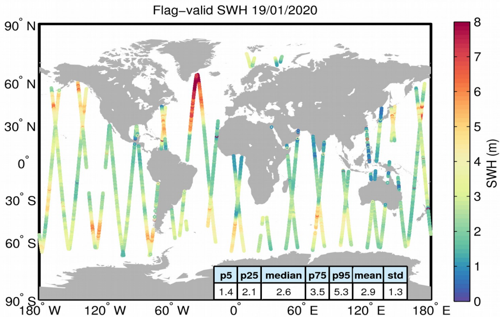
Figure 15. Geographical distribution of flag-valid SWH data over oceans and lakes for 19/01/2020. The statistical values shown in the table refer to the SWH in m and are calculated over all measurements shown in the figure.
