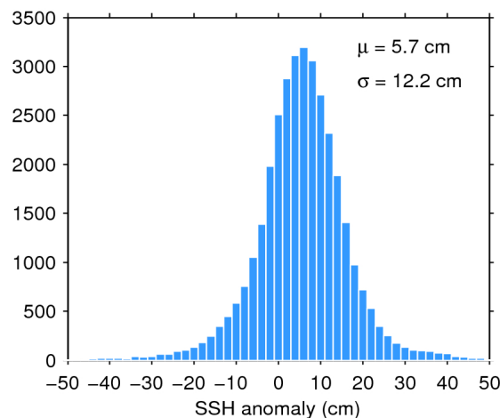
Figure 11. Histogram of science-valid SSH anomaly over oceans and lakes for 19/01/2020. The mean ( \mu ) and standard deviation ( \sigma ) are also shown. Note that values outside [-50 50] cm are excluded from the histogram for the sake of readability but not from the computation of \mu and \sigma .
