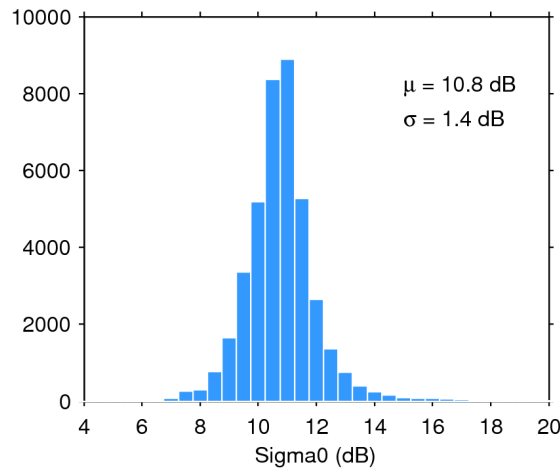
Figure 28. Histogram of science-valid sigma0 over oceans and lakes for 19/01/2020. The mean ( \mu ) and standard deviation ( \sigma ) are also shown. Note that values outside [4 20] dB are excluded from the histogram for the sake of readability but not from the computation of \mu and \sigma .
