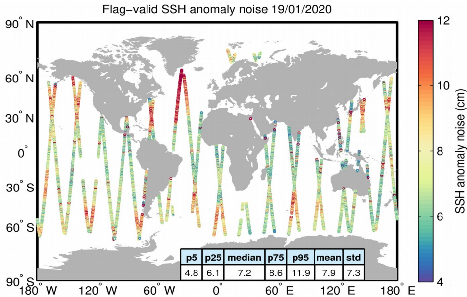
Figure 8. Geographical distribution of flag-valid 20-Hz SSH anomaly measurement noise over oceans and lakes for 19/01/2020. The statistical values shown in the table refer to the SSH anomaly noise and are calculated over all measurements shown in the figure.
