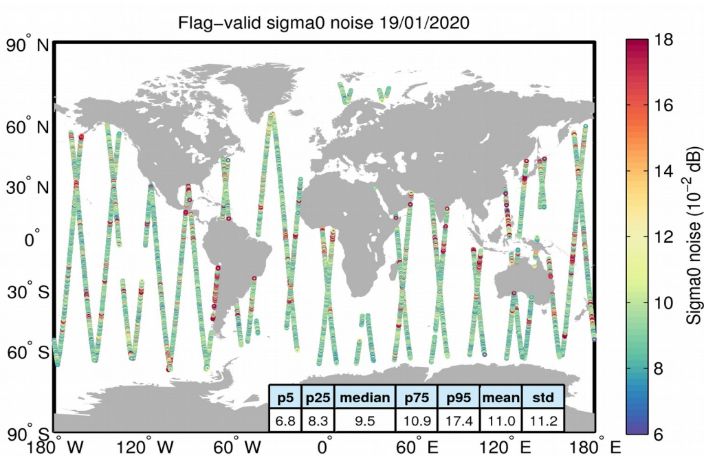
Figure 26. Geographical distribution of flag-valid 20-Hz sigma0 measurement noise over oceans and lakes for 19/01/2020. The statistical values shown in the table refer to the sigma0 noise and are calculated over all measurements shown in the figure.
