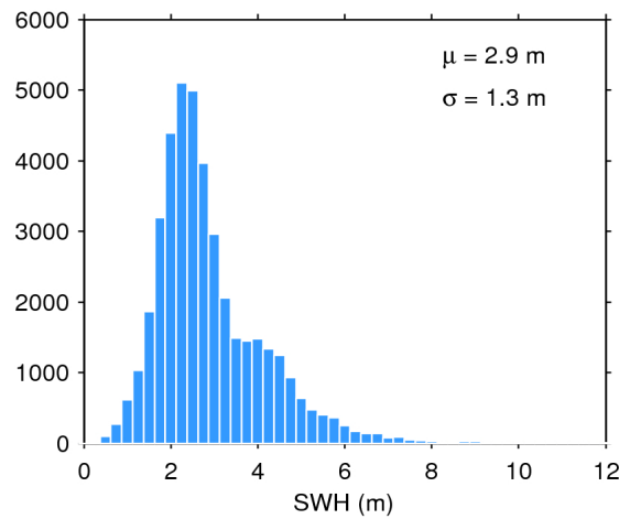
Figure 17. Histogram of flag-valid SWH over oceans and lakes for 19/01/2020. The mean ( \mu ) and standard deviation ( \sigma ) are also shown. Note that values larger than 12 m are excluded from the histogram for the sake of readability but not from the computation of \mu and \sigma .
