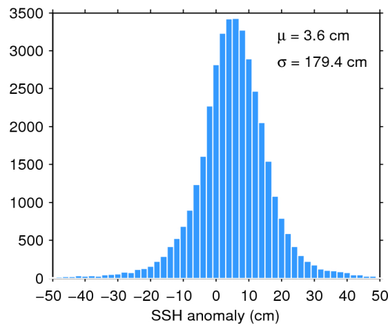
Figure 7. Histogram of flag-valid SSH anomaly over oceans and lakes for 19/01/2020. The mean ( \mu ) and standard deviation ( \sigma ) are also shown. Note that values outside [-50 50] cm are excluded from the histogram for the sake of readability but not from the computation of \mu and \sigma .
