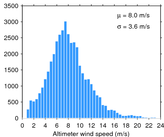
Figure 35. Histogram of science-valid wind over oceans and lakes for 19/01/2020. The mean ( \mu ) and standard deviation ( \sigma ) are also shown. Note that values larger than 24 m/s are excluded from the histogram for the sake of readability but not from the computation of \mu and \sigma .
