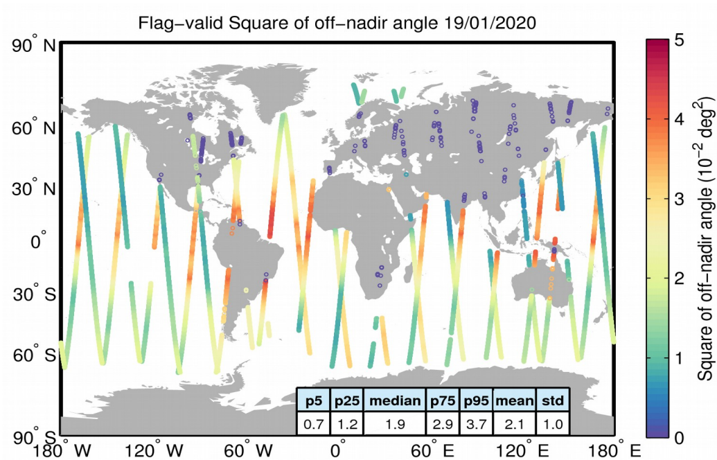
Figure 37. Geographical distribution of flag-valid mispointing data over oceans and lakes for 19/01/2020. The statistical values shown in the table refer to the mispointing in 10^{-2} deg 2 and are calculated over all measurements shown in the figure.
