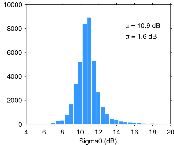
Figure 25. Histogram of flag-valid sigma0 over oceans and lakes for 19/01/2020. The mean ( \mu ) and standard deviation ( \sigma ) are also shown. Note that values outside [4 20] dB are excluded from the histogram for the sake of readability but not from the computation of \mu and \sigma .
