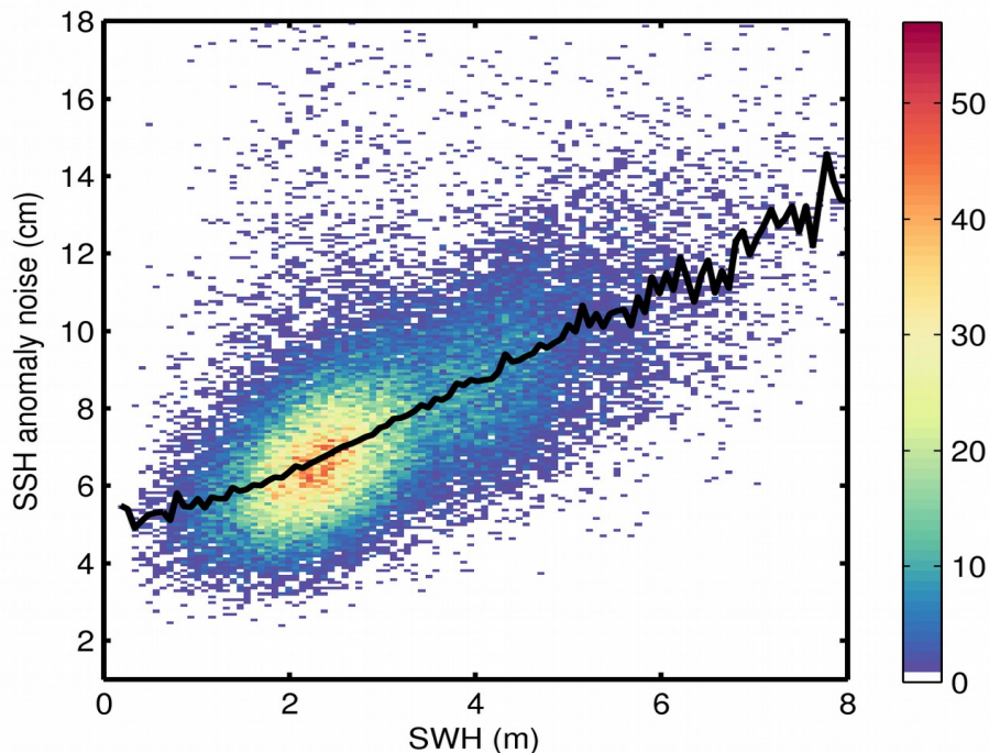
Figure 9. 2D histogram showing flag-valid SSH anomaly noise as a function of SWH for 19/01/2020. The black line denotes the median SSH anomaly noise as a function of SWH.
