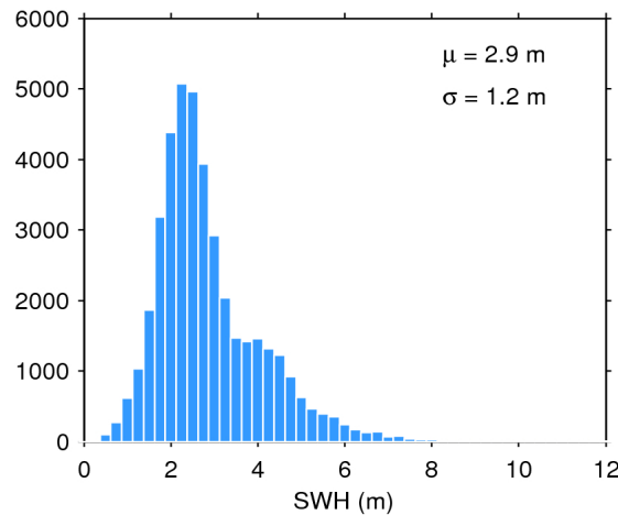
Figure 20. Histogram of science-valid SWH over oceans and lakes for 19/01/2020. The mean ( \mu ) and standard deviation ( \sigma ) are also shown. Note that values larger than 12 m are excluded from the histogram for the sake of readability but not from the computation of \mu and \sigma .
