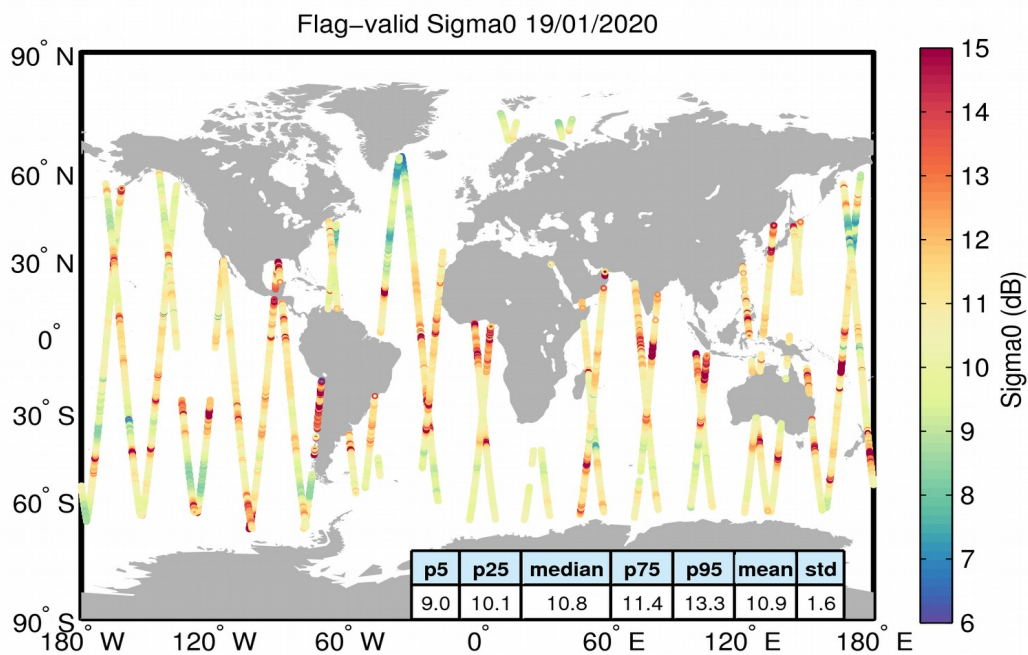
Figure 23. Geographical distribution of flag-valid sigma0 data over oceans and lakes for 19/01/2020. The statistical values shown in the table refer to the sigma0 in dB and are calculated over all measurements shown in the figure.
