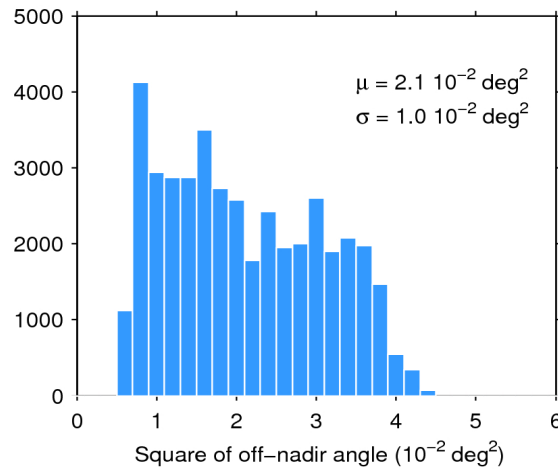
Figure 39. Histogram of flag-valid mispointing over oceans and lakes for 19/01/2020. The mean ( \mu ) and standard deviation ( \sigma ) are also shown. Note that values larger than 6 \cdot 10^{-2} \text{ deg}^2 are excluded from the histogram for the sake of readability but not from the computation of \mu and \sigma .
