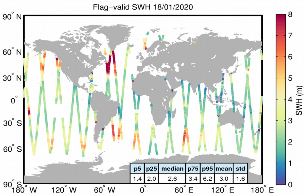
Figure 15. Geographical distribution of flag-valid SWH data over oceans and lakes for 18/01/2020. The statistical values shown in the table refer to the SWH in m and are calculated over all measurements shown in the figure.
