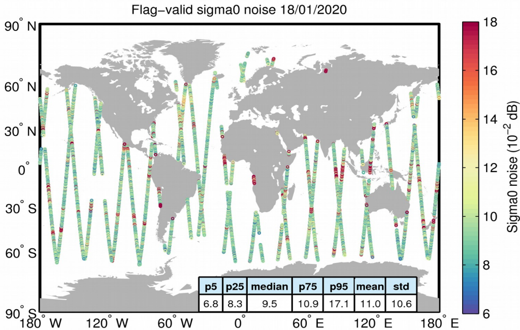
Figure 26. Geographical distribution of flag-valid 20-Hz sigma0 measurement noise over oceans and lakes for 18/01/2020. The statistical values shown in the table refer to the sigma0 noise and are calculated over all measurements shown in the figure.
