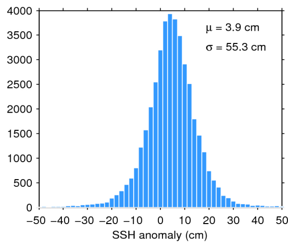
Figure 7. Histogram of flag-valid SSH anomaly over oceans and lakes for 18/01/2020. The mean ( \mu ) and standard deviation ( \sigma ) are also shown. Note that values outside [-50 50] cm are excluded from the histogram for the sake of readability but not from the computation of \mu and \sigma .
