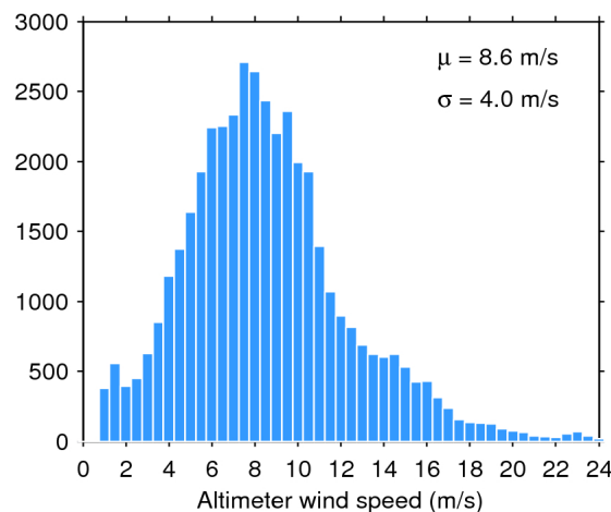
Figure 35. Histogram of science-valid wind over oceans and lakes for 18/01/2020. The mean ( \mu ) and standard deviation ( \sigma ) are also shown. Note that values larger than 24 m/s are excluded from the histogram for the sake of readability but not from the computation of \mu and \sigma .
