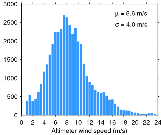
Figure 33. Histogram of flag-valid wind over oceans and lakes for 18/01/2020. The mean ( \mu ) and standard deviation ( \sigma ) are also shown. Note that values larger than 24 m/s are excluded from the histogram for the sake of readability but not from the computation of \mu and \sigma .
