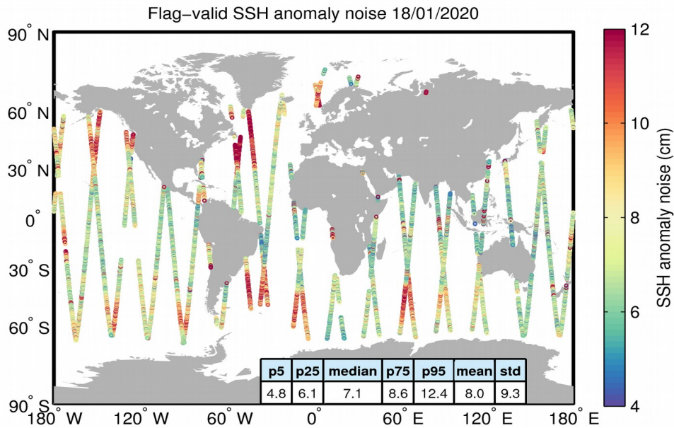
Figure 8. Geographical distribution of flag-valid 20-Hz SSH anomaly measurement noise over oceans and lakes for 18/01/2020. The statistical values shown in the table refer to the SSH anomaly noise and are calculated over all measurements shown in the figure.
