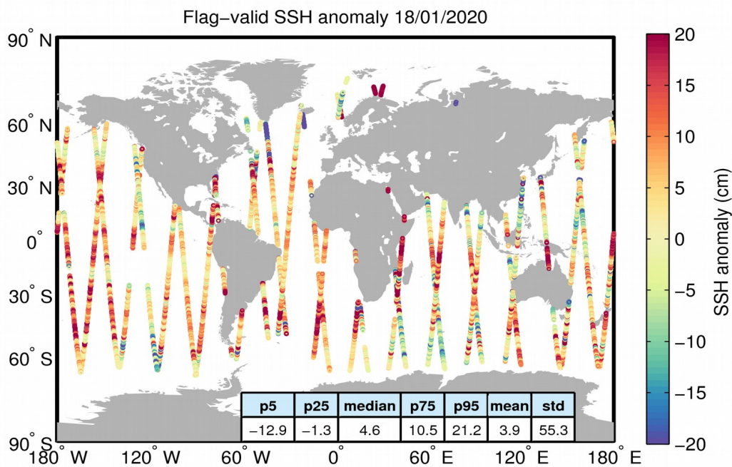
Figure 5. Geographical distribution of flag-valid 1-Hz SSH anomaly data over oceans and lakes for 18/01/2020. The statistical values shown in the table refer to the SSH anomaly in cm and are calculated over all measurements shown in the figure.
