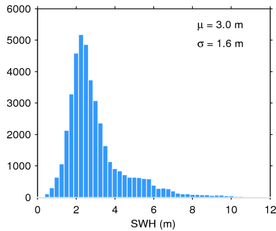
Figure 17. Histogram of flag-valid SWH over oceans and lakes for 18/01/2020. The mean ( \mu ) and standard deviation ( \sigma ) are also shown. Note that values larger than 12 m are excluded from the histogram for the sake of readability but not from the computation of \mu and \sigma .
