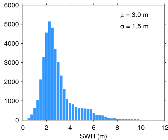
Figure 20. Histogram of science-valid SWH over oceans and lakes for 18/01/2020. The mean ( \mu ) and standard deviation ( \sigma ) are also shown. Note that values larger than 12 m are excluded from the histogram for the sake of readability but not from the computation of \mu and \sigma .
