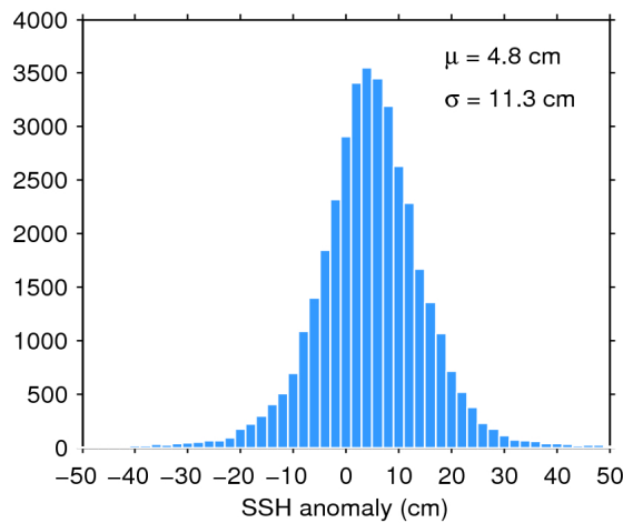
Figure 11. Histogram of science-valid SSH anomaly over oceans and lakes for 18/01/2020. The mean ( \mu ) and standard deviation ( \sigma ) are also shown. Note that values outside [-50 50] cm are excluded from the histogram for the sake of readability but not from the computation of \mu and \sigma .
