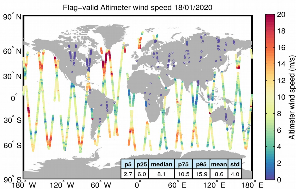
Figure 31. Geographical distribution of flag-valid wind data over oceans and lakes for 18/01/2020. The statistical values shown in the table refer to the wind in m/s and are calculated over all measurements shown in the figure.
