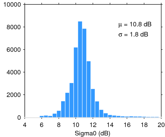
Figure 25. Histogram of flag-valid sigma0 over oceans and lakes for 18/01/2020. The mean ( \mu ) and standard deviation ( \sigma ) are also shown. Note that values outside [4 20] dB are excluded from the histogram for the sake of readability but not from the computation of \mu and \sigma .
