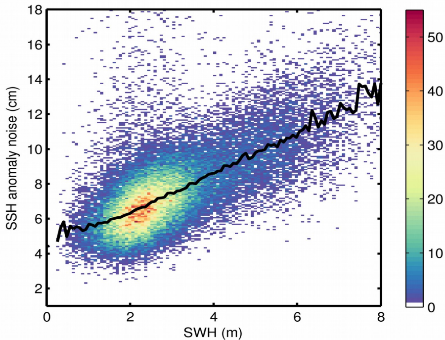
Figure 9. 2D histogram showing flag-valid SSH anomaly noise as a function of SWH for 18/01/2020. The black line denotes the median SSH anomaly noise as a function of SWH.
