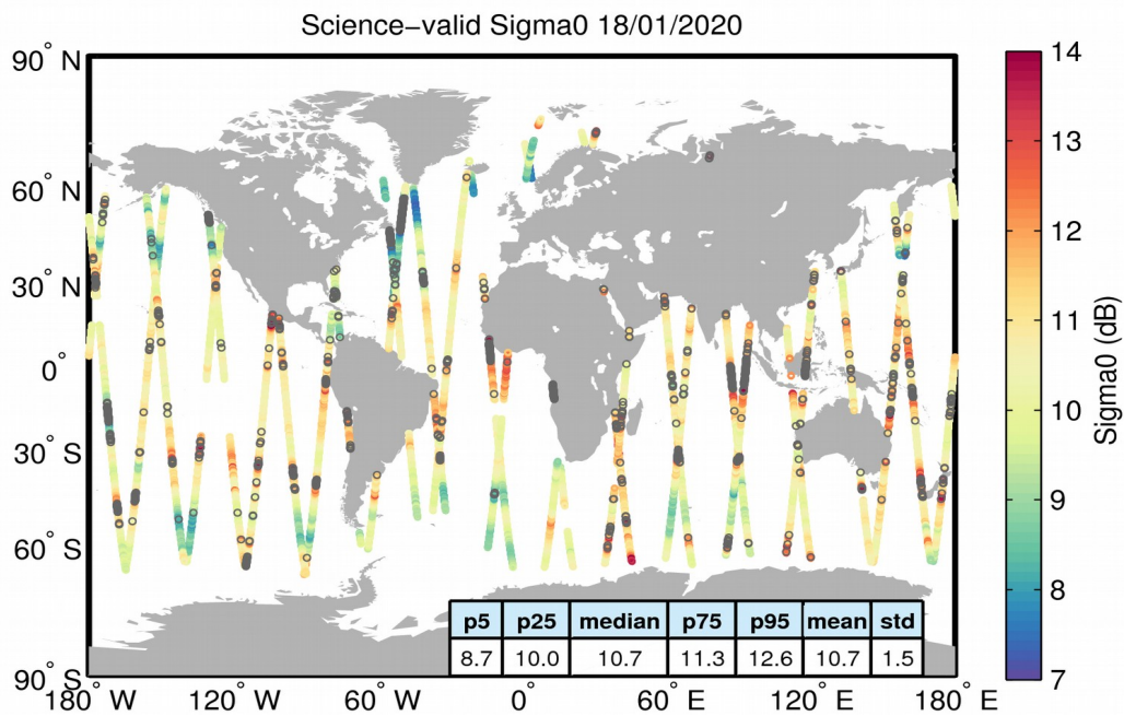
Figure 27. Geographical distribution of science-valid sigma0 data over oceans and lakes for 18/01/2020. The statistical values shown in the table refer to the sigma0 in dB and are calculated over all measurements shown in the figure. Gray circles denote records that have been rejected based on the editing criteria described in Table 4.
