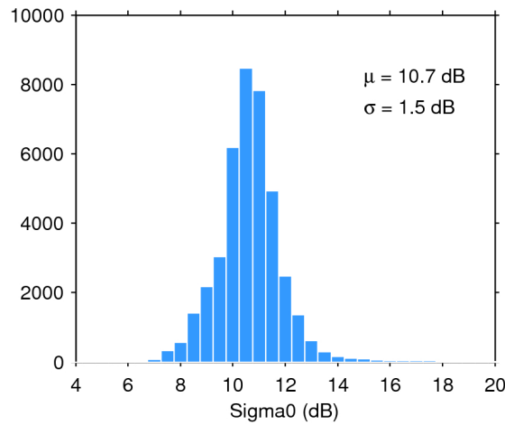
Figure 28. Histogram of science-valid sigma0 over oceans and lakes for 18/01/2020. The mean ( \mu ) and standard deviation ( \sigma ) are also shown. Note that values outside [4 20] dB are excluded from the histogram for the sake of readability but not from the computation of \mu and \sigma .
