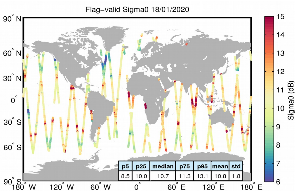
Figure 23. Geographical distribution of flag-valid sigma0 data over oceans and lakes for 18/01/2020. The statistical values shown in the table refer to the sigma0 in dB and are calculated over all measurements shown in the figure.
