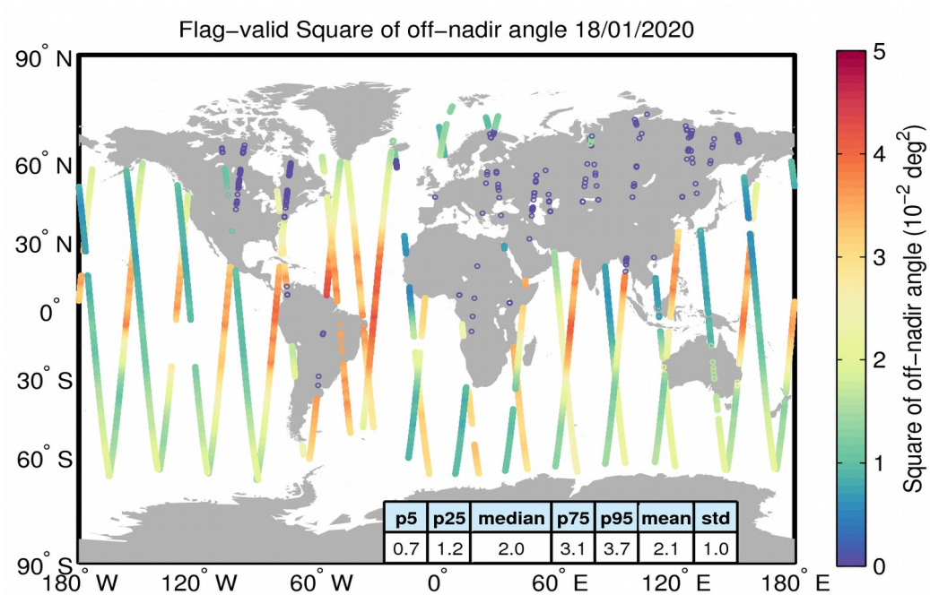
Figure 37. Geographical distribution of flag-valid mispointing data over oceans and lakes for 18/01/2020. The statistical values shown in the table refer to the mispointing in 10^{-2} deg 2 and are calculated over all measurements shown in the figure.
