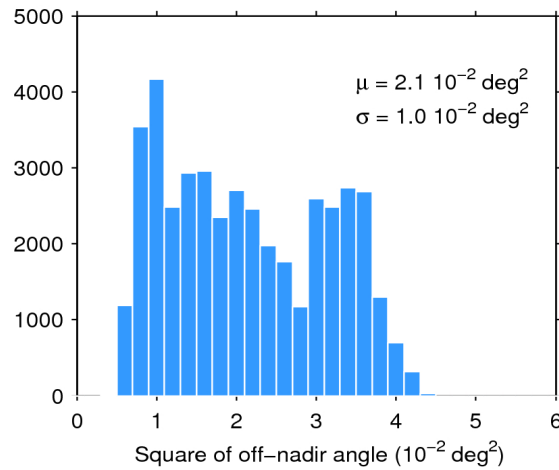
Figure 39. Histogram of flag-valid mispointing over oceans and lakes for 18/01/2020. The mean ( \mu ) and standard deviation ( \sigma ) are also shown. Note that values larger than 6 \cdot 10^{-2} \text{ deg}^2 are excluded from the histogram for the sake of readability but not from the computation of \mu and \sigma .
