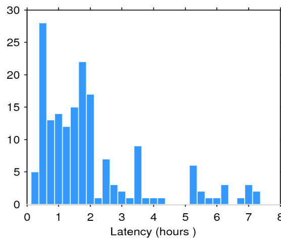
Figure 2. Histogram of the data latency for 18/01/2020. The y-axis denotes the number of files that are made available with a delay of x-hours with respect to the mean time of the records stored in the file.
