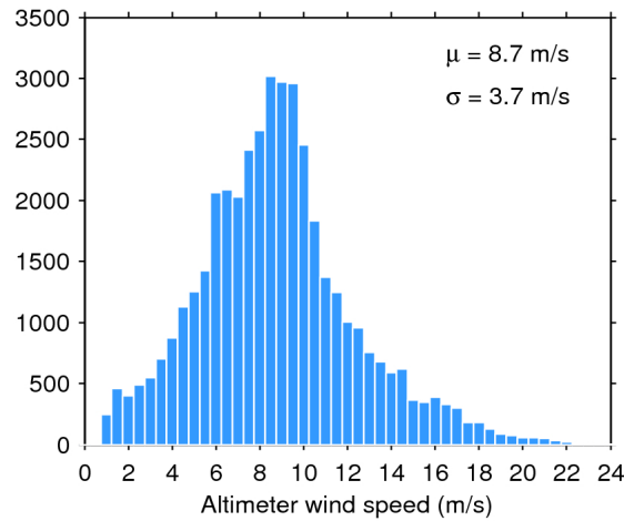
Figure 33. Histogram of flag-valid wind over oceans and lakes for 17/01/2020. The mean ( \mu ) and standard deviation ( \sigma ) are also shown. Note that values larger than 24 m/s are excluded from the histogram for the sake of readability but not from the computation of \mu and \sigma .
