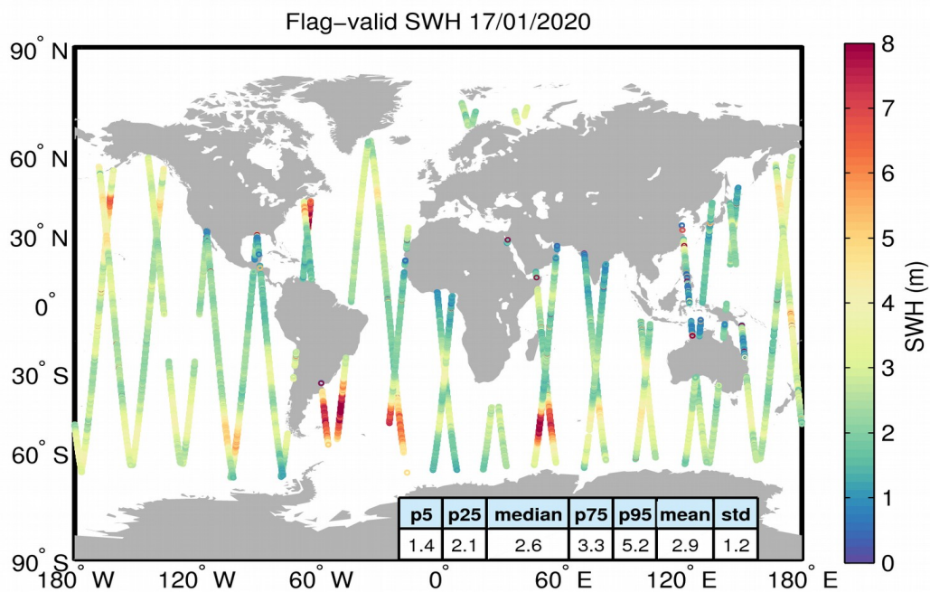
Figure 15. Geographical distribution of flag-valid SWH data over oceans and lakes for 17/01/2020. The statistical values shown in the table refer to the SWH in m and are calculated over all measurements shown in the figure.
