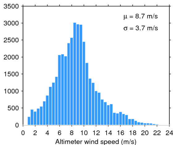
Figure 35. Histogram of science-valid wind over oceans and lakes for 17/01/2020. The mean ( \mu ) and standard deviation ( \sigma ) are also shown. Note that values larger than 24 m/s are excluded from the histogram for the sake of readability but not from the computation of \mu and \sigma .
