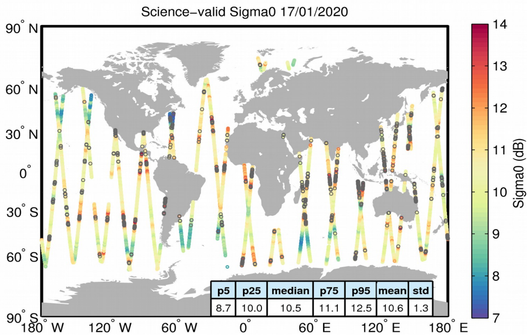
Figure 27. Geographical distribution of science-valid sigma0 data over oceans and lakes for 17/01/2020. The statistical values shown in the table refer to the sigma0 in dB and are calculated over all measurements shown in the figure. Gray circles denote records that have been rejected based on the editing criteria described in Table 4.
