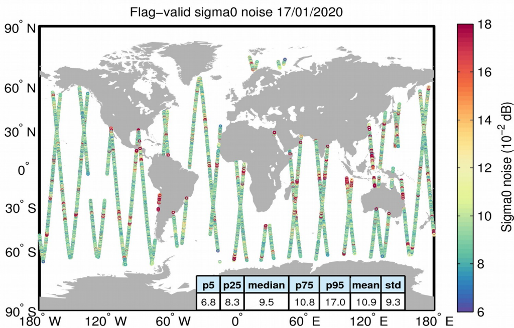
Figure 26. Geographical distribution of flag-valid 20-Hz sigma0 measurement noise over oceans and lakes for 17/01/2020. The statistical values shown in the table refer to the sigma0 noise and are calculated over all measurements shown in the figure.
