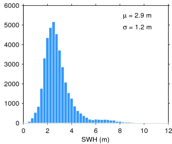
Figure 17. Histogram of flag-valid SWH over oceans and lakes for 17/01/2020. The mean ( \mu ) and standard deviation ( \sigma ) are also shown. Note that values larger than 12 m are excluded from the histogram for the sake of readability but not from the computation of \mu and \sigma .
