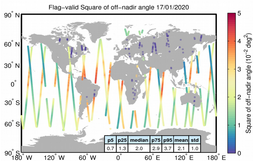
Figure 37. Geographical distribution of flag-valid mispointing data over oceans and lakes for 17/01/2020. The statistical values shown in the table refer to the mispointing in 10^{-2} deg 2 and are calculated over all measurements shown in the figure.
