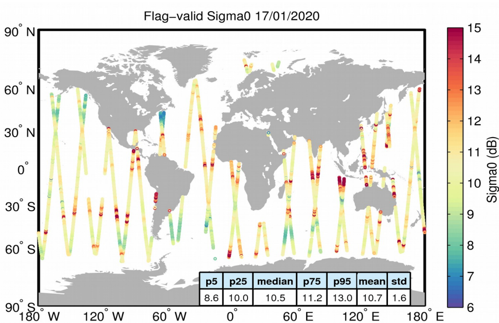
Figure 23. Geographical distribution of flag-valid sigma0 data over oceans and lakes for 17/01/2020. The statistical values shown in the table refer to the sigma0 in dB and are calculated over all measurements shown in the figure.
