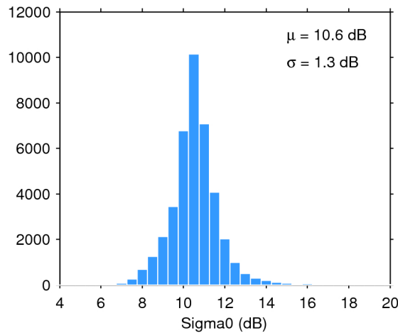
Figure 28. Histogram of science-valid sigma0 over oceans and lakes for 17/01/2020. The mean ( \mu ) and standard deviation ( \sigma ) are also shown. Note that values outside [4 20] dB are excluded from the histogram for the sake of readability but not from the computation of \mu and \sigma .
