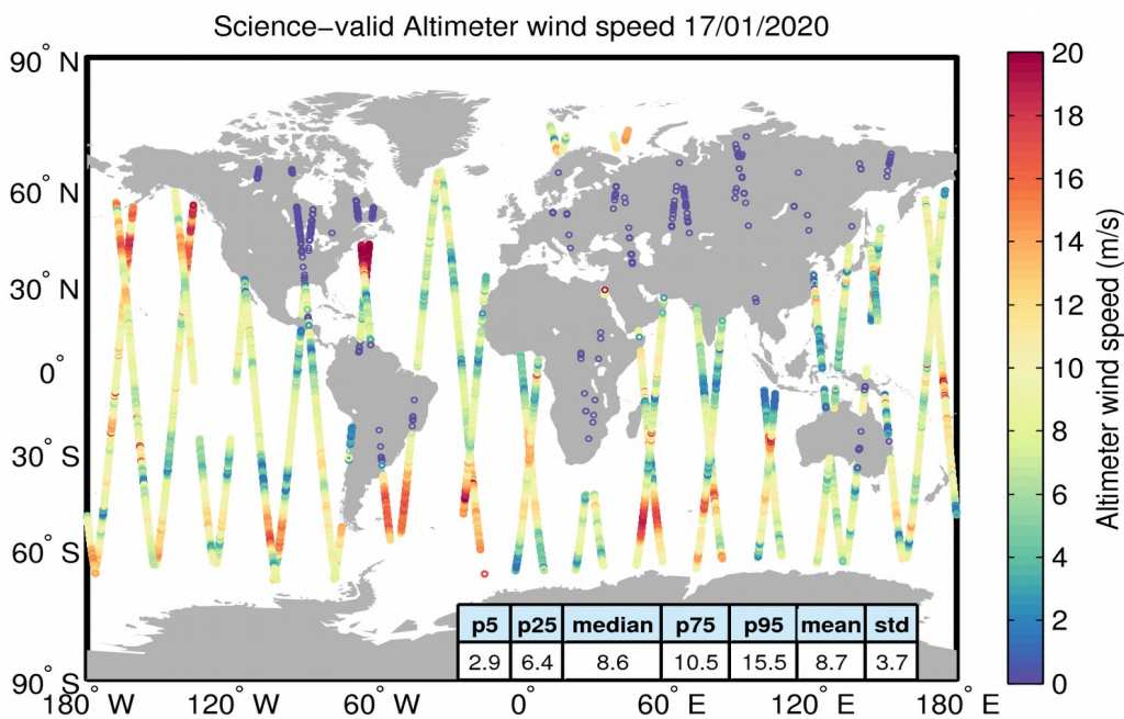
Figure 34. Geographical distribution of science-valid wind data over oceans and lakes for 17/01/2020. The statistical values shown in the table refer to the wind in m/s and are calculated over all measurements shown in the figure. Gray circles denote records that have been rejected based on the editing criteria described in Table 5.
