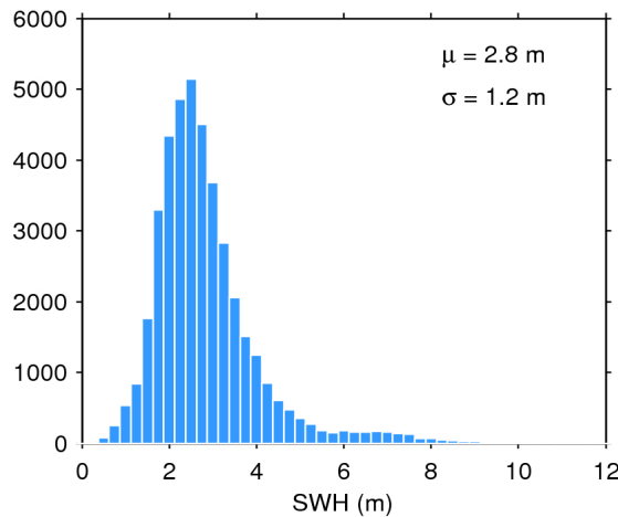
Figure 20. Histogram of science-valid SWH over oceans and lakes for 17/01/2020. The mean ( \mu ) and standard deviation ( \sigma ) are also shown. Note that values larger than 12 m are excluded from the histogram for the sake of readability but not from the computation of \mu and \sigma .
