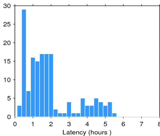
Figure 2. Histogram of the data latency for 17/01/2020. The y-axis denotes the number of files that are made available with a delay of x-hours with respect to the mean time of the records stored in the file.
