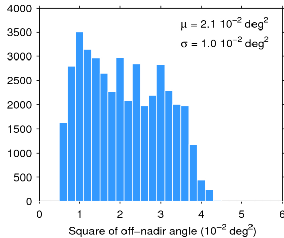
Figure 39. Histogram of flag-valid mispointing over oceans and lakes for 17/01/2020. The mean ( \mu ) and standard deviation ( \sigma ) are also shown. Note that values larger than 6 \cdot 10^{-2} \text{ deg}^2 are excluded from the histogram for the sake of readability but not from the computation of \mu and \sigma .
