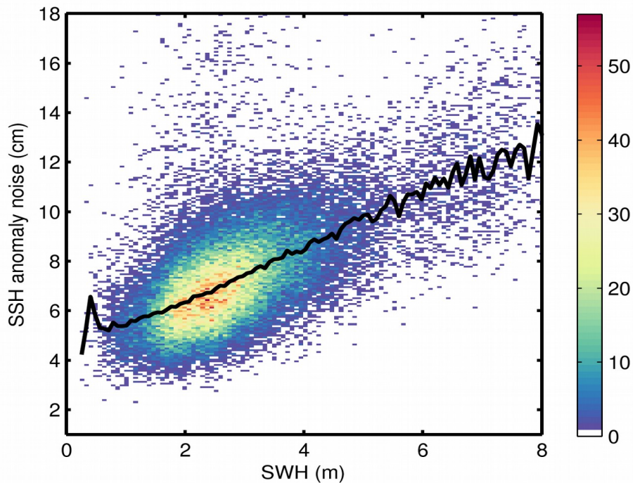
Figure 9. 2D histogram showing flag-valid SSH anomaly noise as a function of SWH for 17/01/2020. The black line denotes the median SSH anomaly noise as a function of SWH.
