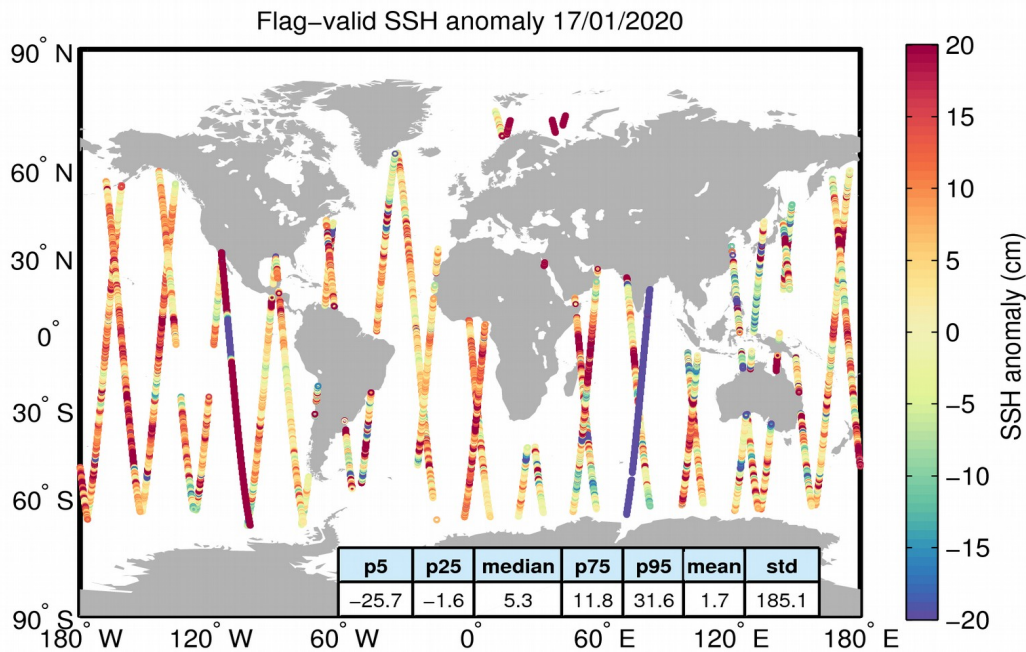
Figure 5. Geographical distribution of flag-valid 1-Hz SSH anomaly data over oceans and lakes for 17/01/2020. The statistical values shown in the table refer to the SSH anomaly in cm and are calculated over all measurements shown in the figure.
