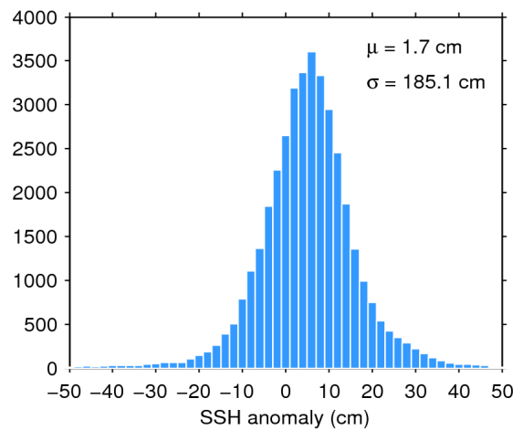
Figure 7. Histogram of flag-valid SSH anomaly over oceans and lakes for 17/01/2020. The mean ( \mu ) and standard deviation ( \sigma ) are also shown. Note that values outside [-50\ 50] cm are excluded from the histogram for the sake of readability but not from the computation of \mu and \sigma .
