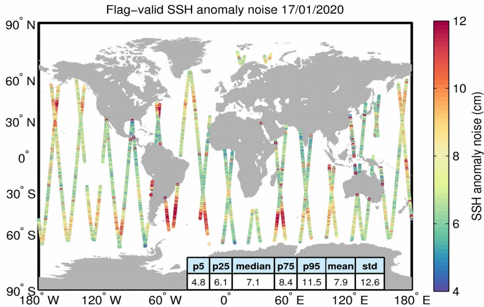
Figure 8. Geographical distribution of flag-valid 20-Hz SSH anomaly measurement noise over oceans and lakes for 17/01/2020. The statistical values shown in the table refer to the SSH anomaly noise and are calculated over all measurements shown in the figure.
