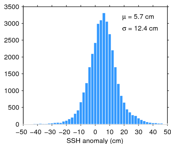
Figure 11. Histogram of science-valid SSH anomaly over oceans and lakes for 17/01/2020. The mean ( \mu ) and standard deviation ( \sigma ) are also shown. Note that values outside [-50 50] cm are excluded from the histogram for the sake of readability but not from the computation of \mu and \sigma .
