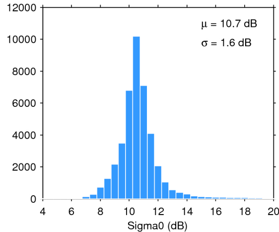
Figure 25. Histogram of flag-valid sigma0 over oceans and lakes for 17/01/2020. The mean ( \mu ) and standard deviation ( \sigma ) are also shown. Note that values outside [4 20] dB are excluded from the histogram for the sake of readability but not from the computation of \mu and \sigma .
