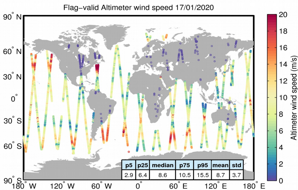
Figure 31. Geographical distribution of flag-valid wind data over oceans and lakes for 17/01/2020. The statistical values shown in the table refer to the wind in m/s and are calculated over all measurements shown in the figure.
