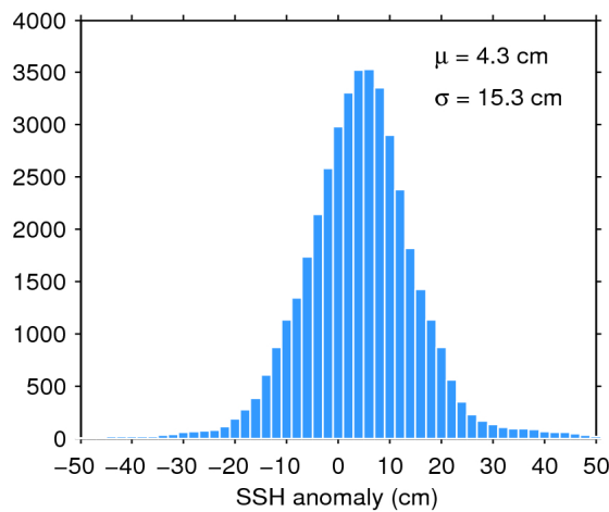
Figure 7. Histogram of flag-valid SSH anomaly over oceans and lakes for 16/01/2020. The mean ( \mu ) and standard deviation ( \sigma ) are also shown. Note that values outside [-50\ 50] cm are excluded from the histogram for the sake of readability but not from the computation of \mu and \sigma .
