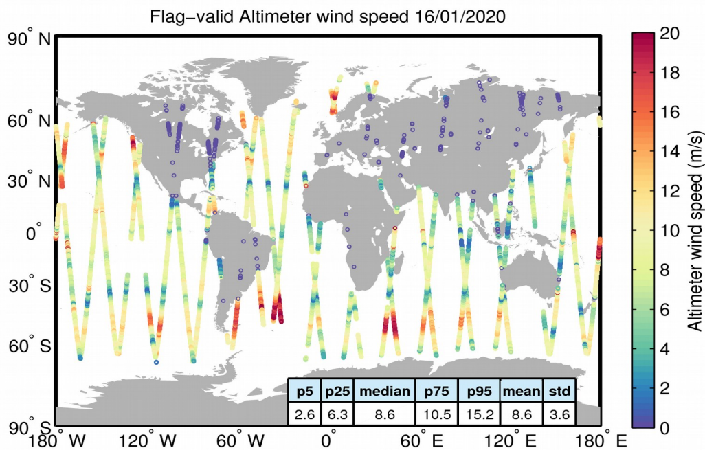
Figure 31. Geographical distribution of flag-valid wind data over oceans and lakes for 16/01/2020. The statistical values shown in the table refer to the wind in m/s and are calculated over all measurements shown in the figure.
