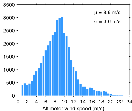
Figure 35. Histogram of science-valid wind over oceans and lakes for 16/01/2020. The mean ( \mu ) and standard deviation ( \sigma ) are also shown. Note that values larger than 24 m/s are excluded from the histogram for the sake of readability but not from the computation of \mu and \sigma .
