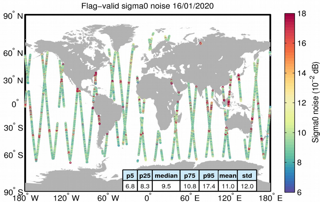
Figure 26. Geographical distribution of flag-valid 20-Hz sigma0 measurement noise over oceans and lakes for 16/01/2020. The statistical values shown in the table refer to the sigma0 noise and are calculated over all measurements shown in the figure.
