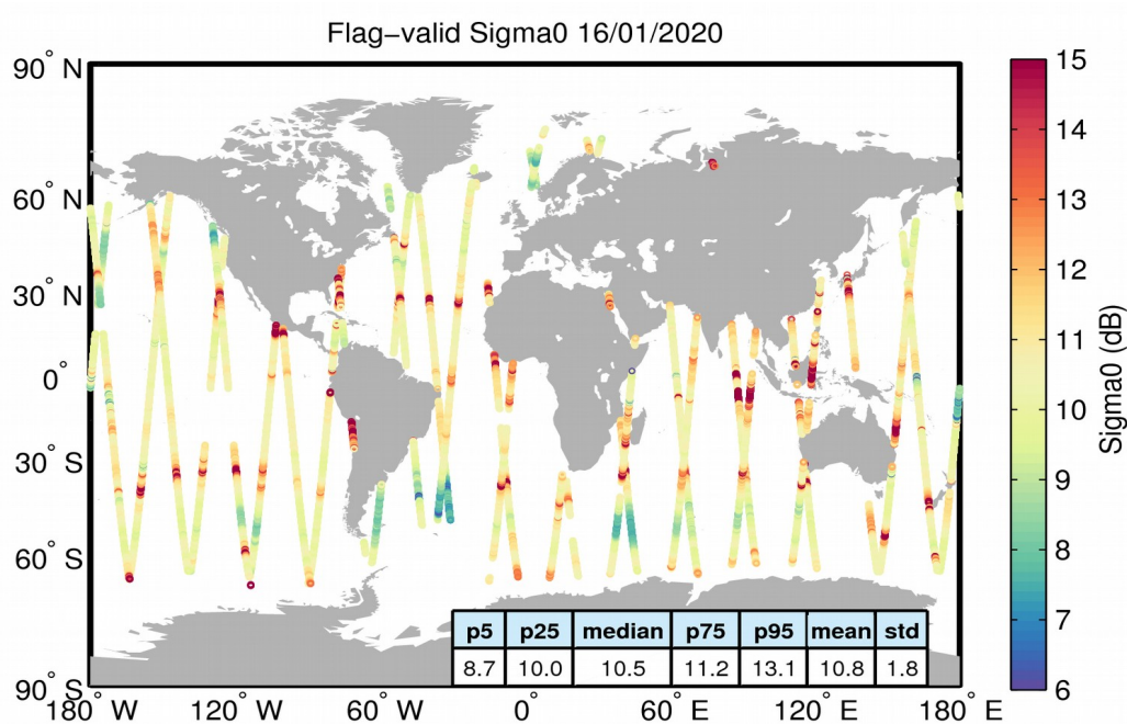
Figure 23. Geographical distribution of flag-valid sigma0 data over oceans and lakes for 16/01/2020. The statistical values shown in the table refer to the sigma0 in dB and are calculated over all measurements shown in the figure.
