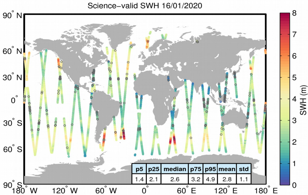
Figure 19. Geographical distribution of science-valid SWH data over oceans and lakes for 16/01/2020. The statistical values shown in the table refer to the SWH in m and are calculated over all measurements shown in the figure. Gray circles denote records that have been rejected based on the editing criteria described in Table 3.
