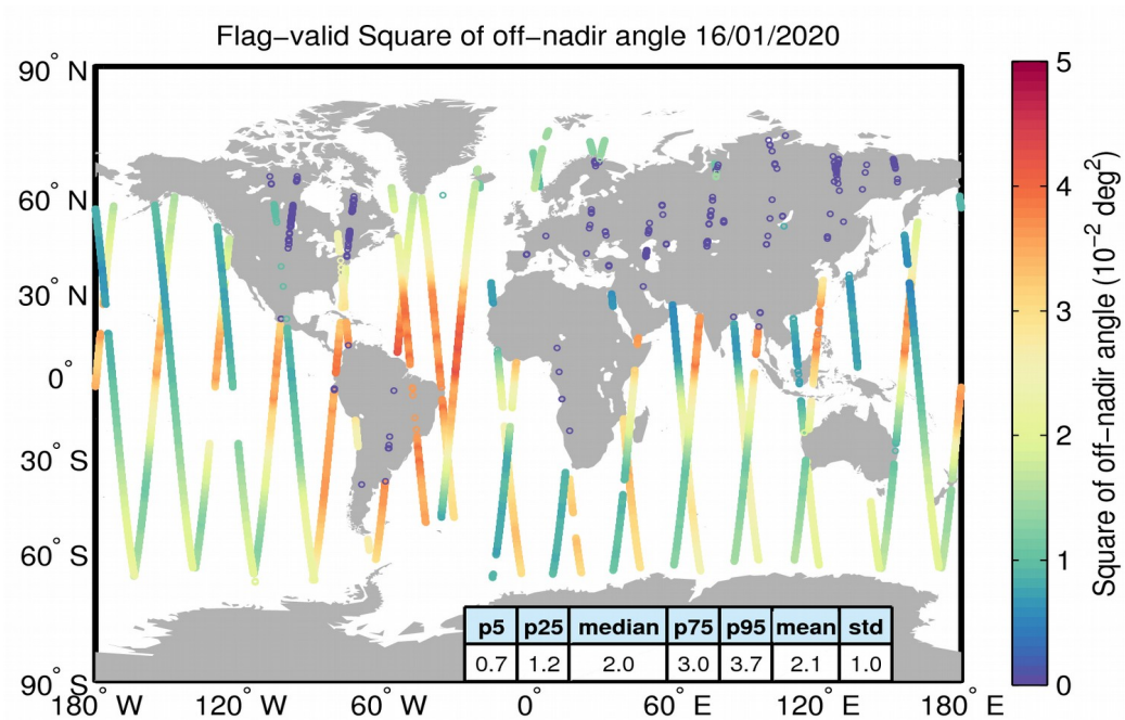
Figure 37. Geographical distribution of flag-valid mispointing data over oceans and lakes for 16/01/2020. The statistical values shown in the table refer to the mispointing in 10^{-2} \text{deg}^2 and are calculated over all measurements shown in the figure.
