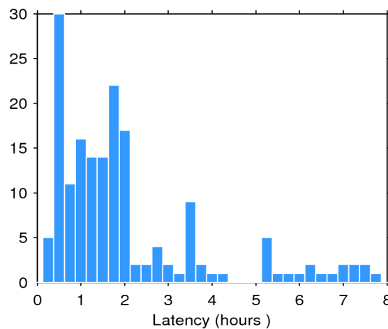
Figure 2. Histogram of the data latency for 16/01/2020. The y-axis denotes the number of files that are made available with a delay of x-hours with respect to the mean time of the records stored in the file.
