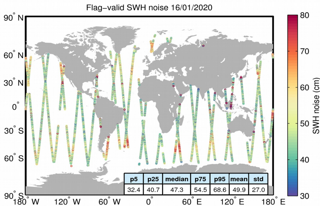
Figure 18. Geographical distribution of flag-valid 20-Hz SWH measurement noise over oceans and lakes for 16/01/2020. The statistical values shown in the figure refer to the SWH noise and are calculated over all measurements shown in the figure.
