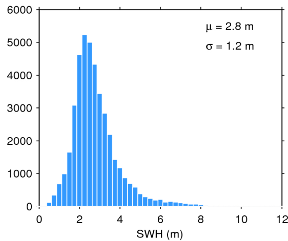
Figure 17. Histogram of flag-valid SWH over oceans and lakes for 16/01/2020. The mean ( \mu ) and standard deviation ( \sigma ) are also shown. Note that values larger than 12 m are excluded from the histogram for the sake of readability but not from the computation of \mu and \sigma .
