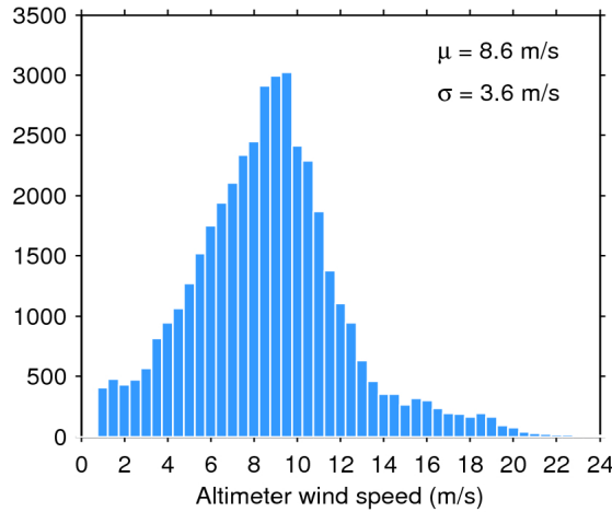
Figure 33. Histogram of flag-valid wind over oceans and lakes for 16/01/2020. The mean ( \mu ) and standard deviation ( \sigma ) are also shown. Note that values larger than 24 m/s are excluded from the histogram for the sake of readability but not from the computation of \mu and \sigma .
