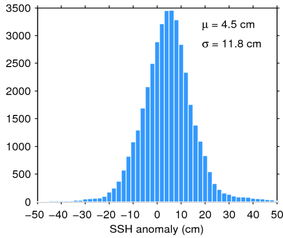
Figure 11. Histogram of science-valid SSH anomaly over oceans and lakes for 16/01/2020. The mean ( \mu ) and standard deviation ( \sigma ) are also shown. Note that values outside [-50 50] cm are excluded from the histogram for the sake of readability but not from the computation of \mu and \sigma .
