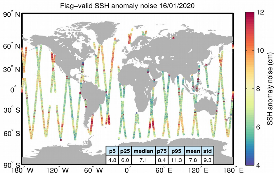
Figure 8. Geographical distribution of flag-valid 20-Hz SSH anomaly measurement noise over oceans and lakes for 16/01/2020. The statistical values shown in the table refer to the SSH anomaly noise and are calculated over all measurements shown in the figure.
