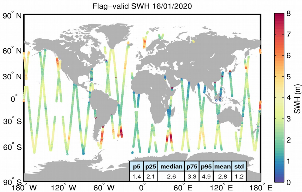
Figure 15. Geographical distribution of flag-valid SWH data over oceans and lakes for 16/01/2020. The statistical values shown in the table refer to the SWH in m and are calculated over all measurements shown in the figure.
