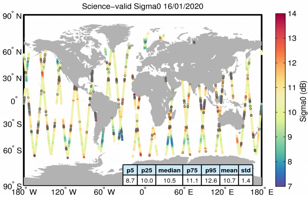
Figure 27. Geographical distribution of science-valid sigma0 data over oceans and lakes for 16/01/2020. The statistical values shown in the table refer to the sigma0 in dB and are calculated over all measurements shown in the figure. Gray circles denote records that have been rejected based on the editing criteria described in Table 4.
