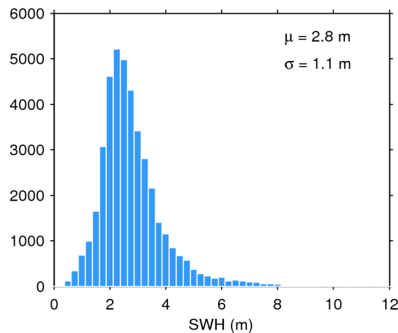
Figure 20. Histogram of science-valid SWH over oceans and lakes for 16/01/2020. The mean ( \mu ) and standard deviation ( \sigma ) are also shown. Note that values larger than 12 m are excluded from the histogram for the sake of readability but not from the computation of \mu and \sigma .
