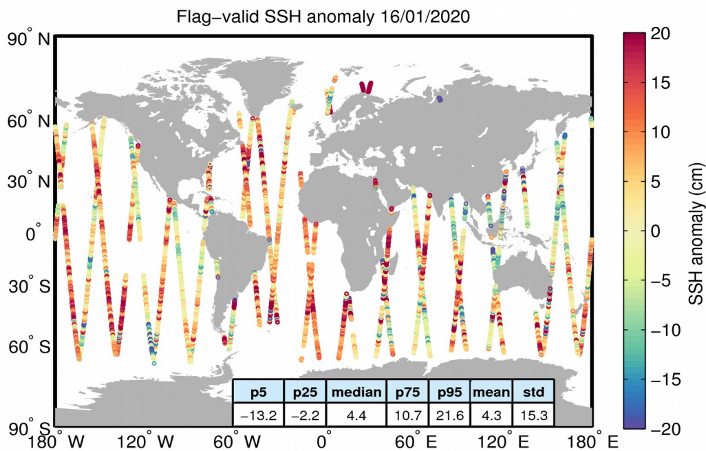
Figure 5. Geographical distribution of flag-valid 1-Hz SSH anomaly data over oceans and lakes for 16/01/2020. The statistical values shown in the table refer to the SSH anomaly in cm and are calculated over all measurements shown in the figure.
