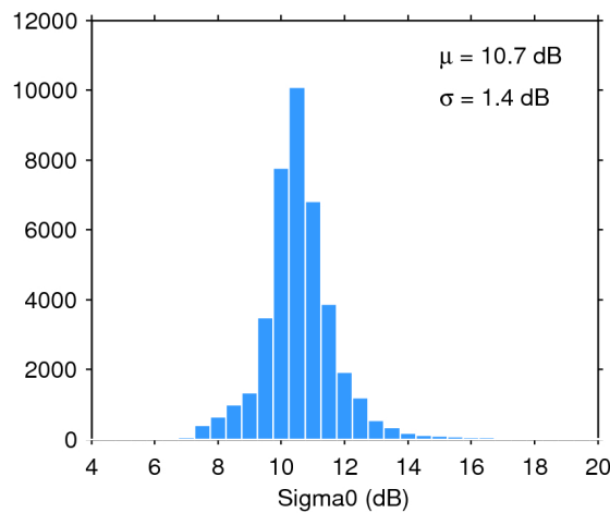
Figure 28. Histogram of science-valid sigma0 over oceans and lakes for 16/01/2020. The mean ( \mu ) and standard deviation ( \sigma ) are also shown. Note that values outside [4 20] dB are excluded from the histogram for the sake of readability but not from the computation of \mu and \sigma .
