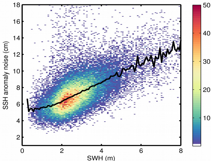
Figure 9. 2D histogram showing flag-valid SSH anomaly noise as a function of SWH for 16/01/2020. The black line denotes the median SSH anomaly noise as a function of SWH.
