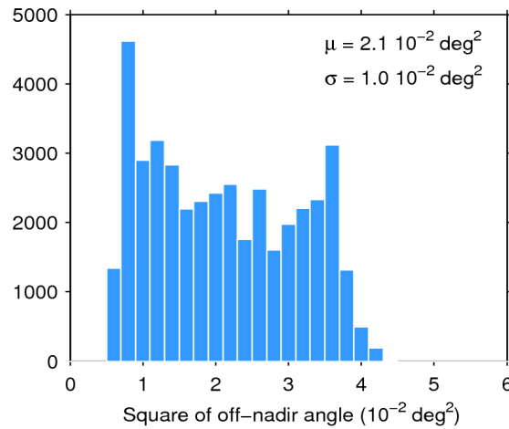
Figure 39. Histogram of flag-valid mispointing over oceans and lakes for 16/01/2020. The mean ( \mu ) and standard deviation ( \sigma ) are also shown. Note that values larger than 6 \cdot 10^{-2} \text{ deg}^2 are excluded from the histogram for the sake of readability but not from the computation of \mu and \sigma .
