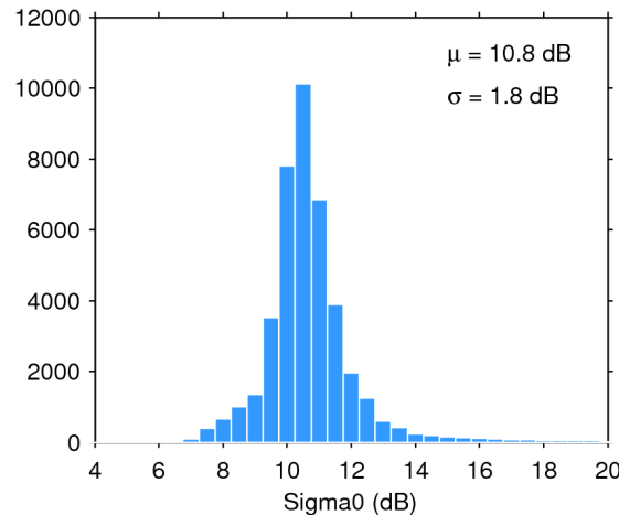
Figure 25. Histogram of flag-valid sigma0 over oceans and lakes for 16/01/2020. The mean ( \mu ) and standard deviation ( \sigma ) are also shown. Note that values outside [4 20] dB are excluded from the histogram for the sake of readability but not from the computation of \mu and \sigma .
