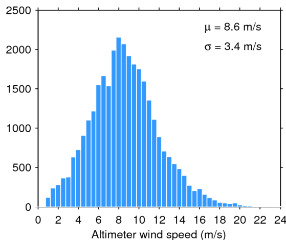
Figure 35. Histogram of science-valid wind over oceans and lakes for 15/01/2020. The mean ( \mu ) and standard deviation ( \sigma ) are also shown. Note that values larger than 24 m/s are excluded from the histogram for the sake of readability but not from the computation of \mu and \sigma .
