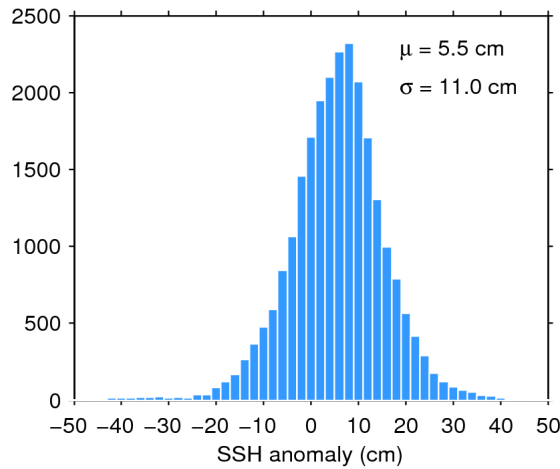
Figure 11. Histogram of science-valid SSH anomaly over oceans and lakes for 15/01/2020. The mean ( \mu ) and standard deviation ( \sigma ) are also shown. Note that values outside [-50 50] cm are excluded from the histogram for the sake of readability but not from the computation of \mu and \sigma .
