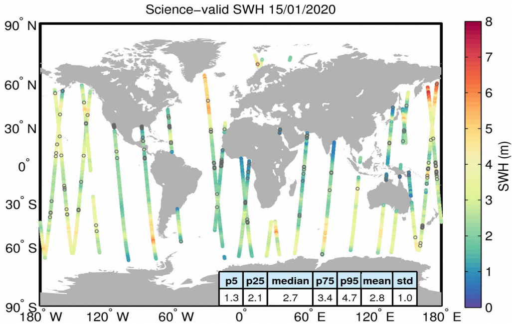
Figure 19. Geographical distribution of science-valid SWH data over oceans and lakes for 15/01/2020. The statistical values shown in the table refer to the SWH in m and are calculated over all measurements shown in the figure. Gray circles denote records that have been rejected based on the editing criteria described in Table 3.
