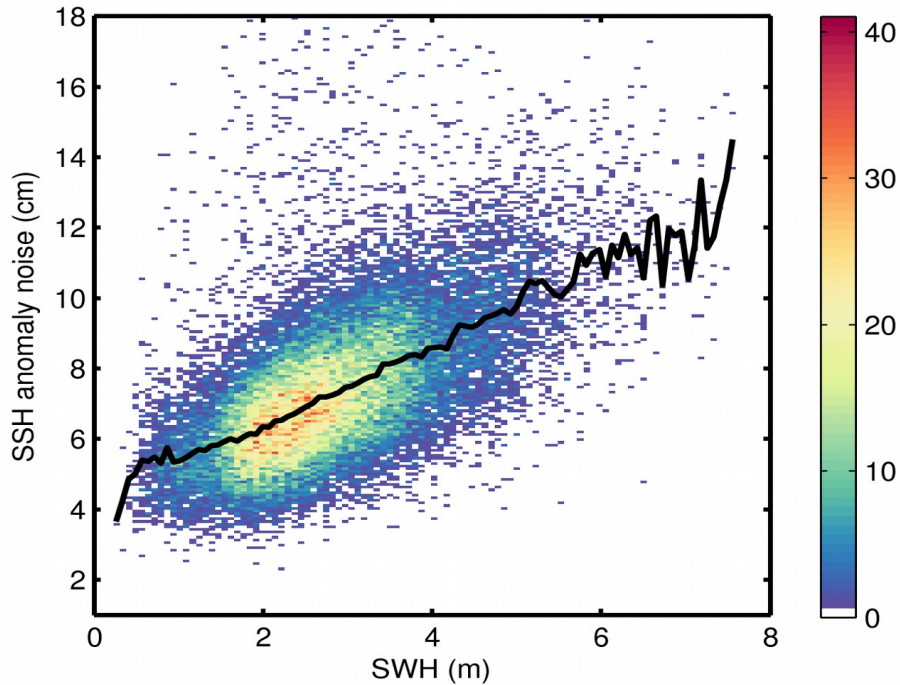
Figure 9. 2D histogram showing flag-valid SSH anomaly noise as a function of SWH for 15/01/2020. The black line denotes the median SSH anomaly noise as a function of SWH.
