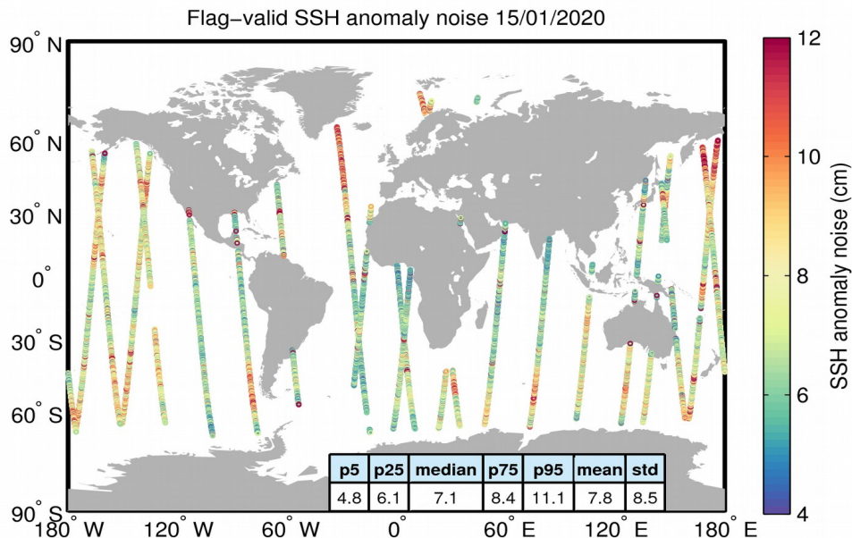
Figure 8. Geographical distribution of flag-valid 20-Hz SSH anomaly measurement noise over oceans and lakes for 15/01/2020. The statistical values shown in the table refer to the SSH anomaly noise and are calculated over all measurements shown in the figure.
