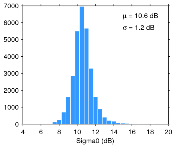
Figure 28. Histogram of science-valid sigma0 over oceans and lakes for 15/01/2020. The mean ( \mu ) and standard deviation ( \sigma ) are also shown. Note that values outside [4 20] dB are excluded from the histogram for the sake of readability but not from the computation of \mu and \sigma .
