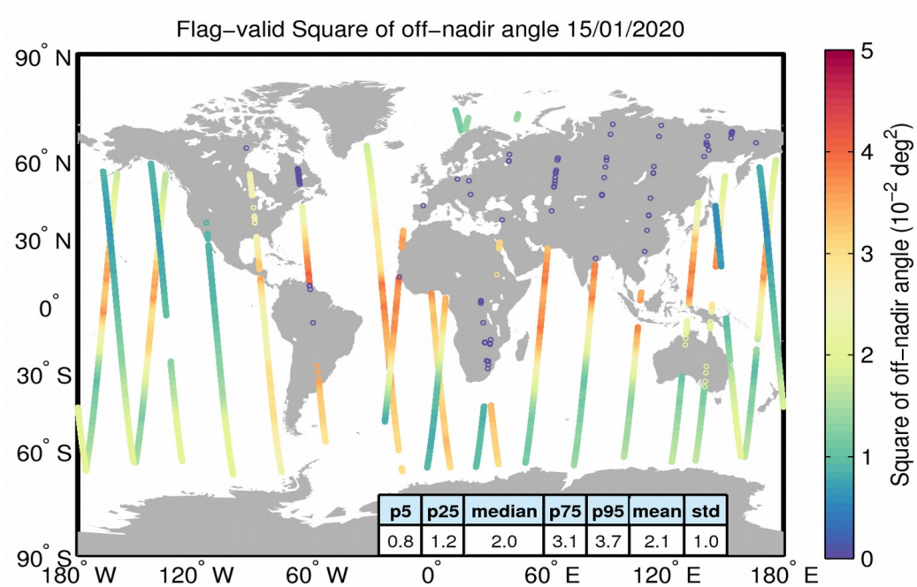
Figure 37. Geographical distribution of flag-valid mispointing data over oceans and lakes for 15/01/2020. The statistical values shown in the table refer to the mispointing in 10^{-2} \text{deg}^2 and are calculated over all measurements shown in the figure.
