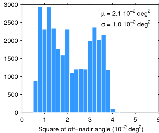
Figure 39. Histogram of flag-valid mispointing over oceans and lakes for 15/01/2020. The mean ( \mu ) and standard deviation ( \sigma ) are also shown. Note that values larger than 6 \cdot 10^{-2} \text{ deg}^2 are excluded from the histogram for the sake of readability but not from the computation of \mu and \sigma .
