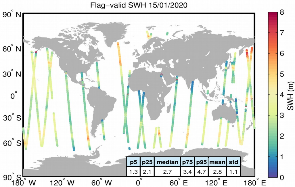
Figure 15. Geographical distribution of flag-valid SWH data over oceans and lakes for 15/01/2020. The statistical values shown in the table refer to the SWH in m and are calculated over all measurements shown in the figure.
