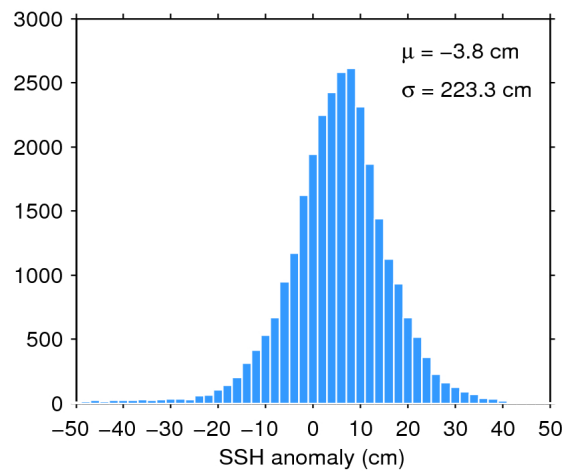
Figure 7. Histogram of flag-valid SSH anomaly over oceans and lakes for 15/01/2020. The mean ( \mu ) and standard deviation ( \sigma ) are also shown. Note that values outside [-50\ 50] cm are excluded from the histogram for the sake of readability but not from the computation of \mu and \sigma .
