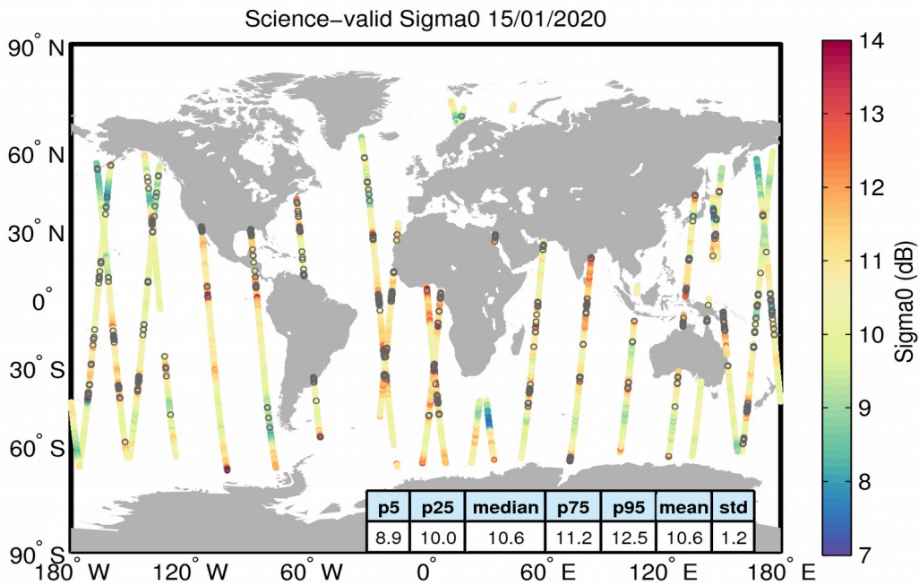
Figure 27. Geographical distribution of science-valid sigma0 data over oceans and lakes for 15/01/2020. The statistical values shown in the table refer to the sigma0 in dB and are calculated over all measurements shown in the figure. Gray circles denote records that have been rejected based on the editing criteria described in Table 4.
