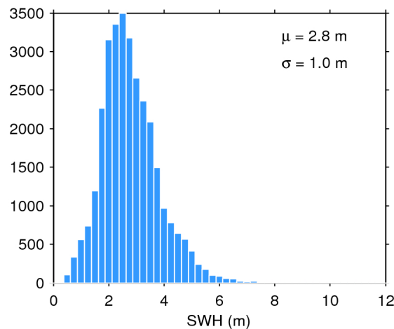
Figure 20. Histogram of science-valid SWH over oceans and lakes for 15/01/2020. The mean ( \mu ) and standard deviation ( \sigma ) are also shown. Note that values larger than 12 m are excluded from the histogram for the sake of readability but not from the computation of \mu and \sigma .
