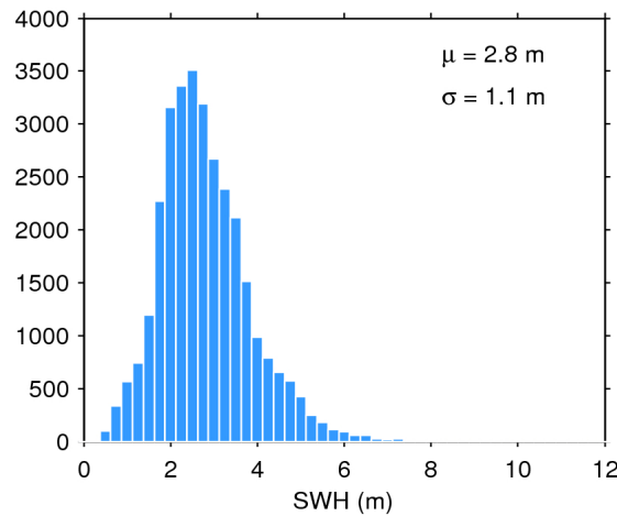
Figure 17. Histogram of flag-valid SWH over oceans and lakes for 15/01/2020. The mean ( \mu ) and standard deviation ( \sigma ) are also shown. Note that values larger than 12 m are excluded from the histogram for the sake of readability but not from the computation of \mu and \sigma .
