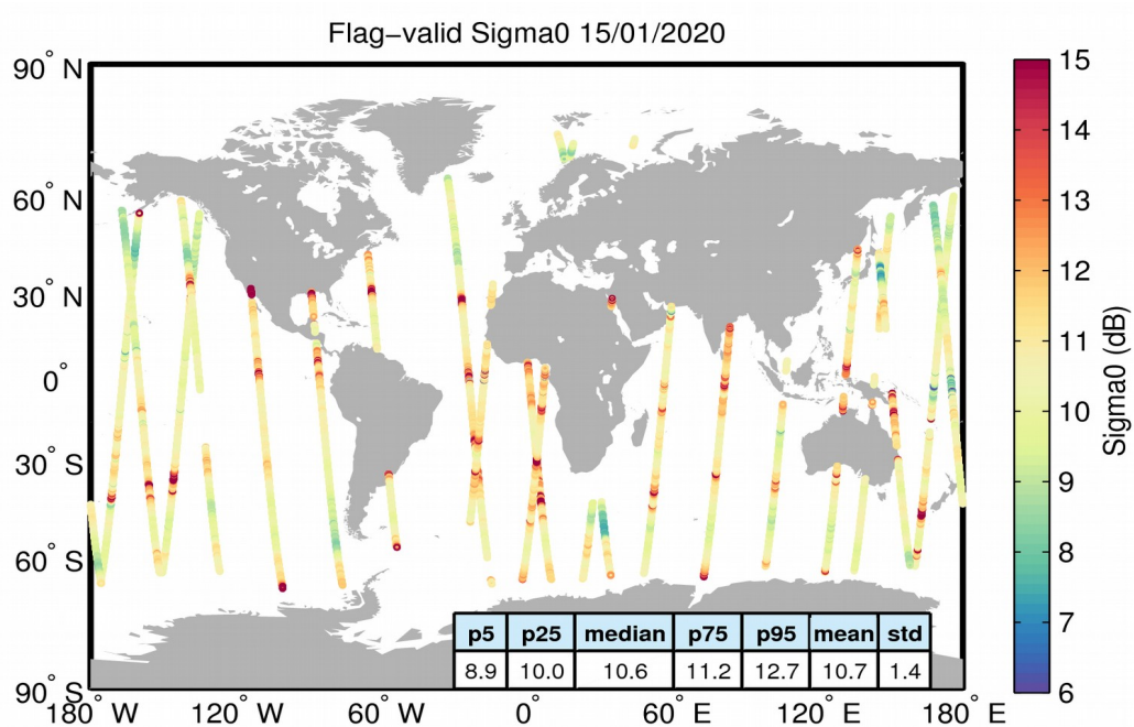
Figure 23. Geographical distribution of flag-valid sigma0 data over oceans and lakes for 15/01/2020. The statistical values shown in the table refer to the sigma0 in dB and are calculated over all measurements shown in the figure.
