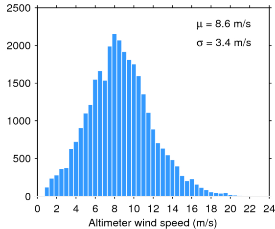
Figure 33. Histogram of flag-valid wind over oceans and lakes for 15/01/2020. The mean ( \mu ) and standard deviation ( \sigma ) are also shown. Note that values larger than 24 m/s are excluded from the histogram for the sake of readability but not from the computation of \mu and \sigma .
