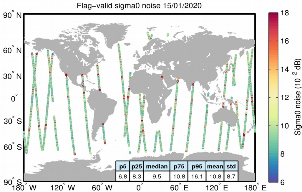
Figure 26. Geographical distribution of flag-valid 20-Hz sigma0 measurement noise over oceans and lakes for 15/01/2020. The statistical values shown in the table refer to the sigma0 noise and are calculated over all measurements shown in the figure.
