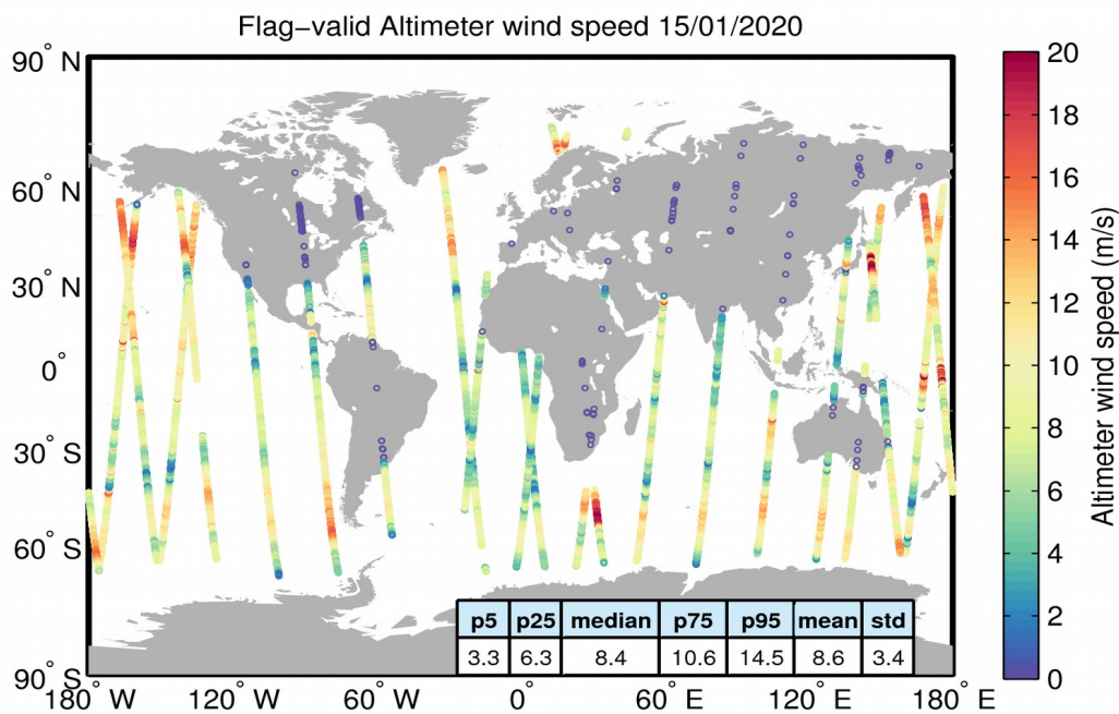
Figure 31. Geographical distribution of flag-valid wind data over oceans and lakes for 15/01/2020. The statistical values shown in the table refer to the wind in m/s and are calculated over all measurements shown in the figure.
