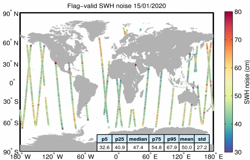
Figure 18. Geographical distribution of flag-valid 20-Hz SWH measurement noise over oceans and lakes for 15/01/2020. The statistical values shown in the figure refer to the SWH noise and are calculated over all measurements shown in the figure.
