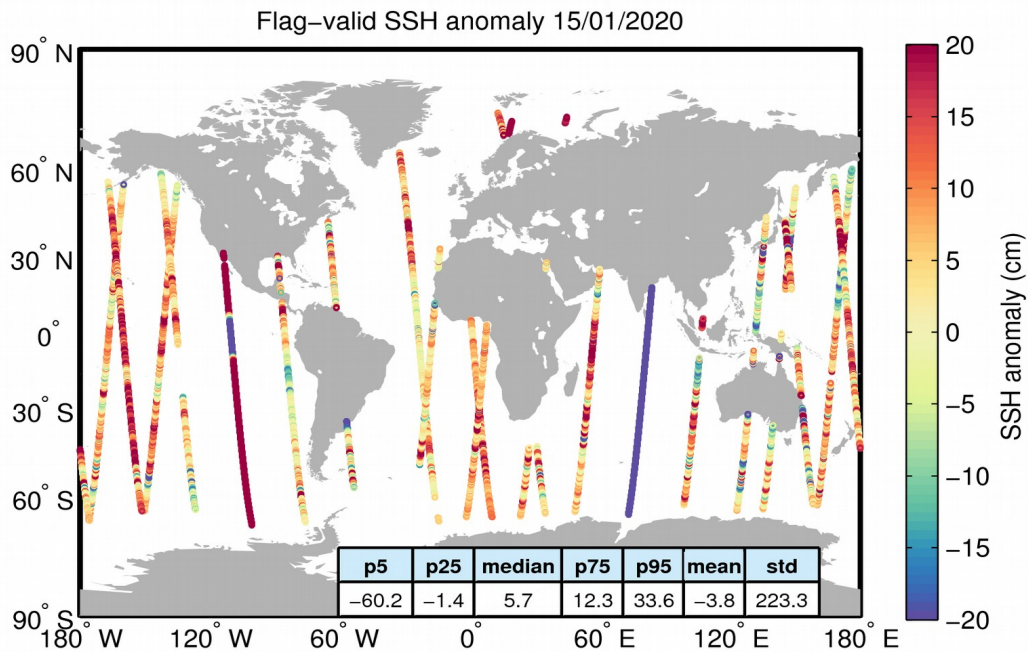
Figure 5. Geographical distribution of flag-valid 1-Hz SSH anomaly data over oceans and lakes for 15/01/2020. The statistical values shown in the table refer to the SSH anomaly in cm and are calculated over all measurements shown in the figure.
