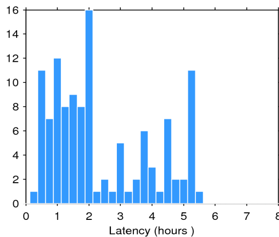
Figure 2. Histogram of the data latency for 15/01/2020. The y-axis denotes the number of files that are made available with a delay of x-hours with respect to the mean time of the records stored in the file.
