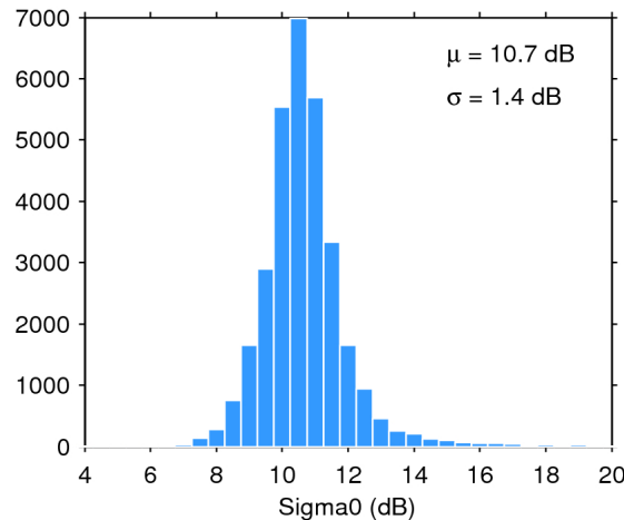
Figure 25. Histogram of flag-valid sigma0 over oceans and lakes for 15/01/2020. The mean ( \mu ) and standard deviation ( \sigma ) are also shown. Note that values outside [4 20] dB are excluded from the histogram for the sake of readability but not from the computation of \mu and \sigma .
