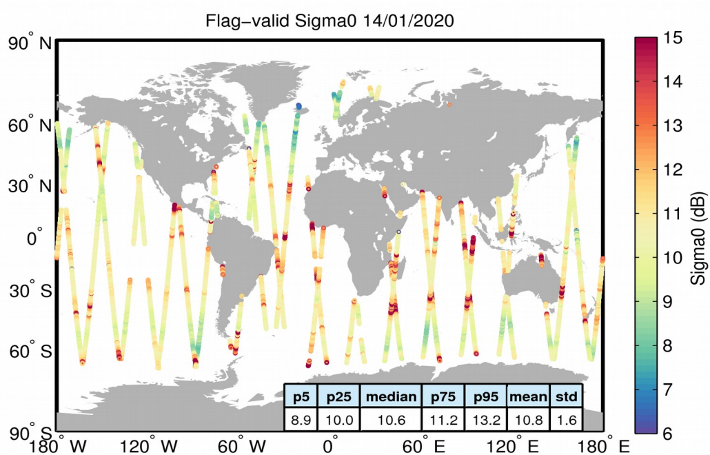
Figure 23. Geographical distribution of flag-valid sigma0 data over oceans and lakes for 14/01/2020. The statistical values shown in the table refer to the sigma0 in dB and are calculated over all measurements shown in the figure.
