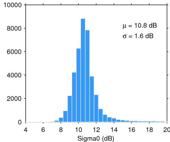
Figure 25. Histogram of flag-valid sigma0 over oceans and lakes for 14/01/2020. The mean ( \mu ) and standard deviation ( \sigma ) are also shown. Note that values outside [4 20] dB are excluded from the histogram for the sake of readability but not from the computation of \mu and \sigma .
