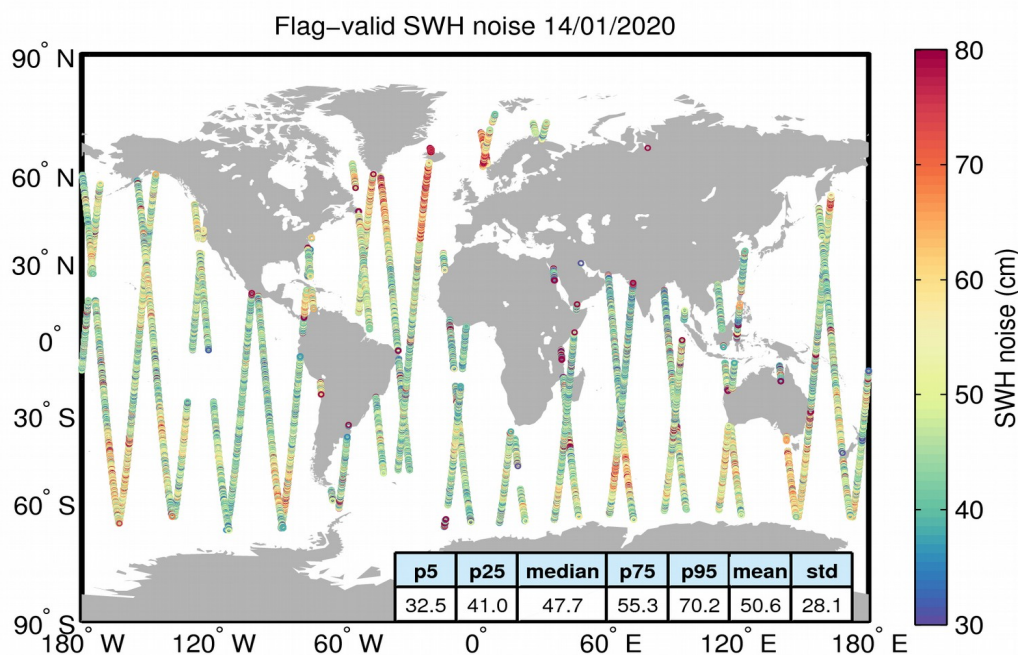
Figure 18. Geographical distribution of flag-valid 20-Hz SWH measurement noise over oceans and lakes for 14/01/2020. The statistical values shown in the table refer to the SWH noise and are calculated over all measurements shown in the figure.
