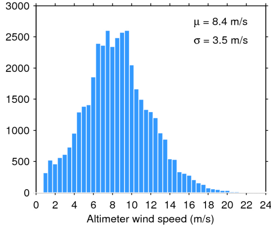
Figure 33. Histogram of flag-valid wind over oceans and lakes for 14/01/2020. The mean ( \mu ) and standard deviation ( \sigma ) are also shown. Note that values larger than 24 m/s are excluded from the histogram for the sake of readability but not from the computation of \mu and \sigma .
