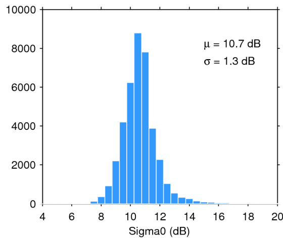
Figure 28. Histogram of science-valid sigma0 over oceans and lakes for 14/01/2020. The mean ( \mu ) and standard deviation ( \sigma ) are also shown. Note that values outside [4 20] dB are excluded from the histogram for the sake of readability but not from the computation of \mu and \sigma .
