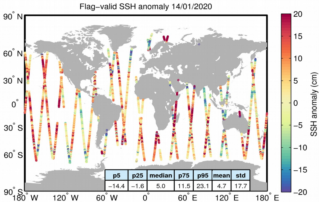
Figure 5. Geographical distribution of flag-valid 1-Hz SSH anomaly data over oceans and lakes for 14/01/2020. The statistical values shown in the table refer to the SSH anomaly in cm and are calculated over all measurements shown in the figure.
