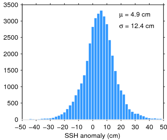
Figure 11. Histogram of science-valid SSH anomaly over oceans and lakes for 14/01/2020. The mean ( \mu ) and standard deviation ( \sigma ) are also shown. Note that values outside [-50 50] cm are excluded from the histogram for the sake of readability but not from the computation of \mu and \sigma .
