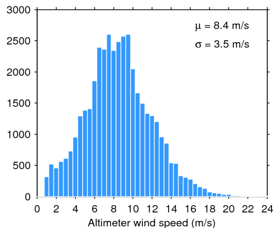
Figure 35. Histogram of science-valid wind over oceans and lakes for 14/01/2020. The mean ( \mu ) and standard deviation ( \sigma ) are also shown. Note that values larger than 24 m/s are excluded from the histogram for the sake of readability but not from the computation of \mu and \sigma .
