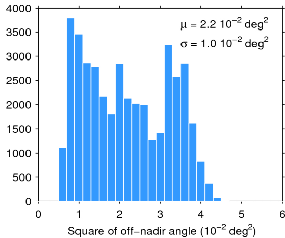
Figure 39. Histogram of flag-valid mispointing over oceans and lakes for 14/01/2020. The mean ( \mu ) and standard deviation ( \sigma ) are also shown. Note that values larger than 6 \cdot 10^{-2} \text{ deg}^2 are excluded from the histogram for the sake of readability but not from the computation of \mu and \sigma .
