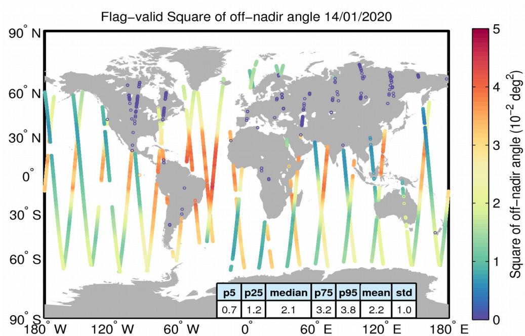
Figure 37. Geographical distribution of flag-valid mispointing data over oceans and lakes for 14/01/2020. The statistical values shown in the table refer to the mispointing in 10^{-2} \text{ deg}^2 and are calculated over all measurements shown in the figure.
