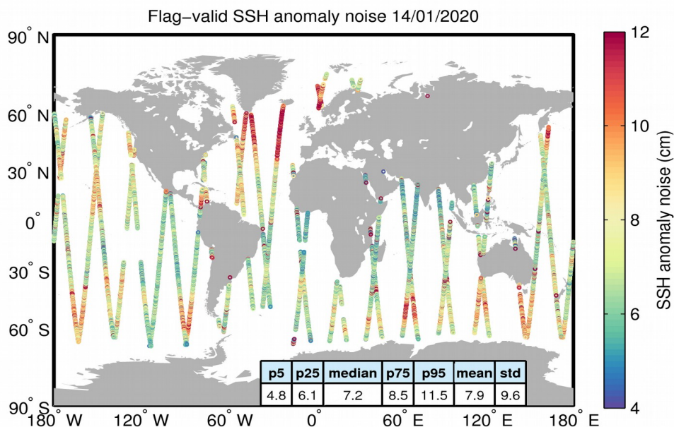
Figure 8. Geographical distribution of flag-valid 20-Hz SSH anomaly measurement noise over oceans and lakes for 14/01/2020. The statistical values shown in the table refer to the SSH anomaly noise and are calculated over all measurements shown in the figure.
