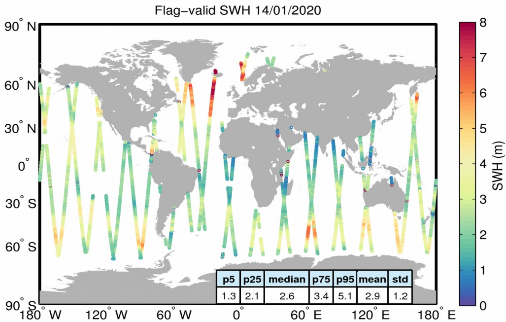
Figure 15. Geographical distribution of flag-valid SWH data over oceans and lakes for 14/01/2020. The statistical values shown in the table refer to the SWH in m and are calculated over all measurements shown in the figure.
