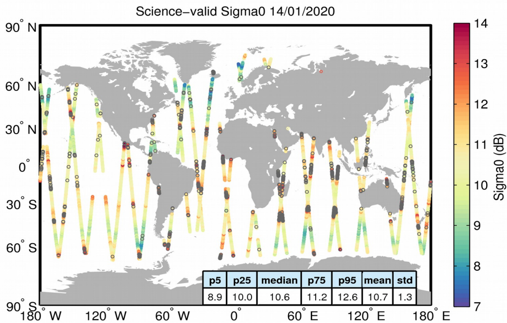
Figure 27. Geographical distribution of science-valid sigma0 data over oceans and lakes for 14/01/2020. The statistical values shown in the table refer to the sigma0 in dB and are calculated over all measurements shown in the figure. Gray circles denote records that have been rejected based on the editing criteria described in Table 4.
