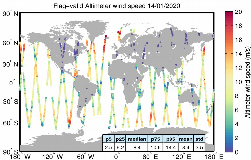
Figure 31. Geographical distribution of flag-valid wind data over oceans and lakes for 14/01/2020. The statistical values shown in the table refer to the wind in m/s and are calculated over all measurements shown in the figure.
