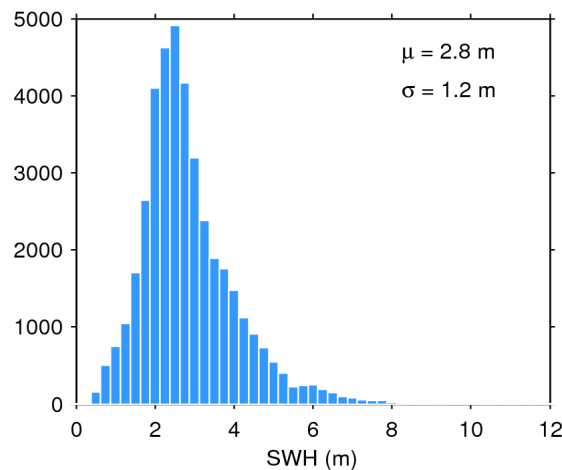
Figure 20. Histogram of science-valid SWH over oceans and lakes for 14/01/2020. The mean ( \mu ) and standard deviation ( \sigma ) are also shown. Note that values larger than 12 m are excluded from the histogram for the sake of readability but not from the computation of \mu and \sigma .
