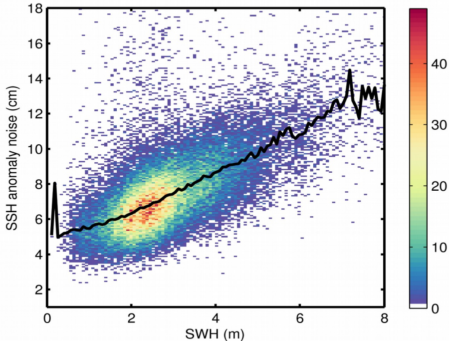
Figure 9. 2D histogram showing flag-valid SSH anomaly noise as a function of SWH for 14/01/2020. The black line denotes the median SSH anomaly noise as a function of SWH.
