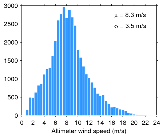
Figure 35. Histogram of science-valid wind over oceans and lakes for 13/01/2020. The mean ( \mu ) and standard deviation ( \sigma ) are also shown. Note that values larger than 24 m/s are excluded from the histogram for the sake of readability but not from the computation of \mu and \sigma .
