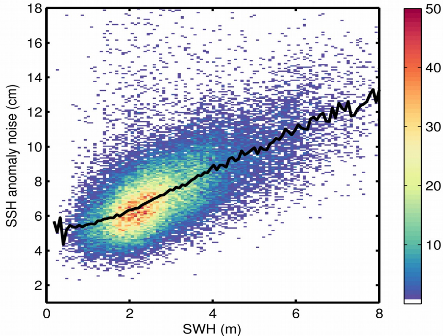
Figure 9. 2D histogram showing flag-valid SSH anomaly noise as a function of SWH for 13/01/2020. The black line denotes the median SSH anomaly noise as a function of SWH.
