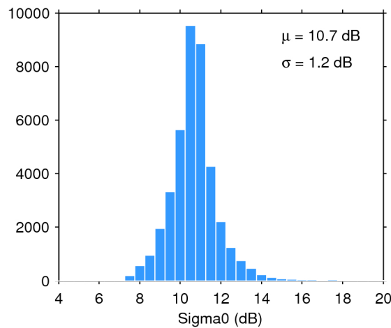
Figure 28. Histogram of science-valid sigma0 over oceans and lakes for 13/01/2020. The mean ( \mu ) and standard deviation ( \sigma ) are also shown. Note that values outside [4 20] dB are excluded from the histogram for the sake of readability but not from the computation of \mu and \sigma .
