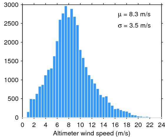
Figure 33. Histogram of flag-valid wind over oceans and lakes for 13/01/2020. The mean ( \mu ) and standard deviation ( \sigma ) are also shown. Note that values larger than 24 m/s are excluded from the histogram for the sake of readability but not from the computation of \mu and \sigma .
