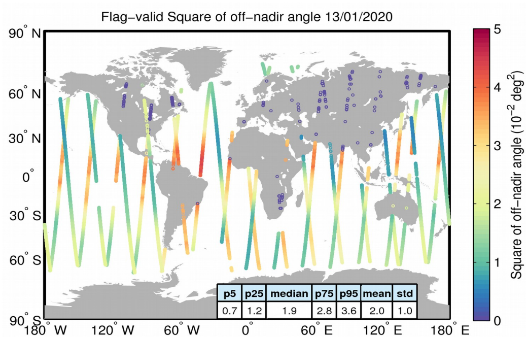
Figure 37. Geographical distribution of flag-valid mispointing data over oceans and lakes for 13/01/2020. The statistical values shown in the table refer to the mispointing in 10^{-2} \text{ deg}^2 and are calculated over all measurements shown in the figure.
