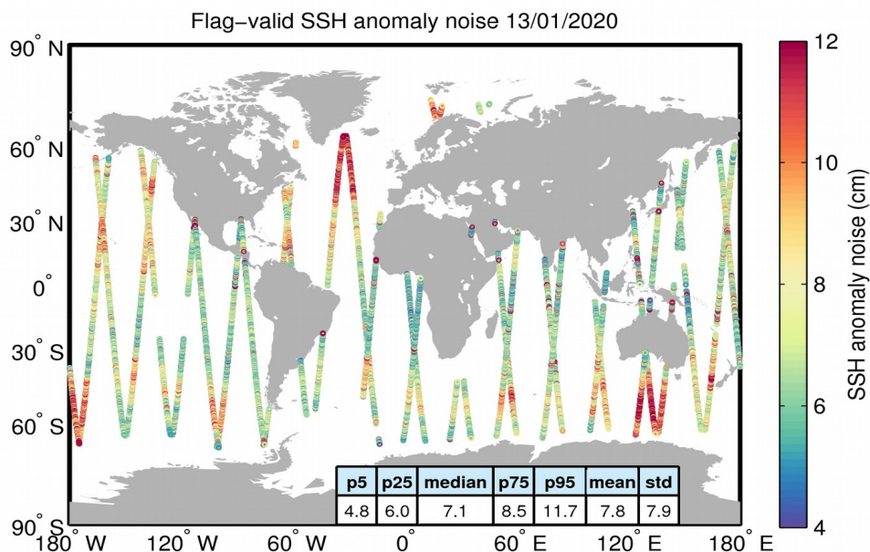
Figure 8. Geographical distribution of flag-valid 20-Hz SSH anomaly measurement noise over oceans and lakes for 13/01/2020. The statistical values shown in the table refer to the SSH anomaly noise and are calculated over all measurements shown in the figure.
