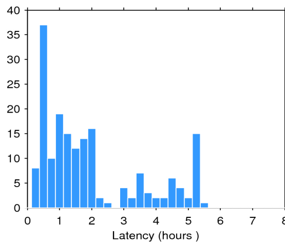
Figure 2. Histogram of the data latency for 13/01/2020. The y-axis denotes the number of files that are made available with a delay of x-hours with respect to the mean time of the records stored in the file.
