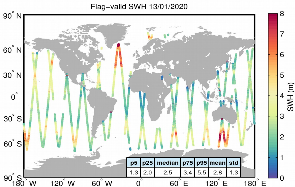
Figure 15. Geographical distribution of flag-valid SWH data over oceans and lakes for 13/01/2020. The statistical values shown in the table refer to the SWH in m and are calculated over all measurements shown in the figure.
