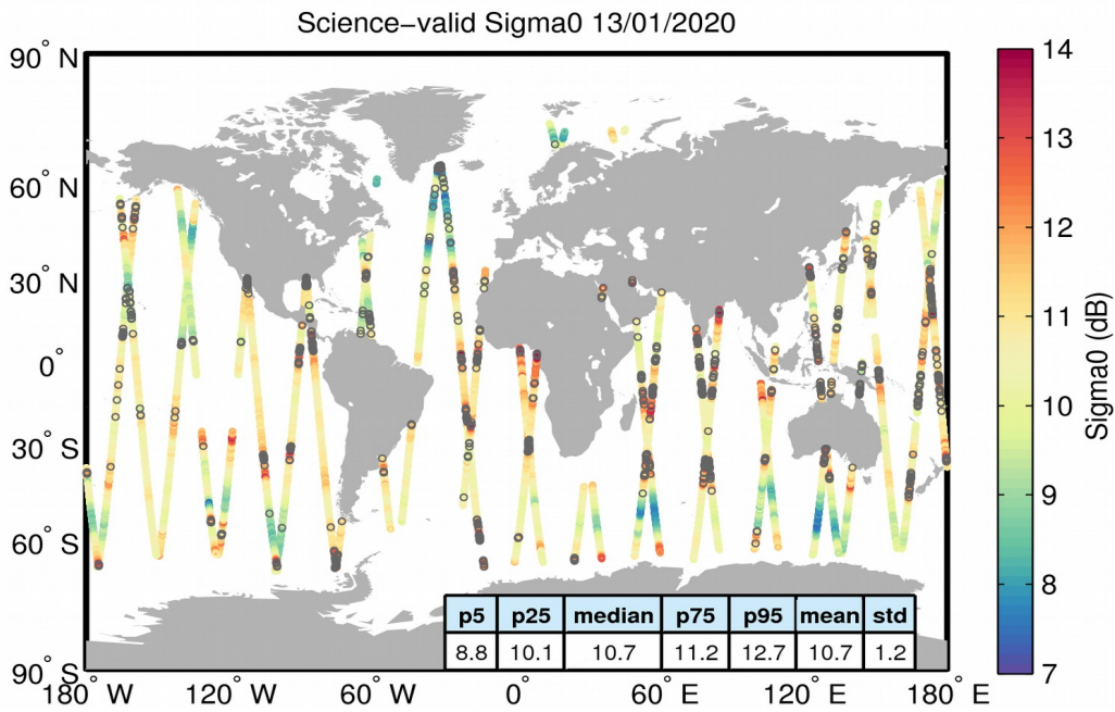
Figure 27. Geographical distribution of science-valid sigma0 data over oceans and lakes for 13/01/2020. The statistical values shown in the table refer to the sigma0 in dB and are calculated over all measurements shown in the figure. Gray circles denote records that have been rejected based on the editing criteria described in Table 4.
