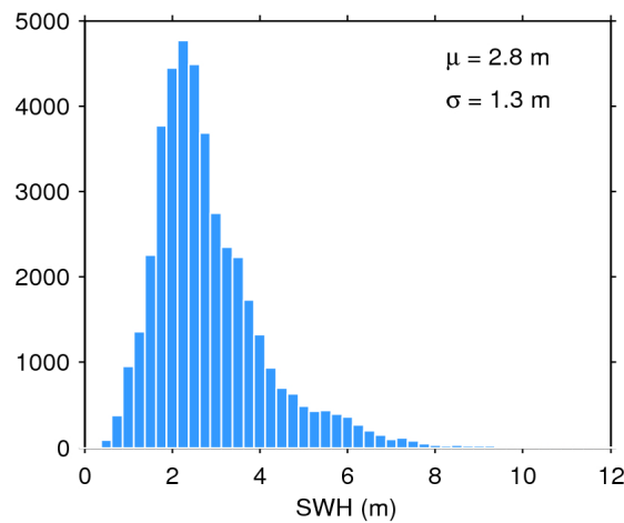
Figure 17. Histogram of flag-valid SWH over oceans and lakes for 13/01/2020. The mean ( \mu ) and standard deviation ( \sigma ) are also shown. Note that values larger than 12 m are excluded from the histogram for the sake of readability but not from the computation of \mu and \sigma .
