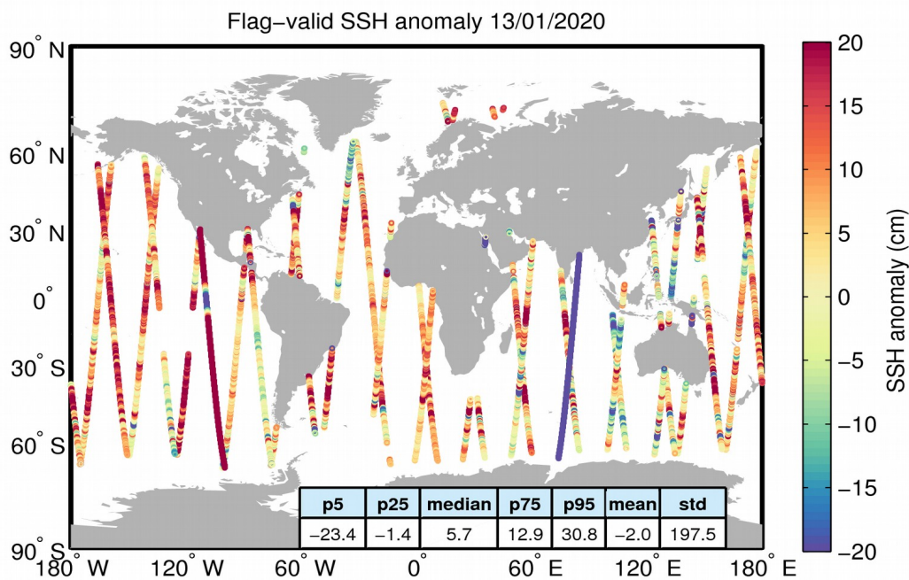
Figure 5. Geographical distribution of flag-valid 1-Hz SSH anomaly data over oceans and lakes for 13/01/2020. The statistical values shown in the table refer to the SSH anomaly in cm and are calculated over all measurements shown in the figure.
