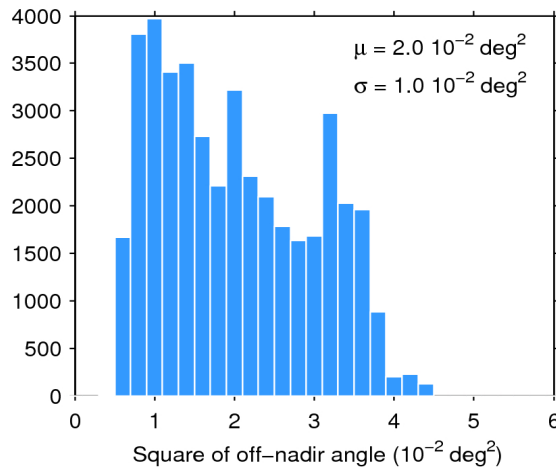
Figure 39. Histogram of flag-valid mispointing over oceans and lakes for 13/01/2020. The mean ( \mu ) and standard deviation ( \sigma ) are also shown. Note that values larger than 6 \cdot 10^{-2} \text{ deg}^2 are excluded from the histogram for the sake of readability but not from the computation of \mu and \sigma .
