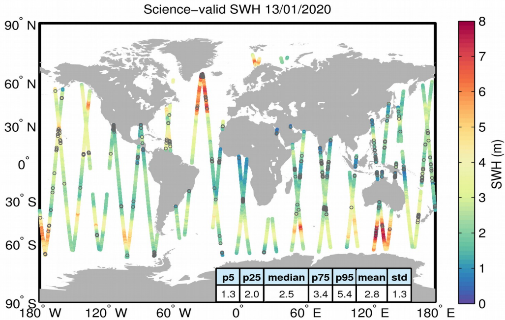
Figure 19. Geographical distribution of science-valid SWH data over oceans and lakes for 13/01/2020. The statistical values shown in the table refer to the SWH in m and are calculated over all measurements shown in the figure. Gray circles denote records that have been rejected based on the editing criteria described in Table 3.
