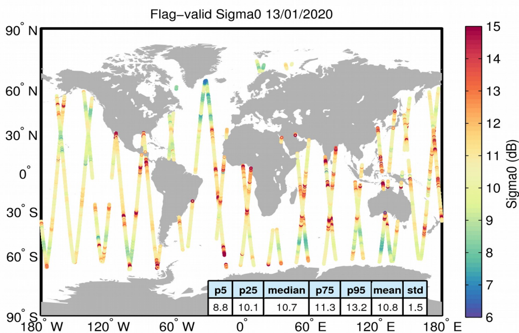
Figure 23. Geographical distribution of flag-valid sigma0 data over oceans and lakes for 13/01/2020. The statistical values shown in the table refer to the sigma0 in dB and are calculated over all measurements shown in the figure.
