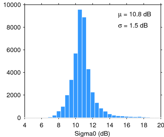
Figure 25. Histogram of flag-valid sigma0 over oceans and lakes for 13/01/2020. The mean ( \mu ) and standard deviation ( \sigma ) are also shown. Note that values outside [4 20] dB are excluded from the histogram for the sake of readability but not from the computation of \mu and \sigma .
