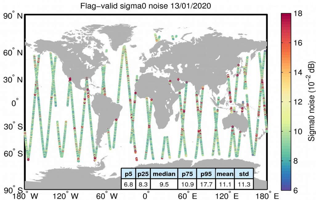
Figure 26. Geographical distribution of flag-valid 20-Hz sigma0 measurement noise over oceans and lakes for 13/01/2020. The statistical values shown in the table refer to the sigma0 noise and are calculated over all measurements shown in the figure.
