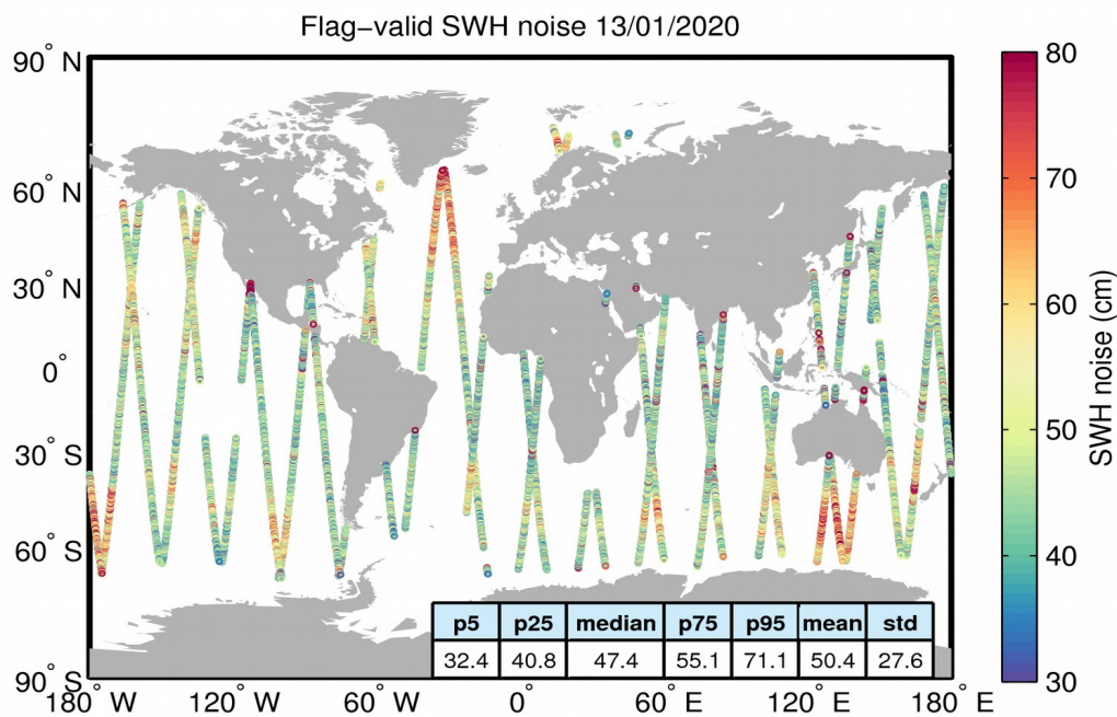
Figure 18. Geographical distribution of flag-valid 20-Hz SWH measurement noise over oceans and lakes for 13/01/2020. The statistical values shown in the table refer to the SWH noise and are calculated over all measurements shown in the figure.
