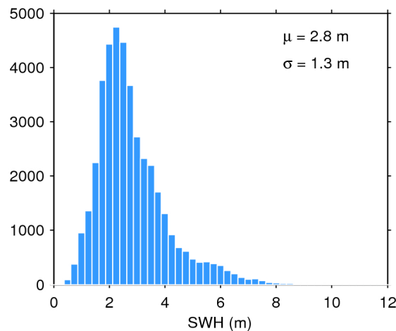
Figure 20. Histogram of science-valid SWH over oceans and lakes for 13/01/2020. The mean ( \mu ) and standard deviation ( \sigma ) are also shown. Note that values larger than 12 m are excluded from the histogram for the sake of readability but not from the computation of \mu and \sigma .
