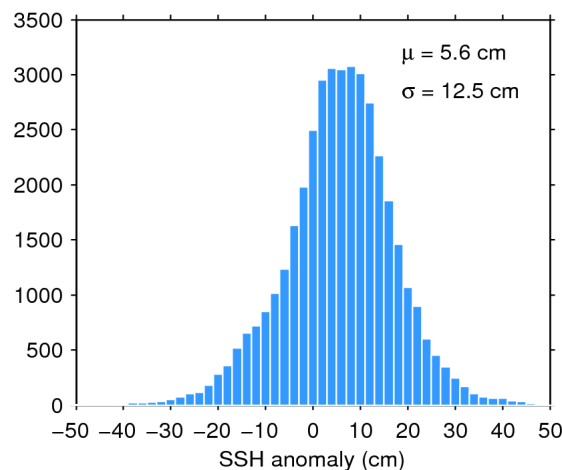
Figure 11. Histogram of science-valid SSH anomaly over oceans and lakes for 12/01/2020. The mean ( \mu ) and standard deviation ( \sigma ) are also shown. Note that values outside [-50 50] cm are excluded from the histogram for the sake of readability but not from the computation of \mu and \sigma .
