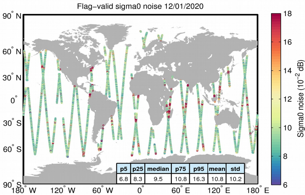
Figure 26. Geographical distribution of flag-valid 20-Hz sigma0 measurement noise over oceans and lakes for 12/01/2020. The statistical values shown in the table refer to the sigma0 noise and are calculated over all measurements shown in the figure.
