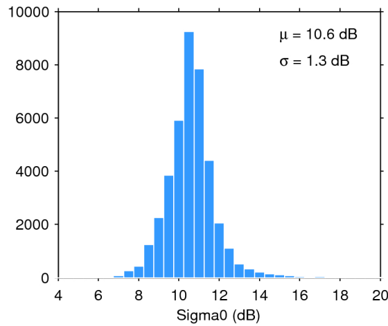
Figure 28. Histogram of science-valid sigma0 over oceans and lakes for 12/01/2020. The mean ( \mu ) and standard deviation ( \sigma ) are also shown. Note that values outside [4 20] dB are excluded from the histogram for the sake of readability but not from the computation of \mu and \sigma .
