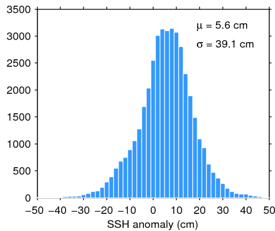
Figure 7. Histogram of flag-valid SSH anomaly over oceans and lakes for 12/01/2020. The mean ( \mu ) and standard deviation ( \sigma ) are also shown. Note that values outside [-50\ 50] cm are excluded from the histogram for the sake of readability but not from the computation of \mu and \sigma .
