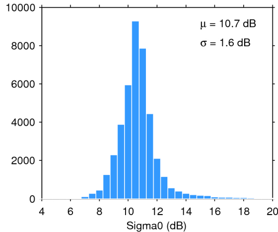
Figure 25. Histogram of flag-valid sigma0 over oceans and lakes for 12/01/2020. The mean ( \mu ) and standard deviation ( \sigma ) are also shown. Note that values outside [4 20] dB are excluded from the histogram for the sake of readability but not from the computation of \mu and \sigma .
