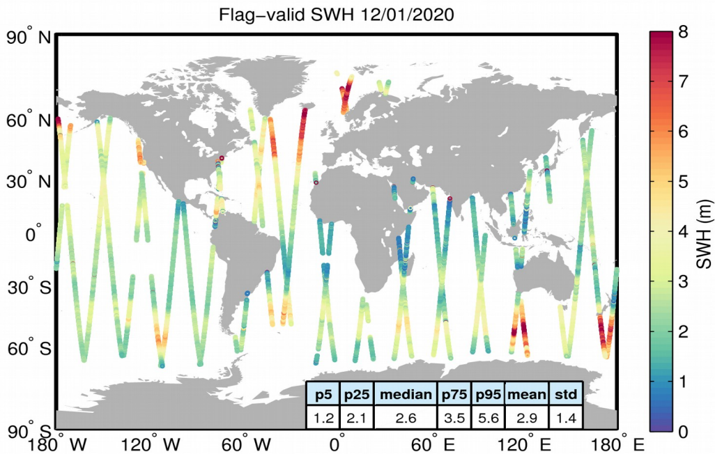
Figure 15. Geographical distribution of flag-valid SWH data over oceans and lakes for 12/01/2020. The statistical values shown in the table refer to the SWH in m and are calculated over all measurements shown in the figure.
