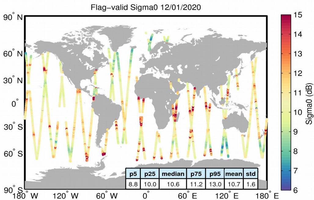
Figure 23. Geographical distribution of flag-valid sigma0 data over oceans and lakes for 12/01/2020. The statistical values shown in the table refer to the sigma0 in dB and are calculated over all measurements shown in the figure.
