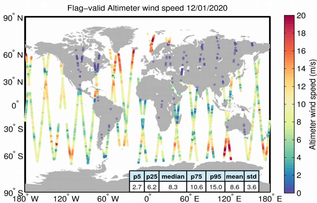
Figure 31. Geographical distribution of flag-valid wind data over oceans and lakes for 12/01/2020. The statistical values shown in the table refer to the wind in m/s and are calculated over all measurements shown in the figure.
