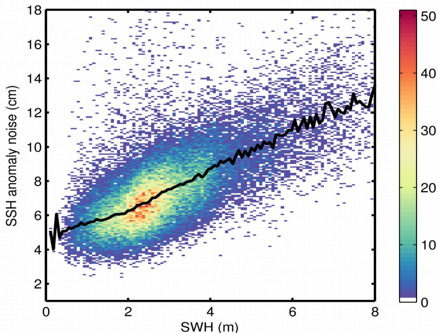
Figure 9. 2D histogram showing flag-valid SSH anomaly noise as a function of SWH for 12/01/2020. The black line denotes the median SSH anomaly noise as a function of SWH.
