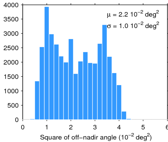
Figure 39. Histogram of flag-valid mispointing over oceans and lakes for 12/01/2020. The mean ( \mu ) and standard deviation ( \sigma ) are also shown. Note that values larger than 6 \cdot 10^{-2} \text{ deg}^2 are excluded from the histogram for the sake of readability but not from the computation of \mu and \sigma .
