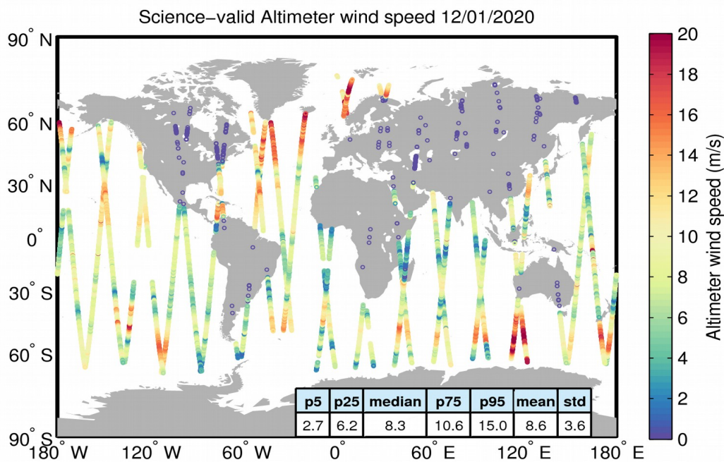
Figure 34. Geographical distribution of science-valid wind data over oceans and lakes for 12/01/2020. The statistical values shown in the table refer to the wind in m/s and are calculated over all measurements shown in the figure. Gray circles denote records that have been rejected based on the editing criteria described in Table 5.
