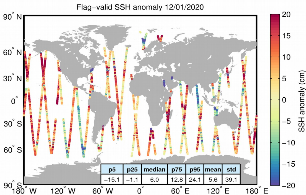
Figure 5. Geographical distribution of flag-valid 1-Hz SSH anomaly data over oceans and lakes for 12/01/2020. The statistical values shown in the table refer to the SSH anomaly in cm and are calculated over all measurements shown in the figure.
