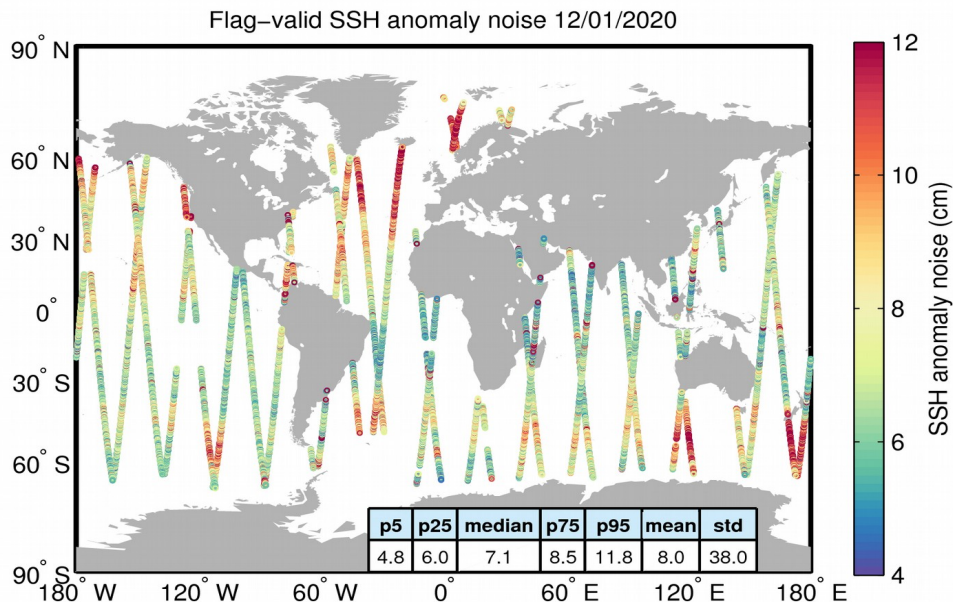
Figure 8. Geographical distribution of flag-valid 20-Hz SSH anomaly measurement noise over oceans and lakes for 12/01/2020. The statistical values shown in the table refer to the SSH anomaly noise and are calculated over all measurements shown in the figure.
