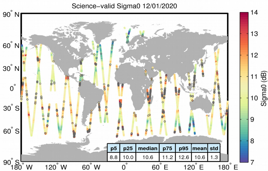
Figure 27. Geographical distribution of science-valid sigma0 data over oceans and lakes for 12/01/2020. The statistical values shown in the table refer to the sigma0 in dB and are calculated over all measurements shown in the figure. Gray circles denote records that have been rejected based on the editing criteria described in Table 4.
