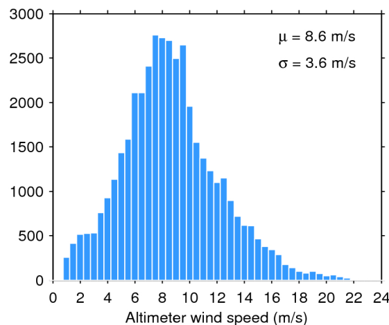
Figure 35. Histogram of science-valid wind over oceans and lakes for 12/01/2020. The mean ( \mu ) and standard deviation ( \sigma ) are also shown. Note that values larger than 24 m/s are excluded from the histogram for the sake of readability but not from the computation of \mu and \sigma .
