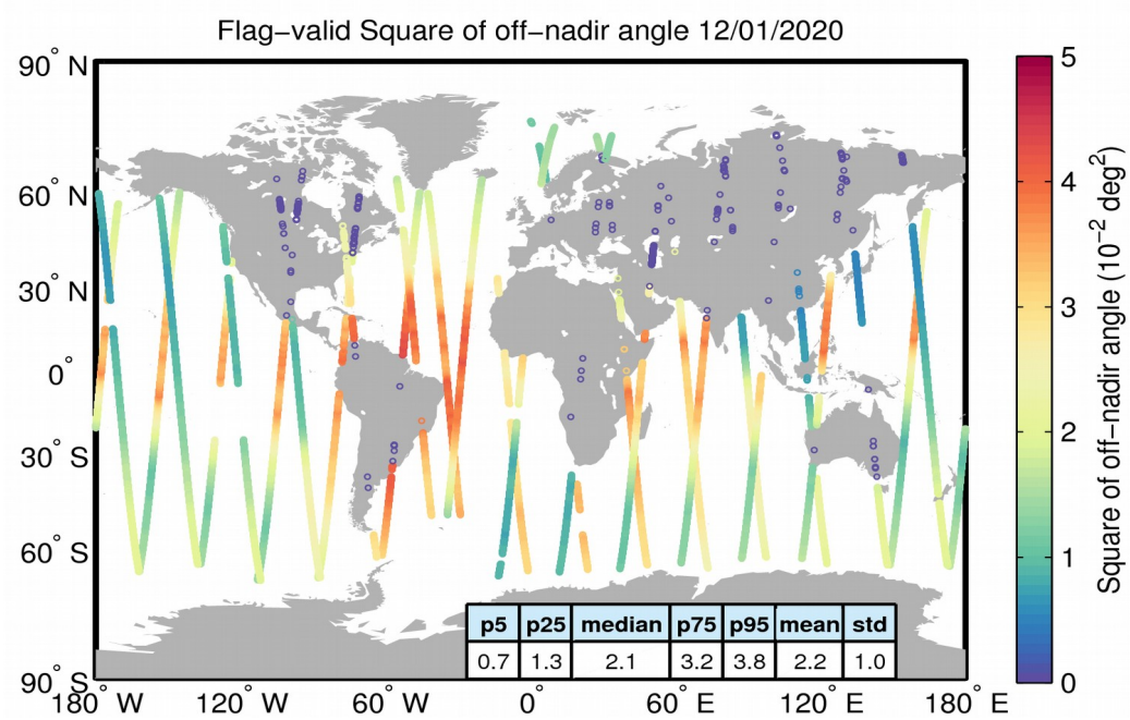
Figure 37. Geographical distribution of flag-valid mispointing data over oceans and lakes for 12/01/2020. The statistical values shown in the table refer to the mispointing in 10^{-2} \text{deg}^2 and are calculated over all measurements shown in the figure.
