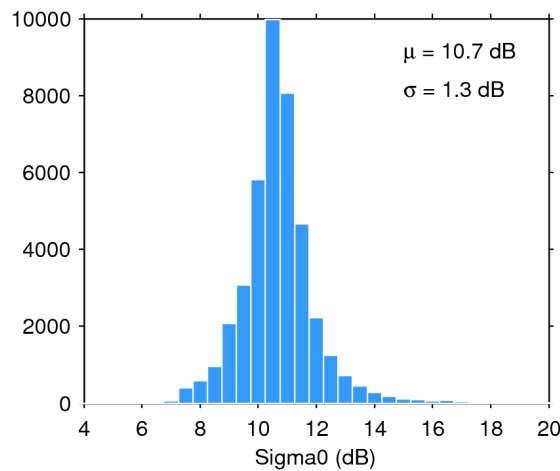
Figure 28. Histogram of science-valid sigma0 over oceans and lakes for 11/01/2020. The mean ( \mu ) and standard deviation ( \sigma ) are also shown. Note that values outside [4 20] dB are excluded from the histogram for the sake of readability but not from the computation of \mu and \sigma .
