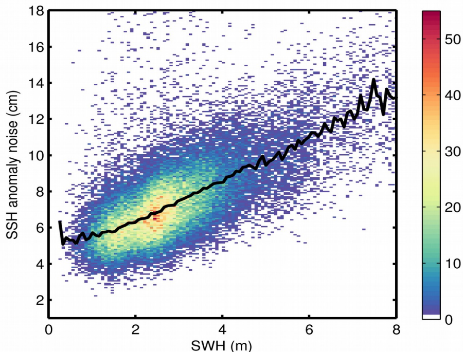
Figure 9. 2D histogram showing flag-valid SSH anomaly noise as a function of SWH for 11/01/2020. The black line denotes the median SSH anomaly noise as a function of SWH.
