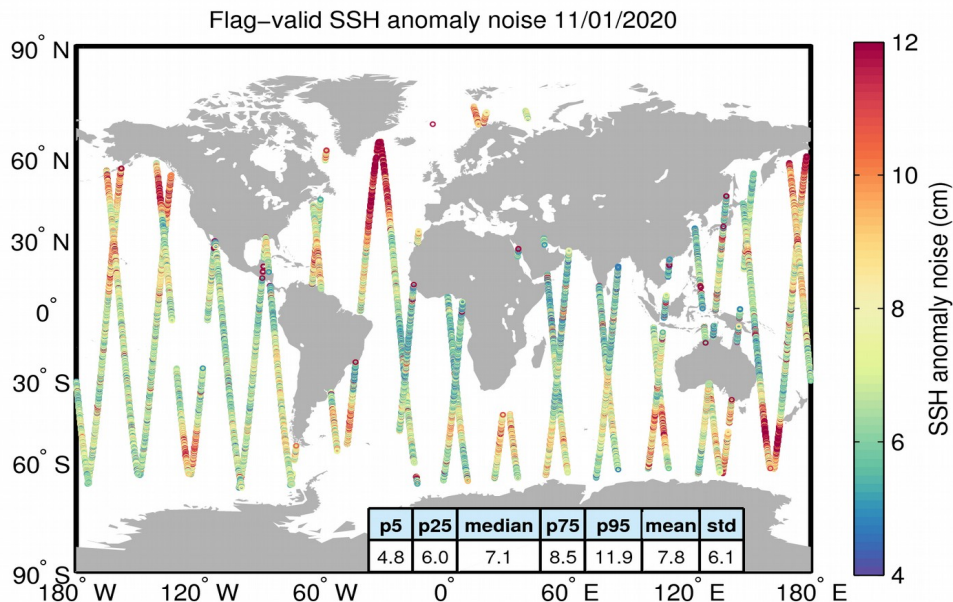
Figure 8. Geographical distribution of flag-valid 20-Hz SSH anomaly measurement noise over oceans and lakes for 11/01/2020. The statistical values shown in the table refer to the SSH anomaly noise and are calculated over all measurements shown in the figure.
