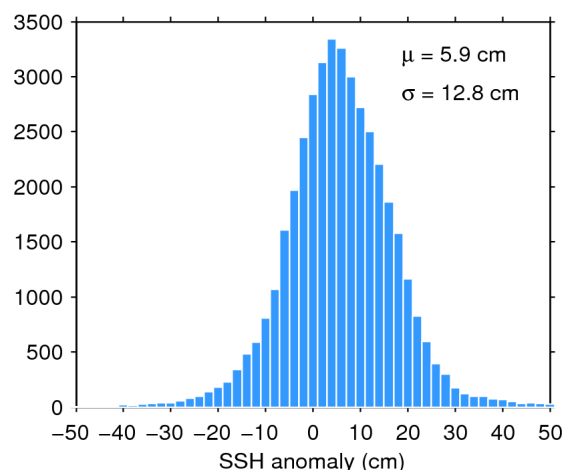
Figure 11. Histogram of science-valid SSH anomaly over oceans and lakes for 11/01/2020. The mean ( \mu ) and standard deviation ( \sigma ) are also shown. Note that values outside [-50 50] cm are excluded from the histogram for the sake of readability but not from the computation of \mu and \sigma .
