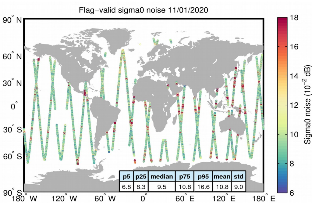
Figure 26. Geographical distribution of flag-valid 20-Hz sigma0 measurement noise over oceans and lakes for 11/01/2020. The statistical values shown in the table refer to the sigma0 noise and are calculated over all measurements shown in the figure.
