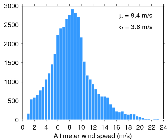
Figure 35. Histogram of science-valid wind over oceans and lakes for 11/01/2020. The mean ( \mu ) and standard deviation ( \sigma ) are also shown. Note that values larger than 24 m/s are excluded from the histogram for the sake of readability but not from the computation of \mu and \sigma .
