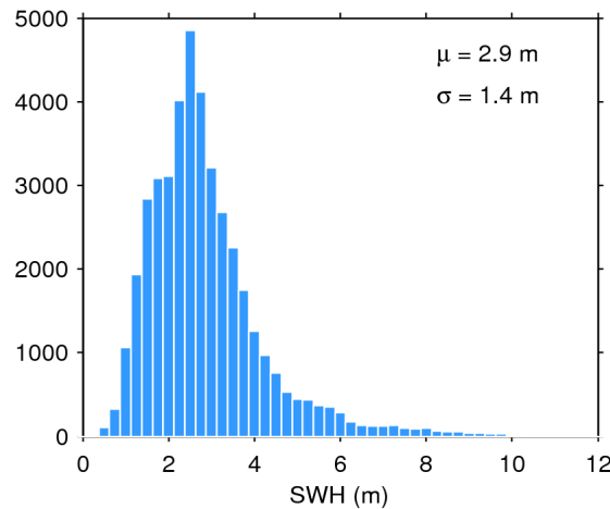
Figure 20. Histogram of science-valid SWH over oceans and lakes for 11/01/2020. The mean ( \mu ) and standard deviation ( \sigma ) are also shown. Note that values larger than 12 m are excluded from the histogram for the sake of readability but not from the computation of \mu and \sigma .
