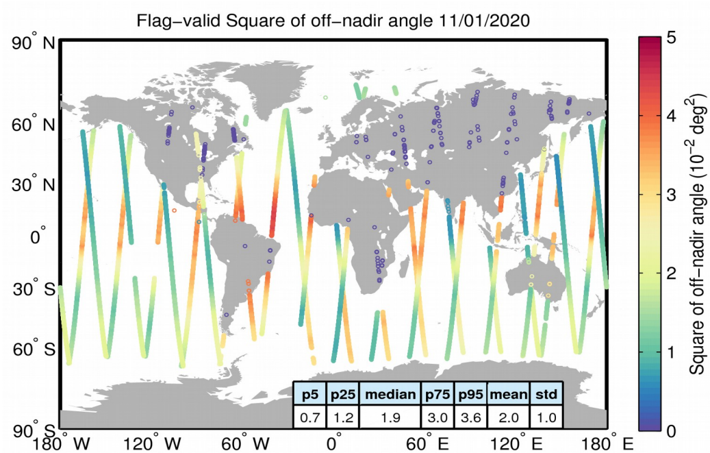
Figure 37. Geographical distribution of flag-valid mispointing data over oceans and lakes for 11/01/2020. The statistical values shown in the table refer to the mispointing in 10^{-2} \text{ deg}^2 and are calculated over all measurements shown in the figure.
