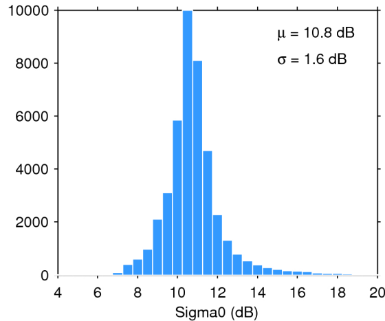
Figure 25. Histogram of flag-valid sigma0 over oceans and lakes for 11/01/2020. The mean ( \mu ) and standard deviation ( \sigma ) are also shown. Note that values outside [4 20] dB are excluded from the histogram for the sake of readability but not from the computation of \mu and \sigma .
