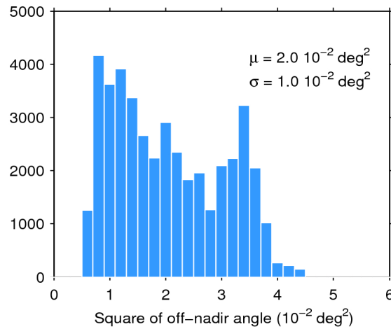
Figure 39. Histogram of flag-valid mispointing over oceans and lakes for 11/01/2020. The mean ( \mu ) and standard deviation ( \sigma ) are also shown. Note that values larger than 6 \cdot 10^{-2} \text{ deg}^2 are excluded from the histogram for the sake of readability but not from the computation of \mu and \sigma .
