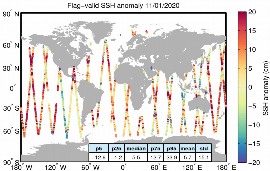
Figure 5. Geographical distribution of flag-valid 1-Hz SSH anomaly data over oceans and lakes for 11/01/2020. The statistical values shown in the table refer to the SSH anomaly in cm and are calculated over all measurements shown in the figure.
