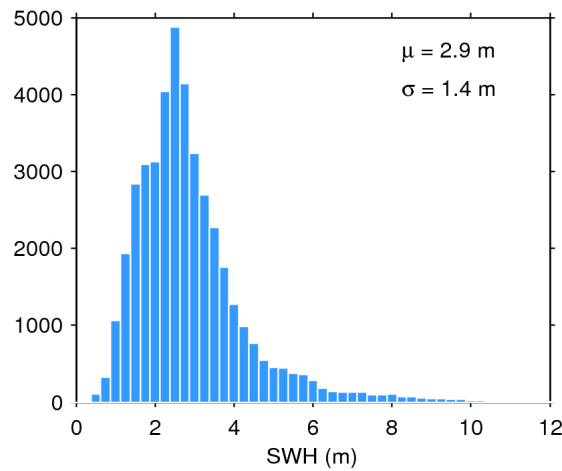
Figure 17. Histogram of flag-valid SWH over oceans and lakes for 11/01/2020. The mean ( \mu ) and standard deviation ( \sigma ) are also shown. Note that values larger than 12 m are excluded from the histogram for the sake of readability but not from the computation of \mu and \sigma .
