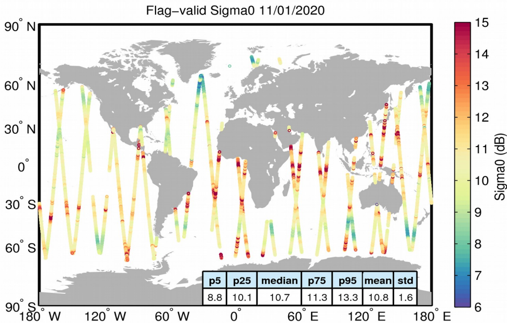
Figure 23. Geographical distribution of flag-valid sigma0 data over oceans and lakes for 11/01/2020. The statistical values shown in the table refer to the sigma0 in dB and are calculated over all measurements shown in the figure.
