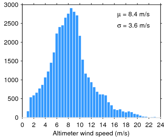
Figure 33. Histogram of flag-valid wind over oceans and lakes for 11/01/2020. The mean ( \mu ) and standard deviation ( \sigma ) are also shown. Note that values larger than 24 m/s are excluded from the histogram for the sake of readability but not from the computation of \mu and \sigma .
