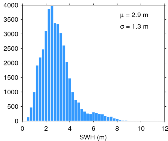
Figure 20. Histogram of science-valid SWH over oceans and lakes for 10/01/2020. The mean ( \mu ) and standard deviation ( \sigma ) are also shown. Note that values larger than 12 m are excluded from the histogram for the sake of readability but not from the computation of \mu and \sigma .
