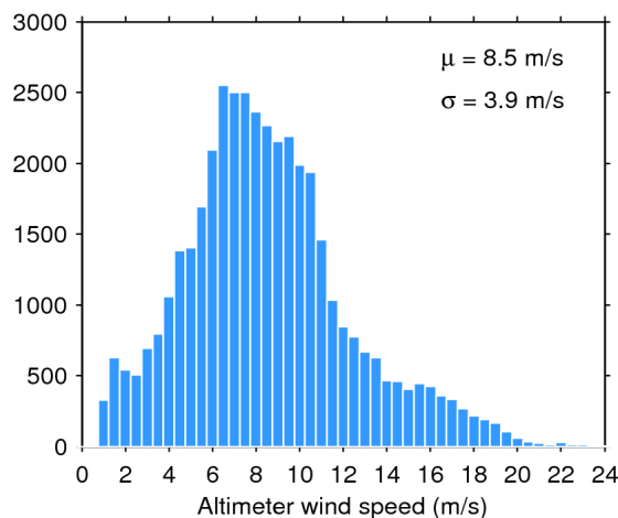
Figure 35. Histogram of science-valid wind over oceans and lakes for 10/01/2020. The mean ( \mu ) and standard deviation ( \sigma ) are also shown. Note that values larger than 24 m/s are excluded from the histogram for the sake of readability but not from the computation of \mu and \sigma .
