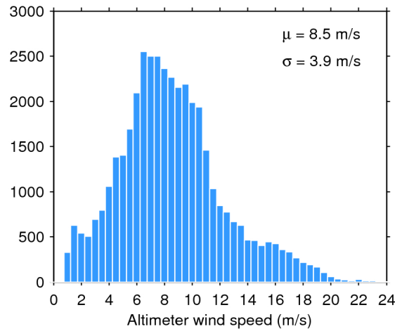
Figure 33. Histogram of flag-valid wind over oceans and lakes for 10/01/2020. The mean ( \mu ) and standard deviation ( \sigma ) are also shown. Note that values larger than 24 m/s are excluded from the histogram for the sake of readability but not from the computation of \mu and \sigma .
