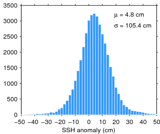
Figure 7. Histogram of flag-valid SSH anomaly over oceans and lakes for 10/01/2020. The mean ( \mu ) and standard deviation ( \sigma ) are also shown. Note that values outside [-50\ 50] cm are excluded from the histogram for the sake of readability but not from the computation of \mu and \sigma .
