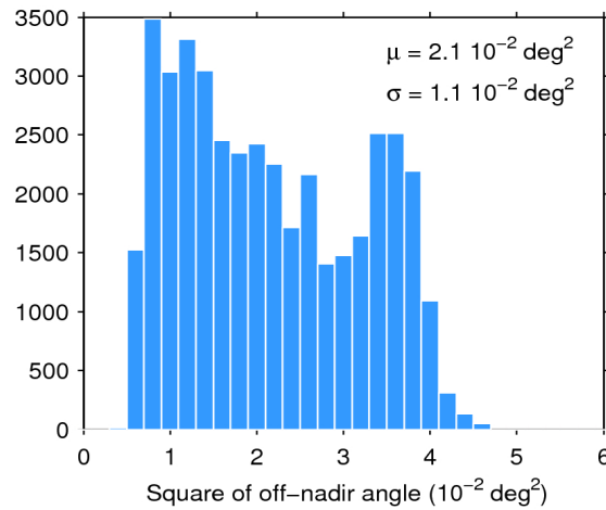
Figure 39. Histogram of flag-valid mispointing over oceans and lakes for 10/01/2020. The mean ( \mu ) and standard deviation ( \sigma ) are also shown. Note that values larger than 6 \cdot 10^{-2} \text{ deg}^2 are excluded from the histogram for the sake of readability but not from the computation of \mu and \sigma .
