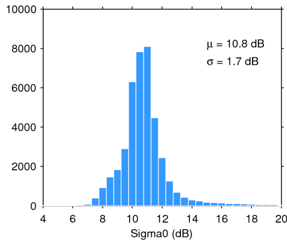
Figure 25. Histogram of flag-valid sigma0 over oceans and lakes for 10/01/2020. The mean ( \mu ) and standard deviation ( \sigma ) are also shown. Note that values outside [4 20] dB are excluded from the histogram for the sake of readability but not from the computation of \mu and \sigma .
