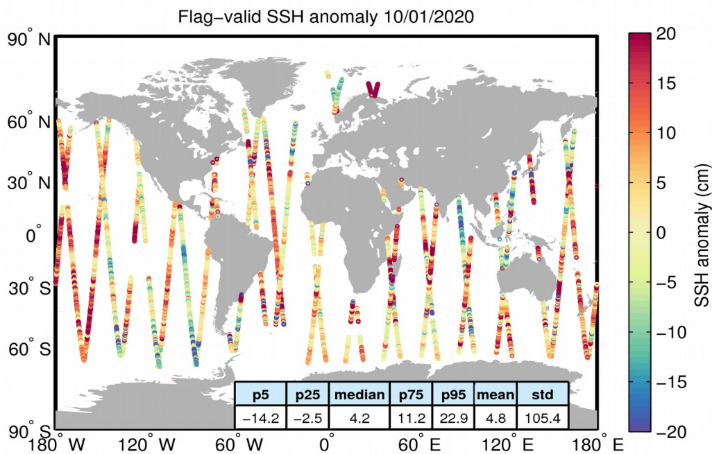
Figure 5. Geographical distribution of flag-valid 1-Hz SSH anomaly data over oceans and lakes for 10/01/2020. The statistical values shown in the table refer to the SSH anomaly in cm and are calculated over all measurements shown in the figure.
