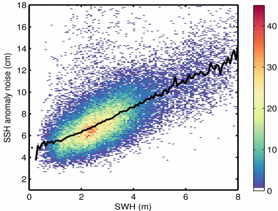
Figure 9. 2D histogram showing flag-valid SSH anomaly noise as a function of SWH for 10/01/2020. The black line denotes the median SSH anomaly noise as a function of SWH.
