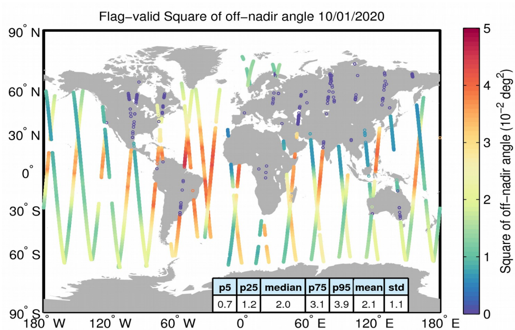
Figure 37. Geographical distribution of flag-valid mispointing data over oceans and lakes for 10/01/2020. The statistical values shown in the table refer to the mispointing in 10^{-2} deg 2 and are calculated over all measurements shown in the figure.
