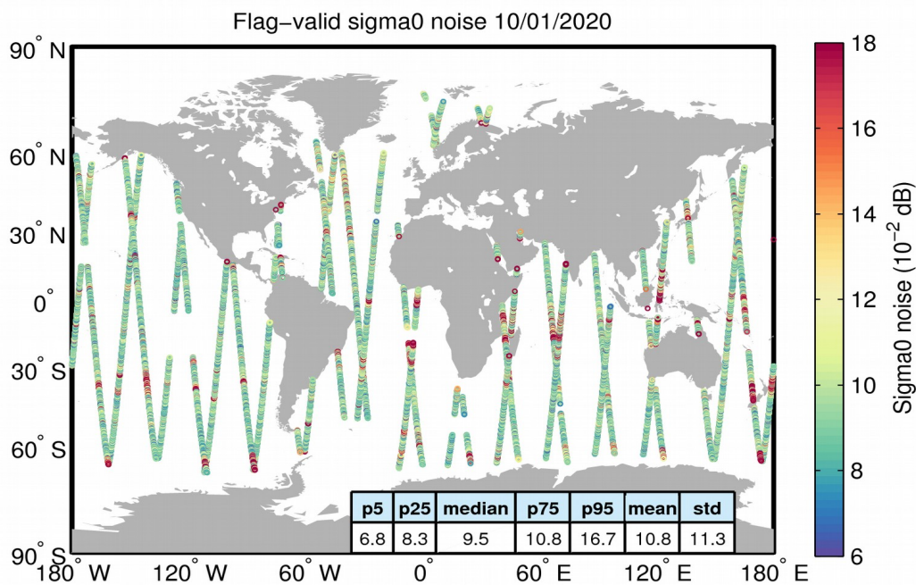
Figure 26. Geographical distribution of flag-valid 20-Hz sigma0 measurement noise over oceans and lakes for 10/01/2020. The statistical values shown in the table refer to the sigma0 noise and are calculated over all measurements shown in the figure.
