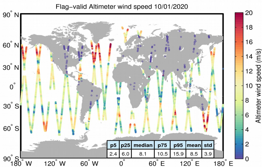
Figure 31. Geographical distribution of flag-valid wind data over oceans and lakes for 10/01/2020. The statistical values shown in the table refer to the wind in m/s and are calculated over all measurements shown in the figure.
