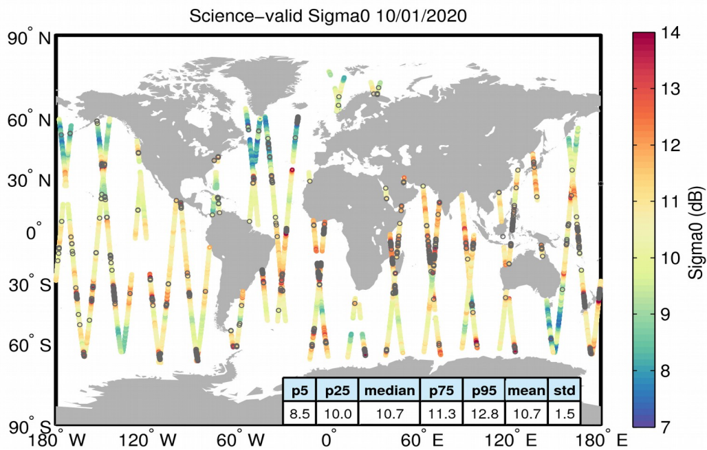
Figure 27. Geographical distribution of science-valid sigma0 data over oceans and lakes for 10/01/2020. The statistical values shown in the table refer to the sigma0 in dB and are calculated over all measurements shown in the figure. Gray circles denote records that have been rejected based on the editing criteria described in Table 4.
