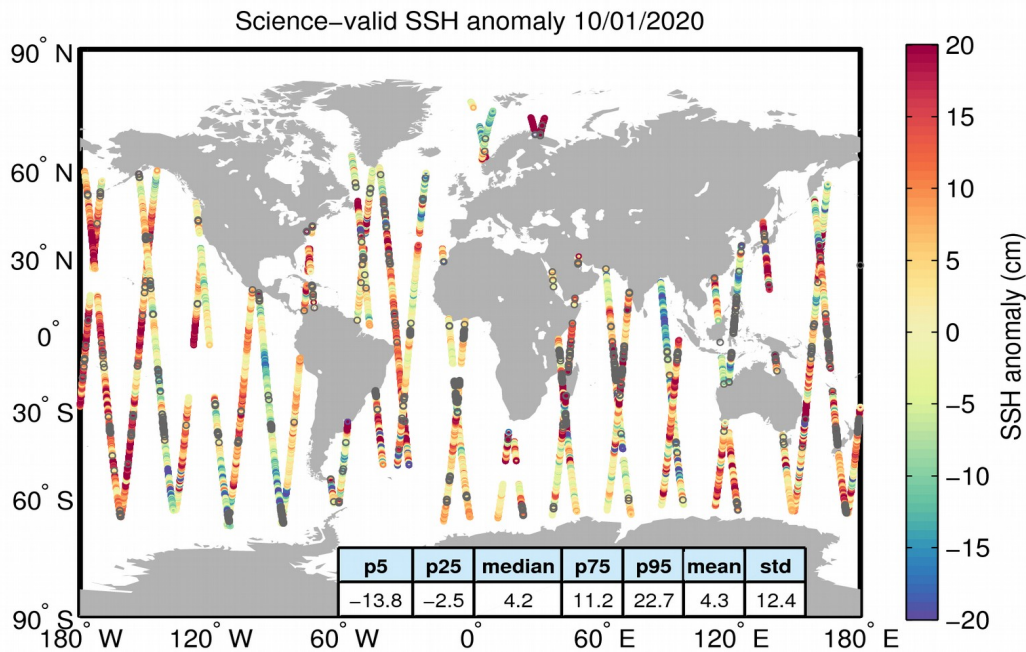
Figure 10. Geographical distribution of science-valid SSH anomaly data over oceans and lakes for 10/01/2020. The statistical values shown in the table refer to the SSH anomaly in cm and are calculated over all measurements shown in the figure. Gray circles denote records that have been rejected based on the editing criteria described in Table 2.
