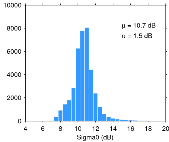
Figure 28. Histogram of science-valid sigma0 over oceans and lakes for 10/01/2020. The mean ( \mu ) and standard deviation ( \sigma ) are also shown. Note that values outside [4 20] dB are excluded from the histogram for the sake of readability but not from the computation of \mu and \sigma .
