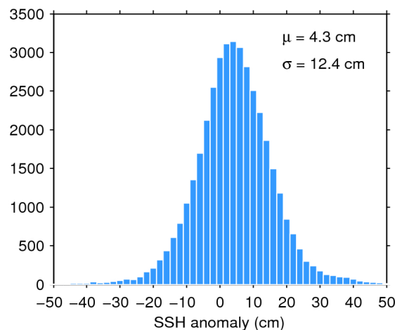
Figure 11. Histogram of science-valid SSH anomaly over oceans and lakes for 10/01/2020. The mean ( \mu ) and standard deviation ( \sigma ) are also shown. Note that values outside [-50 50] cm are excluded from the histogram for the sake of readability but not from the computation of \mu and \sigma .
