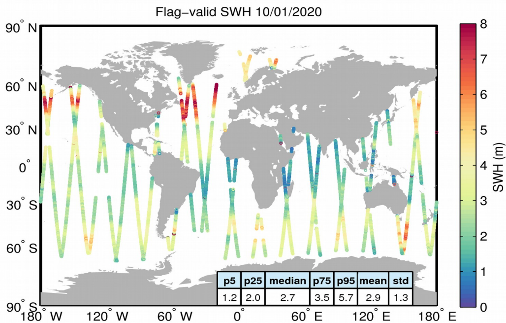
Figure 15. Geographical distribution of flag-valid SWH data over oceans and lakes for 10/01/2020. The statistical values shown in the table refer to the SWH in m and are calculated over all measurements shown in the figure.
