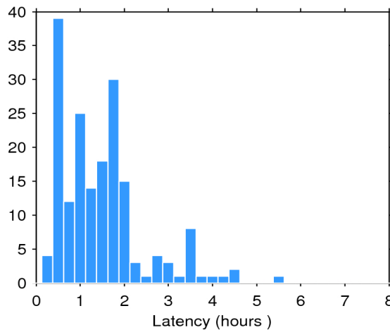
Figure 2. Histogram of the data latency for 10/01/2020. The y-axis denotes the number of files that are made available with a delay of x-hours with respect to the mean time of the records stored in the file.
