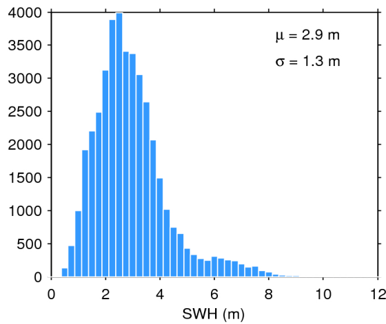
Figure 17. Histogram of flag-valid SWH over oceans and lakes for 10/01/2020. The mean ( \mu ) and standard deviation ( \sigma ) are also shown. Note that values larger than 12 m are excluded from the histogram for the sake of readability but not from the computation of \mu and \sigma .
