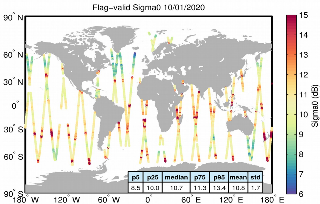
Figure 23. Geographical distribution of flag-valid sigma0 data over oceans and lakes for 10/01/2020. The statistical values shown in the table refer to the sigma0 in dB and are calculated over all measurements shown in the figure.
