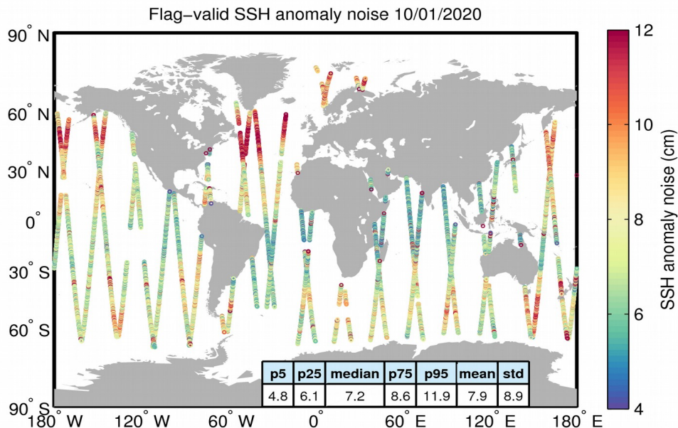
Figure 8. Geographical distribution of flag-valid 20-Hz SSH anomaly measurement noise over oceans and lakes for 10/01/2020. The statistical values shown in the table refer to the SSH anomaly noise and are calculated over all measurements shown in the figure.
