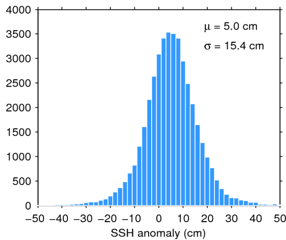
Figure 7. Histogram of flag-valid SSH anomaly over oceans and lakes for 09/01/2020. The mean ( \mu ) and standard deviation ( \sigma ) are also shown. Note that values outside [-50\ 50] cm are excluded from the histogram for the sake of readability but not from the computation of \mu and \sigma .
