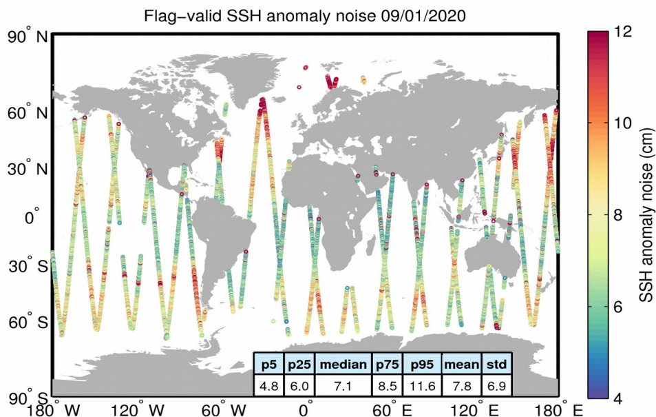
Figure 8. Geographical distribution of flag-valid 20-Hz SSH anomaly measurement noise over oceans and lakes for 09/01/2020. The statistical values shown in the table refer to the SSH anomaly noise and are calculated over all measurements shown in the figure.
