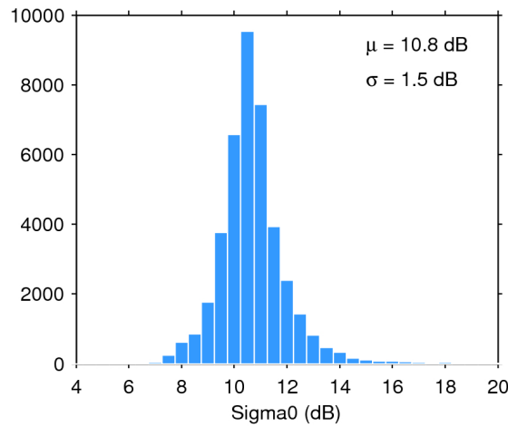
Figure 28. Histogram of science-valid sigma0 over oceans and lakes for 09/01/2020. The mean ( \mu ) and standard deviation ( \sigma ) are also shown. Note that values outside [4 20] dB are excluded from the histogram for the sake of readability but not from the computation of \mu and \sigma .
