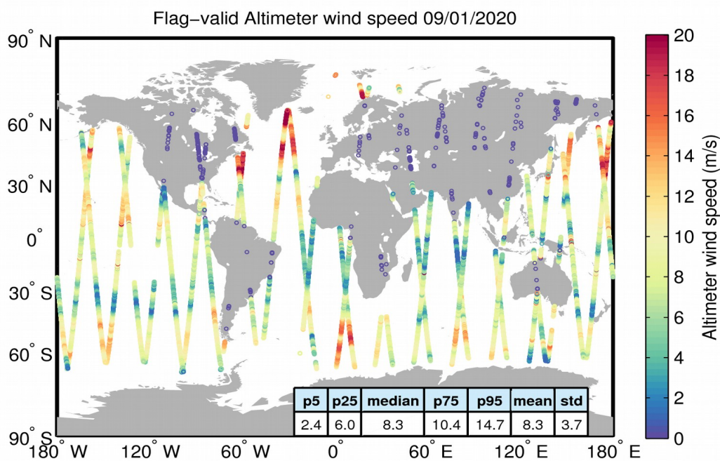
Figure 31. Geographical distribution of flag-valid wind data over oceans and lakes for 09/01/2020. The statistical values shown in the table refer to the wind in m/s and are calculated over all measurements shown in the figure.
