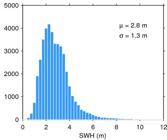
Figure 17. Histogram of flag-valid SWH over oceans and lakes for 09/01/2020. The mean ( \mu ) and standard deviation ( \sigma ) are also shown. Note that values larger than 12 m are excluded from the histogram for the sake of readability but not from the computation of \mu and \sigma .
