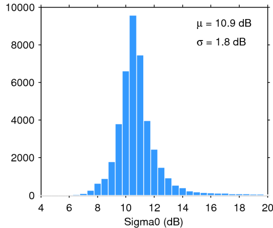
Figure 25. Histogram of flag-valid sigma0 over oceans and lakes for 09/01/2020. The mean ( \mu ) and standard deviation ( \sigma ) are also shown. Note that values outside [4 20] dB are excluded from the histogram for the sake of readability but not from the computation of \mu and \sigma .
