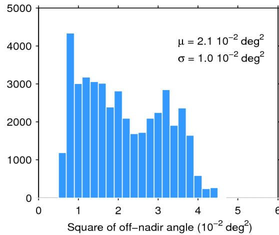
Figure 39. Histogram of flag-valid mispointing over oceans and lakes for 09/01/2020. The mean ( \mu ) and standard deviation ( \sigma ) are also shown. Note that values larger than 6 \cdot 10^{-2} \text{ deg}^2 are excluded from the histogram for the sake of readability but not from the computation of \mu and \sigma .
