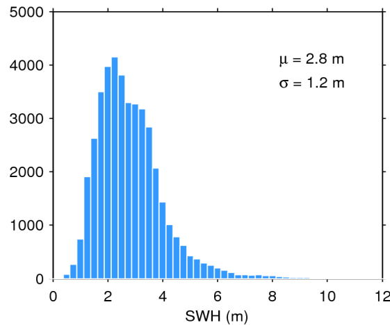
Figure 20. Histogram of science-valid SWH over oceans and lakes for 09/01/2020. The mean ( \mu ) and standard deviation ( \sigma ) are also shown. Note that values larger than 12 m are excluded from the histogram for the sake of readability but not from the computation of \mu and \sigma .
