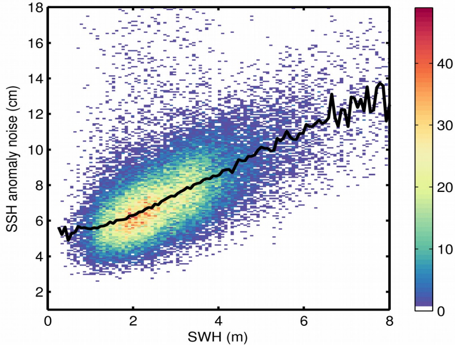
Figure 9. 2D histogram showing flag-valid SSH anomaly noise as a function of SWH for 09/01/2020. The black line denotes the median SSH anomaly noise as a function of SWH.
