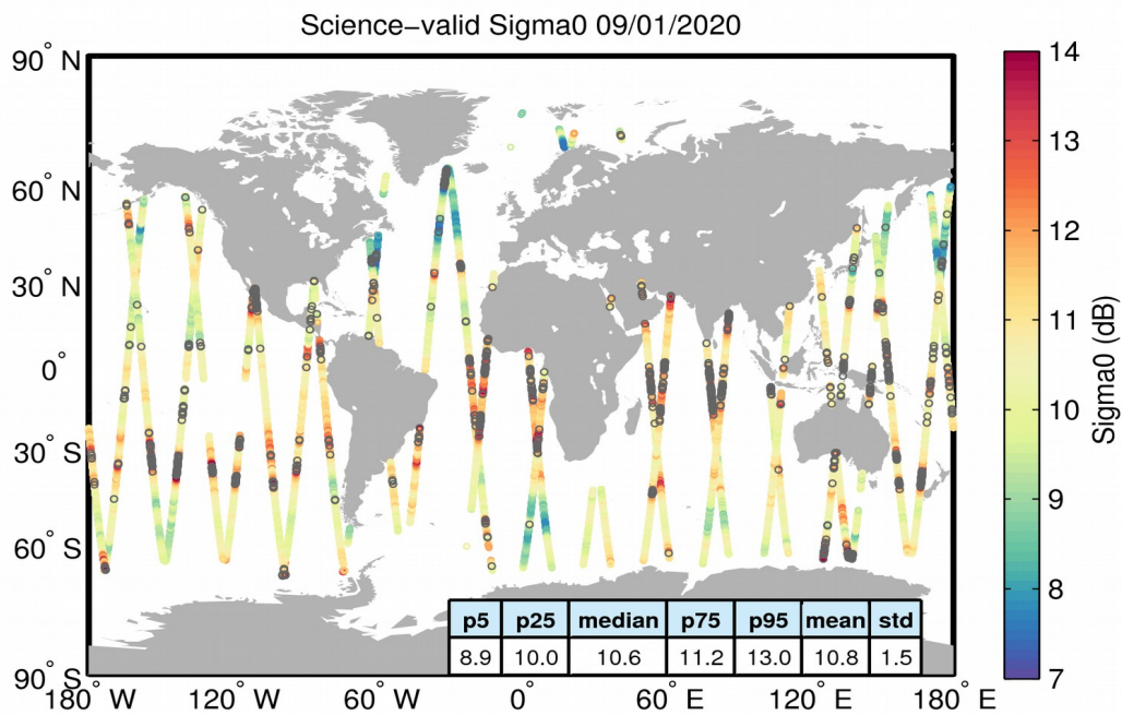
Figure 27. Geographical distribution of science-valid sigma0 data over oceans and lakes for 09/01/2020. The statistical values shown in the table refer to the sigma0 in dB and are calculated over all measurements shown in the figure. Gray circles denote records that have been rejected based on the editing criteria described in Table 4.
