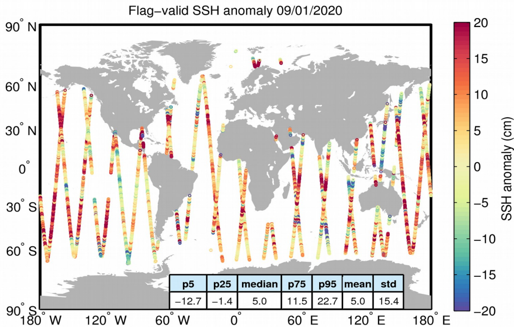
Figure 5. Geographical distribution of flag-valid 1-Hz SSH anomaly data over oceans and lakes for 09/01/2020. The statistical values shown in the table refer to the SSH anomaly in cm and are calculated over all measurements shown in the figure.
