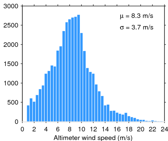
Figure 35. Histogram of science-valid wind over oceans and lakes for 09/01/2020. The mean ( \mu ) and standard deviation ( \sigma ) are also shown. Note that values larger than 24 m/s are excluded from the histogram for the sake of readability but not from the computation of \mu and \sigma .
