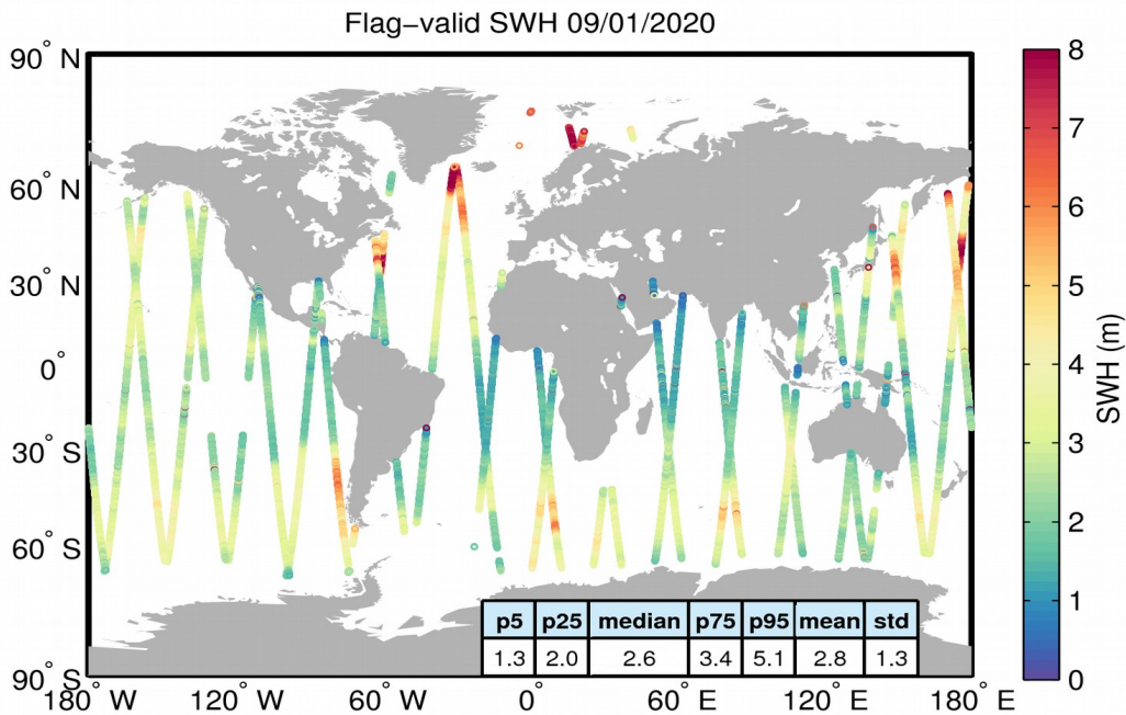
Figure 15. Geographical distribution of flag-valid SWH data over oceans and lakes for 09/01/2020. The statistical values shown in the table refer to the SWH in m and are calculated over all measurements shown in the figure.
