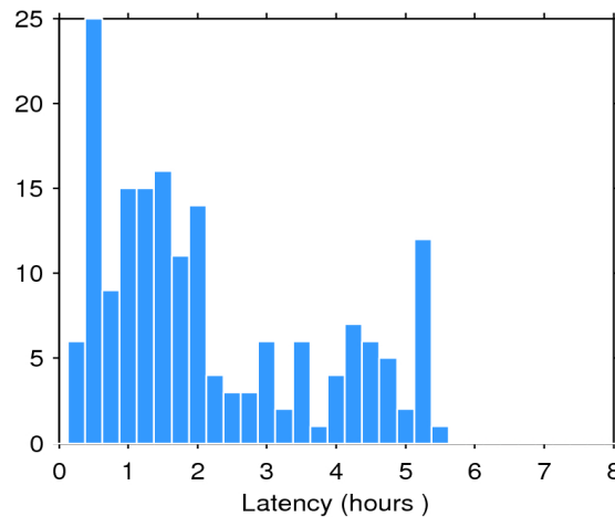
Figure 2. Histogram of the data latency for 09/01/2020. The y-axis denotes the number of files that are made available with a delay of x-hours with respect to the mean time of the records stored in the file.
