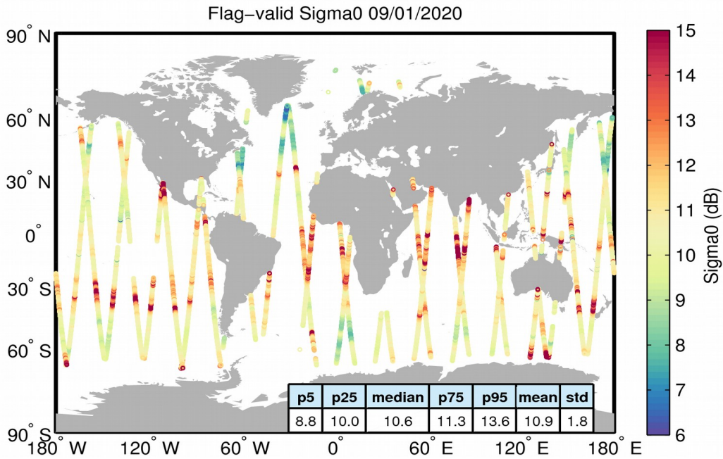
Figure 23. Geographical distribution of flag-valid sigma0 data over oceans and lakes for 09/01/2020. The statistical values shown in the table refer to the sigma0 in dB and are calculated over all measurements shown in the figure.
