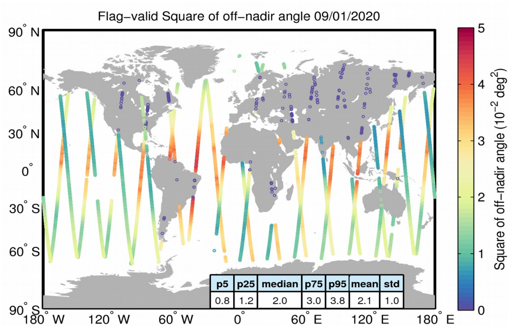
Figure 37. Geographical distribution of flag-valid mispointing data over oceans and lakes for 09/01/2020. The statistical values shown in the table refer to the mispointing in 10^{-2} \text{ deg}^2 and are calculated over all measurements shown in the figure.
