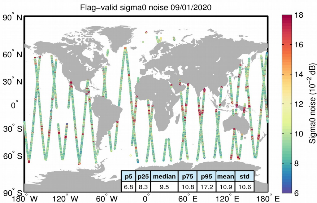
Figure 26. Geographical distribution of flag-valid 20-Hz sigma0 measurement noise over oceans and lakes for 09/01/2020. The statistical values shown in the table refer to the sigma0 noise and are calculated over all measurements shown in the figure.
