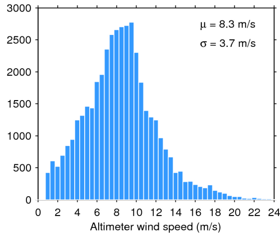
Figure 33. Histogram of flag-valid wind over oceans and lakes for 09/01/2020. The mean ( \mu ) and standard deviation ( \sigma ) are also shown. Note that values larger than 24 m/s are excluded from the histogram for the sake of readability but not from the computation of \mu and \sigma .
