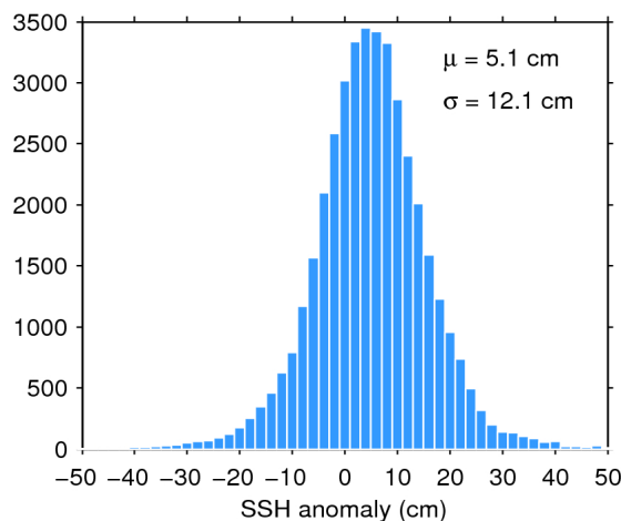
Figure 11. Histogram of science-valid SSH anomaly over oceans and lakes for 09/01/2020. The mean ( \mu ) and standard deviation ( \sigma ) are also shown. Note that values outside [-50 50] cm are excluded from the histogram for the sake of readability but not from the computation of \mu and \sigma .
