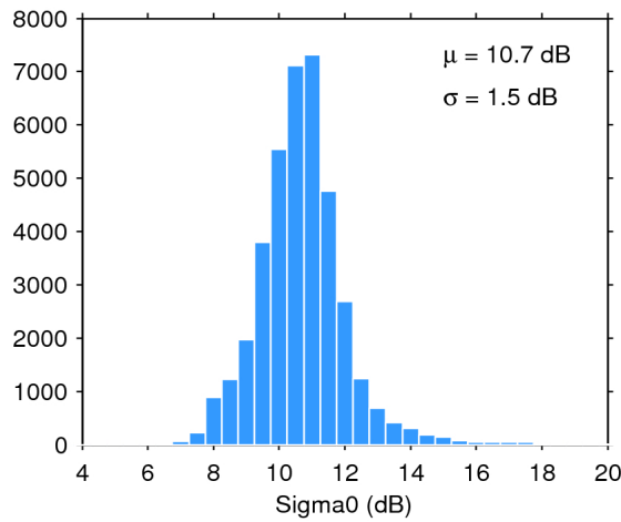
Figure 28. Histogram of science-valid sigma0 over oceans and lakes for 07/01/2020. The mean ( \mu ) and standard deviation ( \sigma ) are also shown. Note that values outside [4 20] dB are excluded from the histogram for the sake of readability but not from the computation of \mu and \sigma .
