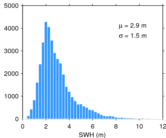
Figure 20. Histogram of science-valid SWH over oceans and lakes for 07/01/2020. The mean ( \mu ) and standard deviation ( \sigma ) are also shown. Note that values larger than 12 m are excluded from the histogram for the sake of readability but not from the computation of \mu and \sigma .
