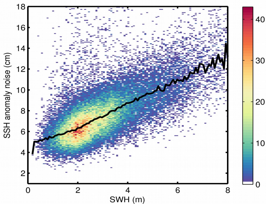
Figure 9. 2D histogram showing flag-valid SSH anomaly noise as a function of SWH for 07/01/2020. The black line denotes the median SSH anomaly noise as a function of SWH.
