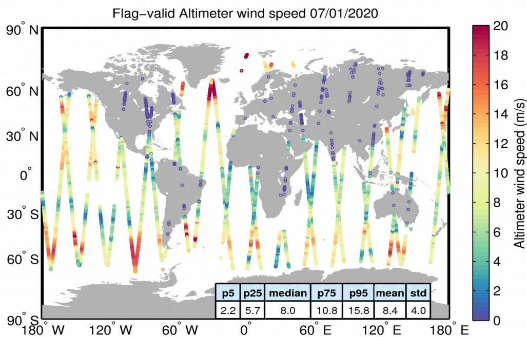
Figure 31. Geographical distribution of flag-valid wind data over oceans and lakes for 07/01/2020. The statistical values shown in the table refer to the wind in m/s and are calculated over all measurements shown in the figure.
