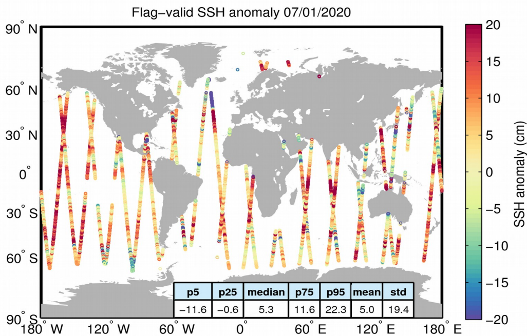
Figure 5. Geographical distribution of flag-valid 1-Hz SSH anomaly data over oceans and lakes for 07/01/2020. The statistical values shown in the table refer to the SSH anomaly in cm and are calculated over all measurements shown in the figure.
