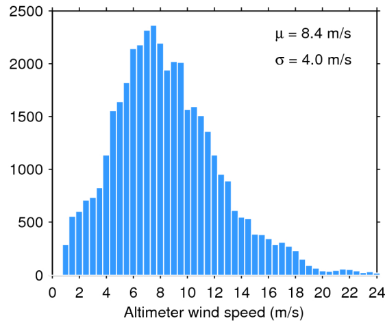
Figure 33. Histogram of flag-valid wind over oceans and lakes for 07/01/2020. The mean ( \mu ) and standard deviation ( \sigma ) are also shown. Note that values larger than 24 m/s are excluded from the histogram for the sake of readability but not from the computation of \mu and \sigma .
