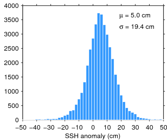
Figure 7. Histogram of flag-valid SSH anomaly over oceans and lakes for 07/01/2020. The mean ( \mu ) and standard deviation ( \sigma ) are also shown. Note that values outside [-50 50] cm are excluded from the histogram for the sake of readability but not from the computation of \mu and \sigma .
