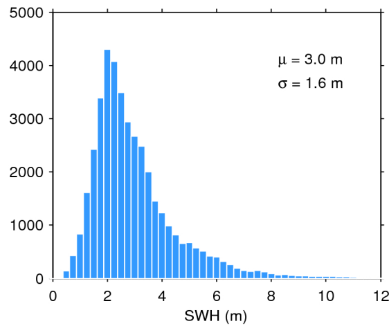
Figure 17. Histogram of flag-valid SWH over oceans and lakes for 07/01/2020. The mean ( \mu ) and standard deviation ( \sigma ) are also shown. Note that values larger than 12 m are excluded from the histogram for the sake of readability but not from the computation of \mu and \sigma .
