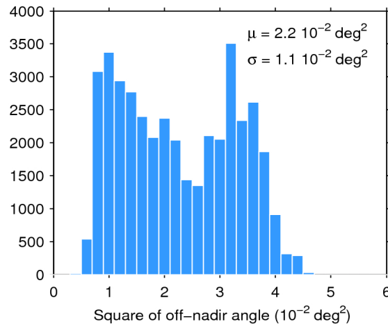
Figure 39. Histogram of flag-valid mispointing over oceans and lakes for 07/01/2020. The mean ( \mu ) and standard deviation ( \sigma ) are also shown. Note that values larger than 6 \cdot 10^{-2} \text{ deg}^2 are excluded from the histogram for the sake of readability but not from the computation of \mu and \sigma .
