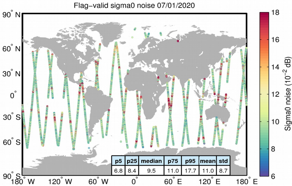
Figure 26. Geographical distribution of flag-valid 20-Hz sigma0 measurement noise over oceans and lakes for 07/01/2020. The statistical values shown in the figure refer to the sigma0 noise and are calculated over all measurements shown in the figure.
