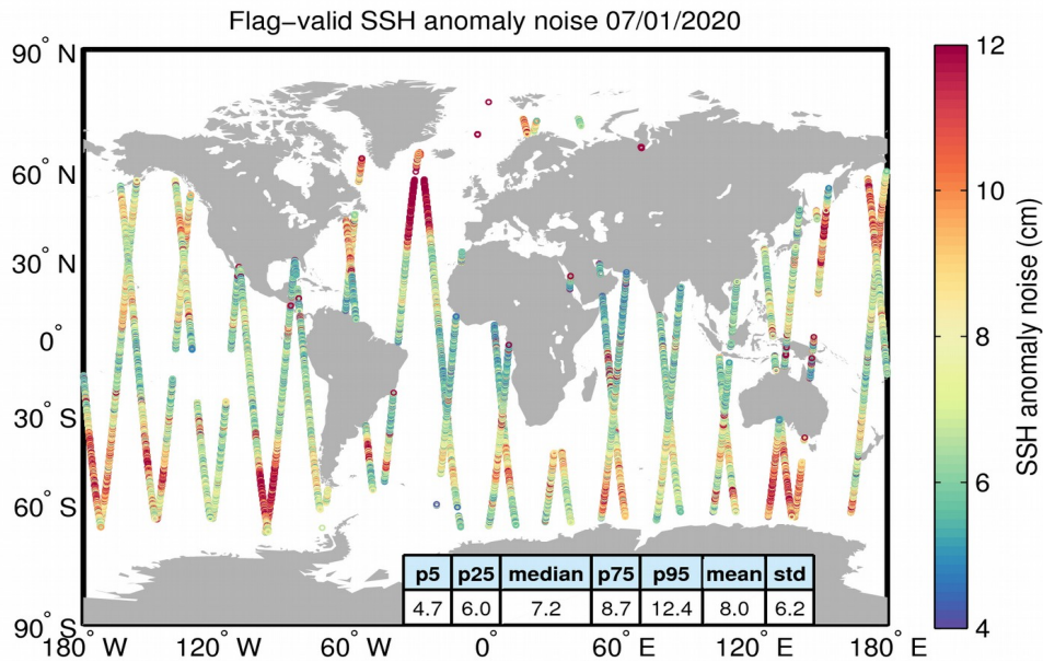
Figure 8. Geographical distribution of flag-valid 20-Hz SSH anomaly measurement noise over oceans and lakes for 07/01/2020. The statistical values shown in the table refer to the SSH anomaly noise and are calculated over all measurements shown in the figure.
