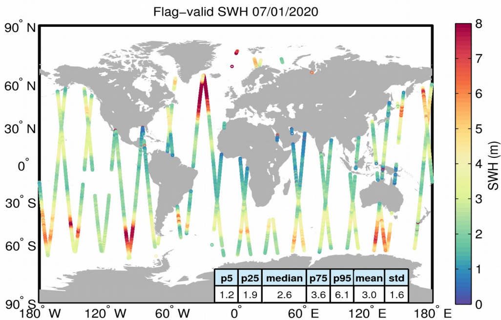
Figure 15. Geographical distribution of flag-valid SWH data over oceans and lakes for 07/01/2020. The statistical values shown in the table refer to the SWH in m and are calculated over all measurements shown in the figure.
