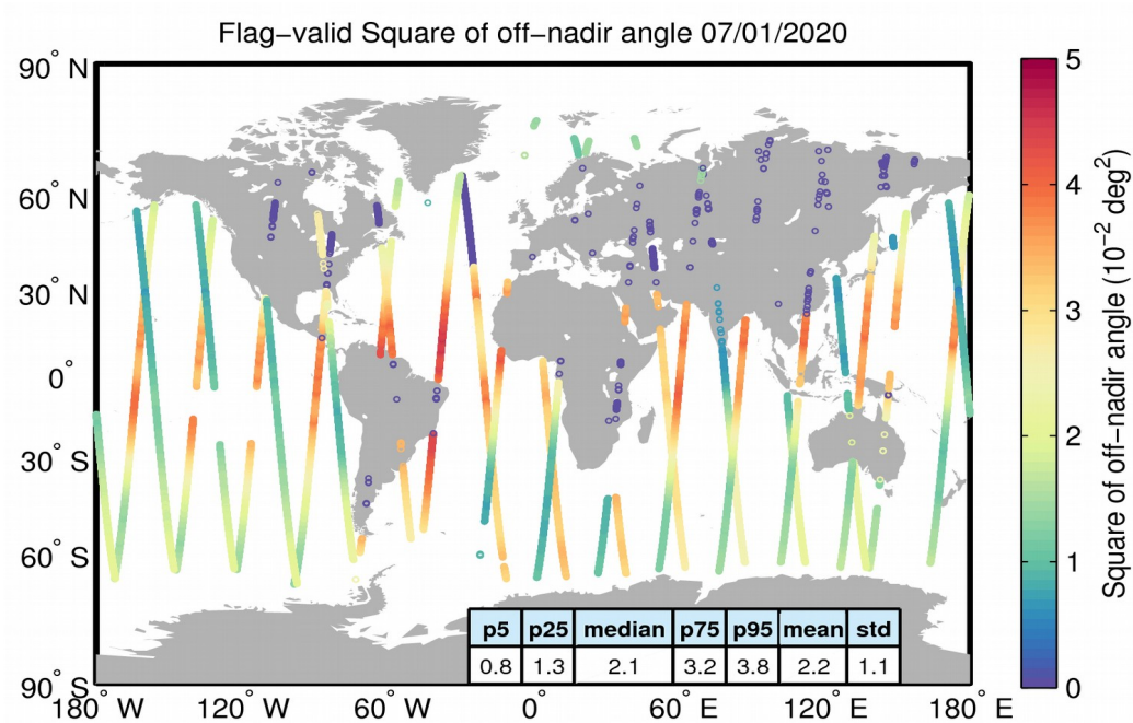
Figure 37. Geographical distribution of flag-valid mispointing data over oceans and lakes for 07/01/2020. The statistical values shown in the table refer to the mispointing in 10^{-2} deg 2 and are calculated over all measurements shown in the figure.
