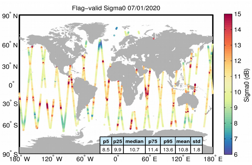
Figure 23. Geographical distribution of flag-valid sigma0 data over oceans and lakes for 07/01/2020. The statistical values shown in the table refer to the sigma0 in dB and are calculated over all measurements shown in the figure.
