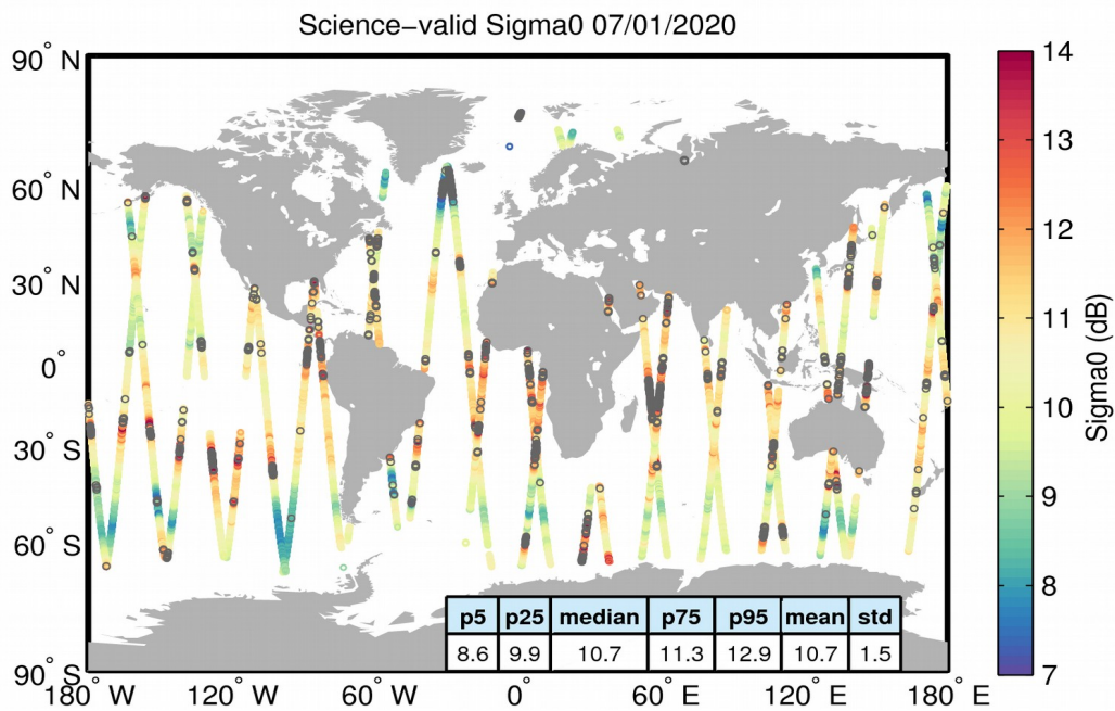
Figure 27. Geographical distribution of science-valid sigma0 data over oceans and lakes for 07/01/2020. The statistical values shown in the table refer to the sigma0 in dB and are calculated over all measurements shown in the figure. Gray circles denote records that have been rejected based on the editing criteria described in Table 4.
