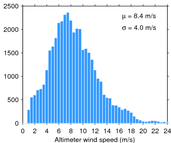
Figure 35. Histogram of science-valid wind over oceans and lakes for 07/01/2020. The mean ( \mu ) and standard deviation ( \sigma ) are also shown. Note that values larger than 24 m/s are excluded from the histogram for the sake of readability but not from the computation of \mu and \sigma .
