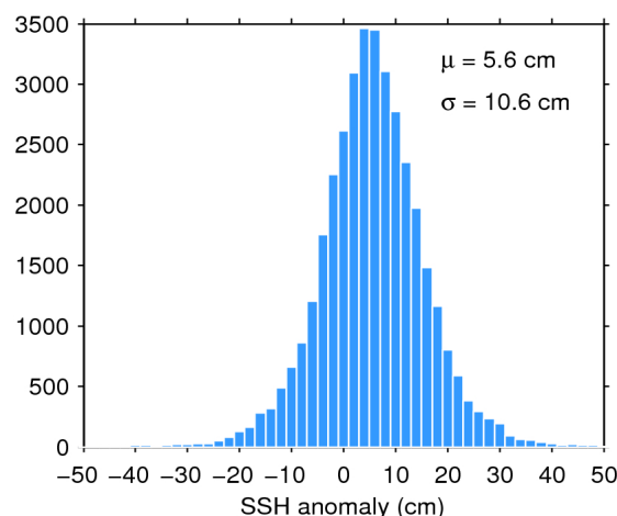
Figure 11. Histogram of science-valid SSH anomaly over oceans and lakes for 07/01/2020. The mean ( \mu ) and standard deviation ( \sigma ) are also shown. Note that values outside [-50 50] cm are excluded from the histogram for the sake of readability but not from the computation of \mu and \sigma .
