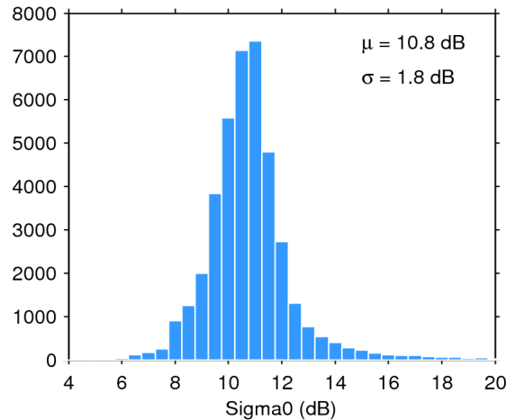
Figure 25. Histogram of flag-valid sigma0 over oceans and lakes for 07/01/2020. The mean ( \mu ) and standard deviation ( \sigma ) are also shown. Note that values outside [4 20] dB are excluded from the histogram for the sake of readability but not from the computation of \mu and \sigma .
