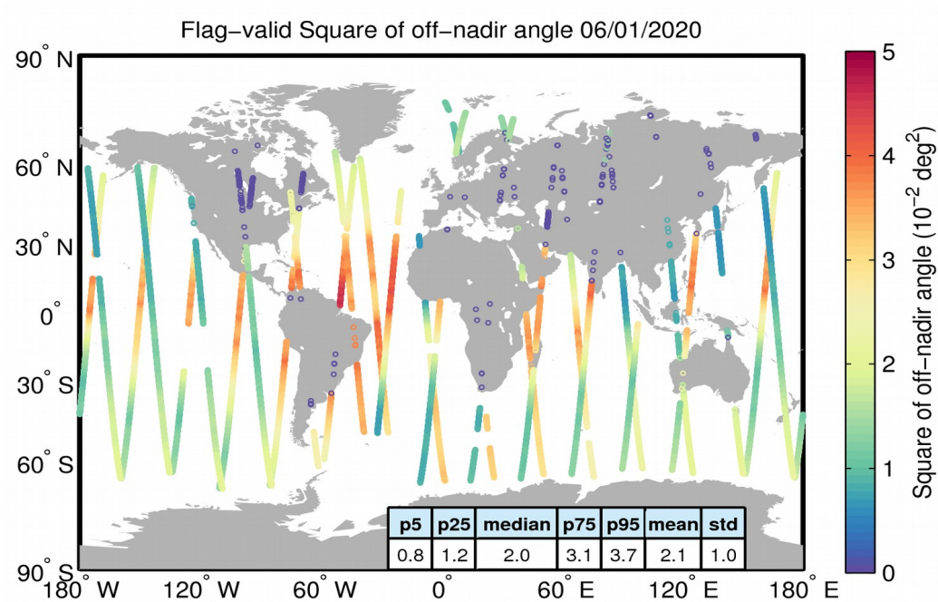
Figure 37. Geographical distribution of flag-valid mispointing data over oceans and lakes for 06/01/2020. The statistical values shown in the table refer to the mispointing in 10^{-2} deg 2 and are calculated over all measurements shown in the figure.
