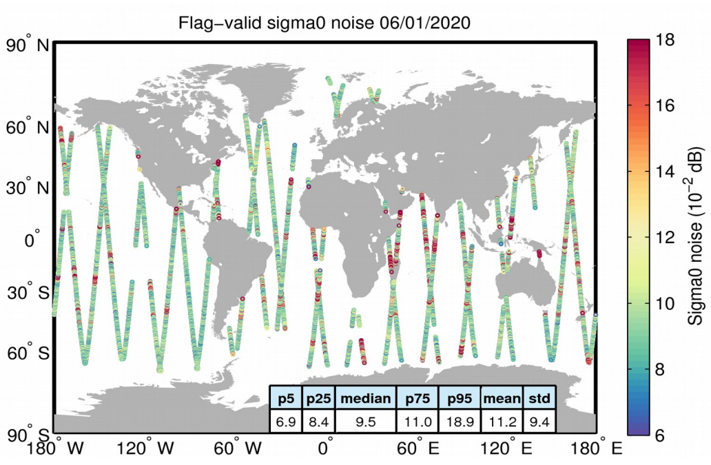
Figure 26. Geographical distribution of flag-valid 20-Hz sigma0 measurement noise over oceans and lakes for 06/01/2020. The statistical values shown in the table refer to the sigma0 noise and are calculated over all measurements shown in the figure.
