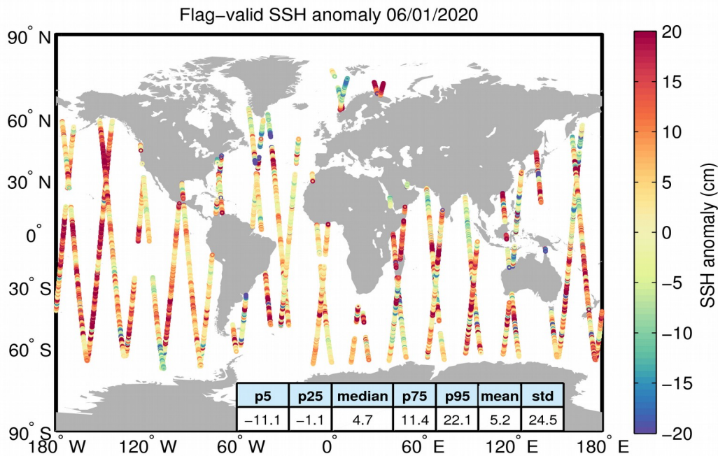
Figure 5. Geographical distribution of flag-valid 1-Hz SSH anomaly data over oceans and lakes for 06/01/2020. The statistical values shown in the table refer to the SSH anomaly in cm and are calculated over all measurements shown in the figure.
