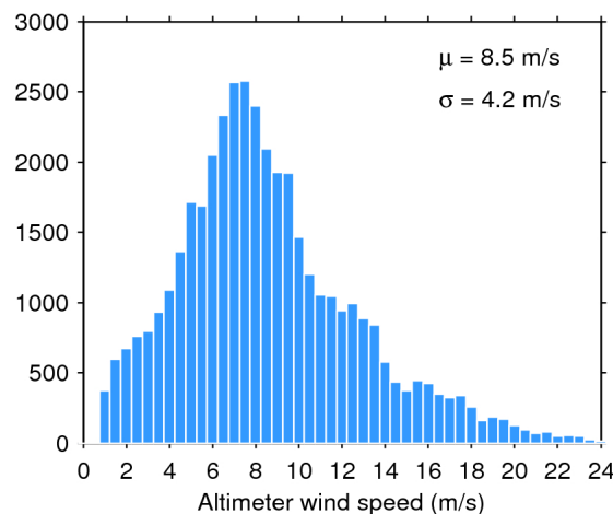
Figure 35. Histogram of science-valid wind over oceans and lakes for 06/01/2020. The mean ( \mu ) and standard deviation ( \sigma ) are also shown. Note that values larger than 24 m/s are excluded from the histogram for the sake of readability but not from the computation of \mu and \sigma .
