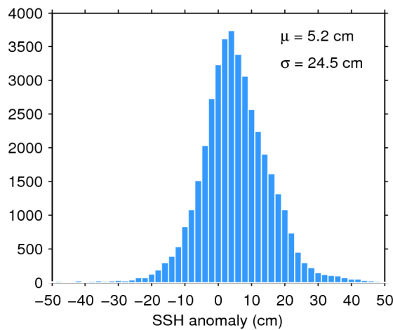
Figure 7. Histogram of flag-valid SSH anomaly over oceans and lakes for 06/01/2020. The mean ( \mu ) and standard deviation ( \sigma ) are also shown. Note that values outside [-50 50] cm are excluded from the histogram for the sake of readability but not from the computation of \mu and \sigma .
