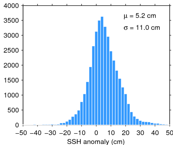
Figure 11. Histogram of science-valid SSH anomaly over oceans and lakes for 06/01/2020. The mean ( \mu ) and standard deviation ( \sigma ) are also shown. Note that values outside [-50 50] cm are excluded from the histogram for the sake of readability but not from the computation of \mu and \sigma .
