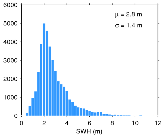
Figure 20. Histogram of science-valid SWH over oceans and lakes for 06/01/2020. The mean ( \mu ) and standard deviation ( \sigma ) are also shown. Note that values larger than 12 m are excluded from the histogram for the sake of readability but not from the computation of \mu and \sigma .
