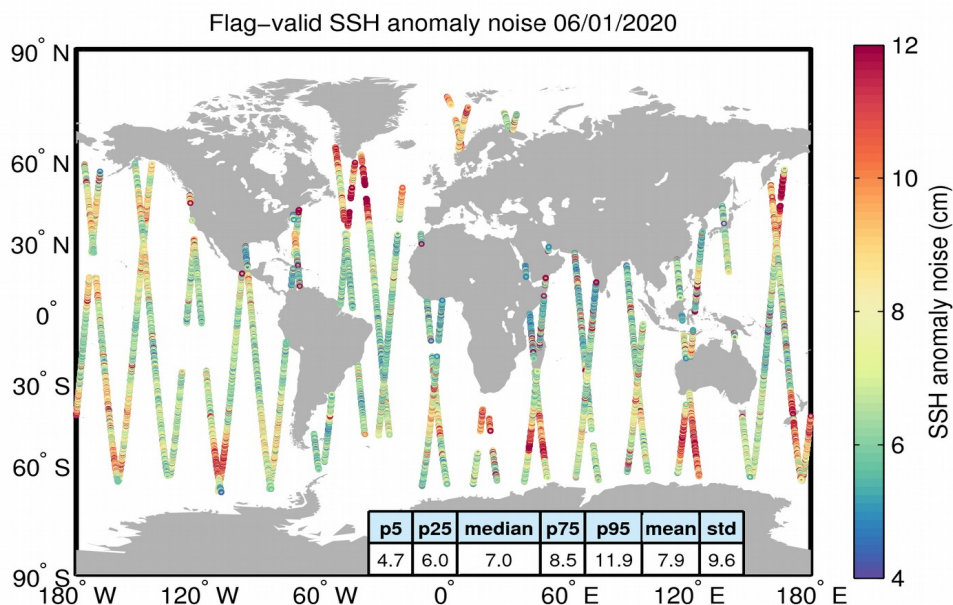
Figure 8. Geographical distribution of flag-valid 20-Hz SSH anomaly measurement noise over oceans and lakes for 06/01/2020. The statistical values shown in the table refer to the SSH anomaly noise and are calculated over all measurements shown in the figure.
