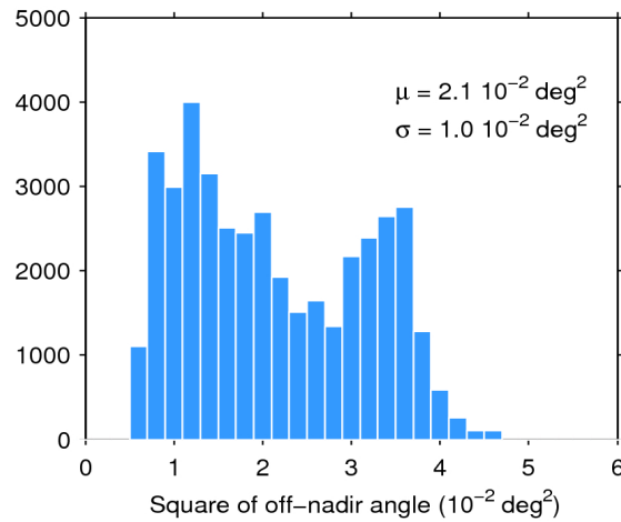
Figure 39. Histogram of flag-valid mispointing over oceans and lakes for 06/01/2020. The mean ( \mu ) and standard deviation ( \sigma ) are also shown. Note that values larger than 6 \cdot 10^{-2} \text{ deg}^2 are excluded from the histogram for the sake of readability but not from the computation of \mu and \sigma .
