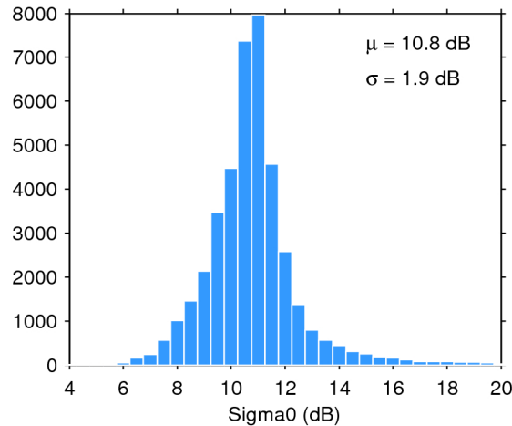
Figure 25. Histogram of flag-valid sigma0 over oceans and lakes for 06/01/2020. The mean ( \mu ) and standard deviation ( \sigma ) are also shown. Note that values outside [4 20] dB are excluded from the histogram for the sake of readability but not from the computation of \mu and \sigma .
