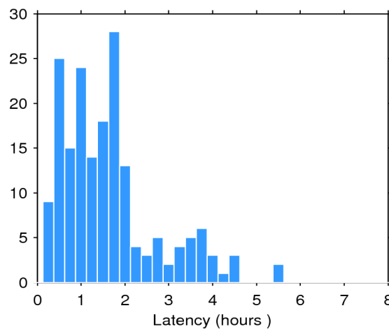
Figure 2. Histogram of the data latency for 06/01/2020. The y-axis denotes the number of files that are made available with a delay of x-hours with respect to the mean time of the records stored in the file.
