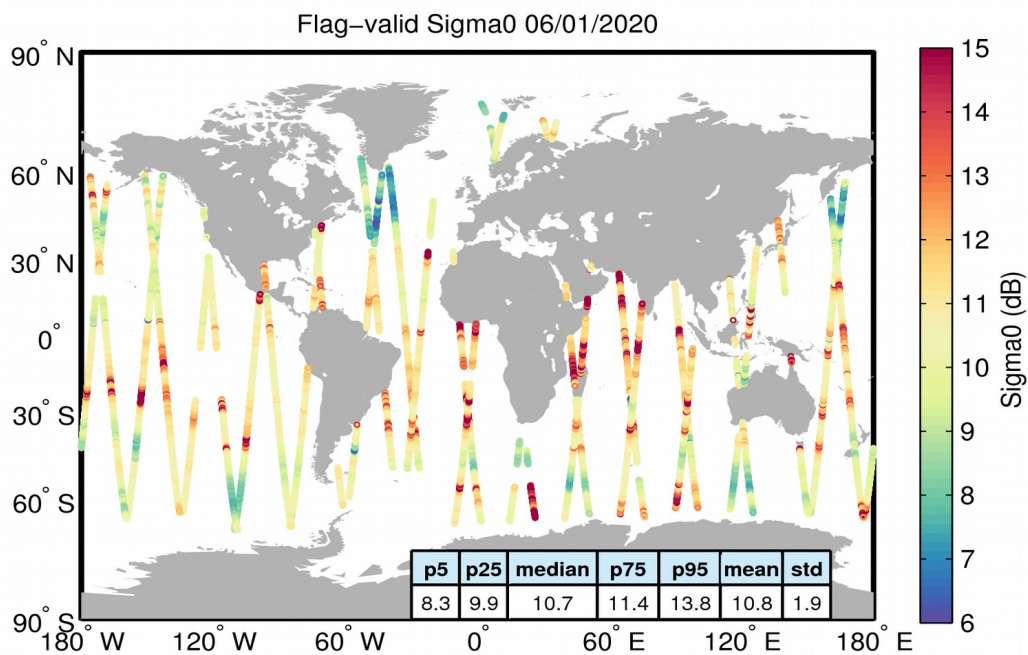
Figure 23. Geographical distribution of flag-valid sigma0 data over oceans and lakes for 06/01/2020. The statistical values shown in the table refer to the sigma0 in dB and are calculated over all measurements shown in the figure.
