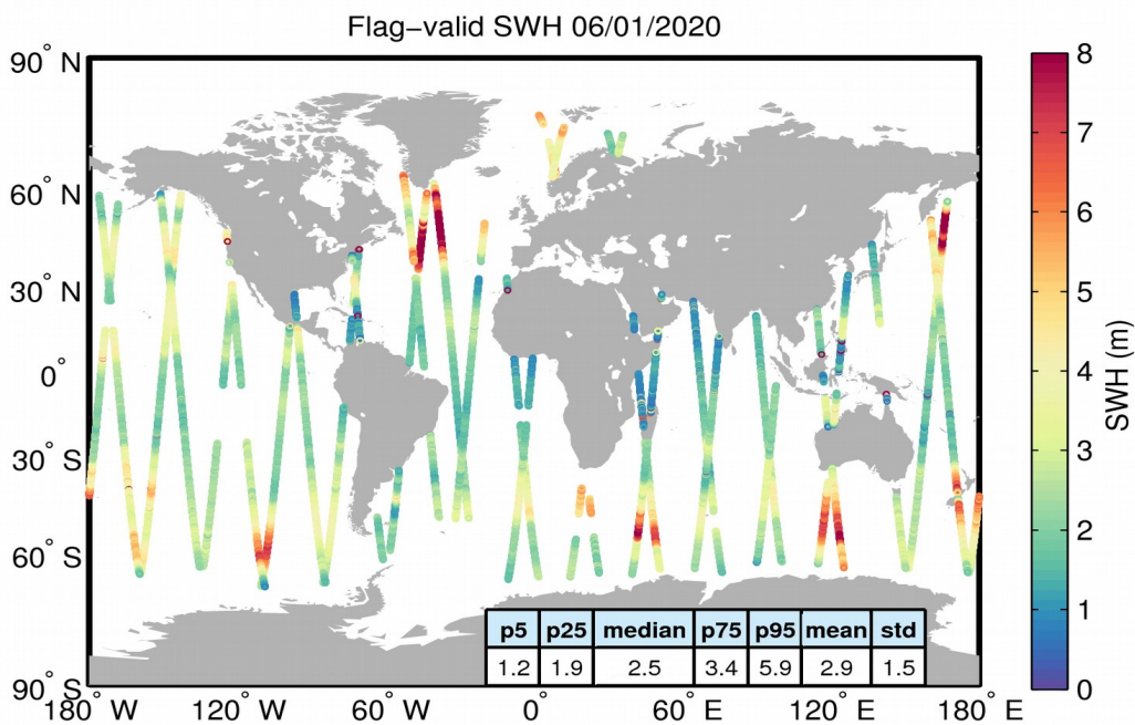
Figure 15. Geographical distribution of flag-valid SWH data over oceans and lakes for 06/01/2020. The statistical values shown in the table refer to the SWH in m and are calculated over all measurements shown in the figure.
