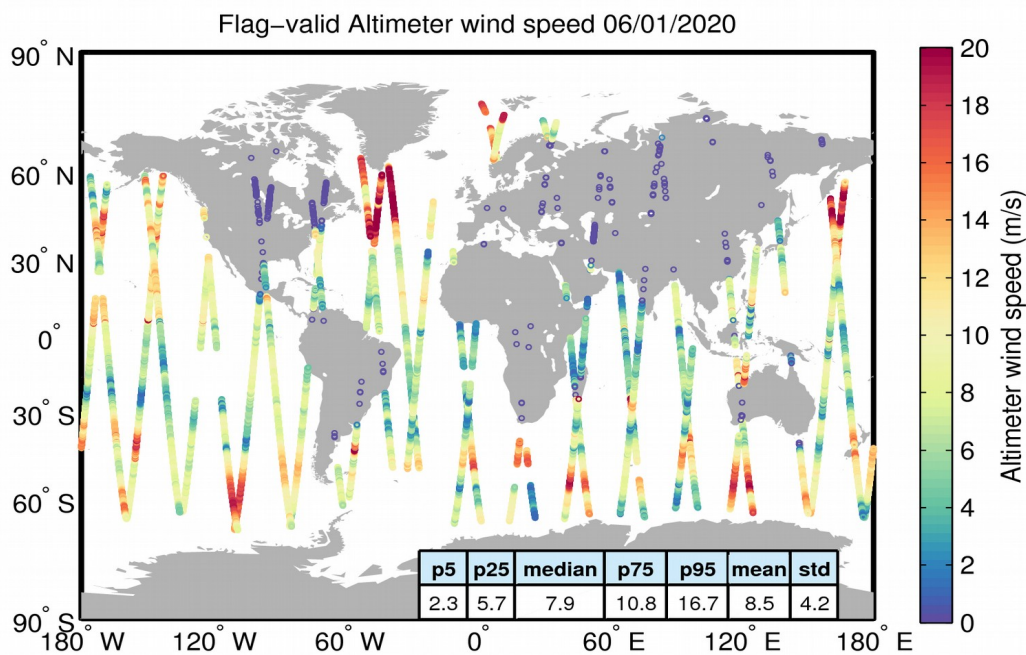
Figure 31. Geographical distribution of flag-valid wind data over oceans and lakes for 06/01/2020. The statistical values shown in the table refer to the wind in m/s and are calculated over all measurements shown in the figure.
