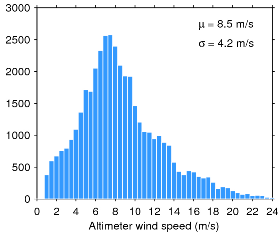
Figure 33. Histogram of flag-valid wind over oceans and lakes for 06/01/2020. The mean ( \mu ) and standard deviation ( \sigma ) are also shown. Note that values larger than 24 m/s are excluded from the histogram for the sake of readability but not from the computation of \mu and \sigma .
