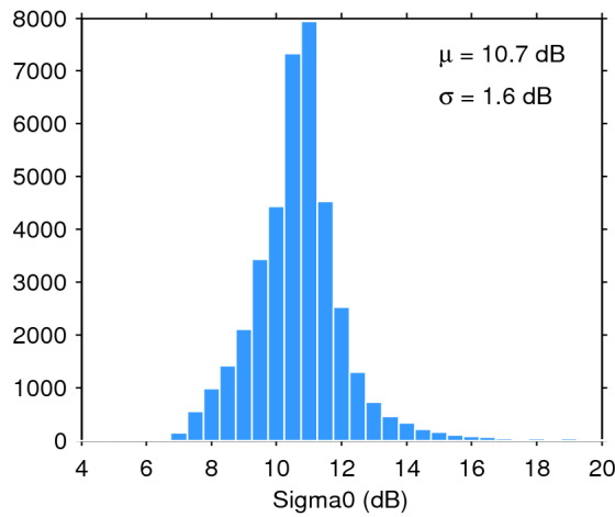
Figure 28. Histogram of science-valid sigma0 over oceans and lakes for 06/01/2020. The mean ( \mu ) and standard deviation ( \sigma ) are also shown. Note that values outside [4 20] dB are excluded from the histogram for the sake of readability but not from the computation of \mu and \sigma .
