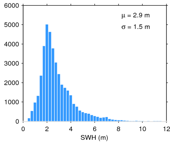
Figure 17. Histogram of flag-valid SWH over oceans and lakes for 06/01/2020. The mean ( \mu ) and standard deviation ( \sigma ) are also shown. Note that values larger than 12 m are excluded from the histogram for the sake of readability but not from the computation of \mu and \sigma .
