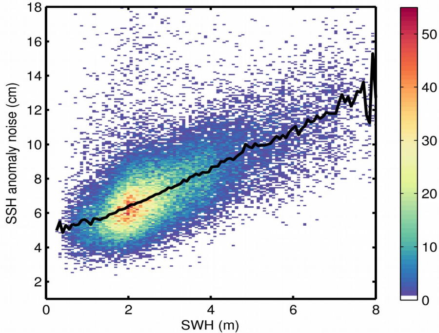
Figure 9. 2D histogram showing flag-valid SSH anomaly noise as a function of SWH for 06/01/2020. The black line denotes the median SSH anomaly noise as a function of SWH.
