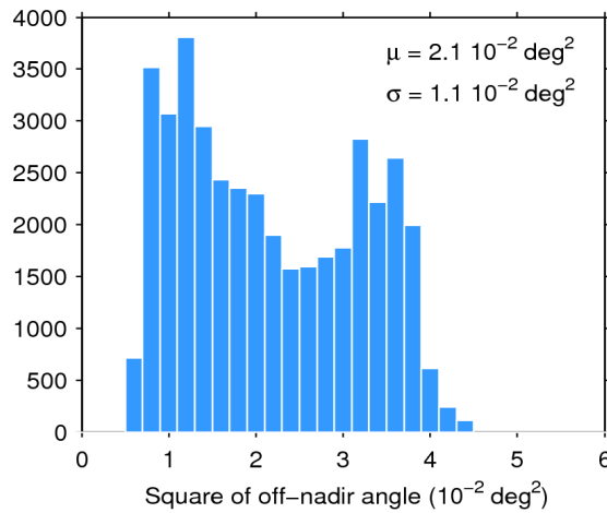
Figure 39. Histogram of flag-valid mispointing over oceans and lakes for 05/01/2020. The mean ( \mu ) and standard deviation ( \sigma ) are also shown. Note that values larger than 6 \cdot 10^{-2} \text{ deg}^2 are excluded from the histogram for the sake of readability but not from the computation of \mu and \sigma .
