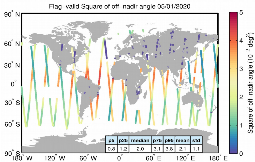
Figure 37. Geographical distribution of flag-valid mispointing data over oceans and lakes for 05/01/2020. The statistical values shown in the table refer to the mispointing in 10^{-2} \text{ deg}^2 and are calculated over all measurements shown in the figure.
