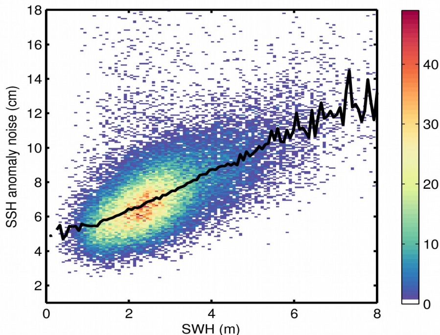
Figure 9. 2D histogram showing flag-valid SSH anomaly noise as a function of SWH for 05/01/2020. The black line denotes the median SSH anomaly noise as a function of SWH.
