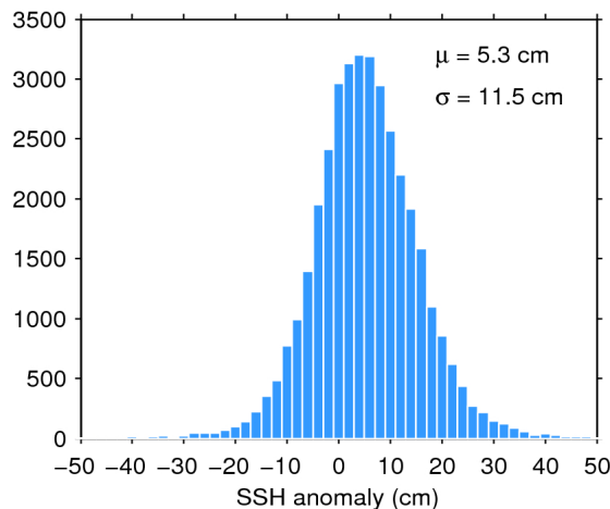
Figure 11. Histogram of science-valid SSH anomaly over oceans and lakes for 05/01/2020. The mean ( \mu ) and standard deviation ( \sigma ) are also shown. Note that values outside [-50 50] cm are excluded from the histogram for the sake of readability but not from the computation of \mu and \sigma .
