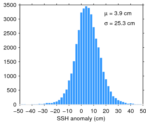
Figure 7. Histogram of flag-valid SSH anomaly over oceans and lakes for 05/01/2020. The mean ( \mu ) and standard deviation ( \sigma ) are also shown. Note that values outside [-50\ 50] cm are excluded from the histogram for the sake of readability but not from the computation of \mu and \sigma .
