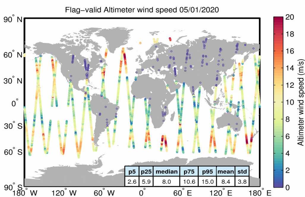
Figure 31. Geographical distribution of flag-valid wind data over oceans and lakes for 05/01/2020. The statistical values shown in the table refer to the wind in m/s and are calculated over all measurements shown in the figure.
