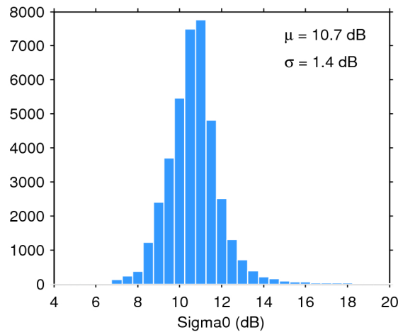
Figure 28. Histogram of science-valid sigma0 over oceans and lakes for 05/01/2020. The mean ( \mu ) and standard deviation ( \sigma ) are also shown. Note that values outside [4 20] dB are excluded from the histogram for the sake of readability but not from the computation of \mu and \sigma .
