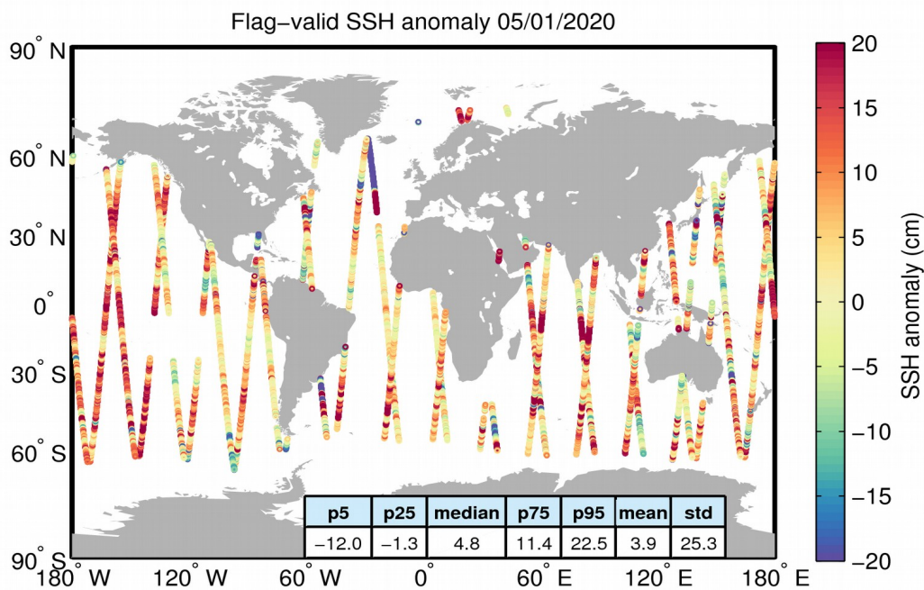
Figure 5. Geographical distribution of flag-valid 1-Hz SSH anomaly data over oceans and lakes for 05/01/2020. The statistical values shown in the table refer to the SSH anomaly in cm and are calculated over all measurements shown in the figure.
