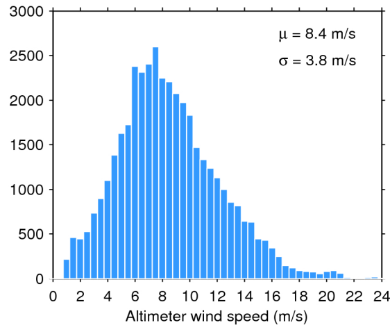
Figure 33. Histogram of flag-valid wind over oceans and lakes for 05/01/2020. The mean ( \mu ) and standard deviation ( \sigma ) are also shown. Note that values larger than 24 m/s are excluded from the histogram for the sake of readability but not from the computation of \mu and \sigma .
