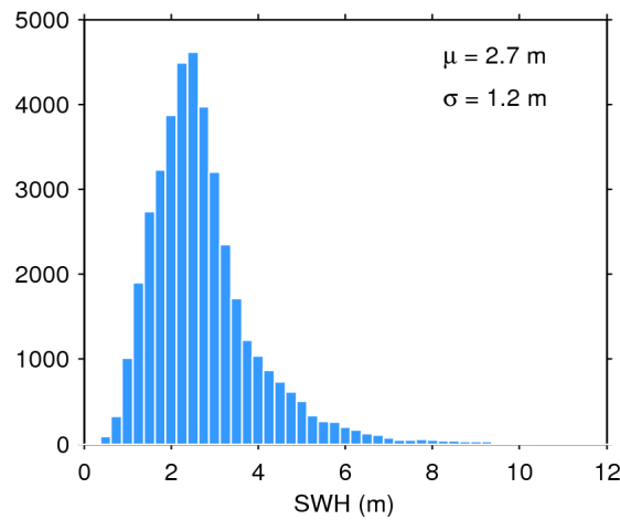
Figure 17. Histogram of flag-valid SWH over oceans and lakes for 05/01/2020. The mean ( \mu ) and standard deviation ( \sigma ) are also shown. Note that values larger than 12 m are excluded from the histogram for the sake of readability but not from the computation of \mu and \sigma .
