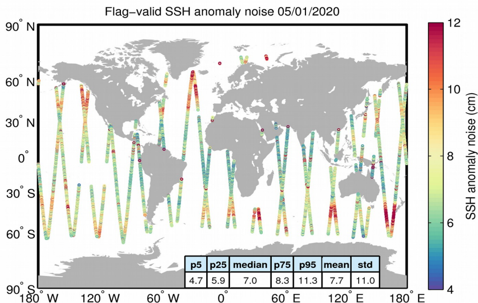
Figure 8. Geographical distribution of flag-valid 20-Hz SSH anomaly measurement noise over oceans and lakes for 05/01/2020. The statistical values shown in the table refer to the SSH anomaly noise and are calculated over all measurements shown in the figure.
