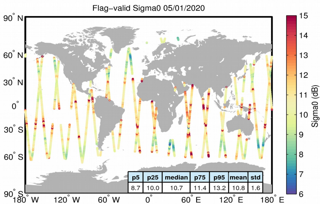
Figure 23. Geographical distribution of flag-valid sigma0 data over oceans and lakes for 05/01/2020. The statistical values shown in the table refer to the sigma0 in dB and are calculated over all measurements shown in the figure.
