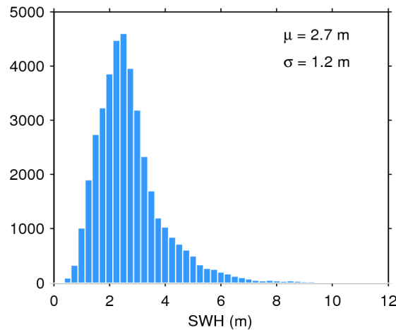
Figure 20. Histogram of science-valid SWH over oceans and lakes for 05/01/2020. The mean ( \mu ) and standard deviation ( \sigma ) are also shown. Note that values larger than 12 m are excluded from the histogram for the sake of readability but not from the computation of \mu and \sigma .
