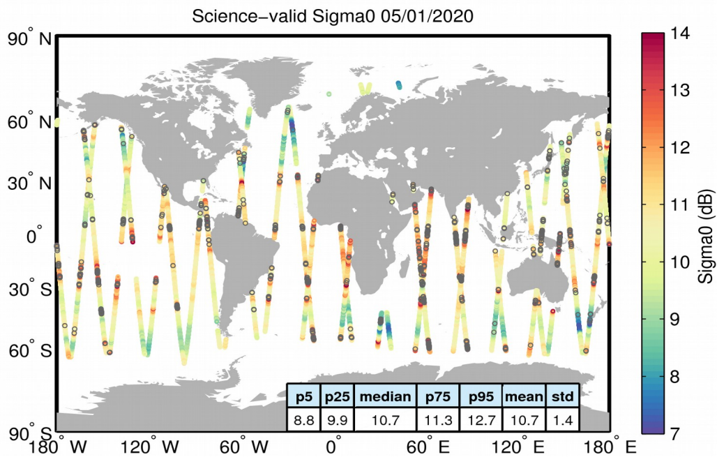
Figure 27. Geographical distribution of science-valid sigma0 data over oceans and lakes for 05/01/2020. The statistical values shown in the table refer to the sigma0 in dB and are calculated over all measurements shown in the figure. Gray circles denote records that have been rejected based on the editing criteria described in Table 4.
