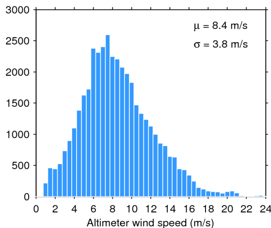
Figure 35. Histogram of science-valid wind over oceans and lakes for 05/01/2020. The mean ( \mu ) and standard deviation ( \sigma ) are also shown. Note that values larger than 24 m/s are excluded from the histogram for the sake of readability but not from the computation of \mu and \sigma .
