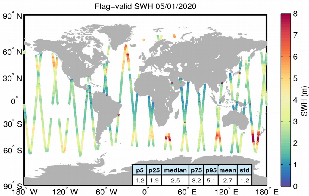
Figure 15. Geographical distribution of flag-valid SWH data over oceans and lakes for 05/01/2020. The statistical values shown in the table refer to the SWH in m and are calculated over all measurements shown in the figure.
