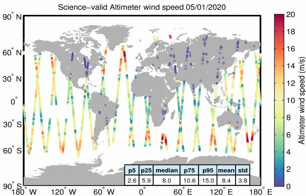
Figure 34. Geographical distribution of science-valid wind data over oceans and lakes for 05/01/2020. The statistical values shown in the table refer to the wind in m/s and are calculated over all measurements shown in the figure. Gray circles denote records that have been rejected based on the editing criteria described in Table 5.
