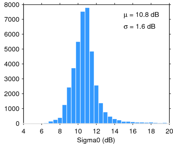
Figure 25. Histogram of flag-valid sigma0 over oceans and lakes for 05/01/2020. The mean ( \mu ) and standard deviation ( \sigma ) are also shown. Note that values outside [4 20] dB are excluded from the histogram for the sake of readability but not from the computation of \mu and \sigma .
