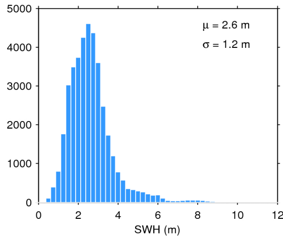
Figure 20. Histogram of science-valid SWH over oceans and lakes for 04/01/2020. The mean ( \mu ) and standard deviation ( \sigma ) are also shown. Note that values larger than 12 m are excluded from the histogram for the sake of readability but not from the computation of \mu and \sigma .
