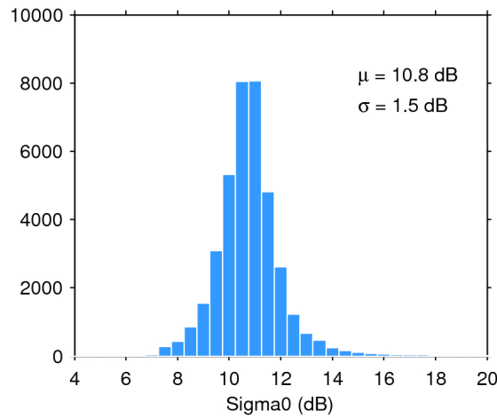
Figure 28. Histogram of science-valid sigma0 over oceans and lakes for 04/01/2020. The mean ( \mu ) and standard deviation ( \sigma ) are also shown. Note that values outside [4 20] dB are excluded from the histogram for the sake of readability but not from the computation of \mu and \sigma .
