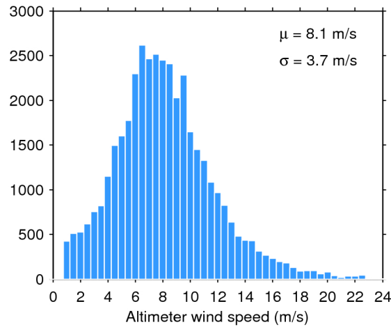
Figure 33. Histogram of flag-valid wind over oceans and lakes for 04/01/2020. The mean ( \mu ) and standard deviation ( \sigma ) are also shown. Note that values larger than 24 m/s are excluded from the histogram for the sake of readability but not from the computation of \mu and \sigma .
