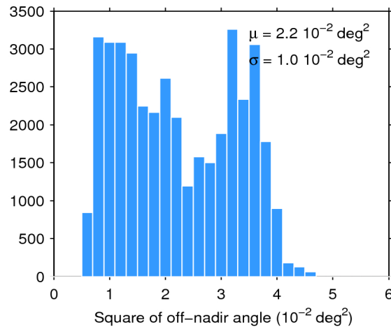
Figure 39. Histogram of flag-valid mispointing over oceans and lakes for 04/01/2020. The mean ( \mu ) and standard deviation ( \sigma ) are also shown. Note that values larger than 6 \cdot 10^{-2} \text{ deg}^2 are excluded from the histogram for the sake of readability but not from the computation of \mu and \sigma .
