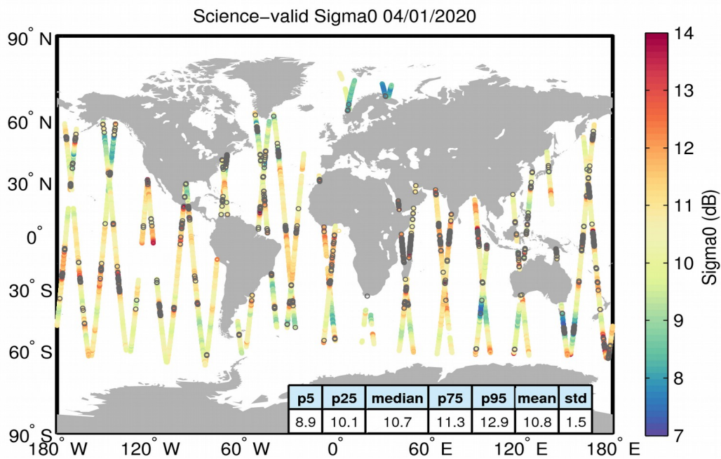
Figure 27. Geographical distribution of science-valid sigma0 data over oceans and lakes for 04/01/2020. The statistical values shown in the table refer to the sigma0 in dB and are calculated over all measurements shown in the figure. Gray circles denote records that have been rejected based on the editing criteria described in Table 4.
