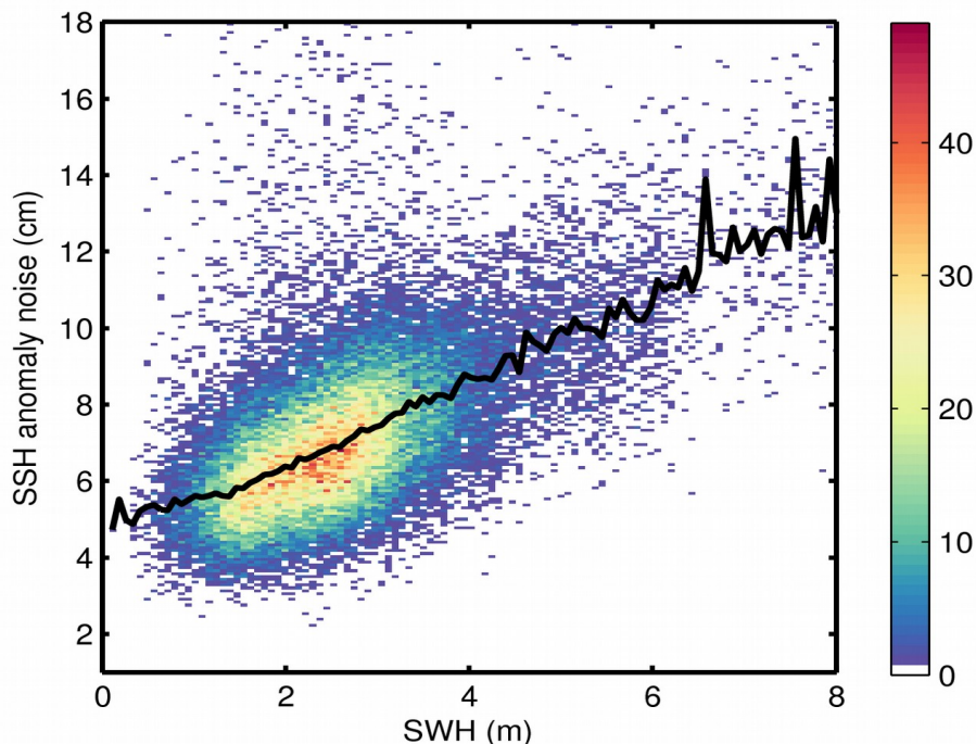
Figure 9. 2D histogram showing flag-valid SSH anomaly noise as a function of SWH for 04/01/2020. The black line denotes the median SSH anomaly noise as a function of SWH.
