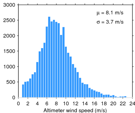
Figure 35. Histogram of science-valid wind over oceans and lakes for 04/01/2020. The mean ( \mu ) and standard deviation ( \sigma ) are also shown. Note that values larger than 24 m/s are excluded from the histogram for the sake of readability but not from the computation of \mu and \sigma .
