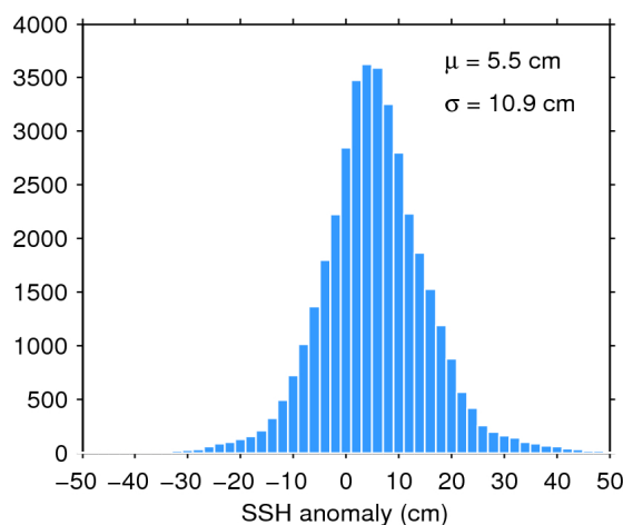
Figure 11. Histogram of science-valid SSH anomaly over oceans and lakes for 04/01/2020. The mean ( \mu ) and standard deviation ( \sigma ) are also shown. Note that values outside [-50 50] cm are excluded from the histogram for the sake of readability but not from the computation of \mu and \sigma .
