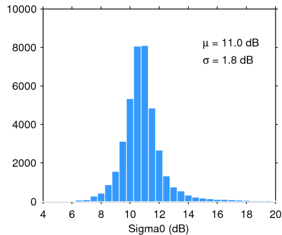
Figure 25. Histogram of flag-valid sigma0 over oceans and lakes for 04/01/2020. The mean ( \mu ) and standard deviation ( \sigma ) are also shown. Note that values outside [4 20] dB are excluded from the histogram for the sake of readability but not from the computation of \mu and \sigma .
