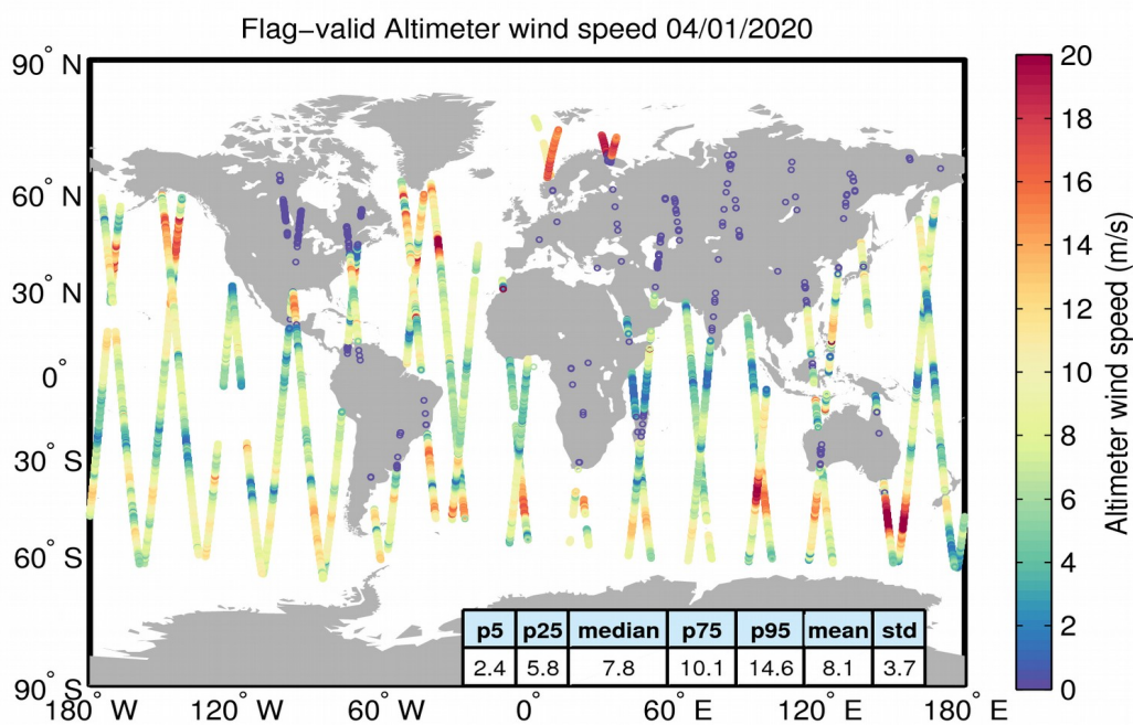
Figure 31. Geographical distribution of flag-valid wind data over oceans and lakes for 04/01/2020. The statistical values shown in the table refer to the wind in m/s and are calculated over all measurements shown in the figure.
