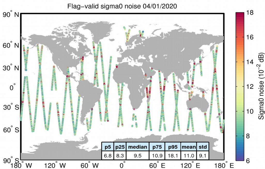
Figure 26. Geographical distribution of flag-valid 20-Hz sigma0 measurement noise over oceans and lakes for 04/01/2020. The statistical values shown in the table refer to the sigma0 noise and are calculated over all measurements shown in the figure.
