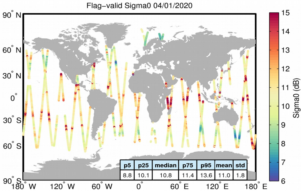
Figure 23. Geographical distribution of flag-valid sigma0 data over oceans and lakes for 04/01/2020. The statistical values shown in the table refer to the sigma0 in dB and are calculated over all measurements shown in the figure.
