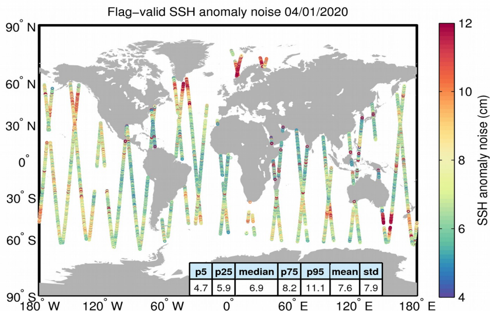
Figure 8. Geographical distribution of flag-valid 20-Hz SSH anomaly measurement noise over oceans and lakes for 04/01/2020. The statistical values shown in the table refer to the SSH anomaly noise and are calculated over all measurements shown in the figure.
