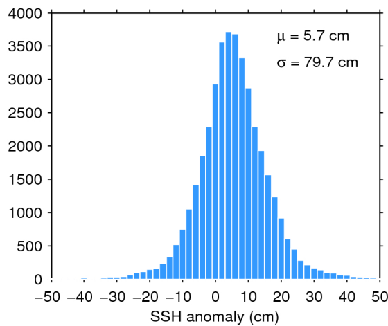
Figure 7. Histogram of flag-valid SSH anomaly over oceans and lakes for 04/01/2020. The mean ( \mu ) and standard deviation ( \sigma ) are also shown. Note that values outside [-50 50] cm are excluded from the histogram for the sake of readability but not from the computation of \mu and \sigma .
