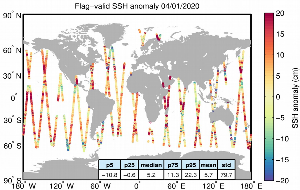
Figure 5. Geographical distribution of flag-valid 1-Hz SSH anomaly data over oceans and lakes for 04/01/2020. The statistical values shown in the table refer to the SSH anomaly in cm and are calculated over all measurements shown in the figure.
