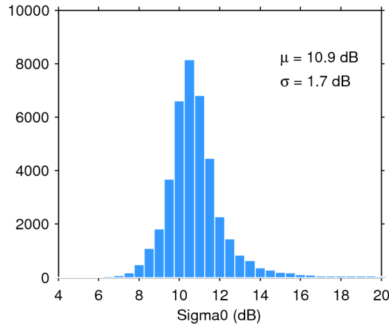
Figure 25. Histogram of flag-valid sigma0 over oceans and lakes for 03/01/2020. The mean ( \mu ) and standard deviation ( \sigma ) are also shown. Note that values outside [4 20] dB are excluded from the histogram for the sake of readability but not from the computation of \mu and \sigma .
