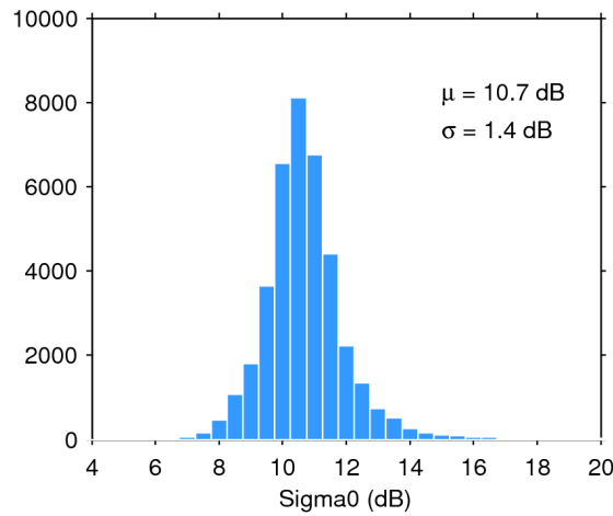
Figure 28. Histogram of science-valid sigma0 over oceans and lakes for 03/01/2020. The mean ( \mu ) and standard deviation ( \sigma ) are also shown. Note that values outside [4 20] dB are excluded from the histogram for the sake of readability but not from the computation of \mu and \sigma .
