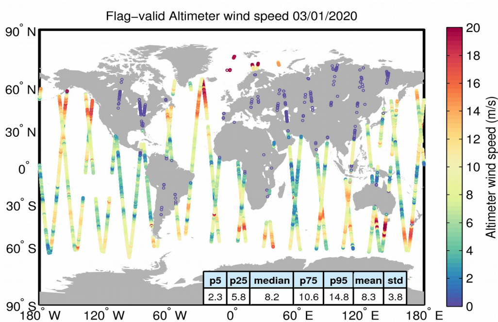
Figure 31. Geographical distribution of flag-valid wind data over oceans and lakes for 03/01/2020. The statistical values shown in the table refer to the wind in m/s and are calculated over all measurements shown in the figure.
