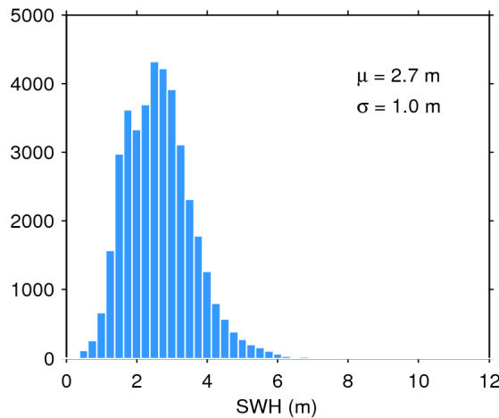
Figure 20. Histogram of science-valid SWH over oceans and lakes for 03/01/2020. The mean ( \mu ) and standard deviation ( \sigma ) are also shown. Note that values larger than 12 m are excluded from the histogram for the sake of readability but not from the computation of \mu and \sigma .
