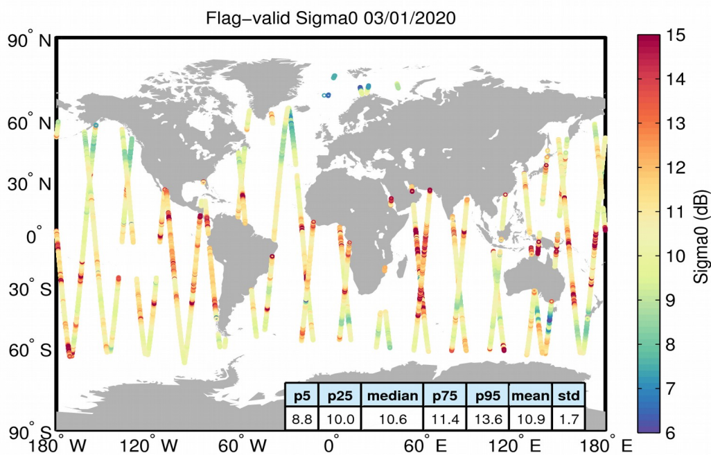
Figure 23. Geographical distribution of flag-valid sigma0 data over oceans and lakes for 03/01/2020. The statistical values shown in the table refer to the sigma0 in dB and are calculated over all measurements shown in the figure.
