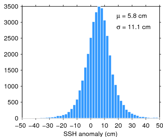
Figure 11. Histogram of science-valid SSH anomaly over oceans and lakes for 03/01/2020. The mean ( \mu ) and standard deviation ( \sigma ) are also shown. Note that values outside [-50 50] cm are excluded from the histogram for the sake of readability but not from the computation of \mu and \sigma .
