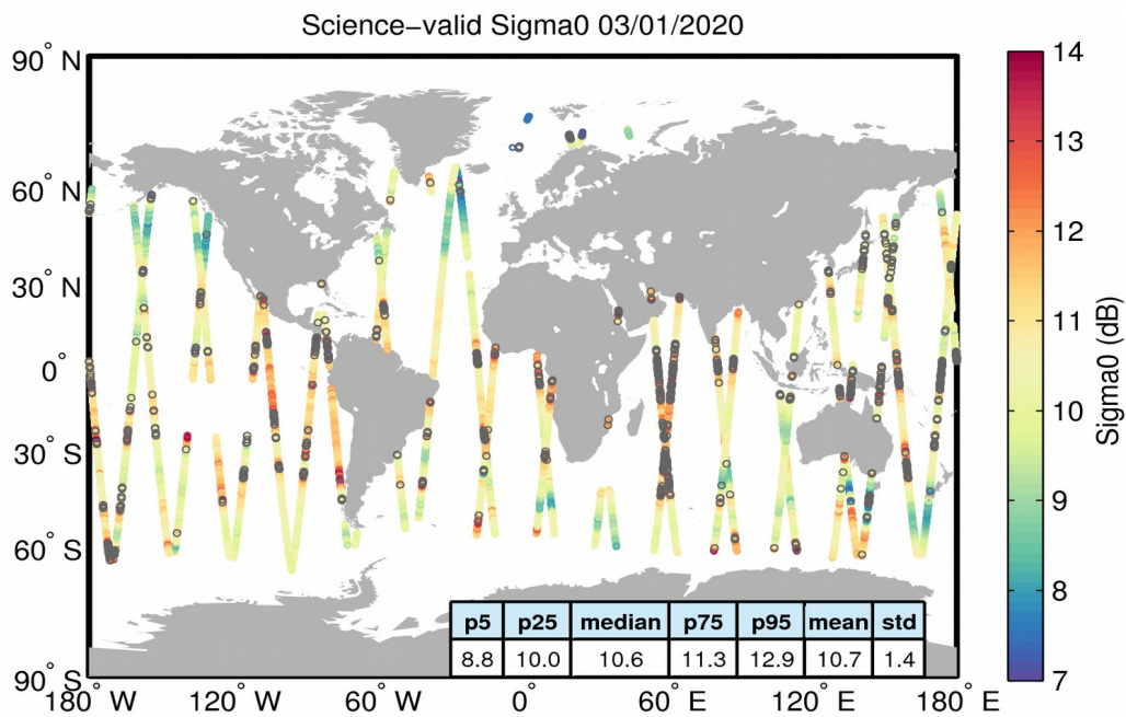
Figure 27. Geographical distribution of science-valid sigma0 data over oceans and lakes for 03/01/2020. The statistical values shown in the table refer to the sigma0 in dB and are calculated over all measurements shown in the figure. Gray circles denote records that have been rejected based on the editing criteria described in Table 4.
