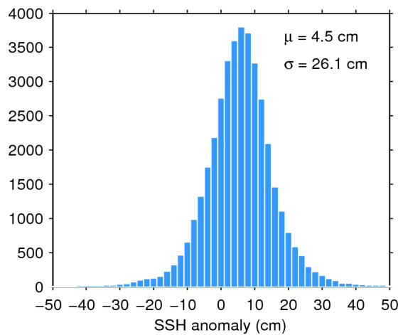
Figure 7. Histogram of flag-valid SSH anomaly over oceans and lakes for 03/01/2020. The mean ( \mu ) and standard deviation ( \sigma ) are also shown. Note that values outside [-50\ 50] cm are excluded from the histogram for the sake of readability but not from the computation of \mu and \sigma .
