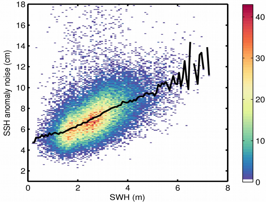
Figure 9. 2D histogram showing flag-valid SSH anomaly noise as a function of SWH for 03/01/2020. The black line denotes the median SSH anomaly noise as a function of SWH.
