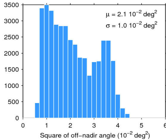
Figure 39. Histogram of flag-valid mispointing over oceans and lakes for 03/01/2020. The mean ( \mu ) and standard deviation ( \sigma ) are also shown. Note that values larger than 6 \cdot 10^{-2} \text{ deg}^2 are excluded from the histogram for the sake of readability but not from the computation of \mu and \sigma .
