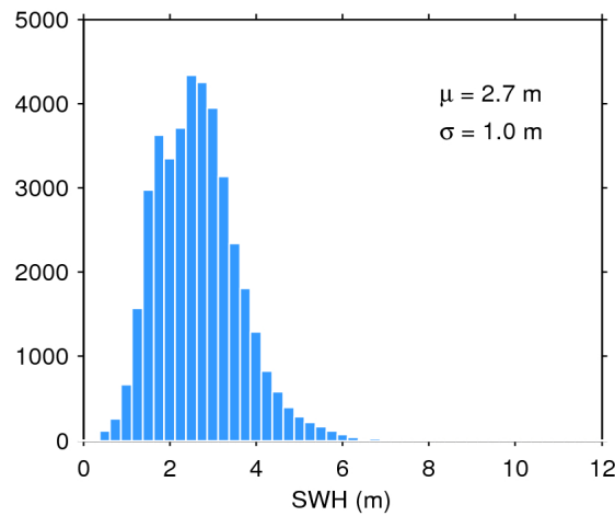
Figure 17. Histogram of flag-valid SWH over oceans and lakes for 03/01/2020. The mean ( \mu ) and standard deviation ( \sigma ) are also shown. Note that values larger than 12 m are excluded from the histogram for the sake of readability but not from the computation of \mu and \sigma .
