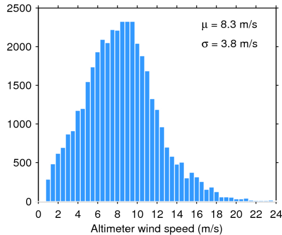
Figure 33. Histogram of flag-valid wind over oceans and lakes for 03/01/2020. The mean ( \mu ) and standard deviation ( \sigma ) are also shown. Note that values larger than 24 m/s are excluded from the histogram for the sake of readability but not from the computation of \mu and \sigma .
