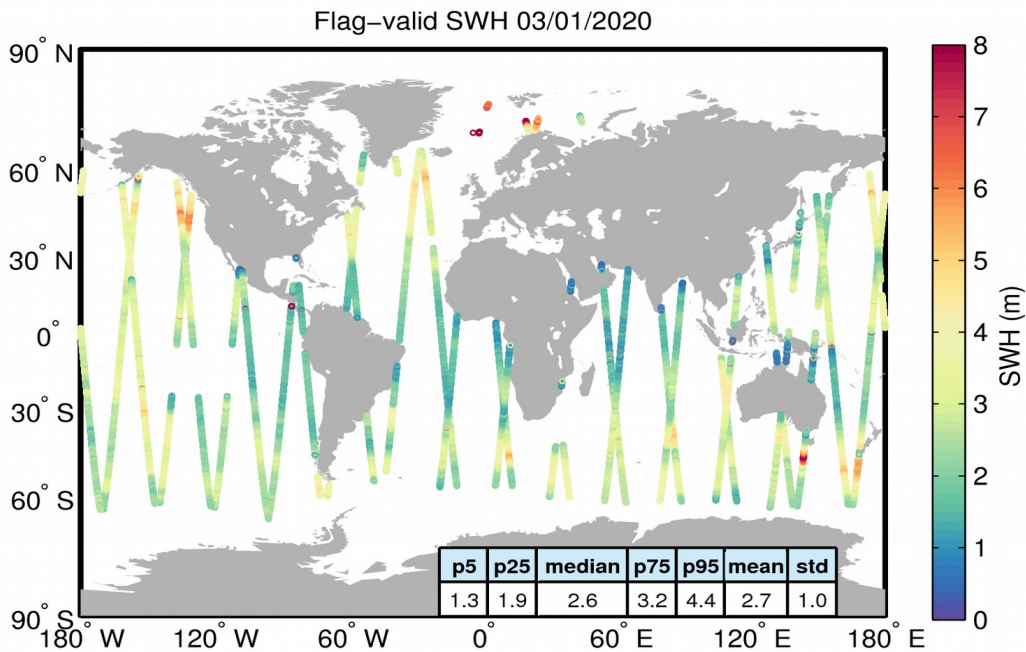
Figure 15. Geographical distribution of flag-valid SWH data over oceans and lakes for 03/01/2020. The statistical values shown in the table refer to the SWH in m and are calculated over all measurements shown in the figure.
