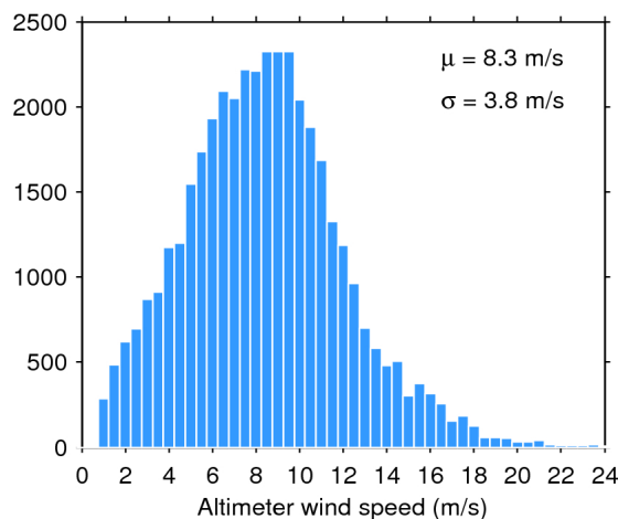
Figure 35. Histogram of science-valid wind over oceans and lakes for 03/01/2020. The mean ( \mu ) and standard deviation ( \sigma ) are also shown. Note that values larger than 24 m/s are excluded from the histogram for the sake of readability but not from the computation of \mu and \sigma .
