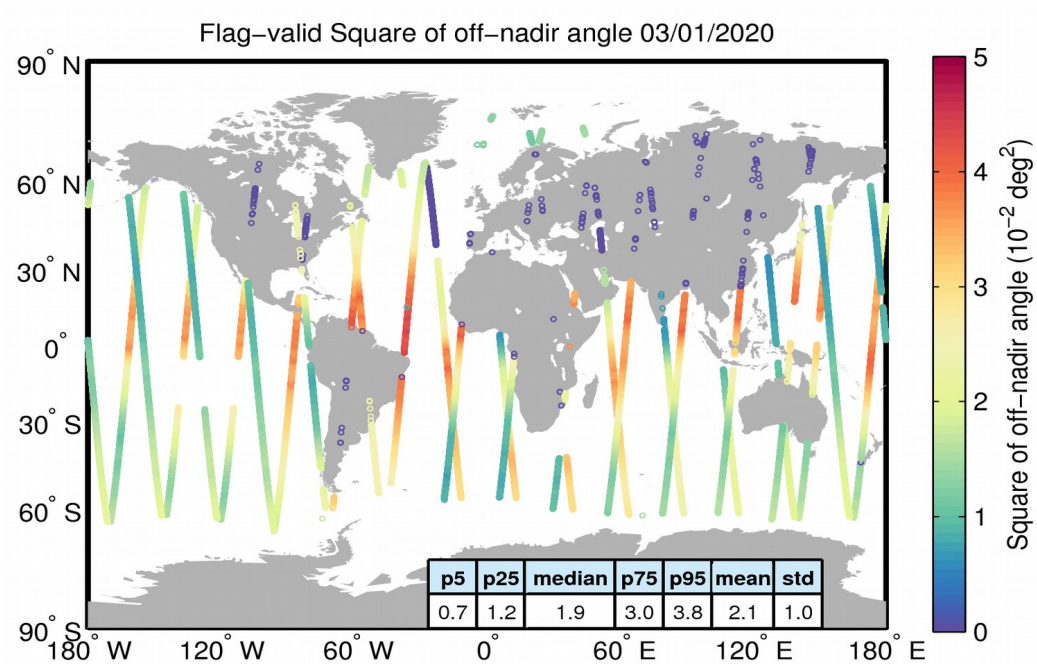
Figure 37. Geographical distribution of flag-valid mispointing data over oceans and lakes for 03/01/2020. The statistical values shown in the table refer to the mispointing in 10^{-2} deg 2 and are calculated over all measurements shown in the figure.
