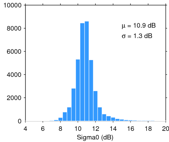
Figure 28. Histogram of science-valid sigma0 over oceans and lakes for 02/01/2020. The mean ( \mu ) and standard deviation ( \sigma ) are also shown. Note that values outside [4 20] dB are excluded from the histogram for the sake of readability but not from the computation of \mu and \sigma .
