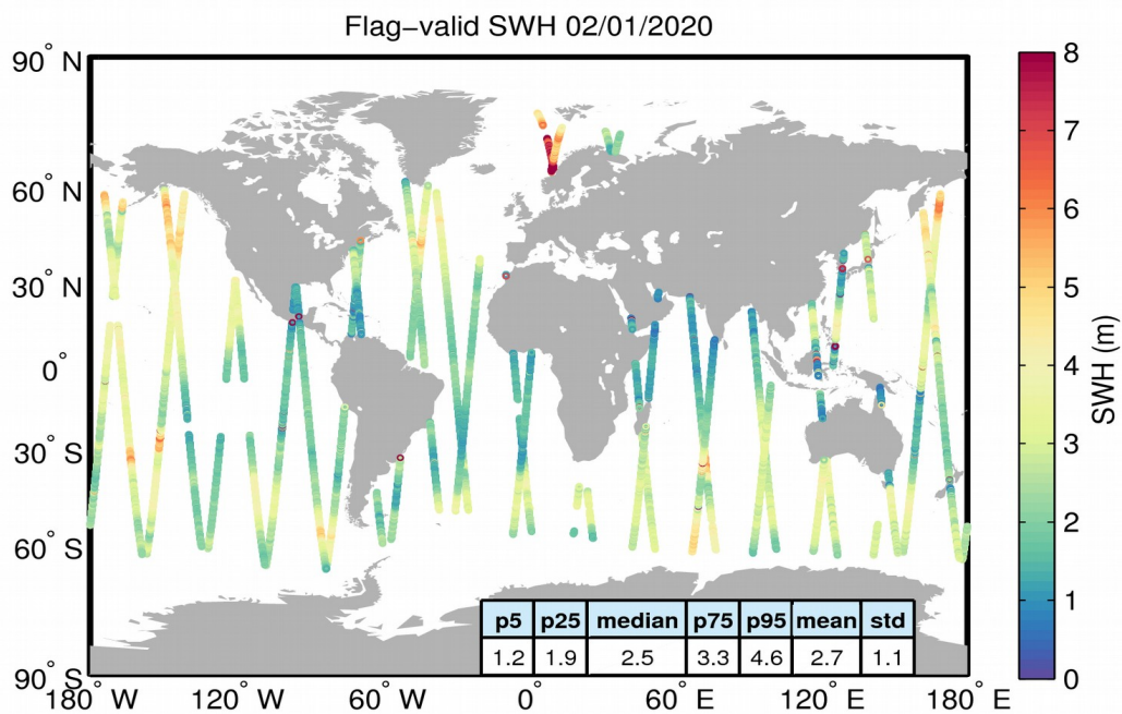
Figure 15. Geographical distribution of flag-valid SWH data over oceans and lakes for 02/01/2020. The statistical values shown in the table refer to the SWH in m and are calculated over all measurements shown in the figure.
