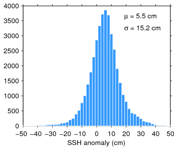
Figure 7. Histogram of flag-valid SSH anomaly over oceans and lakes for 02/01/2020. The mean ( \mu ) and standard deviation ( \sigma ) are also shown. Note that values outside [-50 50] cm are excluded from the histogram for the sake of readability but not from the computation of \mu and \sigma .
