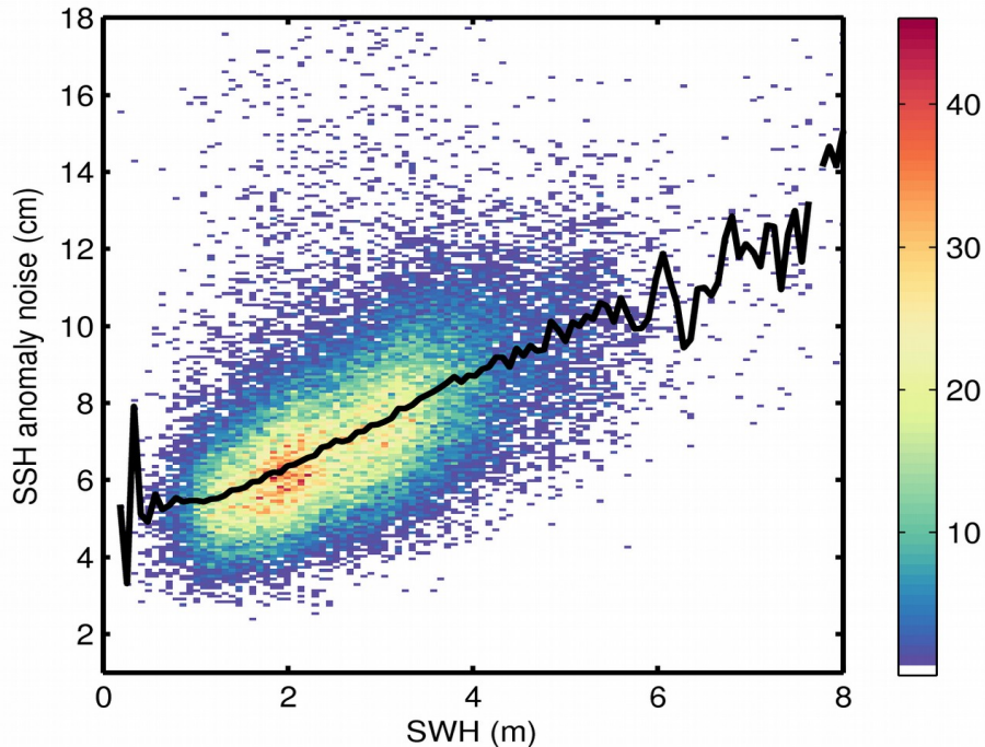
Figure 9. 2D histogram showing flag-valid SSH anomaly noise as a function of SWH for 02/01/2020. The black line denotes the median SSH anomaly noise as a function of SWH.
