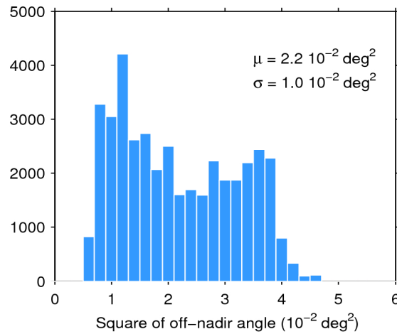
Figure 39. Histogram of flag-valid mispointing over oceans and lakes for 02/01/2020. The mean ( \mu ) and standard deviation ( \sigma ) are also shown. Note that values larger than 6 \cdot 10^{-2} \text{ deg}^2 are excluded from the histogram for the sake of readability but not from the computation of \mu and \sigma .
