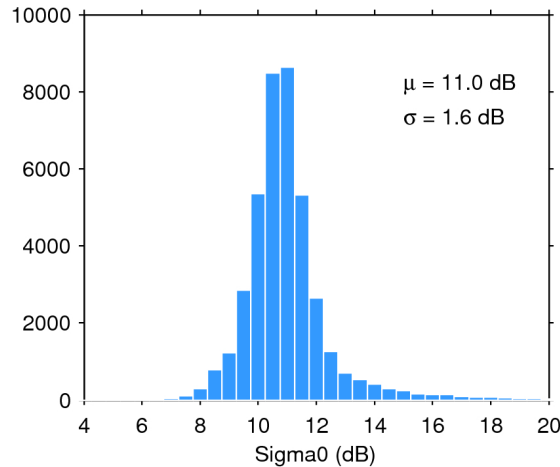
Figure 25. Histogram of flag-valid sigma0 over oceans and lakes for 02/01/2020. The mean ( \mu ) and standard deviation ( \sigma ) are also shown. Note that values outside [4 20] dB are excluded from the histogram for the sake of readability but not from the computation of \mu and \sigma .
