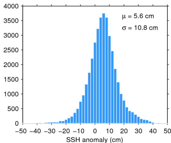
Figure 11. Histogram of science-valid SSH anomaly over oceans and lakes for 02/01/2020. The mean ( \mu ) and standard deviation ( \sigma ) are also shown. Note that values outside [-50 50] cm are excluded from the histogram for the sake of readability but not from the computation of \mu and \sigma .
