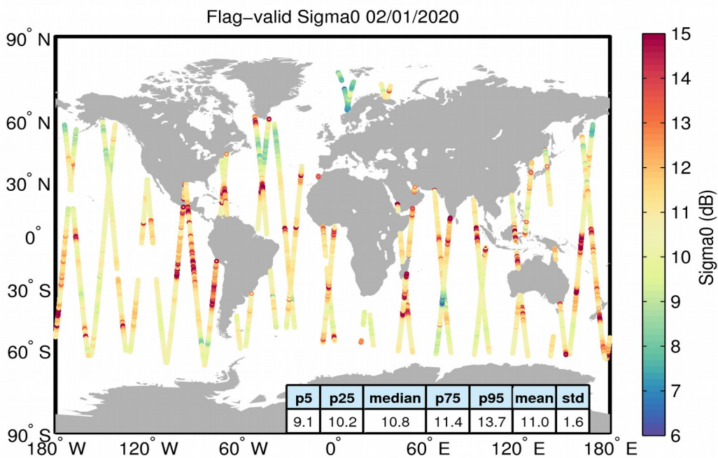
Figure 23. Geographical distribution of flag-valid sigma0 data over oceans and lakes for 02/01/2020. The statistical values shown in the table refer to the sigma0 in dB and are calculated over all measurements shown in the figure.
