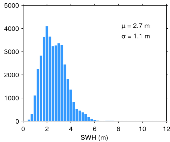
Figure 17. Histogram of flag-valid SWH over oceans and lakes for 02/01/2020. The mean ( \mu ) and standard deviation ( \sigma ) are also shown. Note that values larger than 12 m are excluded from the histogram for the sake of readability but not from the computation of \mu and \sigma .
