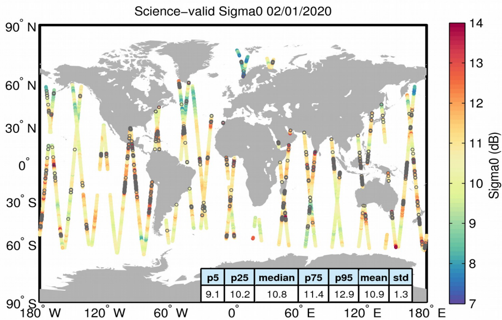
Figure 27. Geographical distribution of science-valid sigma0 data over oceans and lakes for 02/01/2020. The statistical values shown in the table refer to the sigma0 in dB and are calculated over all measurements shown in the figure. Gray circles denote records that have been rejected based on the editing criteria described in Table 4.
