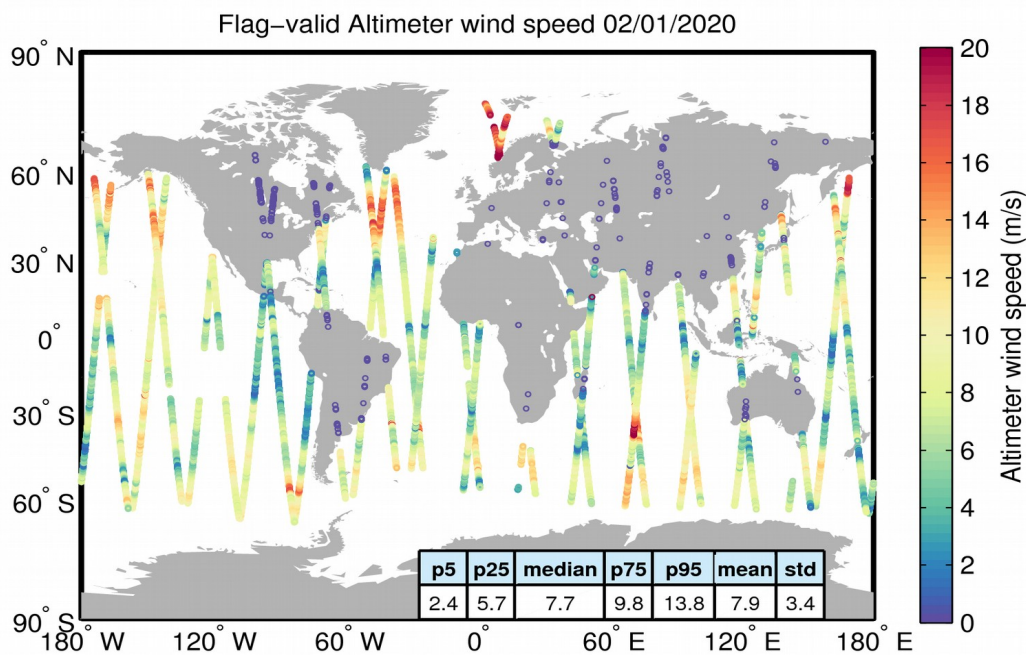
Figure 31. Geographical distribution of flag-valid wind data over oceans and lakes for 02/01/2020. The statistical values shown in the table refer to the wind in m/s and are calculated over all measurements shown in the figure.
