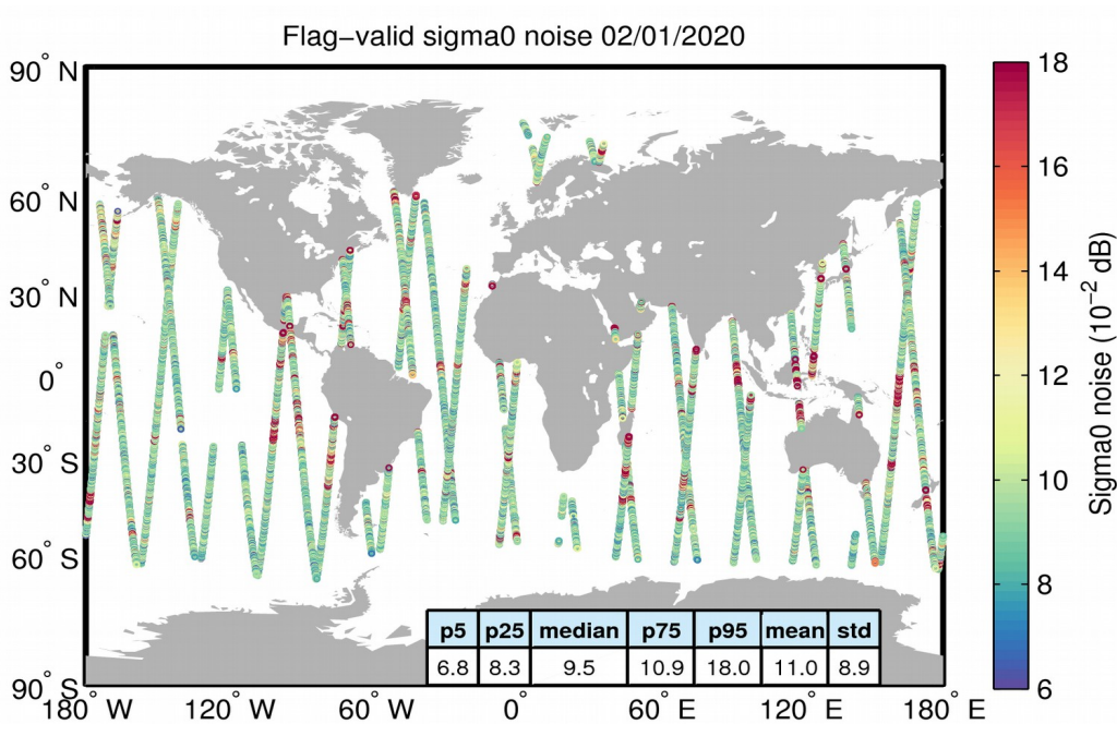
Figure 26. Geographical distribution of flag-valid 20-Hz sigma0 measurement noise over oceans and lakes for 02/01/2020. The statistical values shown in the table refer to the sigma0 noise and are calculated over all measurements shown in the figure.
