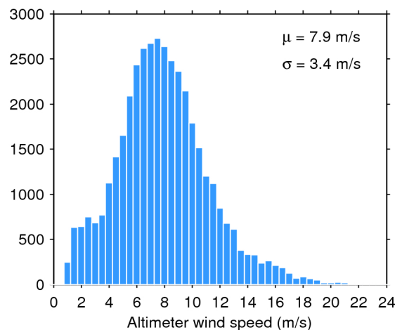
Figure 35. Histogram of science-valid wind over oceans and lakes for 02/01/2020. The mean ( \mu ) and standard deviation ( \sigma ) are also shown. Note that values larger than 24 m/s are excluded from the histogram for the sake of readability but not from the computation of \mu and \sigma .
