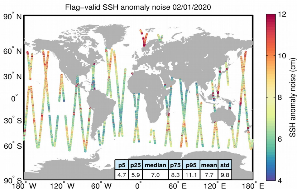
Figure 8. Geographical distribution of flag-valid 20-Hz SSH anomaly measurement noise over oceans and lakes for 02/01/2020. The statistical values shown in the table refer to the SSH anomaly noise and are calculated over all measurements shown in the figure.
