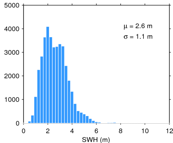
Figure 20. Histogram of science-valid SWH over oceans and lakes for 02/01/2020. The mean ( \mu ) and standard deviation ( \sigma ) are also shown. Note that values larger than 12 m are excluded from the histogram for the sake of readability but not from the computation of \mu and \sigma .
