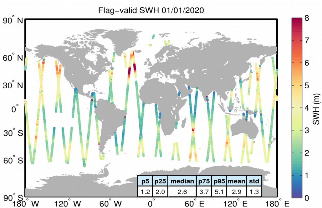
Figure 15. Geographical distribution of flag-valid SWH data over oceans and lakes for 01/01/2020. The statistical values shown in the table refer to the SWH in m and are calculated over all measurements shown in the figure.
