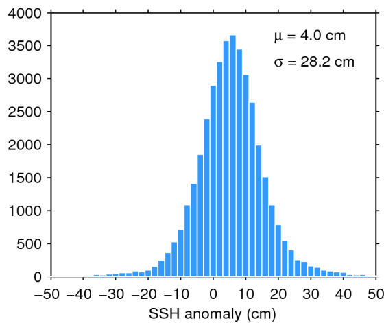
Figure 7. Histogram of flag-valid SSH anomaly over oceans and lakes for 01/01/2020. The mean ( \mu ) and standard deviation ( \sigma ) are also shown. Note that values outside [-50\ 50] cm are excluded from the histogram for the sake of readability but not from the computation of \mu and \sigma .
