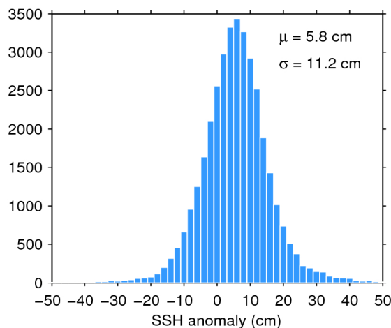
Figure 11. Histogram of science-valid SSH anomaly over oceans and lakes for 01/01/2020. The mean ( \mu ) and standard deviation ( \sigma ) are also shown. Note that values outside [-50 50] cm are excluded from the histogram for the sake of readability but not from the computation of \mu and \sigma .
