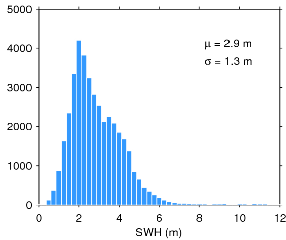
Figure 17. Histogram of flag-valid SWH over oceans and lakes for 01/01/2020. The mean ( \mu ) and standard deviation ( \sigma ) are also shown. Note that values larger than 12 m are excluded from the histogram for the sake of readability but not from the computation of \mu and \sigma .
