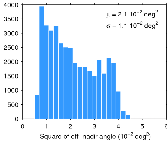
Figure 39. Histogram of flag-valid mispointing over oceans and lakes for 01/01/2020. The mean ( \mu ) and standard deviation ( \sigma ) are also shown. Note that values larger than 6 \cdot 10^{-2} \text{ deg}^2 are excluded from the histogram for the sake of readability but not from the computation of \mu and \sigma .
