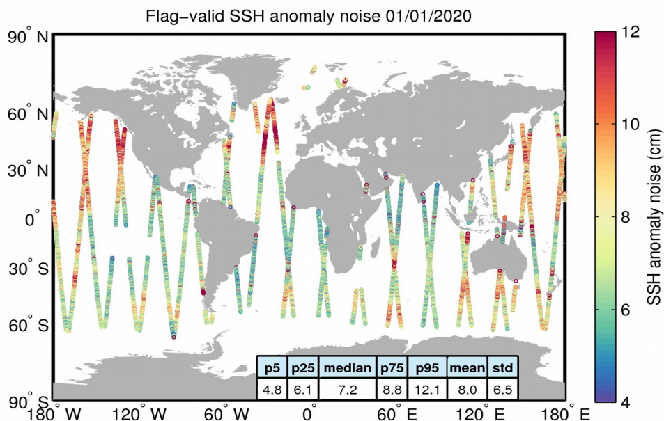
Figure 8. Geographical distribution of flag-valid 20-Hz SSH anomaly measurement noise over oceans and lakes for 01/01/2020. The statistical values shown in the table refer to the SSH anomaly noise and are calculated over all measurements shown in the figure.
