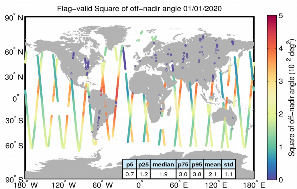
Figure 37. Geographical distribution of flag-valid mispointing data over oceans and lakes for 01/01/2020. The statistical values shown in the table refer to the mispointing in 10^{-2} deg 2 and are calculated over all measurements shown in the figure.
