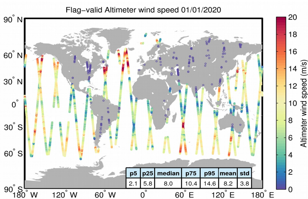
Figure 31. Geographical distribution of flag-valid wind data over oceans and lakes for 01/01/2020. The statistical values shown in the table refer to the wind in m/s and are calculated over all measurements shown in the figure.
