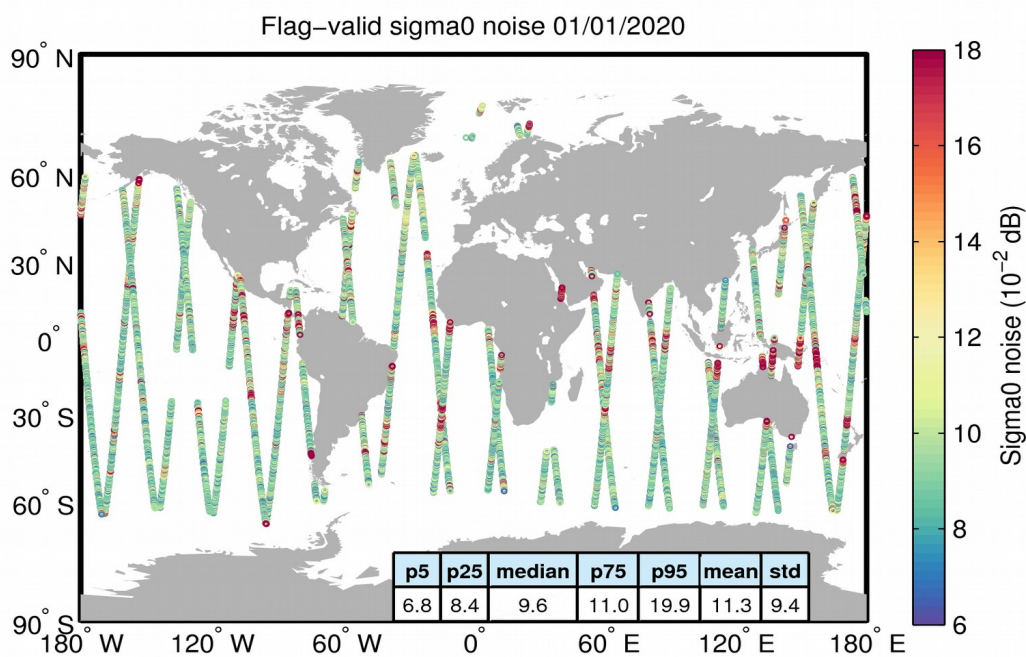
Figure 26. Geographical distribution of flag-valid 20-Hz sigma0 measurement noise over oceans and lakes for 01/01/2020. The statistical values shown in the table refer to the sigma0 noise and are calculated over all measurements shown in the figure.
