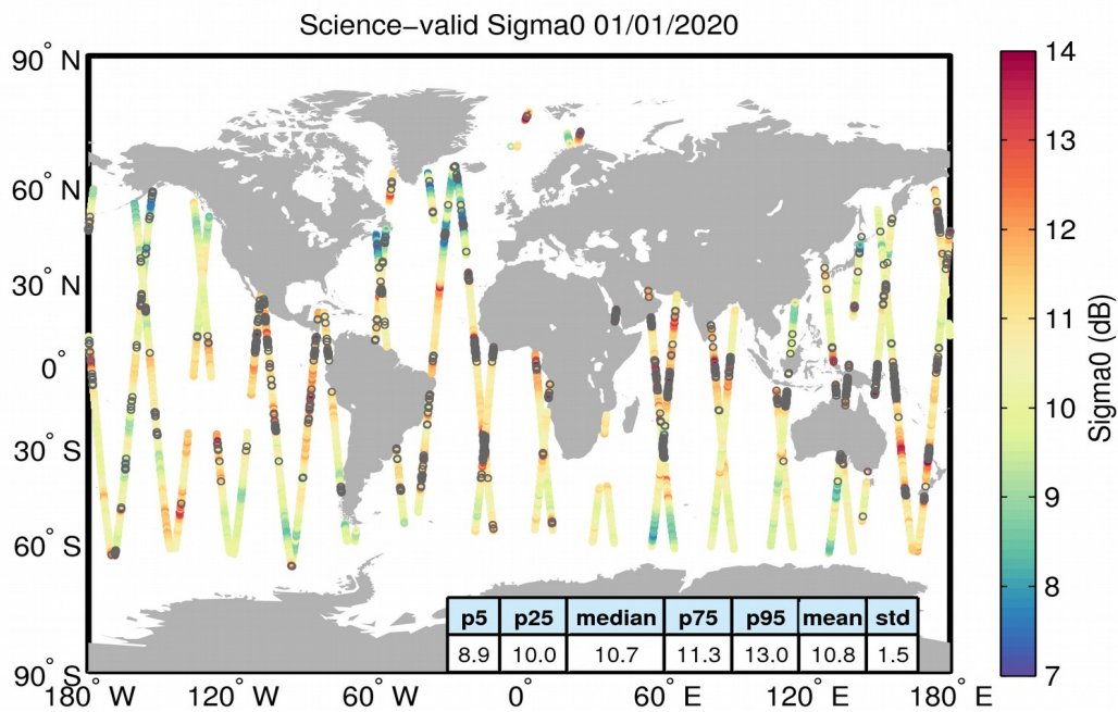
Figure 27. Geographical distribution of science-valid sigma0 data over oceans and lakes for 01/01/2020. The statistical values shown in the table refer to the sigma0 in dB and are calculated over all measurements shown in the figure. Gray circles denote records that have been rejected based on the editing criteria described in Table 4.
