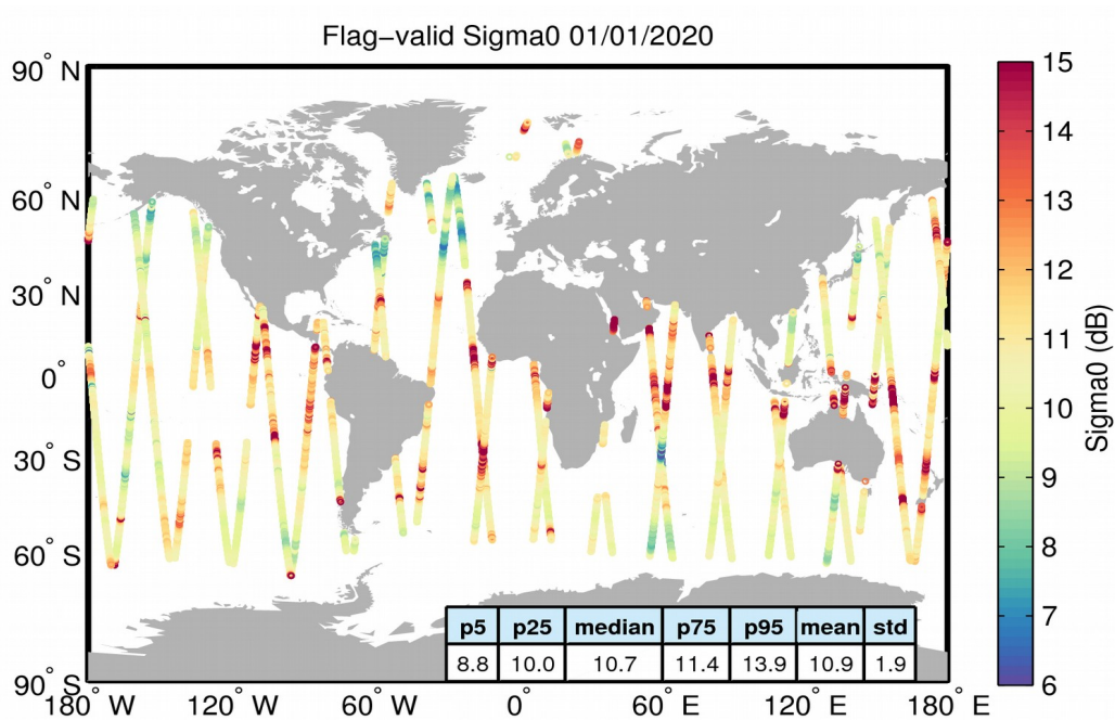
Figure 23. Geographical distribution of flag-valid sigma0 data over oceans and lakes for 01/01/2020. The statistical values shown in the table refer to the sigma0 in dB and are calculated over all measurements shown in the figure.
