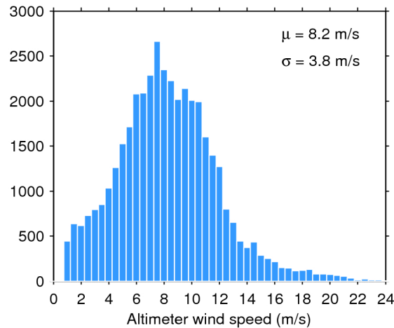
Figure 33. Histogram of flag-valid wind over oceans and lakes for 01/01/2020. The mean ( \mu ) and standard deviation ( \sigma ) are also shown. Note that values larger than 24 m/s are excluded from the histogram for the sake of readability but not from the computation of \mu and \sigma .
