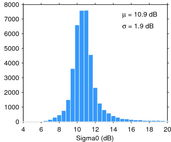
Figure 25. Histogram of flag-valid sigma0 over oceans and lakes for 01/01/2020. The mean ( \mu ) and standard deviation ( \sigma ) are also shown. Note that values outside [4 20] dB are excluded from the histogram for the sake of readability but not from the computation of \mu and \sigma .
