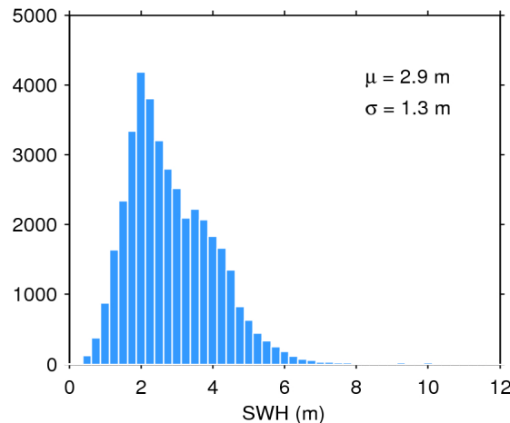
Figure 20. Histogram of science-valid SWH over oceans and lakes for 01/01/2020. The mean ( \mu ) and standard deviation ( \sigma ) are also shown. Note that values larger than 12 m are excluded from the histogram for the sake of readability but not from the computation of \mu and \sigma .
