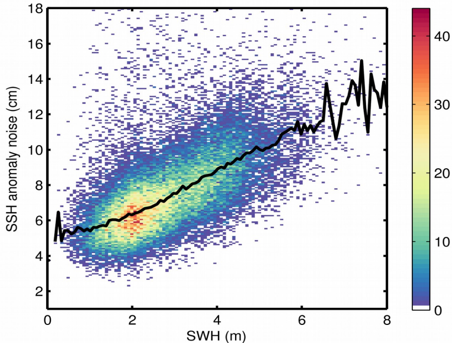
Figure 9. 2D histogram showing flag-valid SSH anomaly noise as a function of SWH for 01/01/2020. The black line denotes the median SSH anomaly noise as a function of SWH.
