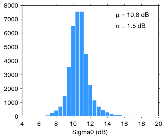
Figure 28. Histogram of science-valid sigma0 over oceans and lakes for 01/01/2020. The mean ( \mu ) and standard deviation ( \sigma ) are also shown. Note that values outside [4 20] dB are excluded from the histogram for the sake of readability but not from the computation of \mu and \sigma .
