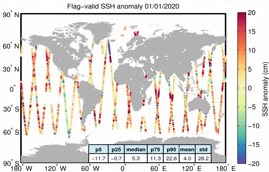
Figure 5. Geographical distribution of flag-valid 1-Hz SSH anomaly data over oceans and lakes for 01/01/2020. The statistical values shown in the table refer to the SSH anomaly in cm and are calculated over all measurements shown in the figure.
