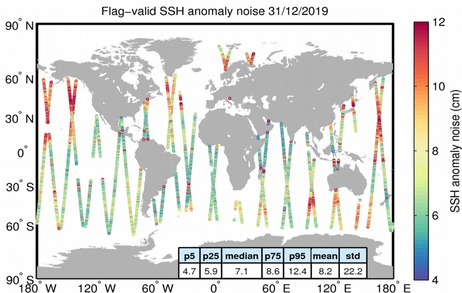
Figure 8. Geographical distribution of flag-valid 20-Hz SSH anomaly measurement noise over oceans and lakes for 31/12/2019. The statistical values shown in the table refer to the SSH anomaly noise and are calculated over all measurements shown in the figure.
