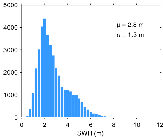
Figure 20. Histogram of science-valid SWH over oceans and lakes for 31/12/2019. The mean ( \mu ) and standard deviation ( \sigma ) are also shown. Note that values larger than 12 m are excluded from the histogram for the sake of readability but not from the computation of \mu and \sigma .
