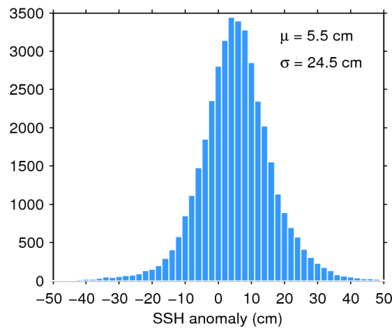
Figure 7. Histogram of flag-valid SSH anomaly over oceans and lakes for 31/12/2019. The mean ( \mu ) and standard deviation ( \sigma ) are also shown. Note that values outside [-50\ 50] cm are excluded from the histogram for the sake of readability but not from the computation of \mu and \sigma .
