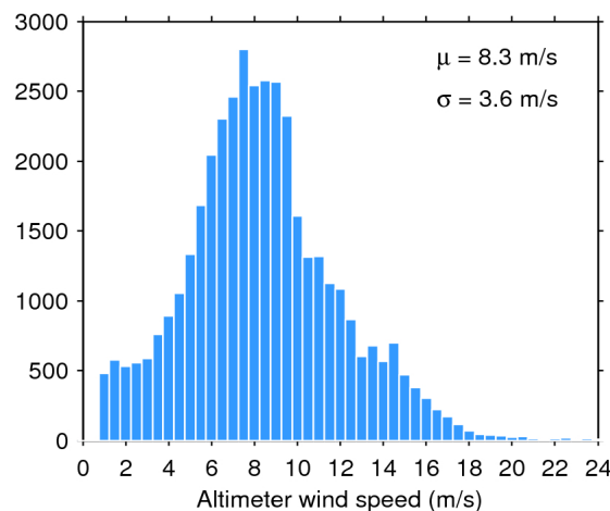
Figure 35. Histogram of science-valid wind over oceans and lakes for 31/12/2019. The mean ( \mu ) and standard deviation ( \sigma ) are also shown. Note that values larger than 24 m/s are excluded from the histogram for the sake of readability but not from the computation of \mu and \sigma .
