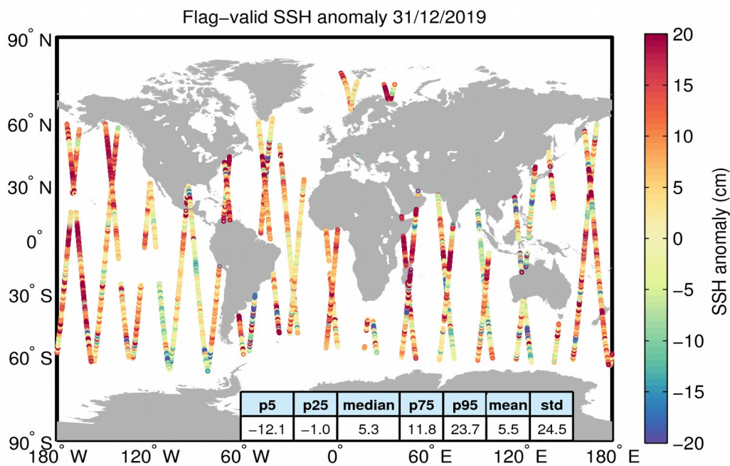
Figure 5. Geographical distribution of flag-valid 1-Hz SSH anomaly data over oceans and lakes for 31/12/2019. The statistical values shown in the table refer to the SSH anomaly in cm and are calculated over all measurements shown in the figure.
