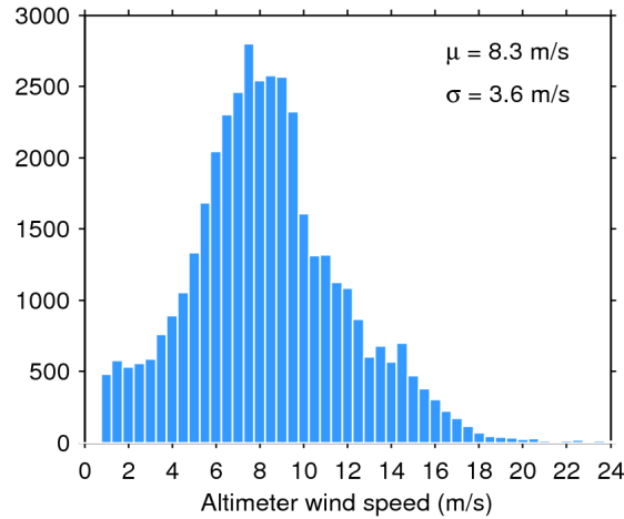
Figure 33. Histogram of flag-valid wind over oceans and lakes for 31/12/2019. The mean ( \mu ) and standard deviation ( \sigma ) are also shown. Note that values larger than 24 m/s are excluded from the histogram for the sake of readability but not from the computation of \mu and \sigma .
