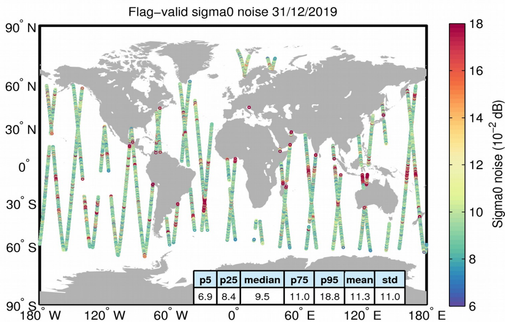
Figure 26. Geographical distribution of flag-valid 20-Hz sigma0 measurement noise over oceans and lakes for 31/12/2019. The statistical values shown in the table refer to the sigma0 noise and are calculated over all measurements shown in the figure.
