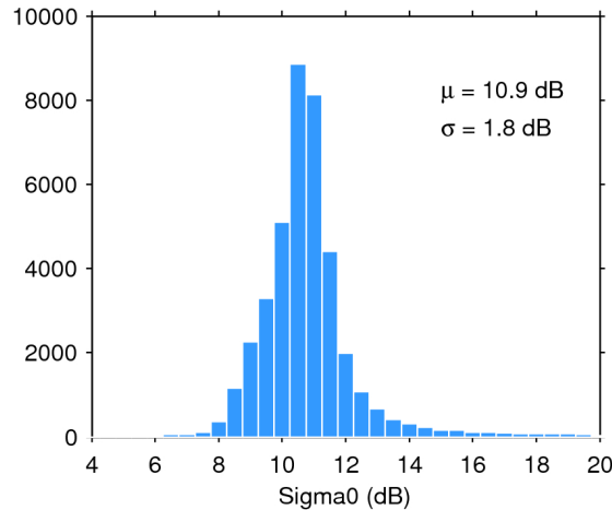
Figure 25. Histogram of flag-valid sigma0 over oceans and lakes for 31/12/2019. The mean ( \mu ) and standard deviation ( \sigma ) are also shown. Note that values outside [4 20] dB are excluded from the histogram for the sake of readability but not from the computation of \mu and \sigma .
