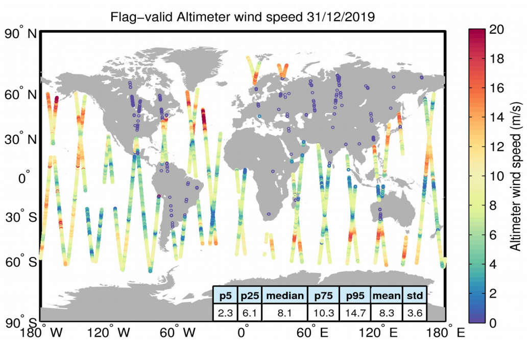
Figure 31. Geographical distribution of flag-valid wind data over oceans and lakes for 31/12/2019. The statistical values shown in the table refer to the wind in m/s and are calculated over all measurements shown in the figure.
