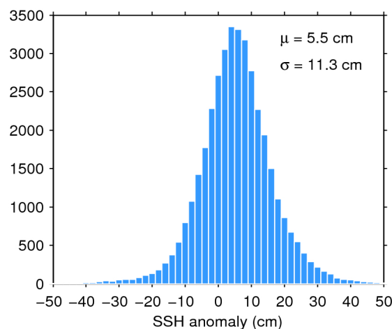
Figure 11. Histogram of science-valid SSH anomaly over oceans and lakes for 31/12/2019. The mean ( \mu ) and standard deviation ( \sigma ) are also shown. Note that values outside [-50 50] cm are excluded from the histogram for the sake of readability but not from the computation of \mu and \sigma .
