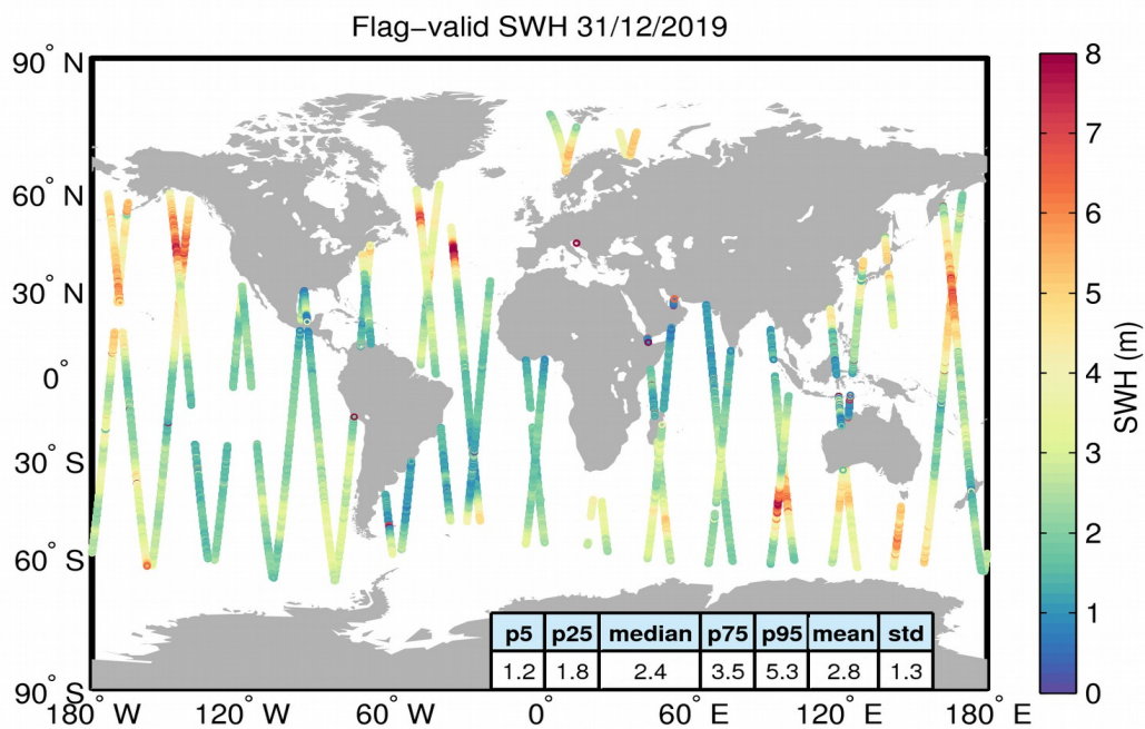
Figure 15. Geographical distribution of flag-valid SWH data over oceans and lakes for 31/12/2019. The statistical values shown in the table refer to the SWH in m and are calculated over all measurements shown in the figure.
