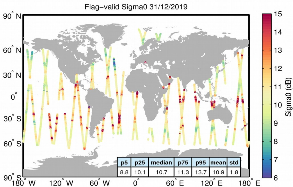
Figure 23. Geographical distribution of flag-valid sigma0 data over oceans and lakes for 31/12/2019. The statistical values shown in the table refer to the sigma0 in dB and are calculated over all measurements shown in the figure.
