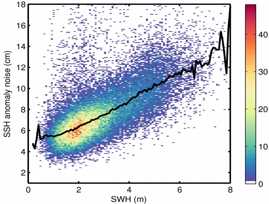
Figure 9. 2D histogram showing flag-valid SSH anomaly noise as a function of SWH for 31/12/2019. The black line denotes the median SSH anomaly noise as a function of SWH.
