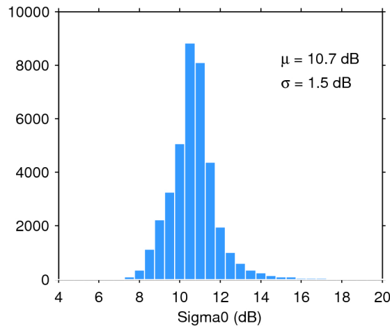
Figure 28. Histogram of science-valid sigma0 over oceans and lakes for 31/12/2019. The mean ( \mu ) and standard deviation ( \sigma ) are also shown. Note that values outside [4 20] dB are excluded from the histogram for the sake of readability but not from the computation of \mu and \sigma .
