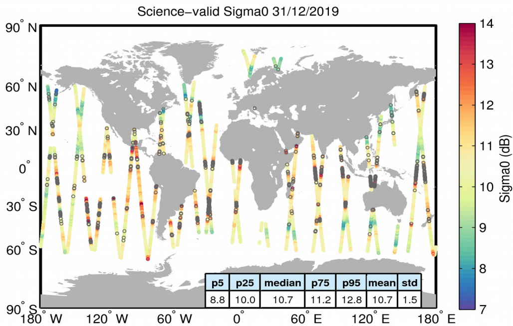
Figure 27. Geographical distribution of science-valid sigma0 data over oceans and lakes for 31/12/2019. The statistical values shown in the table refer to the sigma0 in dB and are calculated over all measurements shown in the figure. Gray circles denote records that have been rejected based on the editing criteria described in Table 4.
