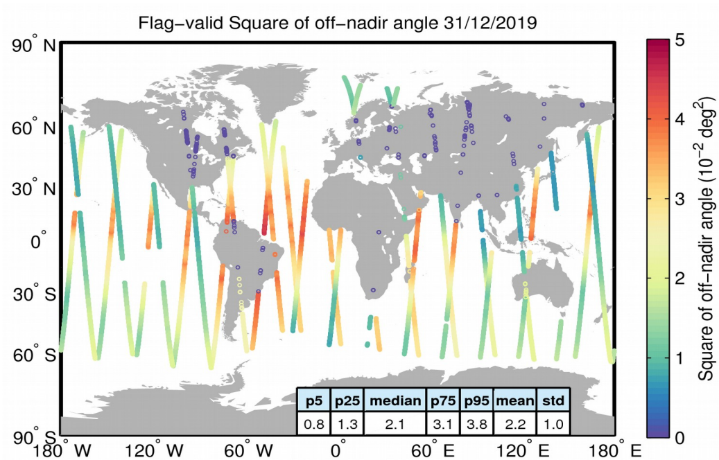
Figure 37. Geographical distribution of flag-valid mispointing data over oceans and lakes for 31/12/2019. The statistical values shown in the table refer to the mispointing in 10^{-2} \text{ deg}^2 and are calculated over all measurements shown in the figure.
