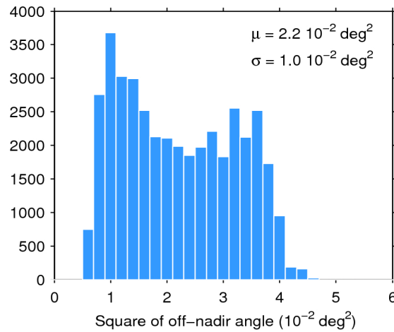
Figure 39. Histogram of flag-valid mispointing over oceans and lakes for 31/12/2019. The mean ( \mu ) and standard deviation ( \sigma ) are also shown. Note that values larger than 6 \cdot 10^{-2} \text{ deg}^2 are excluded from the histogram for the sake of readability but not from the computation of \mu and \sigma .
