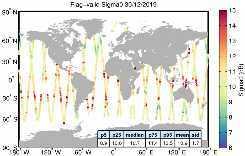
Figure 23. Geographical distribution of flag-valid sigma0 data over oceans and lakes for 30/12/2019. The statistical values shown in the table refer to the sigma0 in dB and are calculated over all measurements shown in the figure.
