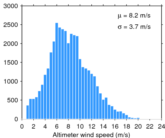
Figure 35. Histogram of science-valid wind over oceans and lakes for 30/12/2019. The mean ( \mu ) and standard deviation ( \sigma ) are also shown. Note that values larger than 24 m/s are excluded from the histogram for the sake of readability but not from the computation of \mu and \sigma .
