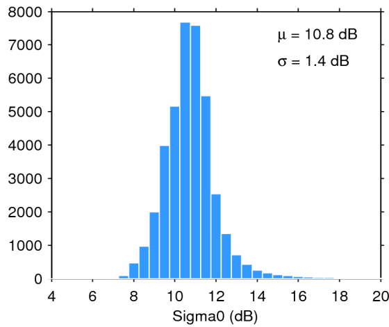
Figure 28. Histogram of science-valid sigma0 over oceans and lakes for 30/12/2019. The mean ( \mu ) and standard deviation ( \sigma ) are also shown. Note that values outside [4 20] dB are excluded from the histogram for the sake of readability but not from the computation of \mu and \sigma .
