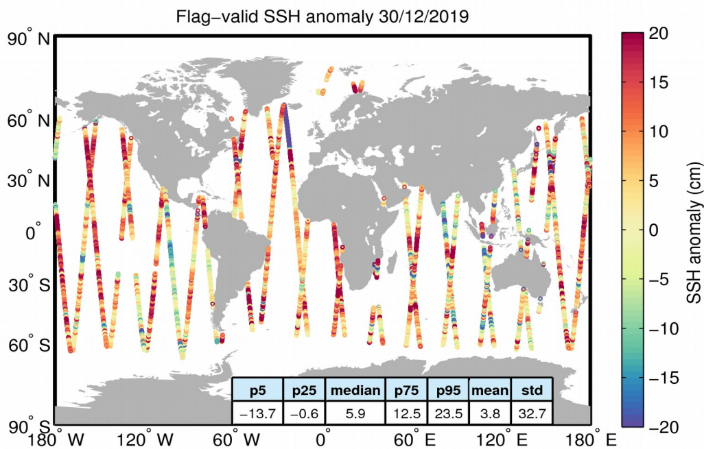
Figure 5. Geographical distribution of flag-valid 1-Hz SSH anomaly data over oceans and lakes for 30/12/2019. The statistical values shown in the table refer to the SSH anomaly in cm and are calculated over all measurements shown in the figure.
