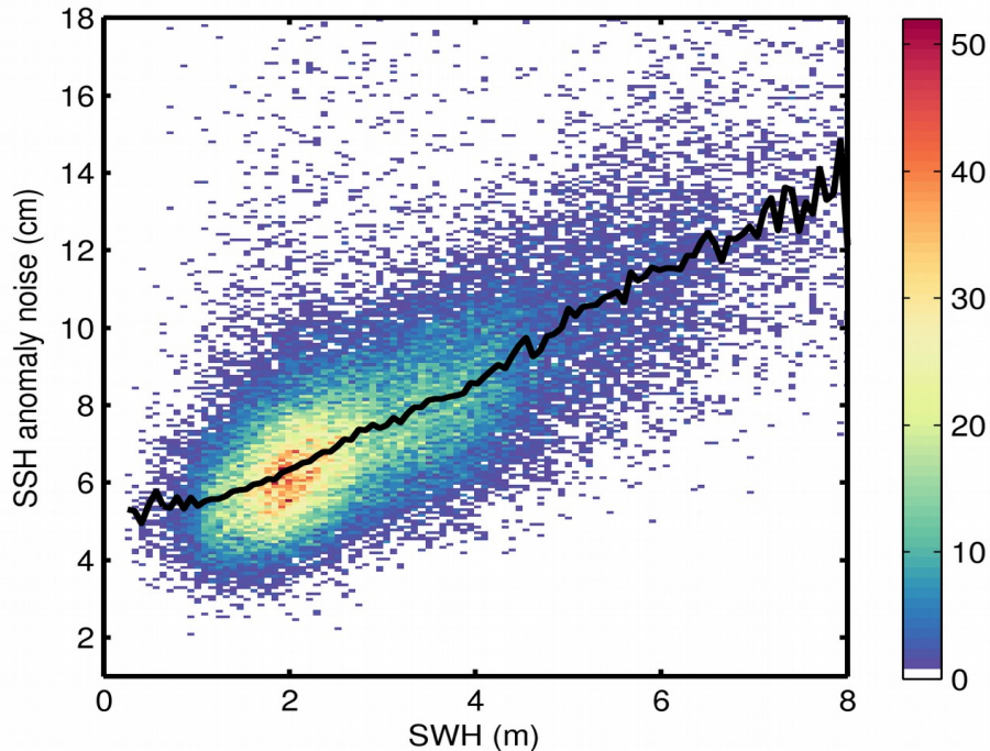
Figure 9. 2D histogram showing flag-valid SSH anomaly noise as a function of SWH for 30/12/2019. The black line denotes the median SSH anomaly noise as a function of SWH.
