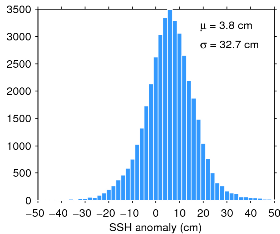
Figure 7. Histogram of flag-valid SSH anomaly over oceans and lakes for 30/12/2019. The mean ( \mu ) and standard deviation ( \sigma ) are also shown. Note that values outside [-50 50] cm are excluded from the histogram for the sake of readability but not from the computation of \mu and \sigma .
