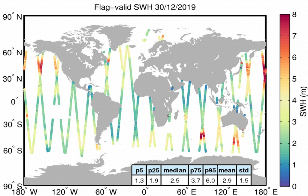
Figure 15. Geographical distribution of flag-valid SWH data over oceans and lakes for 30/12/2019. The statistical values shown in the table refer to the SWH in m and are calculated over all measurements shown in the figure.
