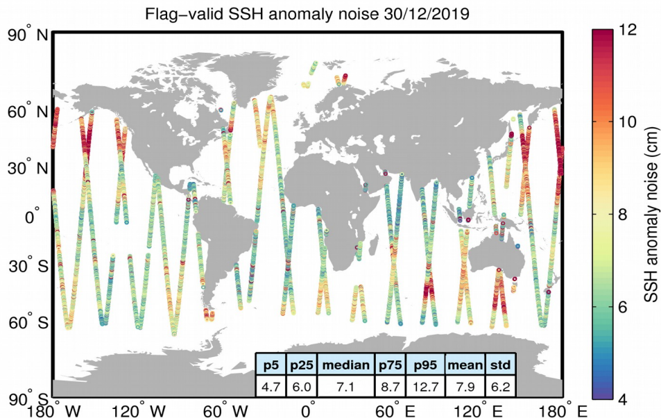
Figure 8. Geographical distribution of flag-valid 20-Hz SSH anomaly measurement noise over oceans and lakes for 30/12/2019. The statistical values shown in the table refer to the SSH anomaly noise and are calculated over all measurements shown in the figure.
