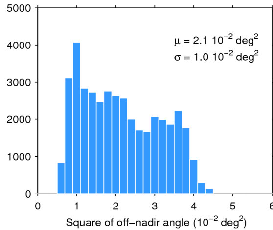
Figure 39. Histogram of flag-valid mispointing over oceans and lakes for 30/12/2019. The mean ( \mu ) and standard deviation ( \sigma ) are also shown. Note that values larger than 6 \cdot 10^{-2} \text{ deg}^2 are excluded from the histogram for the sake of readability but not from the computation of \mu and \sigma .
