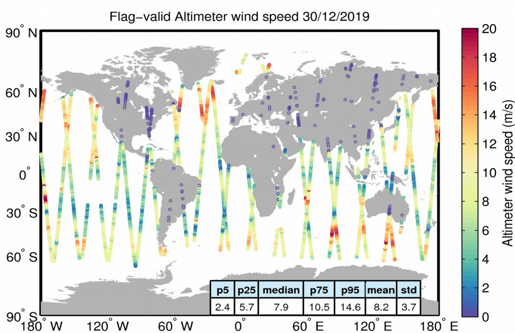
Figure 31. Geographical distribution of flag-valid wind data over oceans and lakes for 30/12/2019. The statistical values shown in the table refer to the wind in m/s and are calculated over all measurements shown in the figure.
