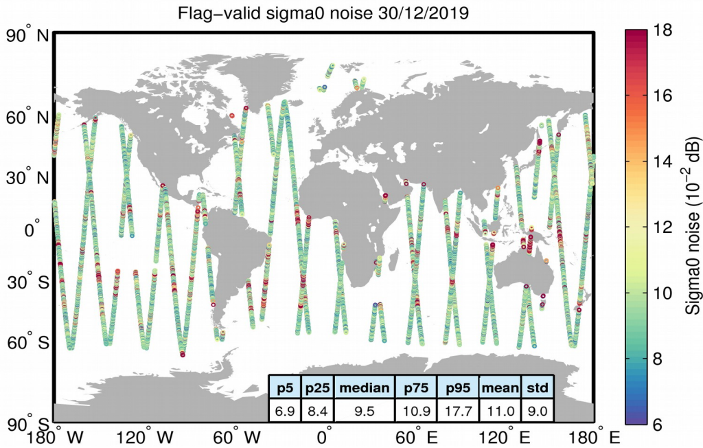
Figure 26. Geographical distribution of flag-valid 20-Hz sigma0 measurement noise over oceans and lakes for 30/12/2019. The statistical values shown in the table refer to the sigma0 noise and are calculated over all measurements shown in the figure.
