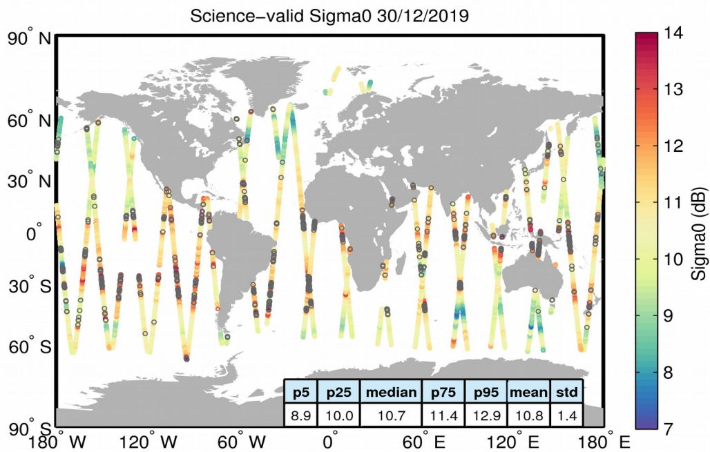
Figure 27. Geographical distribution of science-valid sigma0 data over oceans and lakes for 30/12/2019. The statistical values shown in the table refer to the sigma0 in dB and are calculated over all measurements shown in the figure. Gray circles denote records that have been rejected based on the editing criteria described in Table 4.
