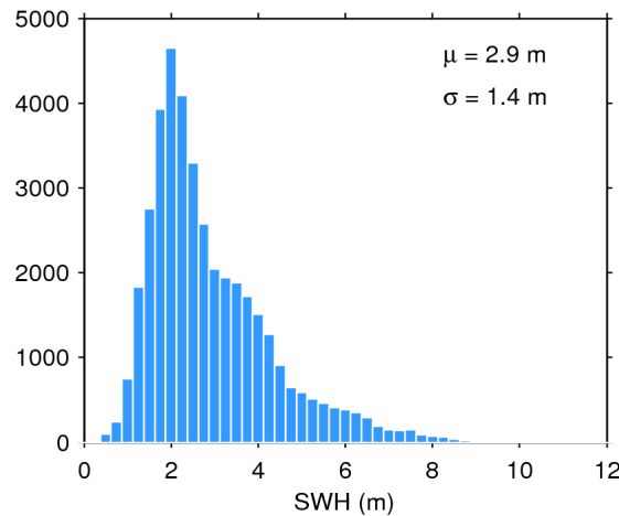
Figure 20. Histogram of science-valid SWH over oceans and lakes for 30/12/2019. The mean ( \mu ) and standard deviation ( \sigma ) are also shown. Note that values larger than 12 m are excluded from the histogram for the sake of readability but not from the computation of \mu and \sigma .
