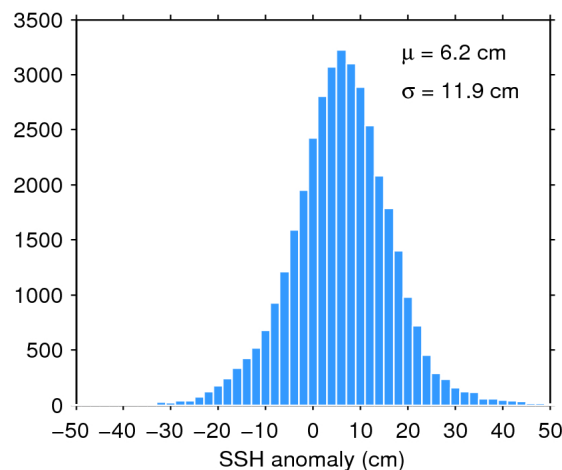
Figure 11. Histogram of science-valid SSH anomaly over oceans and lakes for 30/12/2019. The mean ( \mu ) and standard deviation ( \sigma ) are also shown. Note that values outside [-50 50] cm are excluded from the histogram for the sake of readability but not from the computation of \mu and \sigma .
