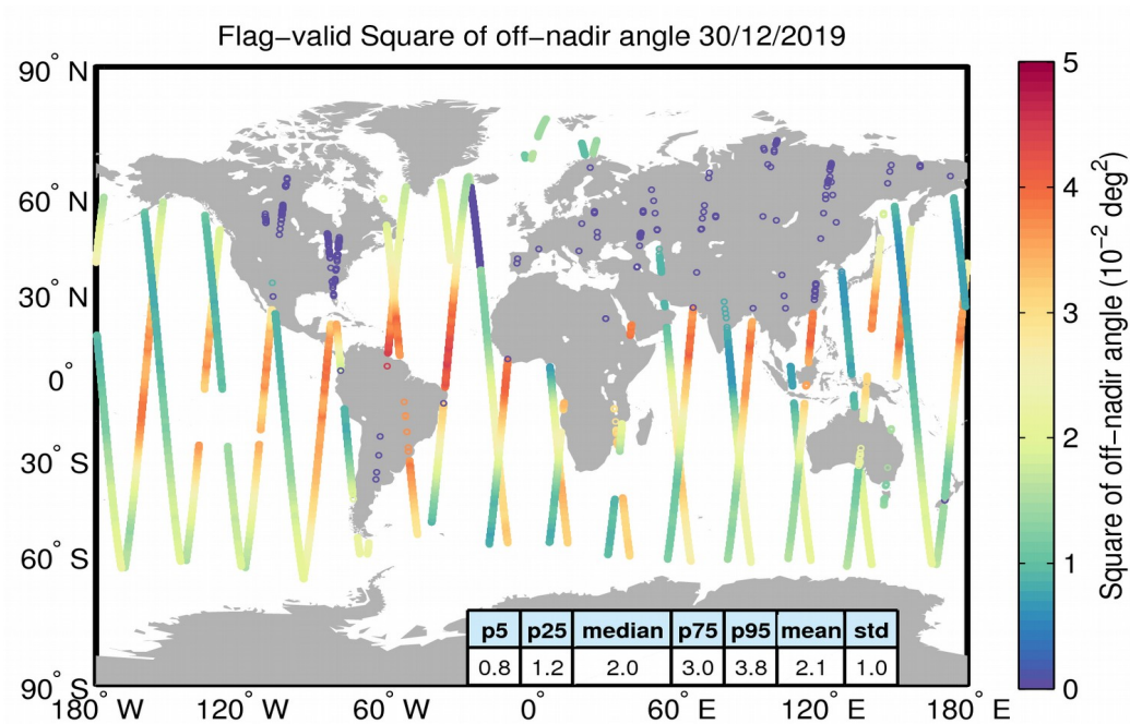
Figure 37. Geographical distribution of flag-valid mispointing data over oceans and lakes for 30/12/2019. The statistical values shown in the table refer to the mispointing in 10^{-2} deg 2 and are calculated over all measurements shown in the figure.
