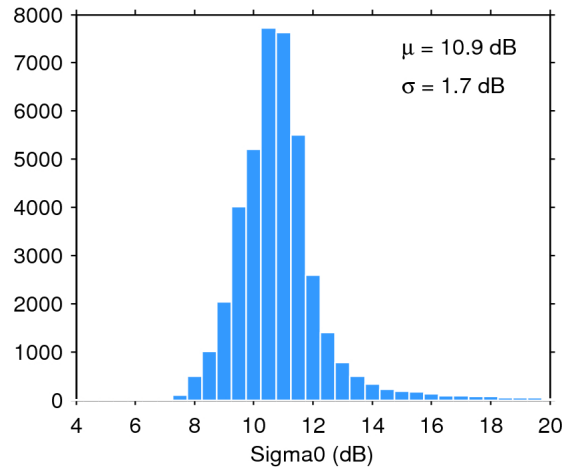
Figure 25. Histogram of flag-valid sigma0 over oceans and lakes for 30/12/2019. The mean ( \mu ) and standard deviation ( \sigma ) are also shown. Note that values outside [4 20] dB are excluded from the histogram for the sake of readability but not from the computation of \mu and \sigma .
