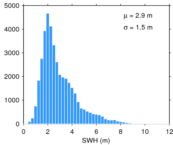
Figure 17. Histogram of flag-valid SWH over oceans and lakes for 30/12/2019. The mean ( \mu ) and standard deviation ( \sigma ) are also shown. Note that values larger than 12 m are excluded from the histogram for the sake of readability but not from the computation of \mu and \sigma .
