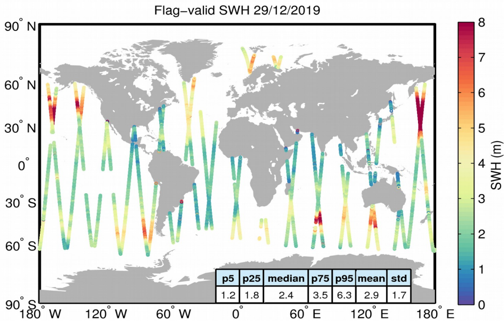
Figure 15. Geographical distribution of flag-valid SWH data over oceans and lakes for 29/12/2019. The statistical values shown in the table refer to the SWH in m and are calculated over all measurements shown in the figure.
