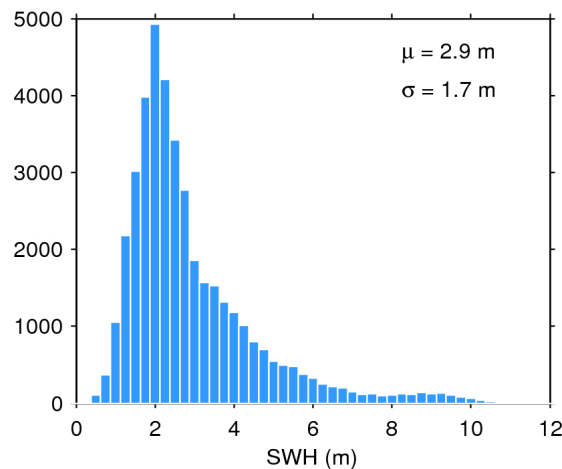
Figure 17. Histogram of flag-valid SWH over oceans and lakes for 29/12/2019. The mean ( \mu ) and standard deviation ( \sigma ) are also shown. Note that values larger than 12 m are excluded from the histogram for the sake of readability but not from the computation of \mu and \sigma .
