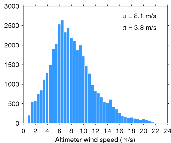
Figure 35. Histogram of science-valid wind over oceans and lakes for 29/12/2019. The mean ( \mu ) and standard deviation ( \sigma ) are also shown. Note that values larger than 24 m/s are excluded from the histogram for the sake of readability but not from the computation of \mu and \sigma .
