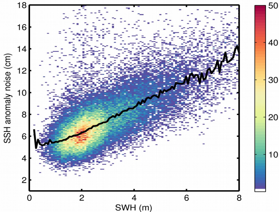
Figure 9. 2D histogram showing flag-valid SSH anomaly noise as a function of SWH for 29/12/2019. The black line denotes the median SSH anomaly noise as a function of SWH.
