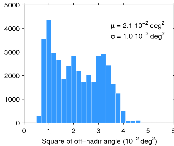
Figure 39. Histogram of flag-valid mispointing over oceans and lakes for 29/12/2019. The mean ( \mu ) and standard deviation ( \sigma ) are also shown. Note that values larger than 6 \cdot 10^{-2} \text{ deg}^2 are excluded from the histogram for the sake of readability but not from the computation of \mu and \sigma .
