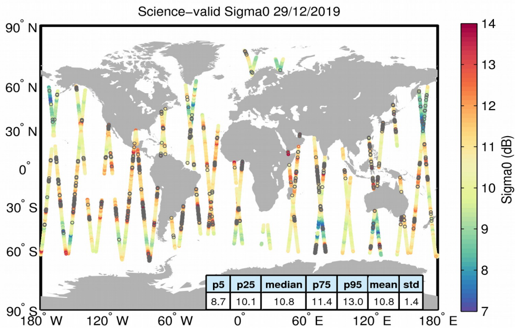
Figure 27. Geographical distribution of science-valid sigma0 data over oceans and lakes for 29/12/2019. The statistical values shown in the table refer to the sigma0 in dB and are calculated over all measurements shown in the figure. Gray circles denote records that have been rejected based on the editing criteria described in Table 4.
