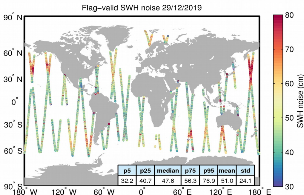
Figure 18. Geographical distribution of flag-valid 20-Hz SWH measurement noise over oceans and lakes for 29/12/2019. The statistical values shown in the figure refer to the SWH noise and are calculated over all measurements shown in the figure.
