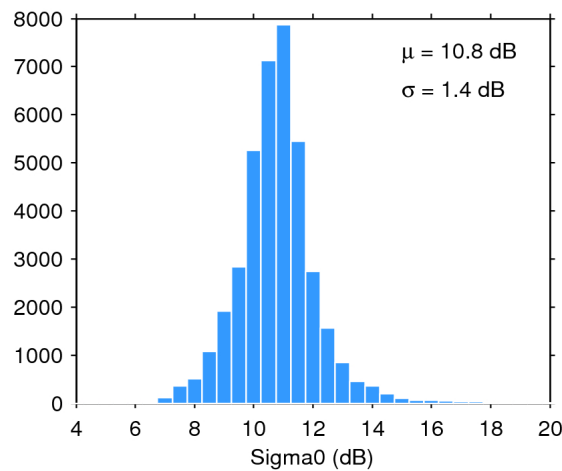
Figure 28. Histogram of science-valid sigma0 over oceans and lakes for 29/12/2019. The mean ( \mu ) and standard deviation ( \sigma ) are also shown. Note that values outside [4 20] dB are excluded from the histogram for the sake of readability but not from the computation of \mu and \sigma .
