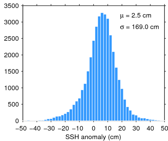
Figure 7. Histogram of flag-valid SSH anomaly over oceans and lakes for 29/12/2019. The mean ( \mu ) and standard deviation ( \sigma ) are also shown. Note that values outside [-50\ 50] cm are excluded from the histogram for the sake of readability but not from the computation of \mu and \sigma .
