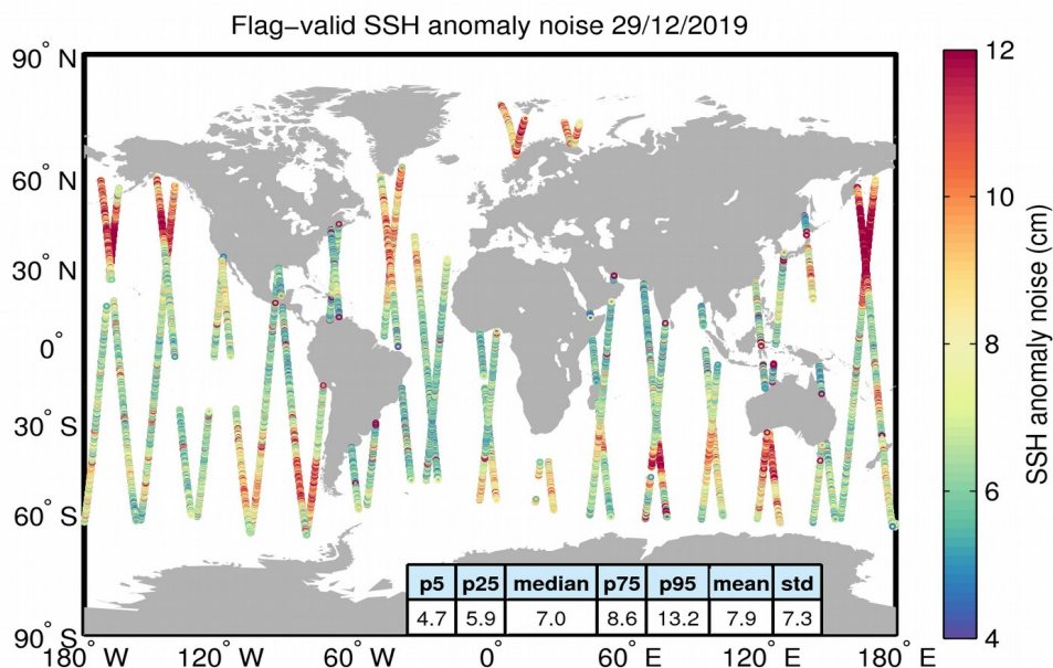
Figure 8. Geographical distribution of flag-valid 20-Hz SSH anomaly measurement noise over oceans and lakes for 29/12/2019. The statistical values shown in the table refer to the SSH anomaly noise and are calculated over all measurements shown in the figure.
