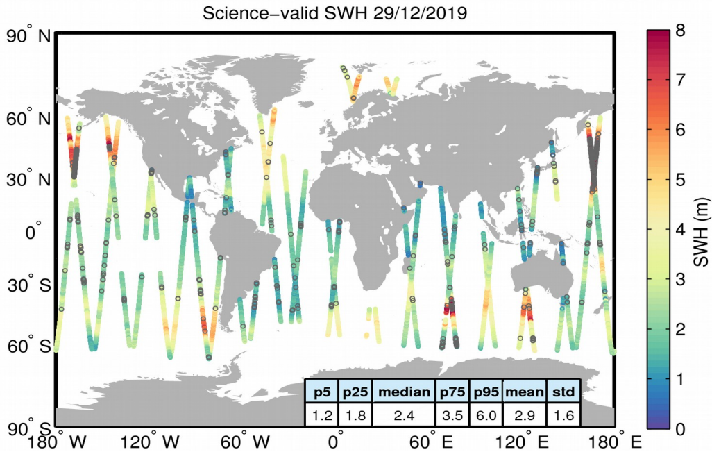
Figure 19. Geographical distribution of science-valid SWH data over oceans and lakes for 29/12/2019. The statistical values shown in the table refer to the SWH in m and are calculated over all measurements shown in the figure. Gray circles denote records that have been rejected based on the editing criteria described in Table 3.
