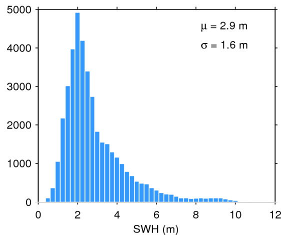
Figure 20. Histogram of science-valid SWH over oceans and lakes for 29/12/2019. The mean ( \mu ) and standard deviation ( \sigma ) are also shown. Note that values larger than 12 m are excluded from the histogram for the sake of readability but not from the computation of \mu and \sigma .
