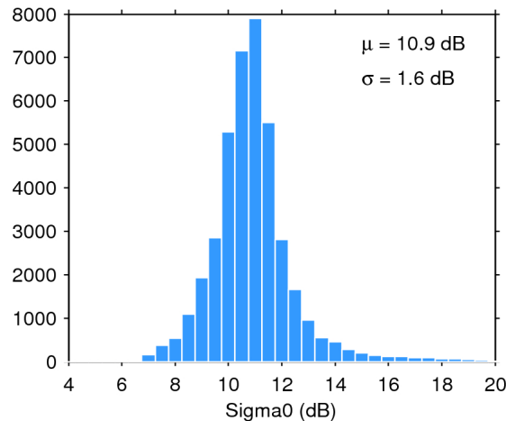
Figure 25. Histogram of flag-valid sigma0 over oceans and lakes for 29/12/2019. The mean ( \mu ) and standard deviation ( \sigma ) are also shown. Note that values outside [4 20] dB are excluded from the histogram for the sake of readability but not from the computation of \mu and \sigma .
