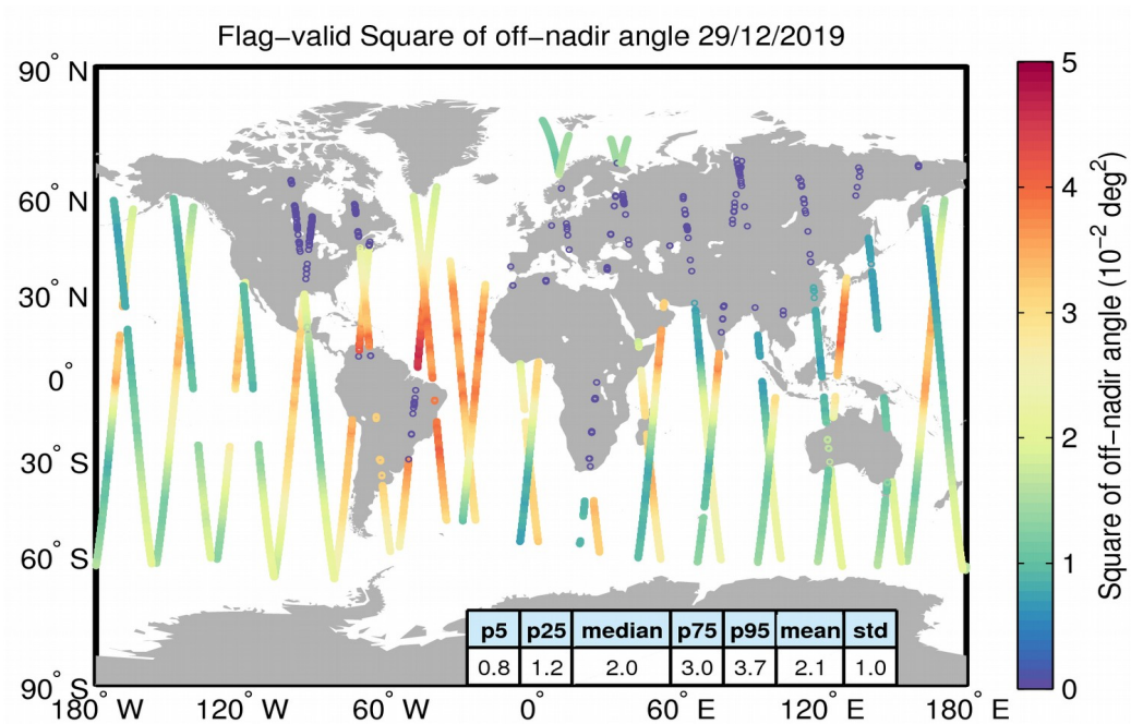
Figure 37. Geographical distribution of flag-valid mispointing data over oceans and lakes for 29/12/2019. The statistical values shown in the table refer to the mispointing in 10^{-2} deg 2 and are calculated over all measurements shown in the figure.
