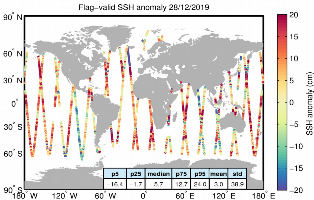
Figure 5. Geographical distribution of flag-valid 1-Hz SSH anomaly data over oceans and lakes for 28/12/2019. The statistical values shown in the table refer to the SSH anomaly in cm and are calculated over all measurements shown in the figure.
