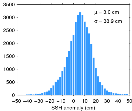
Figure 7. Histogram of flag-valid SSH anomaly over oceans and lakes for 28/12/2019. The mean ( \mu ) and standard deviation ( \sigma ) are also shown. Note that values outside [-50\ 50] cm are excluded from the histogram for the sake of readability but not from the computation of \mu and \sigma .
