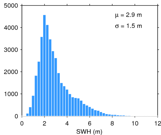
Figure 20. Histogram of science-valid SWH over oceans and lakes for 28/12/2019. The mean ( \mu ) and standard deviation ( \sigma ) are also shown. Note that values larger than 12 m are excluded from the histogram for the sake of readability but not from the computation of \mu and \sigma .
