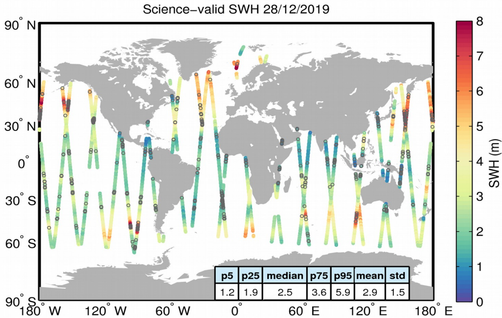
Figure 19. Geographical distribution of science-valid SWH data over oceans and lakes for 28/12/2019. The statistical values shown in the table refer to the SWH in m and are calculated over all measurements shown in the figure. Gray circles denote records that have been rejected based on the editing criteria described in Table 3.
