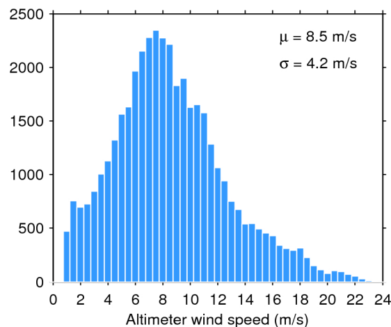
Figure 35. Histogram of science-valid wind over oceans and lakes for 28/12/2019. The mean ( \mu ) and standard deviation ( \sigma ) are also shown. Note that values larger than 24 m/s are excluded from the histogram for the sake of readability but not from the computation of \mu and \sigma .
