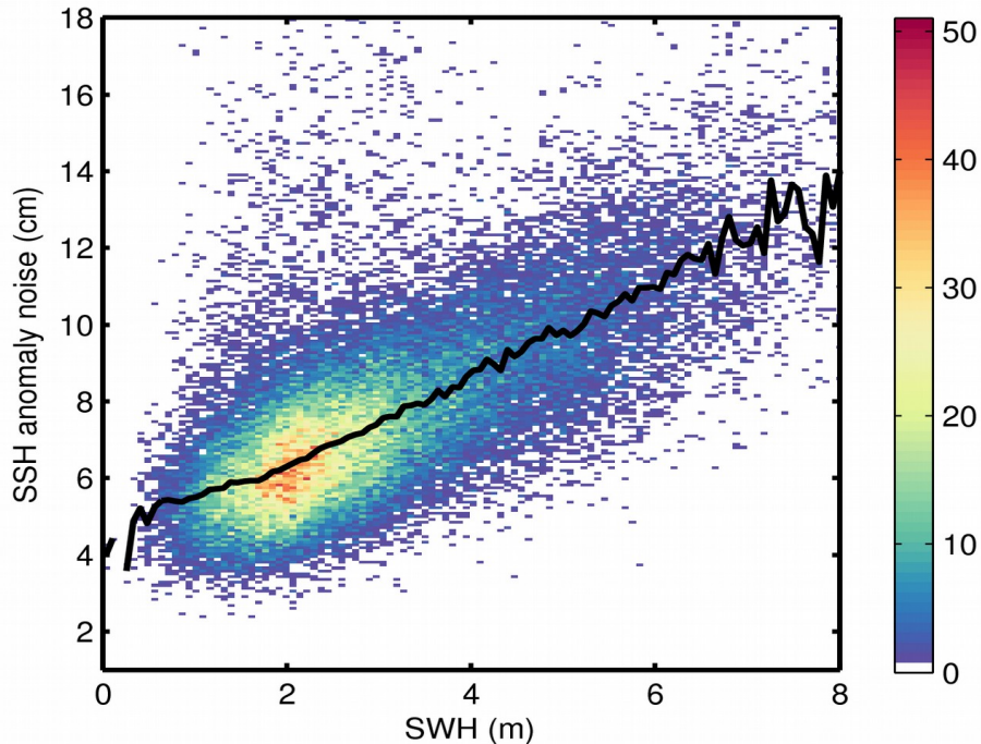
Figure 9. 2D histogram showing flag-valid SSH anomaly noise as a function of SWH for 28/12/2019. The black line denotes the median SSH anomaly noise as a function of SWH.
