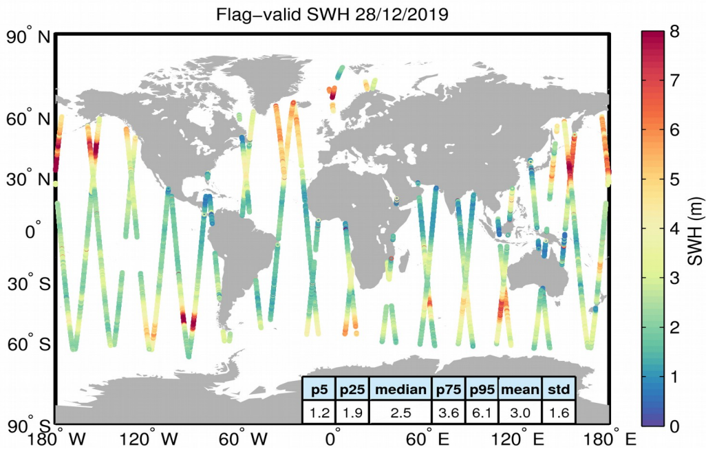
Figure 15. Geographical distribution of flag-valid SWH data over oceans and lakes for 28/12/2019. The statistical values shown in the table refer to the SWH in m and are calculated over all measurements shown in the figure.
