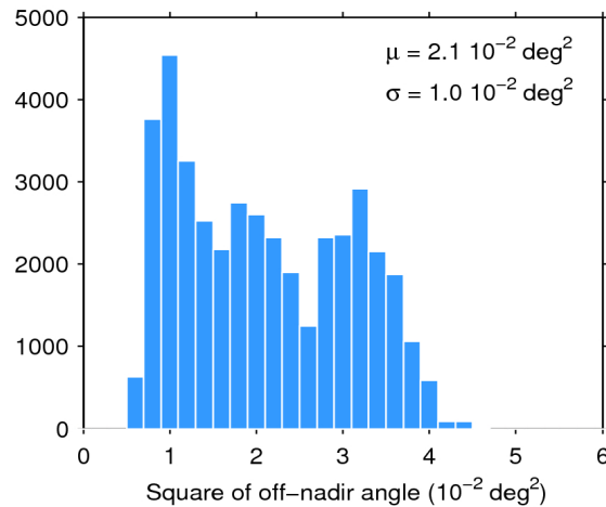
Figure 39. Histogram of flag-valid mispointing over oceans and lakes for 28/12/2019. The mean ( \mu ) and standard deviation ( \sigma ) are also shown. Note that values larger than 6 \cdot 10^{-2} \text{ deg}^2 are excluded from the histogram for the sake of readability but not from the computation of \mu and \sigma .
