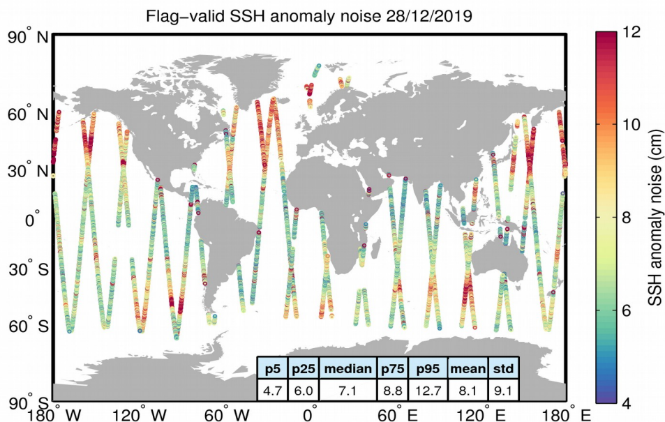
Figure 8. Geographical distribution of flag-valid 20-Hz SSH anomaly measurement noise over oceans and lakes for 28/12/2019. The statistical values shown in the table refer to the SSH anomaly noise and are calculated over all measurements shown in the figure.
