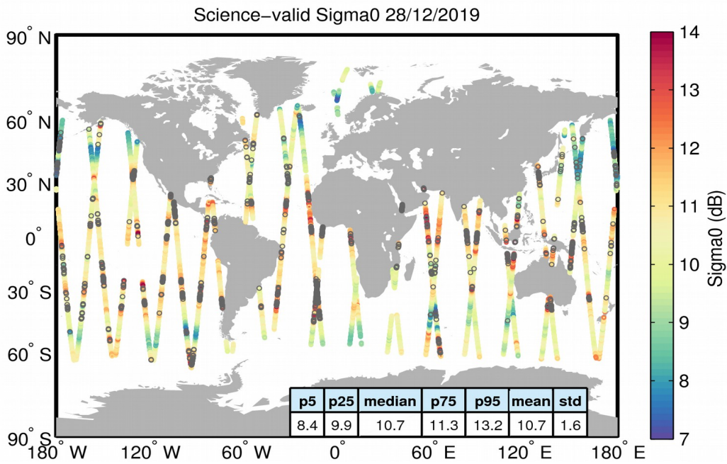
Figure 27. Geographical distribution of science-valid sigma0 data over oceans and lakes for 28/12/2019. The statistical values shown in the table refer to the sigma0 in dB and are calculated over all measurements shown in the figure. Gray circles denote records that have been rejected based on the editing criteria described in Table 4.
