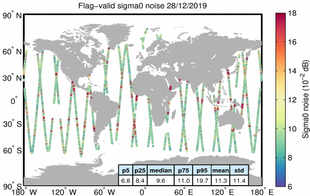
Figure 26. Geographical distribution of flag-valid 20-Hz sigma0 measurement noise over oceans and lakes for 28/12/2019. The statistical values shown in the table refer to the sigma0 noise and are calculated over all measurements shown in the figure.
