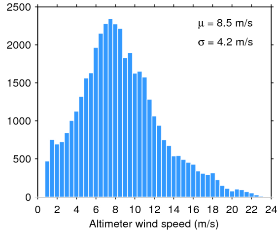
Figure 33. Histogram of flag-valid wind over oceans and lakes for 28/12/2019. The mean ( \mu ) and standard deviation ( \sigma ) are also shown. Note that values larger than 24 m/s are excluded from the histogram for the sake of readability but not from the computation of \mu and \sigma .
