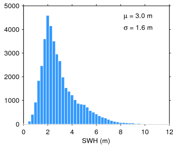
Figure 17. Histogram of flag-valid SWH over oceans and lakes for 28/12/2019. The mean ( \mu ) and standard deviation ( \sigma ) are also shown. Note that values larger than 12 m are excluded from the histogram for the sake of readability but not from the computation of \mu and \sigma .
