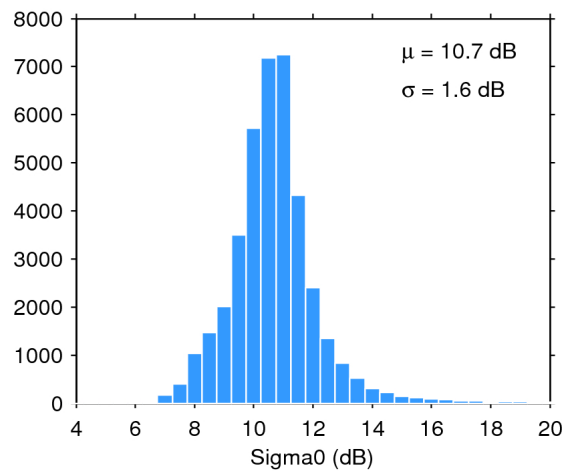
Figure 28. Histogram of science-valid sigma0 over oceans and lakes for 28/12/2019. The mean ( \mu ) and standard deviation ( \sigma ) are also shown. Note that values outside [4 20] dB are excluded from the histogram for the sake of readability but not from the computation of \mu and \sigma .
