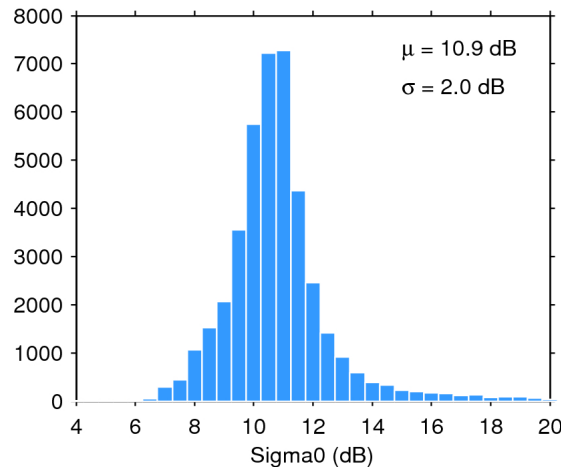
Figure 25. Histogram of flag-valid sigma0 over oceans and lakes for 28/12/2019. The mean ( \mu ) and standard deviation ( \sigma ) are also shown. Note that values outside [4 20] dB are excluded from the histogram for the sake of readability but not from the computation of \mu and \sigma .
