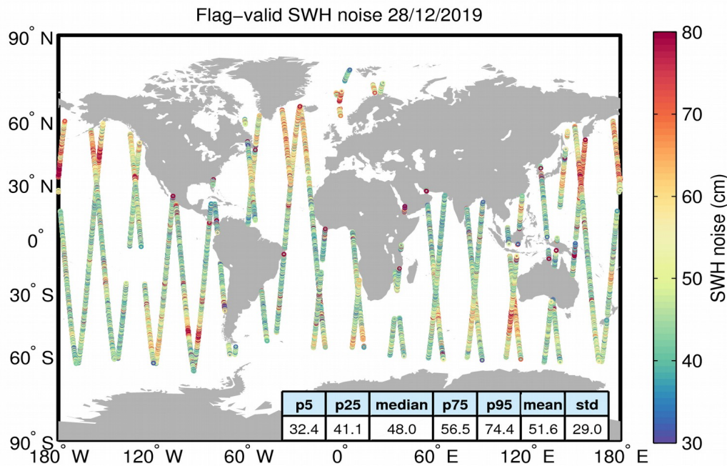
Figure 18. Geographical distribution of flag-valid 20-Hz SWH measurement noise over oceans and lakes for 28/12/2019. The statistical values shown in the figure refer to the SWH noise and are calculated over all measurements shown in the figure.
