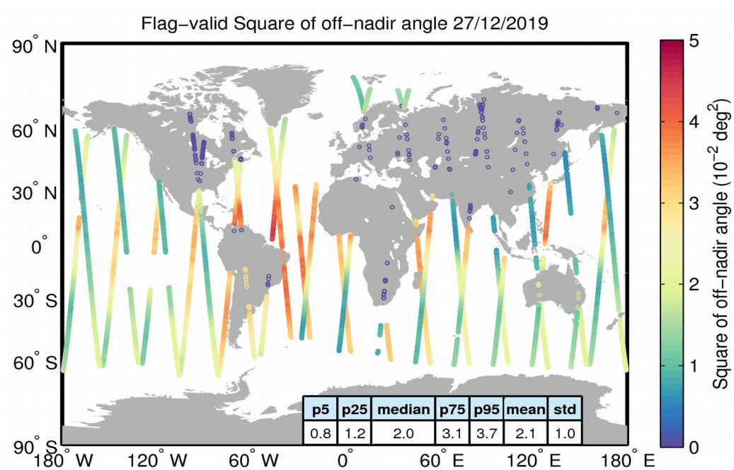
Figure 37. Geographical distribution of flag-valid mispointing data over oceans and lakes for 27/12/2019. The statistical values shown in the table refer to the mispointing in 10^{-2} \text{ deg}^2 and are calculated over all measurements shown in the figure.
