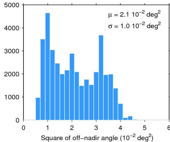
Figure 39. Histogram of flag-valid mispointing over oceans and lakes for 27/12/2019. The mean ( \mu ) and standard deviation ( \sigma ) are also shown. Note that values larger than 6 \cdot 10^{-2} \text{ deg}^2 are excluded from the histogram for the sake of readability but not from the computation of \mu and \sigma .
