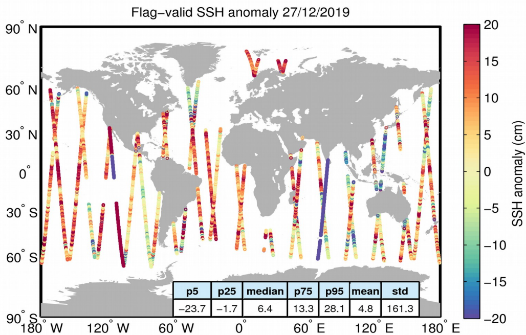
Figure 5. Geographical distribution of flag-valid 1-Hz SSH anomaly data over oceans and lakes for 27/12/2019. The statistical values shown in the table refer to the SSH anomaly in cm and are calculated over all measurements shown in the figure.
