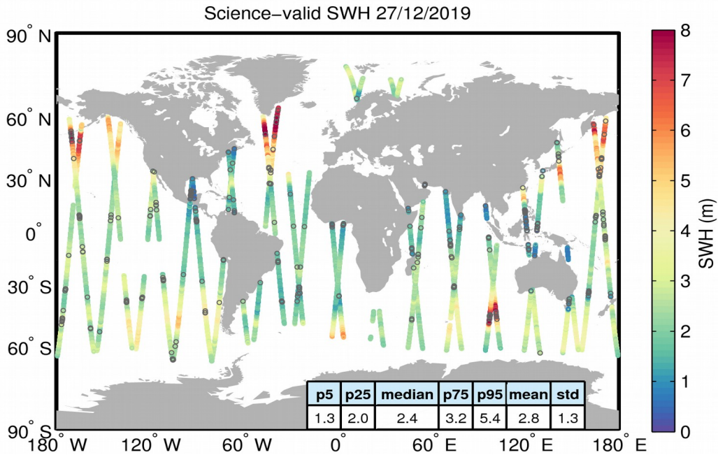
Figure 19. Geographical distribution of science-valid SWH data over oceans and lakes for 27/12/2019. The statistical values shown in the table refer to the SWH in m and are calculated over all measurements shown in the figure. Gray circles denote records that have been rejected based on the editing criteria described in Table 3.
