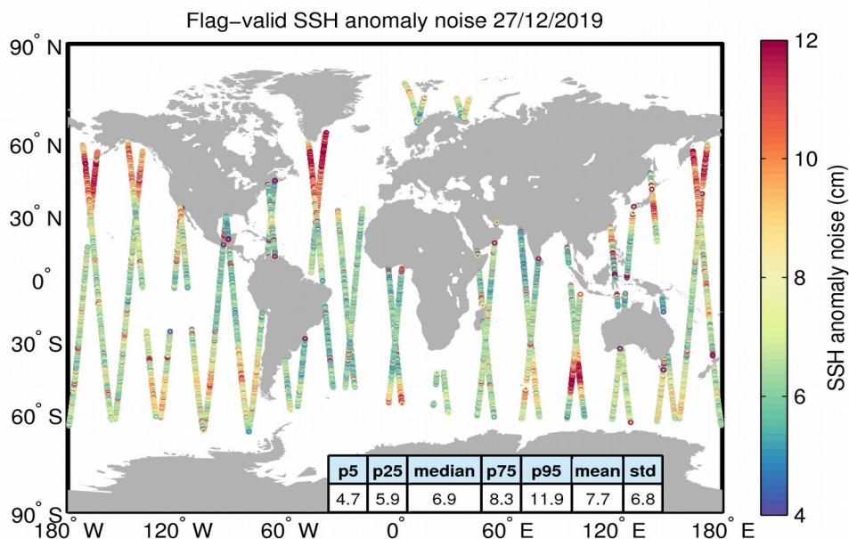
Figure 8. Geographical distribution of flag-valid 20-Hz SSH anomaly measurement noise over oceans and lakes for 27/12/2019. The statistical values shown in the table refer to the SSH anomaly noise and are calculated over all measurements shown in the figure.
