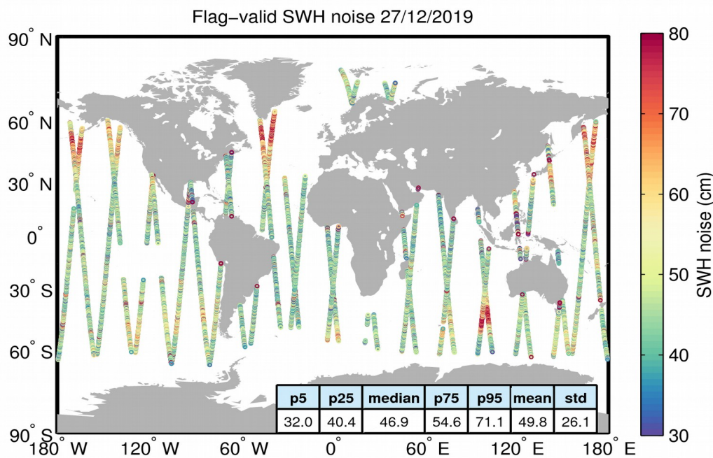
Figure 18. Geographical distribution of flag-valid 20-Hz SWH measurement noise over oceans and lakes for 27/12/2019. The statistical values shown in the figure refer to the SWH noise and are calculated over all measurements shown in the figure.
