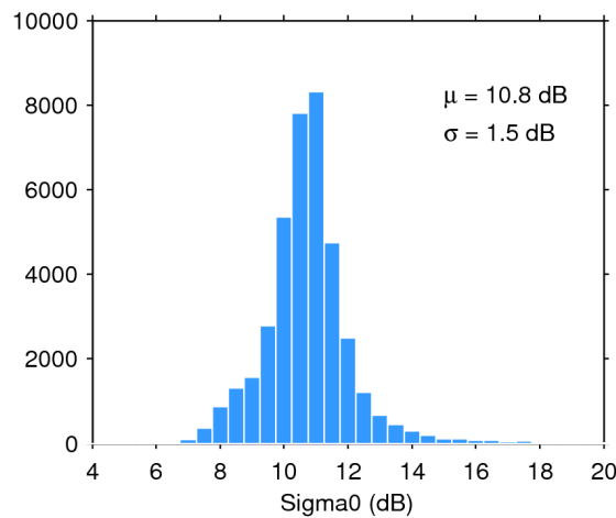
Figure 28. Histogram of science-valid sigma0 over oceans and lakes for 27/12/2019. The mean ( \mu ) and standard deviation ( \sigma ) are also shown. Note that values outside [4 20] dB are excluded from the histogram for the sake of readability but not from the computation of \mu and \sigma .
