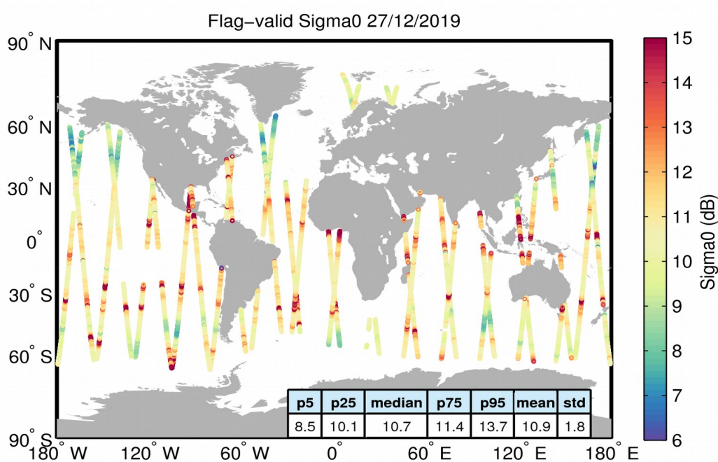
Figure 23. Geographical distribution of flag-valid sigma0 data over oceans and lakes for 27/12/2019. The statistical values shown in the table refer to the sigma0 in dB and are calculated over all measurements shown in the figure.
