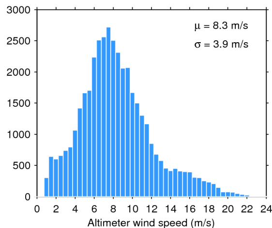
Figure 35. Histogram of science-valid wind over oceans and lakes for 27/12/2019. The mean ( \mu ) and standard deviation ( \sigma ) are also shown. Note that values larger than 24 m/s are excluded from the histogram for the sake of readability but not from the computation of \mu and \sigma .
