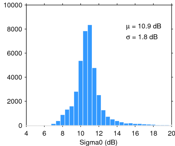
Figure 25. Histogram of flag-valid sigma0 over oceans and lakes for 27/12/2019. The mean ( \mu ) and standard deviation ( \sigma ) are also shown. Note that values outside [4 20] dB are excluded from the histogram for the sake of readability but not from the computation of \mu and \sigma .
