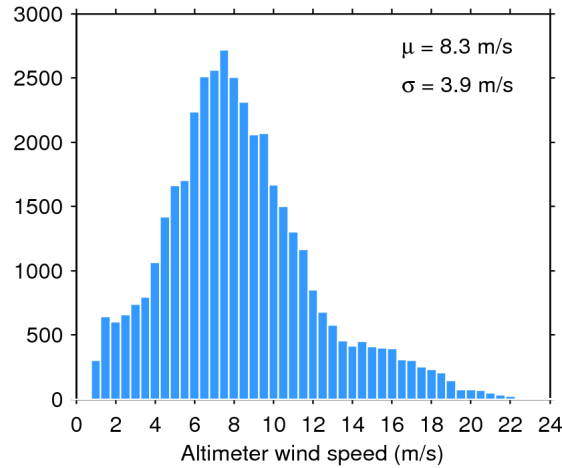
Figure 33. Histogram of flag-valid wind over oceans and lakes for 27/12/2019. The mean ( \mu ) and standard deviation ( \sigma ) are also shown. Note that values larger than 24 m/s are excluded from the histogram for the sake of readability but not from the computation of \mu and \sigma .
