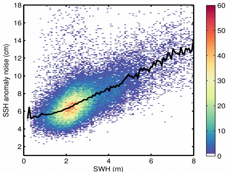
Figure 9. 2D histogram showing flag-valid SSH anomaly noise as a function of SWH for 27/12/2019. The black line denotes the median SSH anomaly noise as a function of SWH.
