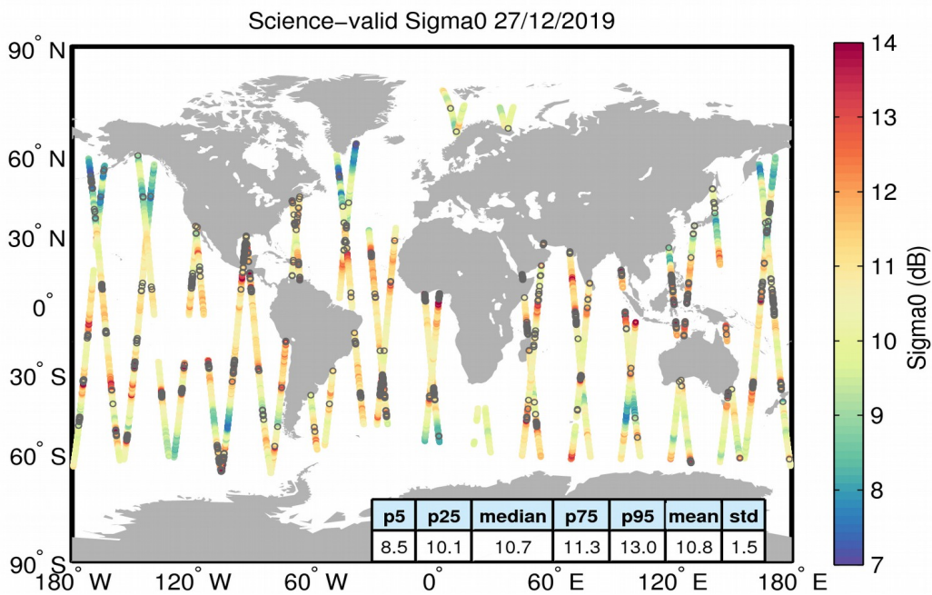
Figure 27. Geographical distribution of science-valid sigma0 data over oceans and lakes for 27/12/2019. The statistical values shown in the table refer to the sigma0 in dB and are calculated over all measurements shown in the figure. Gray circles denote records that have been rejected based on the editing criteria described in Table 4.
