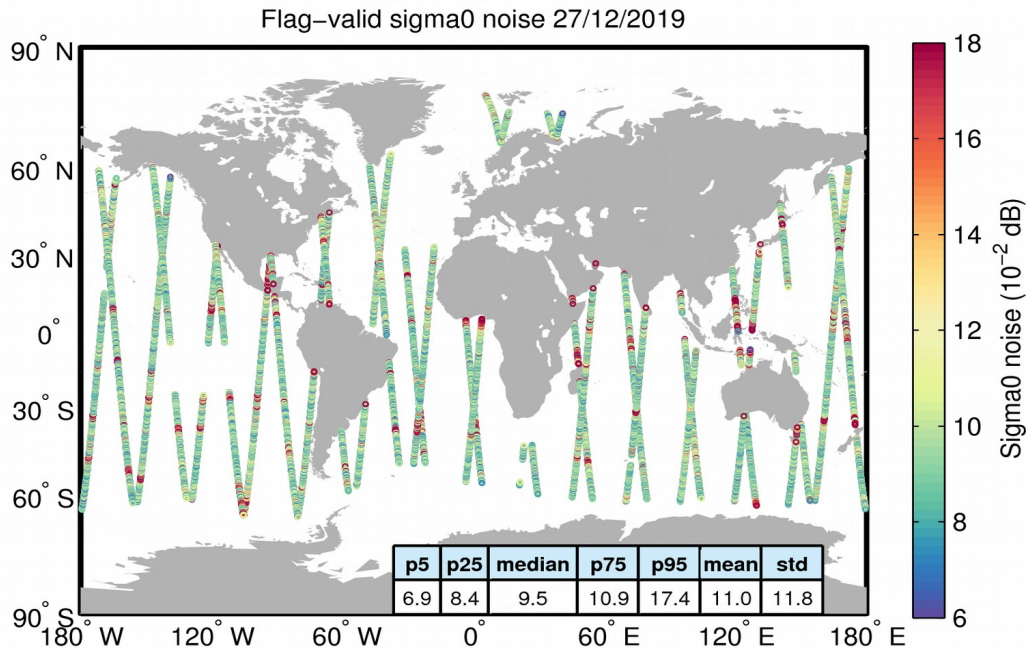
Figure 26. Geographical distribution of flag-valid 20-Hz sigma0 measurement noise over oceans and lakes for 27/12/2019. The statistical values shown in the table refer to the sigma0 noise and are calculated over all measurements shown in the figure.
