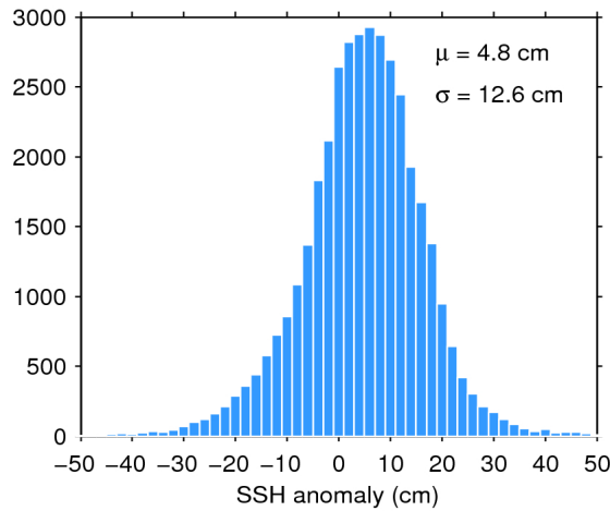
Figure 11. Histogram of science-valid SSH anomaly over oceans and lakes for 26/12/2019. The mean ( \mu ) and standard deviation ( \sigma ) are also shown. Note that values outside [-50 50] cm are excluded from the histogram for the sake of readability but not from the computation of \mu and \sigma .
