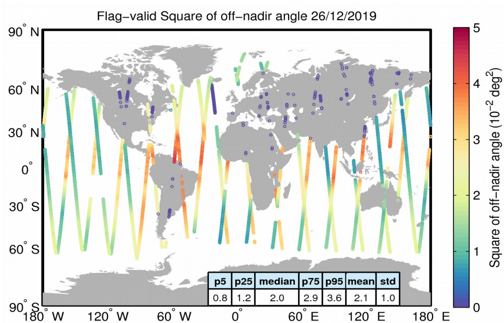
Figure 37. Geographical distribution of flag-valid mispointing data over oceans and lakes for 26/12/2019. The statistical values shown in the table refer to the mispointing in 10^{-2} \text{deg}^2 and are calculated over all measurements shown in the figure.
