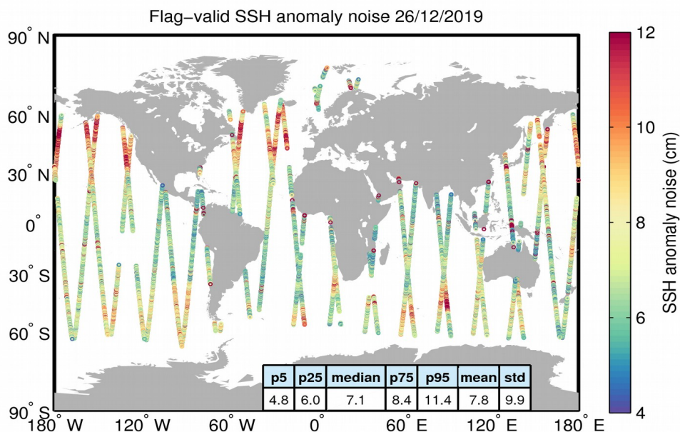
Figure 8. Geographical distribution of flag-valid 20-Hz SSH anomaly measurement noise over oceans and lakes for 26/12/2019. The statistical values shown in the table refer to the SSH anomaly noise and are calculated over all measurements shown in the figure.
