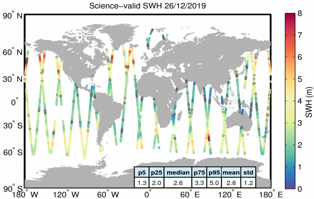
Figure 19. Geographical distribution of science-valid SWH data over oceans and lakes for 26/12/2019. The statistical values shown in the table refer to the SWH in m and are calculated over all measurements shown in the figure. Gray circles denote records that have been rejected based on the editing criteria described in Table 3.
