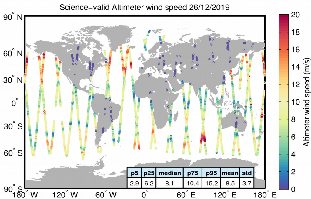
Figure 34. Geographical distribution of science-valid wind data over oceans and lakes for 26/12/2019. The statistical values shown in the table refer to the wind in m/s and are calculated over all measurements shown in the figure. Gray circles denote records that have been rejected based on the editing criteria described in Table 5.
