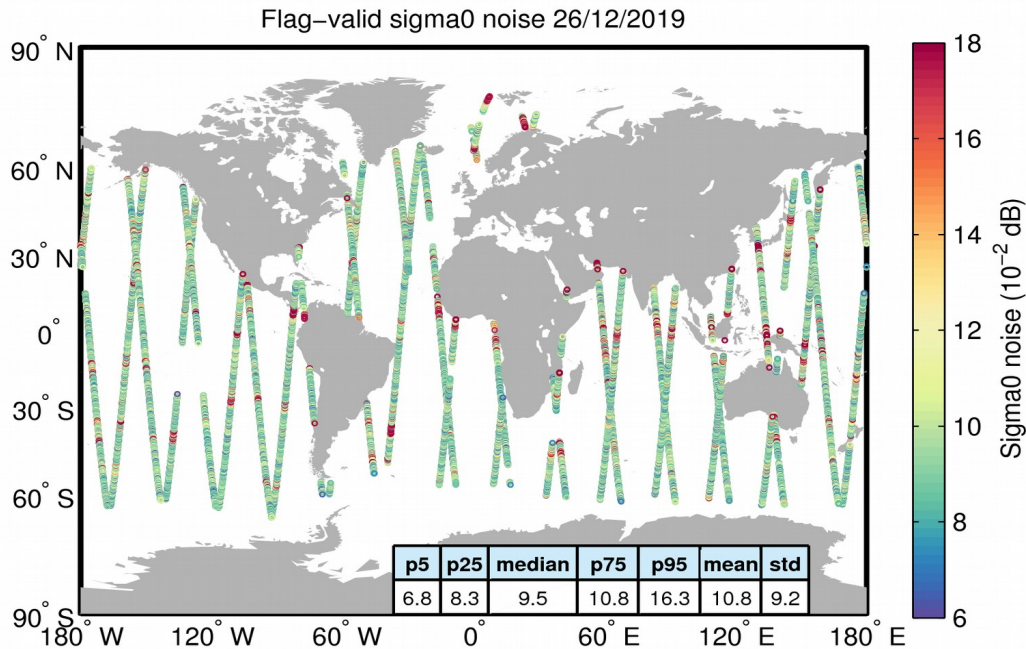
Figure 26. Geographical distribution of flag-valid 20-Hz sigma0 measurement noise over oceans and lakes for 26/12/2019. The statistical values shown in the table refer to the sigma0 noise and are calculated over all measurements shown in the figure.
