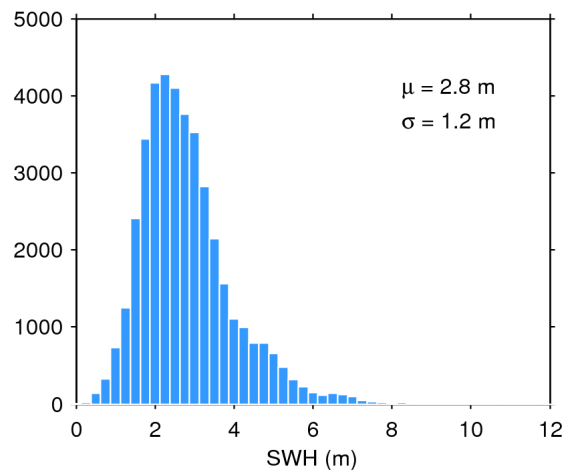
Figure 20. Histogram of science-valid SWH over oceans and lakes for 26/12/2019. The mean ( \mu ) and standard deviation ( \sigma ) are also shown. Note that values larger than 12 m are excluded from the histogram for the sake of readability but not from the computation of \mu and \sigma .
