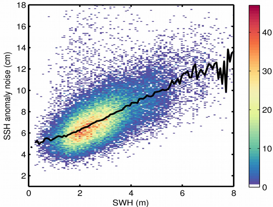
Figure 9. 2D histogram showing flag-valid SSH anomaly noise as a function of SWH for 26/12/2019. The black line denotes the median SSH anomaly noise as a function of SWH.
