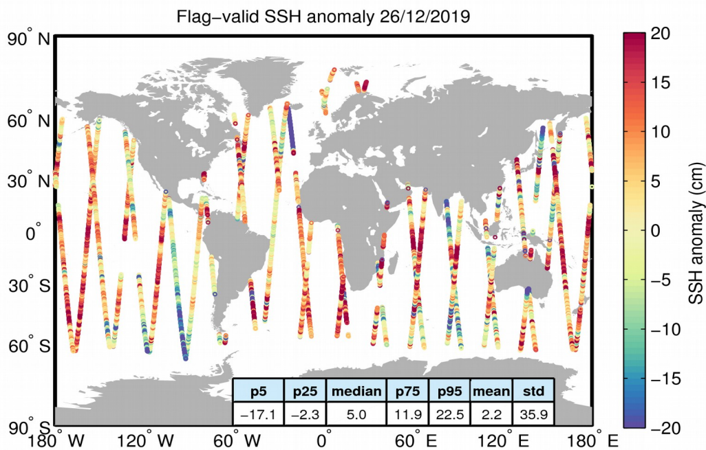
Figure 5. Geographical distribution of flag-valid 1-Hz SSH anomaly data over oceans and lakes for 26/12/2019. The statistical values shown in the table refer to the SSH anomaly in cm and are calculated over all measurements shown in the figure.
