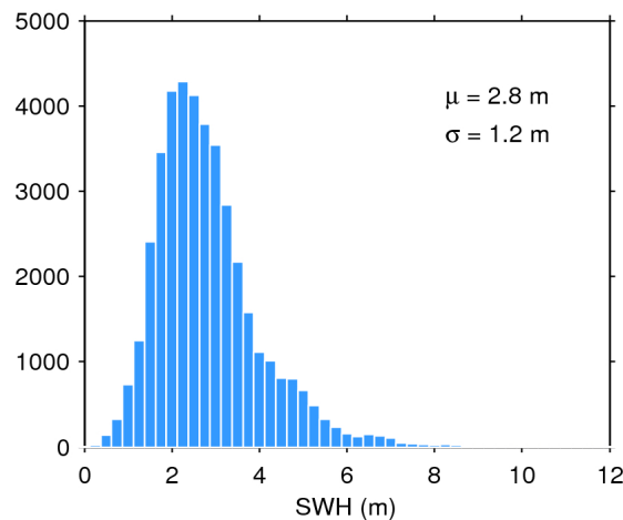
Figure 17. Histogram of flag-valid SWH over oceans and lakes for 26/12/2019. The mean ( \mu ) and standard deviation ( \sigma ) are also shown. Note that values larger than 12 m are excluded from the histogram for the sake of readability but not from the computation of \mu and \sigma .
