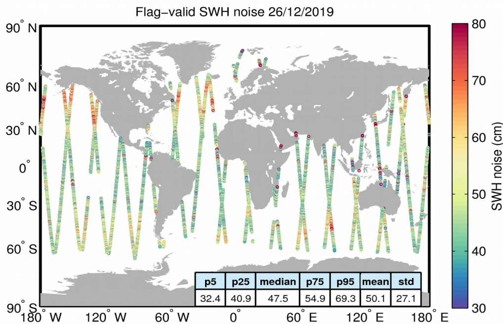
Figure 18. Geographical distribution of flag-valid 20-Hz SWH measurement noise over oceans and lakes for 26/12/2019. The statistical values shown in the figure refer to the SWH noise and are calculated over all measurements shown in the figure.
