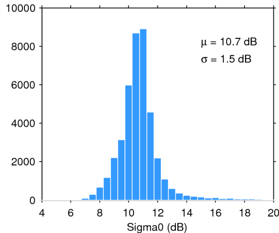
Figure 25. Histogram of flag-valid sigma0 over oceans and lakes for 26/12/2019. The mean ( \mu ) and standard deviation ( \sigma ) are also shown. Note that values outside [4 20] dB are excluded from the histogram for the sake of readability but not from the computation of \mu and \sigma .
