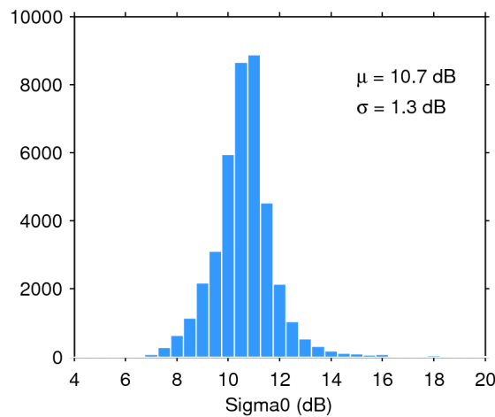
Figure 28. Histogram of science-valid sigma0 over oceans and lakes for 26/12/2019. The mean ( \mu ) and standard deviation ( \sigma ) are also shown. Note that values outside [4 20] dB are excluded from the histogram for the sake of readability but not from the computation of \mu and \sigma .
