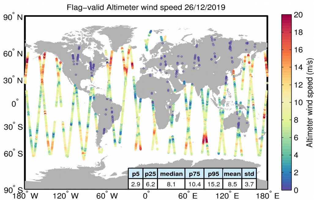
Figure 31. Geographical distribution of flag-valid wind data over oceans and lakes for 26/12/2019. The statistical values shown in the table refer to the wind in m/s and are calculated over all measurements shown in the figure.
