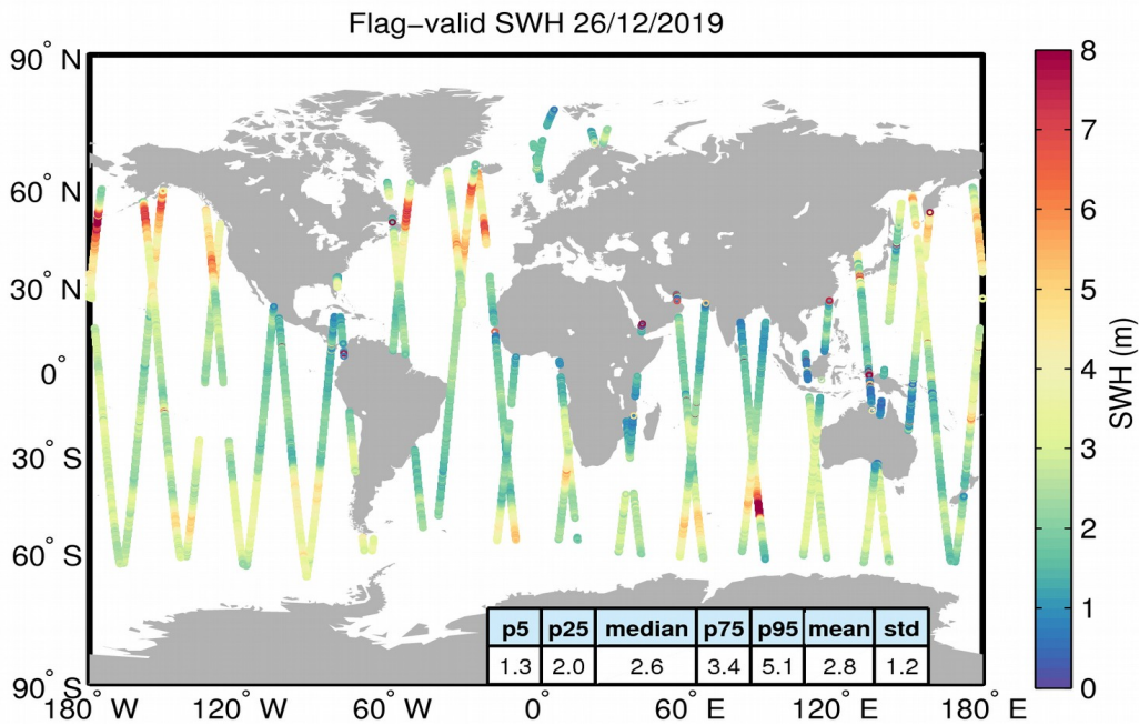
Figure 15. Geographical distribution of flag-valid SWH data over oceans and lakes for 26/12/2019. The statistical values shown in the table refer to the SWH in m and are calculated over all measurements shown in the figure.
