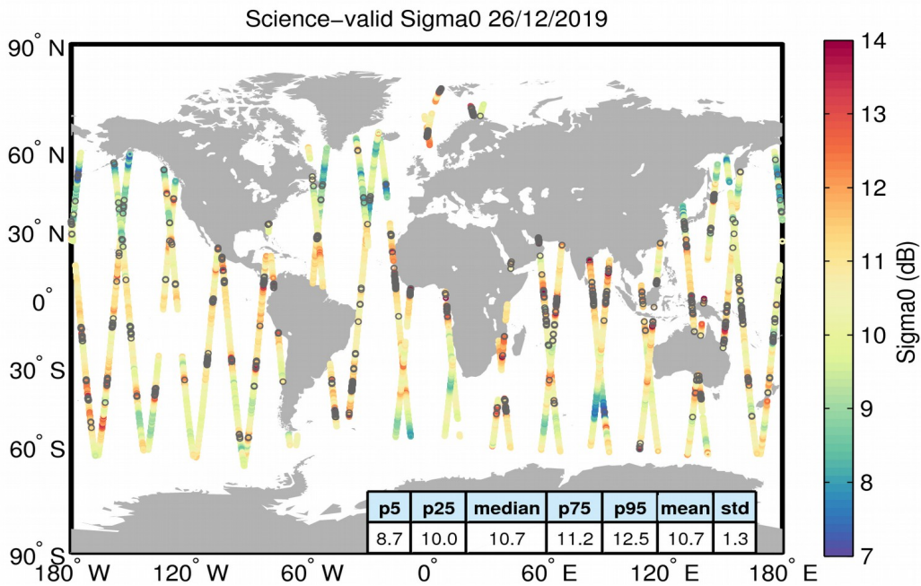
Figure 27. Geographical distribution of science-valid sigma0 data over oceans and lakes for 26/12/2019. The statistical values shown in the table refer to the sigma0 in dB and are calculated over all measurements shown in the figure. Gray circles denote records that have been rejected based on the editing criteria described in Table 4.
