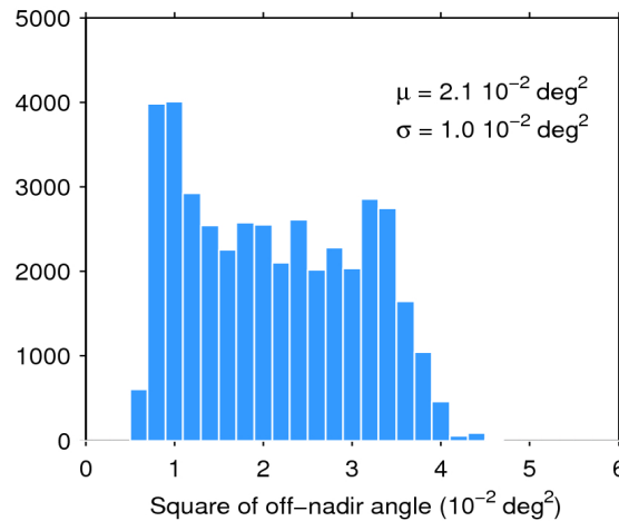
Figure 39. Histogram of flag-valid mispointing over oceans and lakes for 26/12/2019. The mean ( \mu ) and standard deviation ( \sigma ) are also shown. Note that values larger than 6 \cdot 10^{-2} \text{ deg}^2 are excluded from the histogram for the sake of readability but not from the computation of \mu and \sigma .
