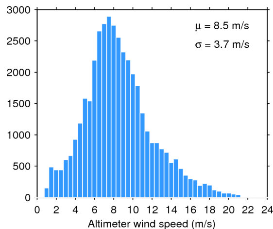
Figure 35. Histogram of science-valid wind over oceans and lakes for 26/12/2019. The mean ( \mu ) and standard deviation ( \sigma ) are also shown. Note that values larger than 24 m/s are excluded from the histogram for the sake of readability but not from the computation of \mu and \sigma .
