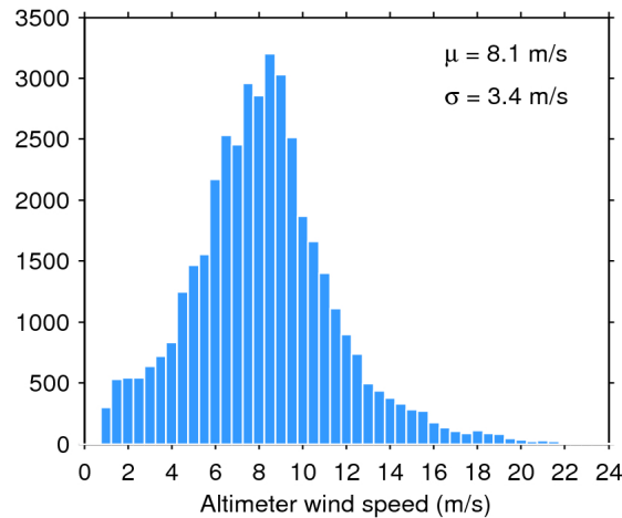
Figure 33. Histogram of flag-valid wind over oceans and lakes for 25/12/2019. The mean ( \mu ) and standard deviation ( \sigma ) are also shown. Note that values larger than 24 m/s are excluded from the histogram for the sake of readability but not from the computation of \mu and \sigma .
