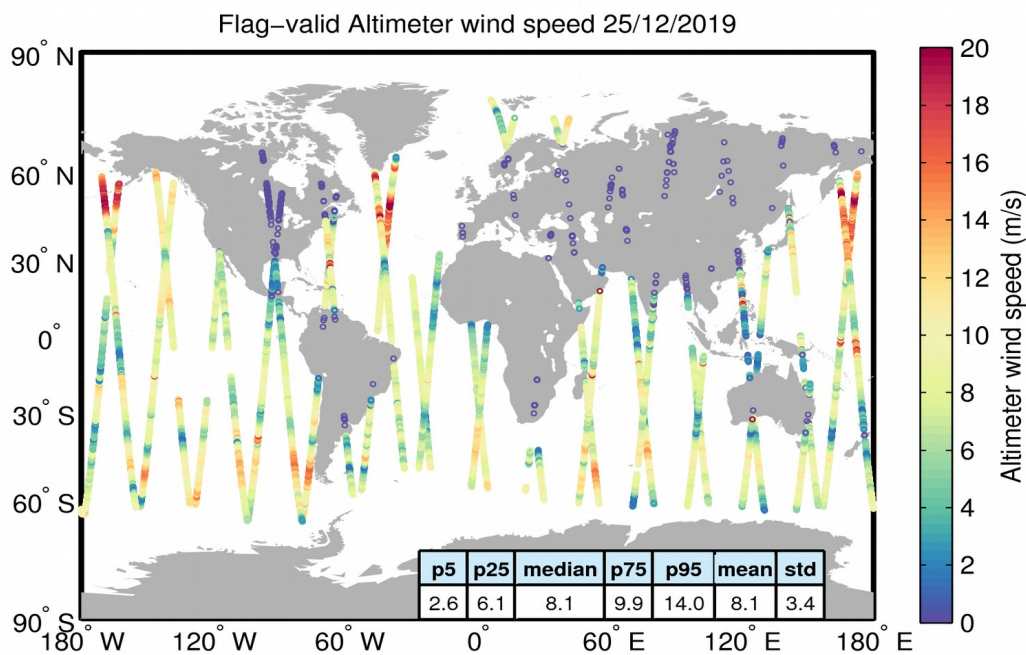
Figure 31. Geographical distribution of flag-valid wind data over oceans and lakes for 25/12/2019. The statistical values shown in the figure refer to the wind in m/s and are calculated over all measurements shown in the figure.
