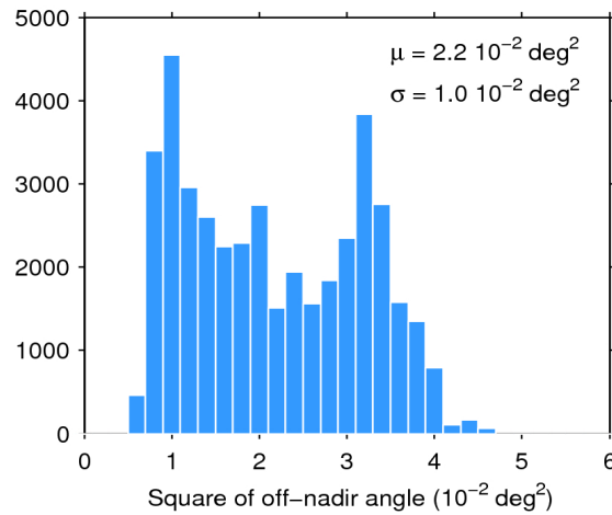
Figure 39. Histogram of flag-valid mispointing over oceans and lakes for 25/12/2019. The mean ( \mu ) and standard deviation ( \sigma ) are also shown. Note that values larger than 6 \cdot 10^{-2} \text{ deg}^2 are excluded from the histogram for the sake of readability but not from the computation of \mu and \sigma .
