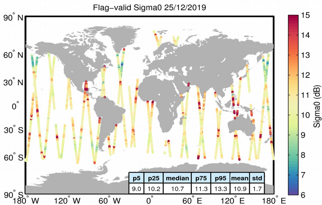
Figure 23. Geographical distribution of flag-valid sigma0 data over oceans and lakes for 25/12/2019. The statistical values shown in the table refer to the sigma0 in dB and are calculated over all measurements shown in the figure.
