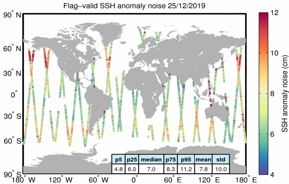
Figure 8. Geographical distribution of flag-valid 20-Hz SSH anomaly measurement noise over oceans and lakes for 25/12/2019. The statistical values shown in the table refer to the SSH anomaly noise and are calculated over all measurements shown in the figure.
