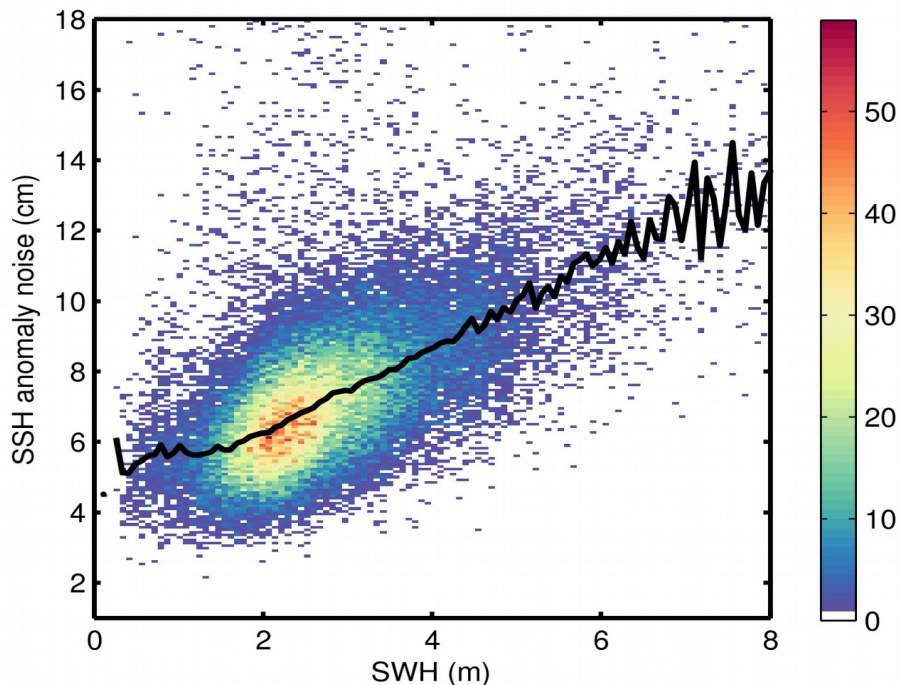
Figure 9. 2D histogram showing flag-valid SSH anomaly noise as a function of SWH for 25/12/2019. The black line denotes the median SSH anomaly noise as a function of SWH.
