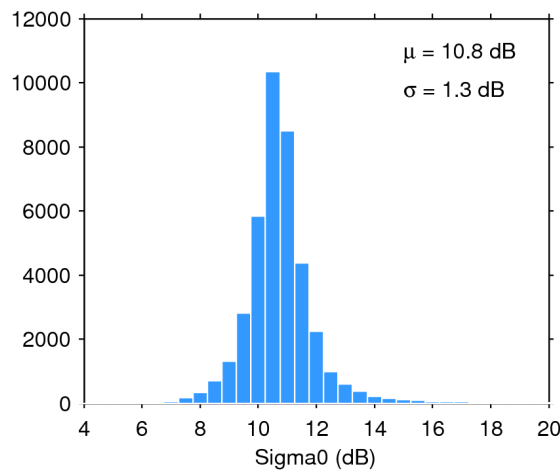
Figure 28. Histogram of science-valid sigma0 over oceans and lakes for 25/12/2019. The mean ( \mu ) and standard deviation ( \sigma ) are also shown. Note that values outside [4 20] dB are excluded from the histogram for the sake of readability but not from the computation of \mu and \sigma .
