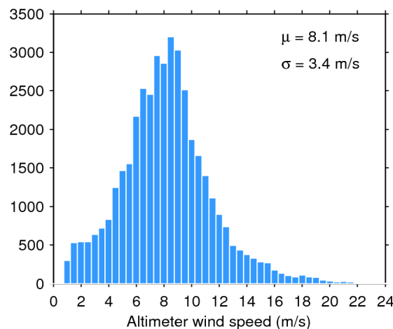
Figure 35. Histogram of science-valid wind over oceans and lakes for 25/12/2019. The mean ( \mu ) and standard deviation ( \sigma ) are also shown. Note that values larger than 24 m/s are excluded from the histogram for the sake of readability but not from the computation of \mu and \sigma .
