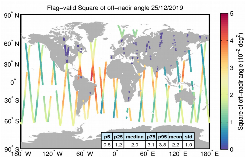
Figure 37. Geographical distribution of flag-valid mispointing data over oceans and lakes for 25/12/2019. The statistical values shown in the table refer to the mispointing in 10^{-2} deg 2 and are calculated over all measurements shown in the figure.
