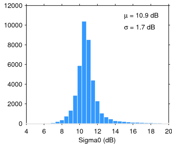
Figure 25. Histogram of flag-valid sigma0 over oceans and lakes for 25/12/2019. The mean ( \mu ) and standard deviation ( \sigma ) are also shown. Note that values outside [4 20] dB are excluded from the histogram for the sake of readability but not from the computation of \mu and \sigma .
