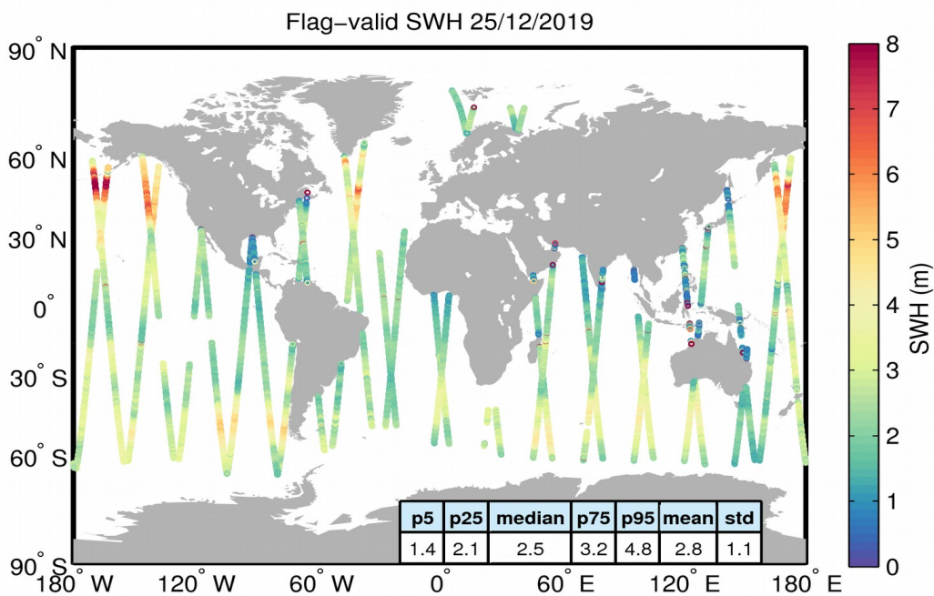
Figure 15. Geographical distribution of flag-valid SWH data over oceans and lakes for 25/12/2019. The statistical values shown in the table refer to the SWH in m and are calculated over all measurements shown in the figure.
