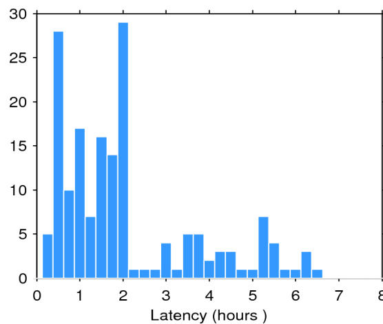
Figure 2. Histogram of the data latency for 25/12/2019. The y-axis denotes the number of files that are made available with a delay of x-hours with respect to the mean time of the records stored in the file.
