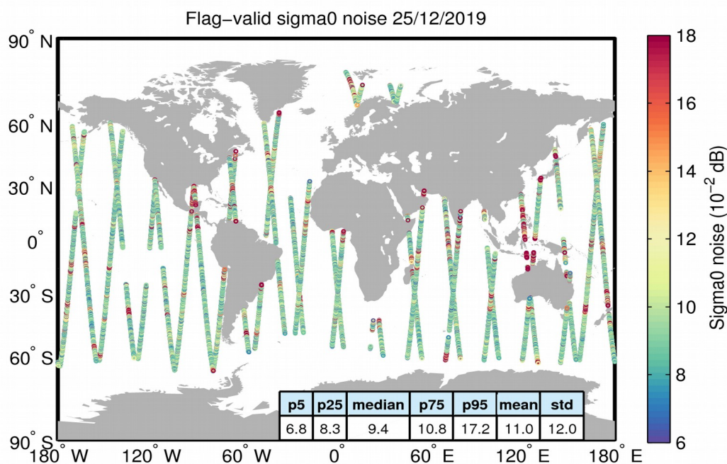
Figure 26. Geographical distribution of flag-valid 20-Hz sigma0 measurement noise over oceans and lakes for 25/12/2019. The statistical values shown in the table refer to the sigma0 noise and are calculated over all measurements shown in the figure.
