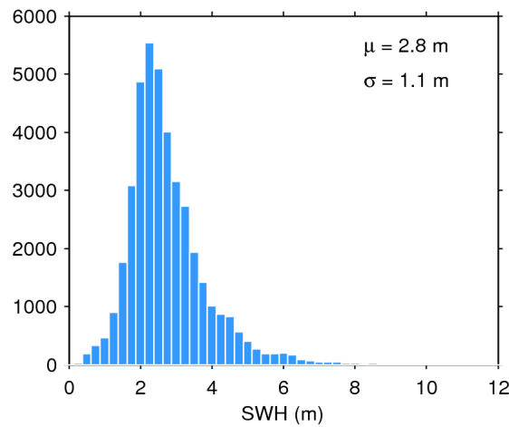
Figure 17. Histogram of flag-valid SWH over oceans and lakes for 25/12/2019. The mean ( \mu ) and standard deviation ( \sigma ) are also shown. Note that values larger than 12 m are excluded from the histogram for the sake of readability but not from the computation of \mu and \sigma .
