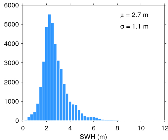
Figure 20. Histogram of science-valid SWH over oceans and lakes for 25/12/2019. The mean ( \mu ) and standard deviation ( \sigma ) are also shown. Note that values larger than 12 m are excluded from the histogram for the sake of readability but not from the computation of \mu and \sigma .
