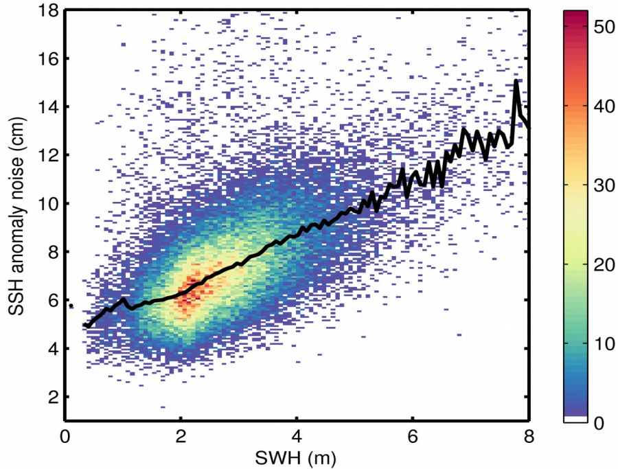
Figure 9. 2D histogram showing flag-valid SSH anomaly noise as a function of SWH for 24/12/2019. The black line denotes the median SSH anomaly noise as a function of SWH.
