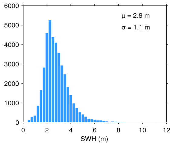
Figure 17. Histogram of flag-valid SWH over oceans and lakes for 24/12/2019. The mean ( \mu ) and standard deviation ( \sigma ) are also shown. Note that values larger than 12 m are excluded from the histogram for the sake of readability but not from the computation of \mu and \sigma .
