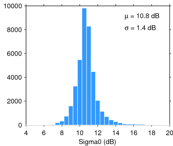
Figure 28. Histogram of science-valid sigma0 over oceans and lakes for 24/12/2019. The mean ( \mu ) and standard deviation ( \sigma ) are also shown. Note that values outside [4 20] dB are excluded from the histogram for the sake of readability but not from the computation of \mu and \sigma .
