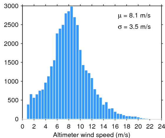
Figure 35. Histogram of science-valid wind over oceans and lakes for 24/12/2019. The mean ( \mu ) and standard deviation ( \sigma ) are also shown. Note that values larger than 24 m/s are excluded from the histogram for the sake of readability but not from the computation of \mu and \sigma .
