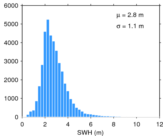
Figure 20. Histogram of science-valid SWH over oceans and lakes for 24/12/2019. The mean ( \mu ) and standard deviation ( \sigma ) are also shown. Note that values larger than 12 m are excluded from the histogram for the sake of readability but not from the computation of \mu and \sigma .
