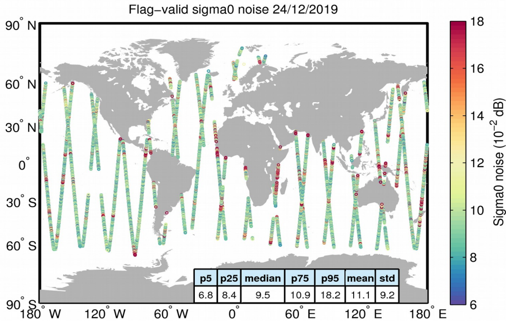
Figure 26. Geographical distribution of flag-valid 20-Hz sigma0 measurement noise over oceans and lakes for 24/12/2019. The statistical values shown in the table refer to the sigma0 noise and are calculated over all measurements shown in the figure.
