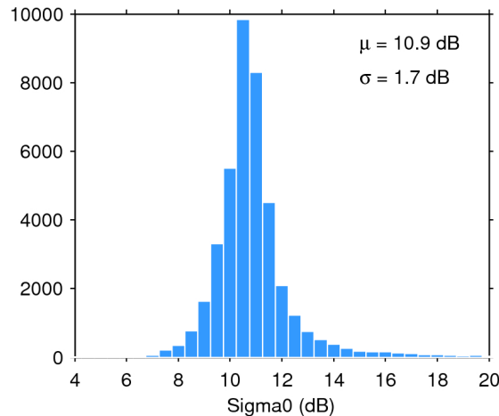
Figure 25. Histogram of flag-valid sigma0 over oceans and lakes for 24/12/2019. The mean ( \mu ) and standard deviation ( \sigma ) are also shown. Note that values outside [4 20] dB are excluded from the histogram for the sake of readability but not from the computation of \mu and \sigma .
