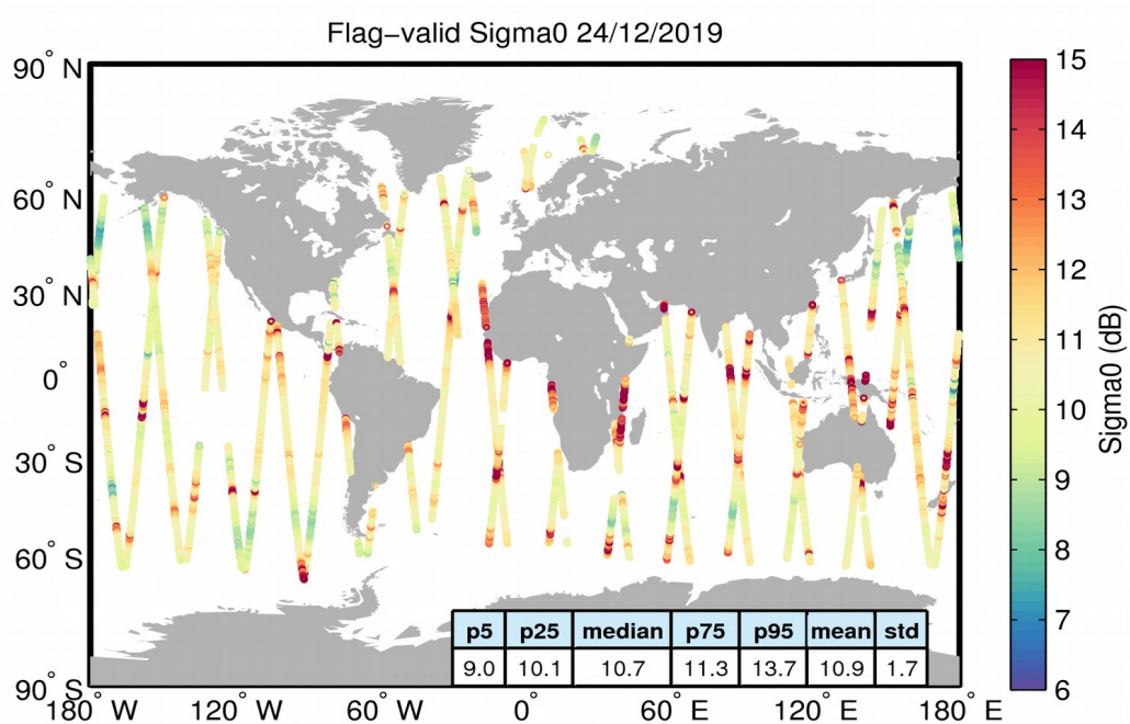
Figure 23. Geographical distribution of flag-valid sigma0 data over oceans and lakes for 24/12/2019. The statistical values shown in the table refer to the sigma0 in dB and are calculated over all measurements shown in the figure.
