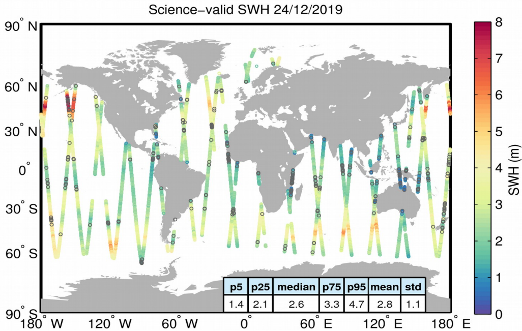
Figure 19. Geographical distribution of science-valid SWH data over oceans and lakes for 24/12/2019. The statistical values shown in the table refer to the SWH in m and are calculated over all measurements shown in the figure. Gray circles denote records that have been rejected based on the editing criteria described in Table 3.
