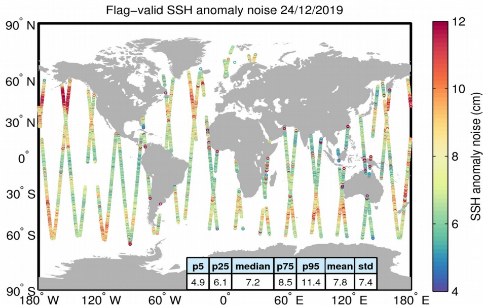
Figure 8. Geographical distribution of flag-valid 20-Hz SSH anomaly measurement noise over oceans and lakes for 24/12/2019. The statistical values shown in the table refer to the SSH anomaly noise and are calculated over all measurements shown in the figure.
