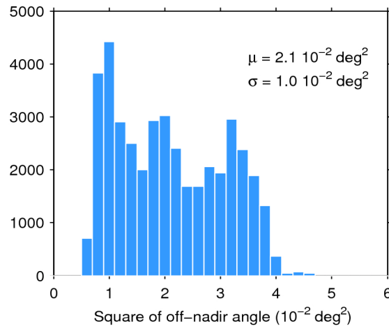
Figure 39. Histogram of flag-valid mispointing over oceans and lakes for 24/12/2019. The mean ( \mu ) and standard deviation ( \sigma ) are also shown. Note that values larger than 6 \cdot 10^{-2} \text{ deg}^2 are excluded from the histogram for the sake of readability but not from the computation of \mu and \sigma .
