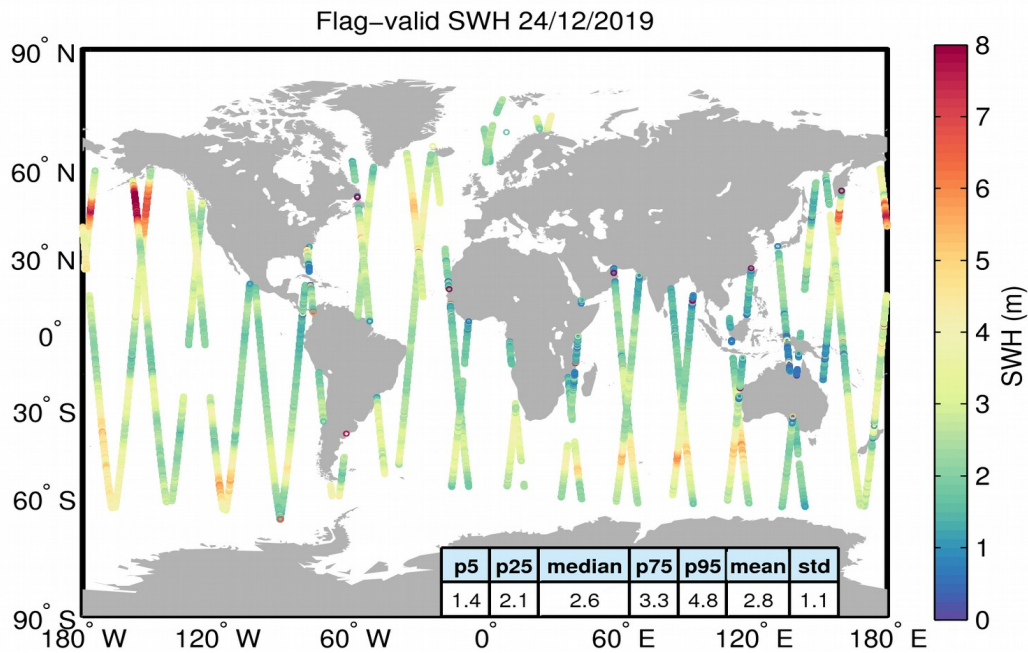
Figure 15. Geographical distribution of flag-valid SWH data over oceans and lakes for 24/12/2019. The statistical values shown in the table refer to the SWH in m and are calculated over all measurements shown in the figure.
