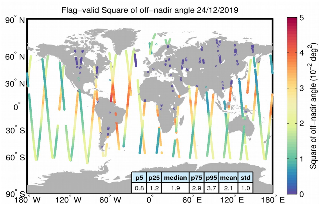
Figure 37. Geographical distribution of flag-valid mispointing data over oceans and lakes for 24/12/2019. The statistical values shown in the table refer to the mispointing in 10^{-2} deg 2 and are calculated over all measurements shown in the figure.
