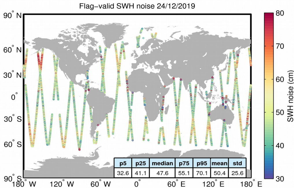
Figure 18. Geographical distribution of flag-valid 20-Hz SWH measurement noise over oceans and lakes for 24/12/2019. The statistical values shown in the table refer to the SWH noise and are calculated over all measurements shown in the figure.
