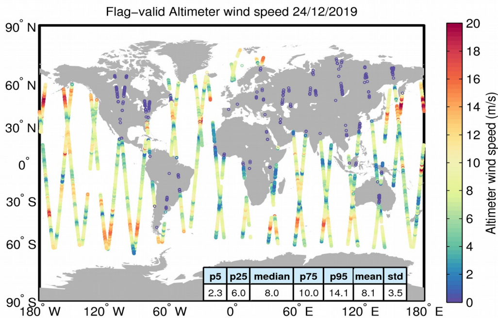
Figure 31. Geographical distribution of flag-valid wind data over oceans and lakes for 24/12/2019. The statistical values shown in the table refer to the wind in m/s and are calculated over all measurements shown in the figure.
