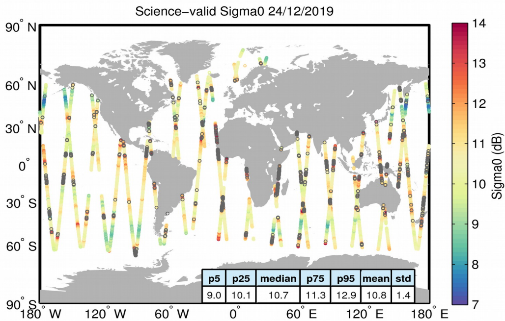
Figure 27. Geographical distribution of science-valid sigma0 data over oceans and lakes for 24/12/2019. The statistical values shown in the table refer to the sigma0 in dB and are calculated over all measurements shown in the figure. Gray circles denote records that have been rejected based on the editing criteria described in Table 4.
