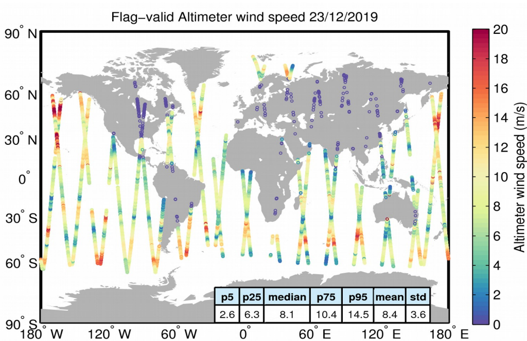
Figure 31. Geographical distribution of flag-valid wind data over oceans and lakes for 23/12/2019. The statistical values shown in the table refer to the wind in m/s and are calculated over all measurements shown in the figure.
