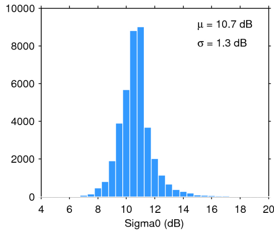
Figure 28. Histogram of science-valid sigma0 over oceans and lakes for 23/12/2019. The mean ( \mu ) and standard deviation ( \sigma ) are also shown. Note that values outside [4 20] dB are excluded from the histogram for the sake of readability but not from the computation of \mu and \sigma .
