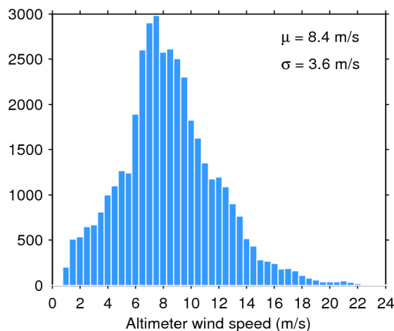
Figure 35. Histogram of science-valid wind over oceans and lakes for 23/12/2019. The mean ( \mu ) and standard deviation ( \sigma ) are also shown. Note that values larger than 24 m/s are excluded from the histogram for the sake of readability but not from the computation of \mu and \sigma .
