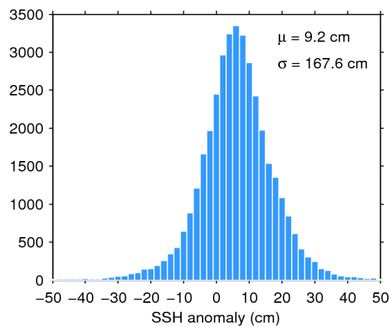
Figure 7. Histogram of flag-valid SSH anomaly over oceans and lakes for 23/12/2019. The mean ( \mu ) and standard deviation ( \sigma ) are also shown. Note that values outside [-50 50] cm are excluded from the histogram for the sake of readability but not from the computation of \mu and \sigma .
