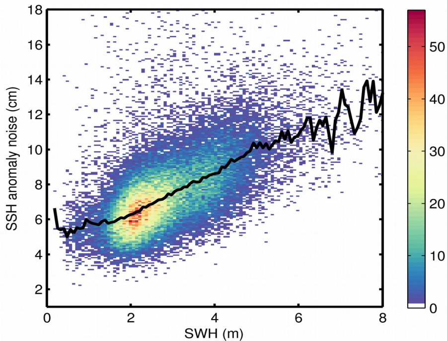
Figure 9. 2D histogram showing flag-valid SSH anomaly noise as a function of SWH for 23/12/2019. The black line denotes the median SSH anomaly noise as a function of SWH.
