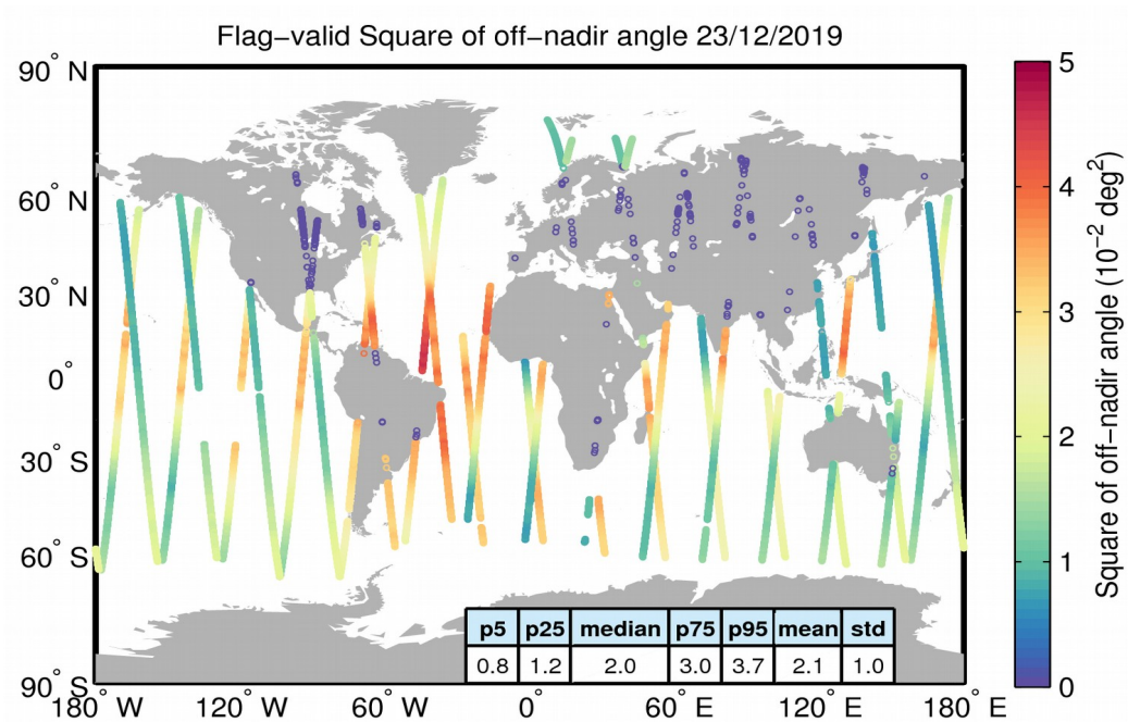
Figure 37. Geographical distribution of flag-valid mispointing data over oceans and lakes for 23/12/2019. The statistical values shown in the table refer to the mispointing in 10^{-2} \text{deg}^2 and are calculated over all measurements shown in the figure.
