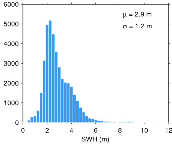
Figure 20. Histogram of science-valid SWH over oceans and lakes for 23/12/2019. The mean ( \mu ) and standard deviation ( \sigma ) are also shown. Note that values larger than 12 m are excluded from the histogram for the sake of readability but not from the computation of \mu and \sigma .
