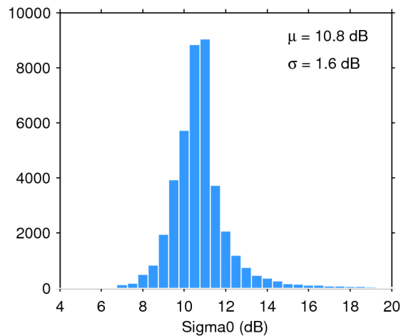
Figure 25. Histogram of flag-valid sigma0 over oceans and lakes for 23/12/2019. The mean ( \mu ) and standard deviation ( \sigma ) are also shown. Note that values outside [4 20] dB are excluded from the histogram for the sake of readability but not from the computation of \mu and \sigma .
