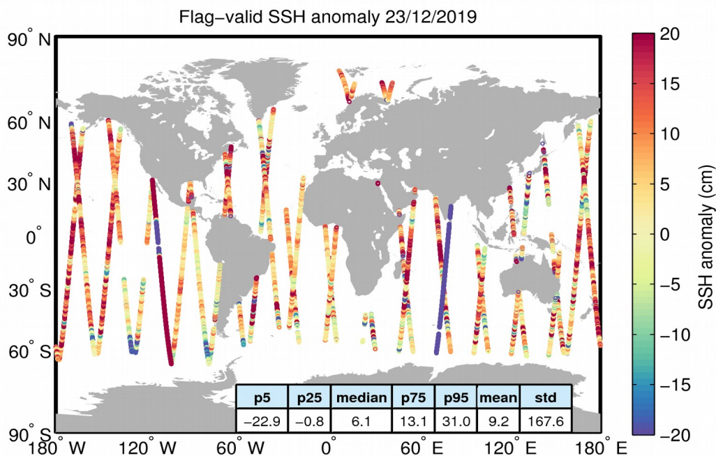
Figure 5. Geographical distribution of flag-valid 1-Hz SSH anomaly data over oceans and lakes for 23/12/2019. The statistical values shown in the table refer to the SSH anomaly in cm and are calculated over all measurements shown in the figure.
