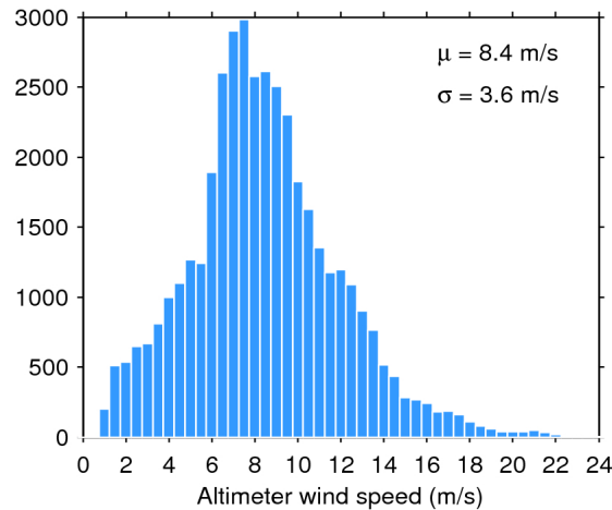
Figure 33. Histogram of flag-valid wind over oceans and lakes for 23/12/2019. The mean ( \mu ) and standard deviation ( \sigma ) are also shown. Note that values larger than 24 m/s are excluded from the histogram for the sake of readability but not from the computation of \mu and \sigma .
