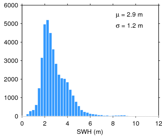
Figure 17. Histogram of flag-valid SWH over oceans and lakes for 23/12/2019. The mean ( \mu ) and standard deviation ( \sigma ) are also shown. Note that values larger than 12 m are excluded from the histogram for the sake of readability but not from the computation of \mu and \sigma .
