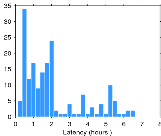
Figure 2. Histogram of the data latency for 23/12/2019. The y-axis denotes the number of files that are made available with a delay of x-hours with respect to the mean time of the records stored in the file.
