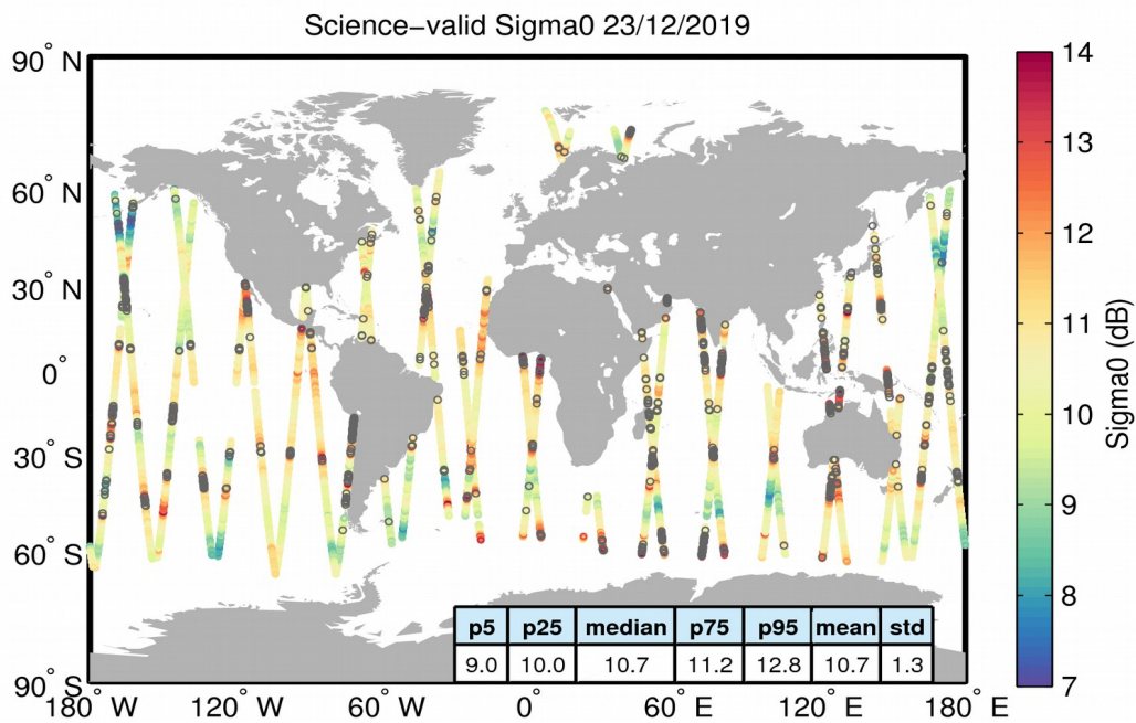
Figure 27. Geographical distribution of science-valid sigma0 data over oceans and lakes for 23/12/2019. The statistical values shown in the table refer to the sigma0 in dB and are calculated over all measurements shown in the figure. Gray circles denote records that have been rejected based on the editing criteria described in Table 4.
