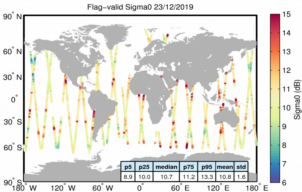
Figure 23. Geographical distribution of flag-valid sigma0 data over oceans and lakes for 23/12/2019. The statistical values shown in the table refer to the sigma0 in dB and are calculated over all measurements shown in the figure.
