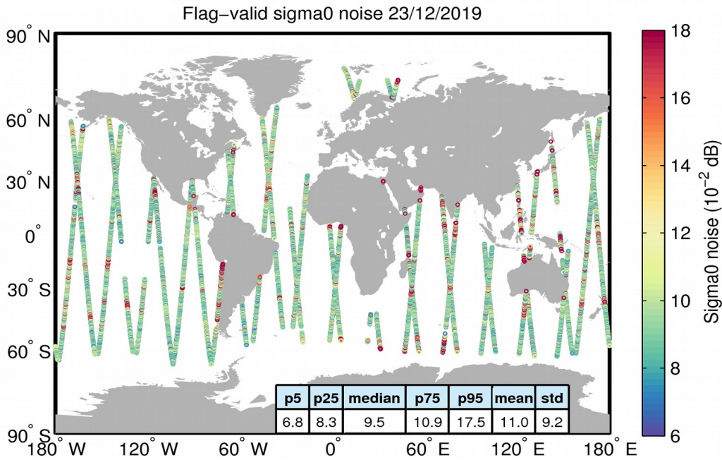
Figure 26. Geographical distribution of flag-valid 20-Hz sigma0 measurement noise over oceans and lakes for 23/12/2019. The statistical values shown in the table refer to the sigma0 noise and are calculated over all measurements shown in the figure.
