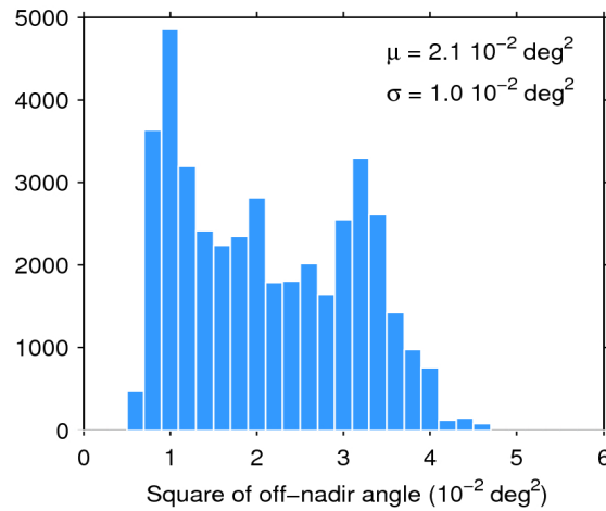
Figure 39. Histogram of flag-valid mispointing over oceans and lakes for 23/12/2019. The mean ( \mu ) and standard deviation ( \sigma ) are also shown. Note that values larger than 6 \cdot 10^{-2} \text{ deg}^2 are excluded from the histogram for the sake of readability but not from the computation of \mu and \sigma .
