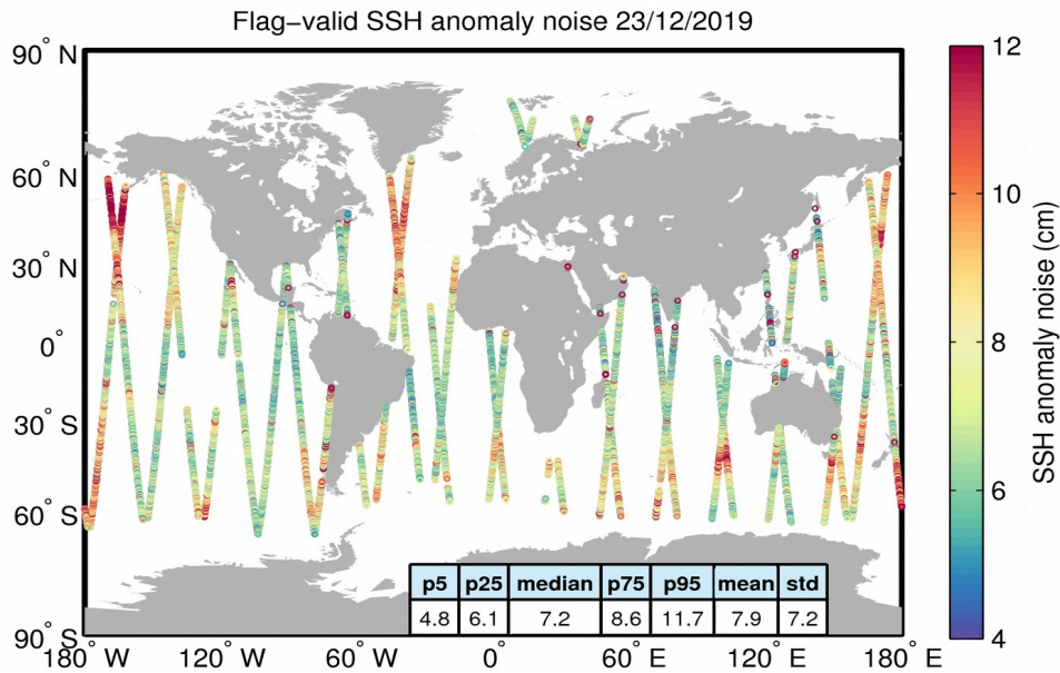
Figure 8. Geographical distribution of flag-valid 20-Hz SSH anomaly measurement noise over oceans and lakes for 23/12/2019. The statistical values shown in the table refer to the SSH anomaly noise and are calculated over all measurements shown in the figure.
