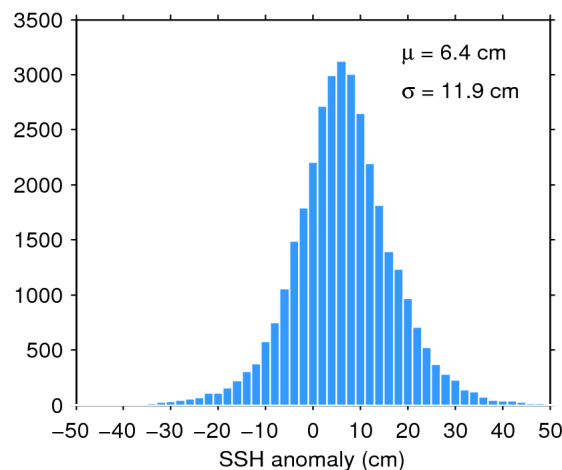
Figure 11. Histogram of science-valid SSH anomaly over oceans and lakes for 23/12/2019. The mean ( \mu ) and standard deviation ( \sigma ) are also shown. Note that values outside [-50 50] cm are excluded from the histogram for the sake of readability but not from the computation of \mu and \sigma .
