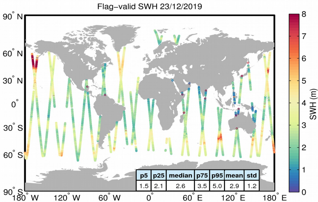
Figure 15. Geographical distribution of flag-valid SWH data over oceans and lakes for 23/12/2019. The statistical values shown in the table refer to the SWH in m and are calculated over all measurements shown in the figure.
